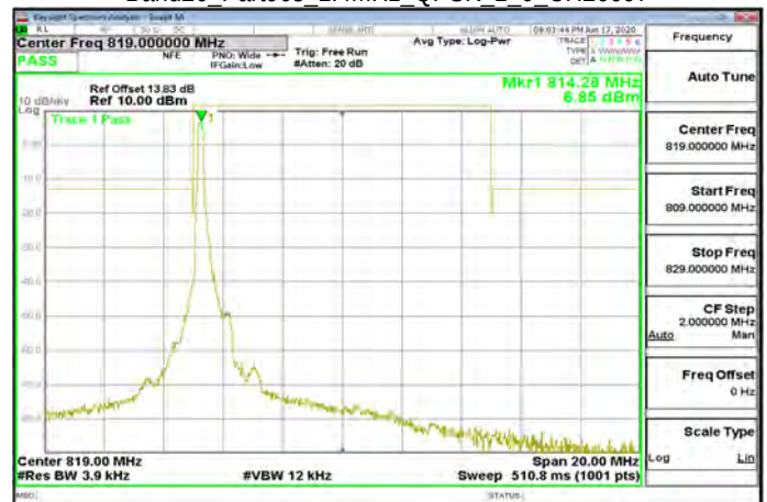
Band26 Part90s 1.4MHz_QPSK_1_0_CH26697
