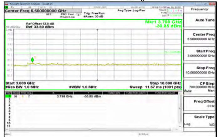
3GHz~10GHz_EDGE_850MHz_HighCH251-848.8
