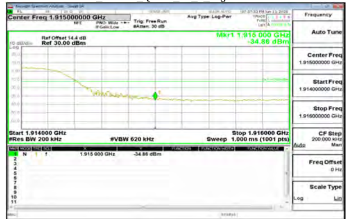
LTE\Band25_15MHz_QPSK_75_0_HighCH26615-1907.5
