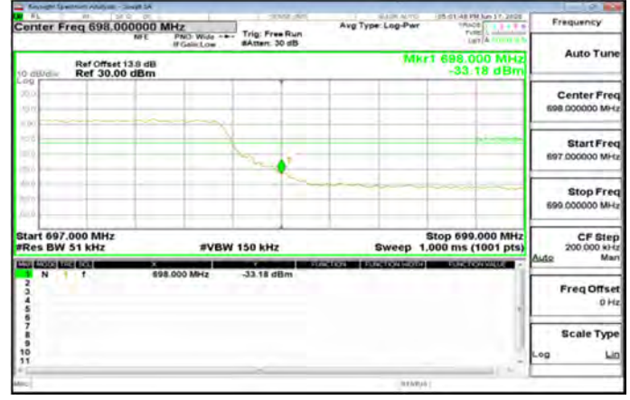
LTE\Band71 5MHz QPSK 25 0 HighCH133447-695.5
