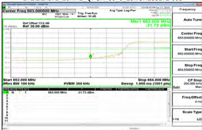
LTE\Band71_10MHz_QPSK_50_0_LowCH133172-668
