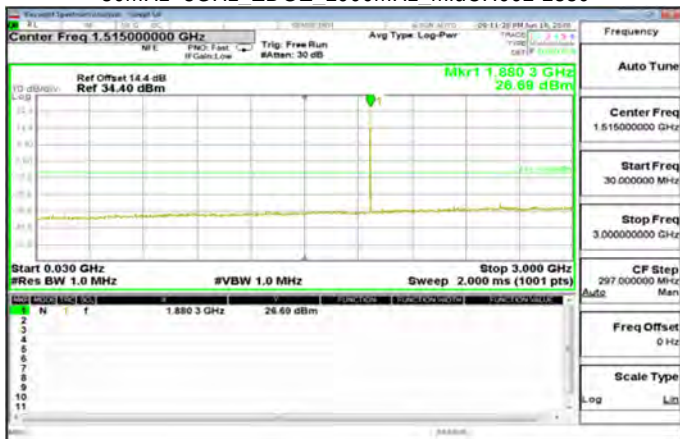
30MHz-3GHz_EDGE_1900MHz_MidCH661-1880
