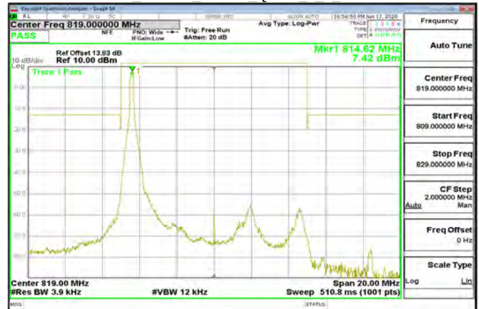
Band26_Part90s_10MHz_QPSK_1_0_CH26740
