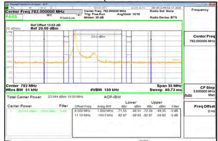
Band13 5MHz QPSK 1 24 CH23255
