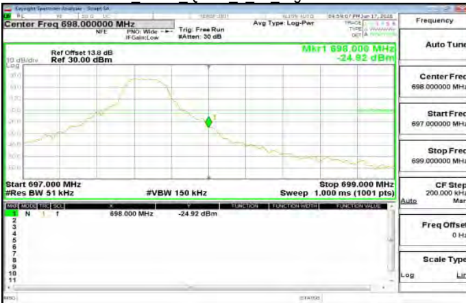
LTE\Band71 5MHz QPSK 1 24_HighCH133447-695.5
