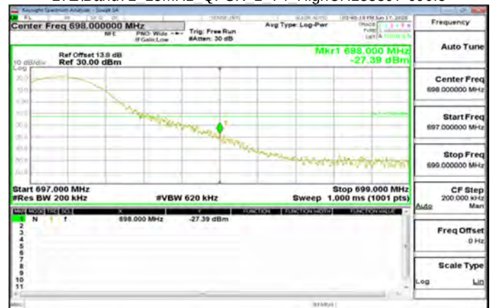
LTE\Band71_15MHz_QPSK_1_74_HighCH133397-690.5
