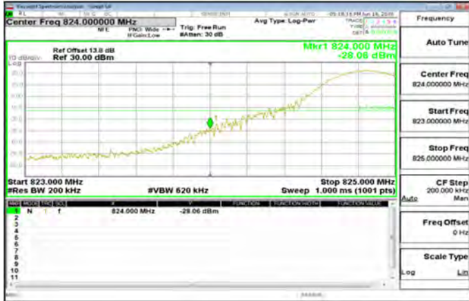
LTE\Band26_15MHz_QPSK_1_0_LowCH26865-831.5
