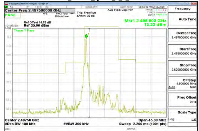
Band41 10MHz_QPSK 1 0 CH39700
