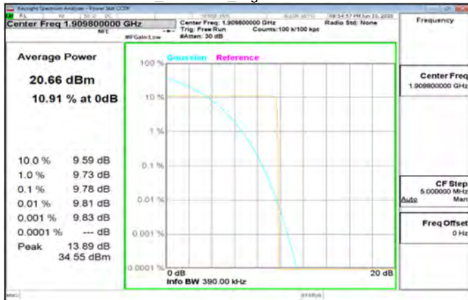
GPRS_1900MHz_HighCH810-1909.8
