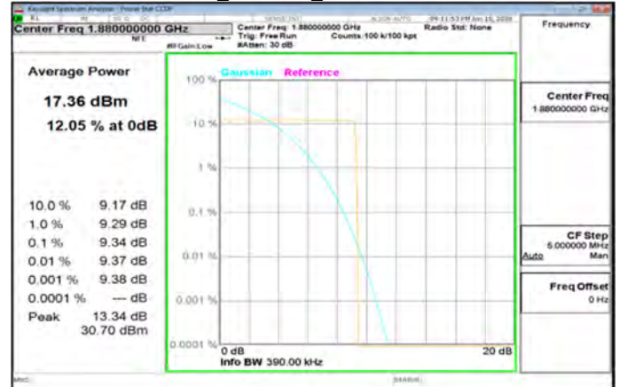
EDGE_1900MHz_MidCH661-1880
