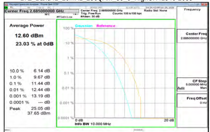
LTE_Band41_10MHz_256QAM_50_0_HighCH41540-2685
