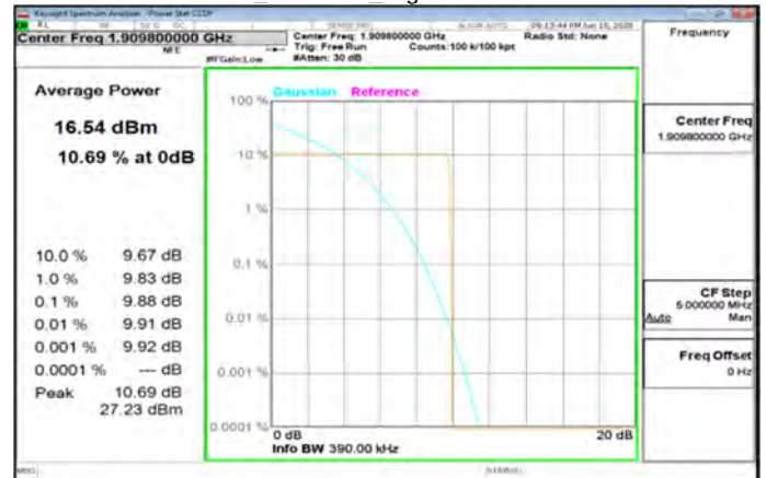
EDGE_1900MHz_HighCH810-1909.8
