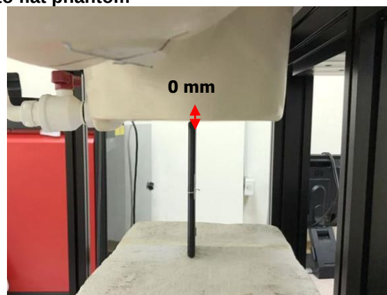
Fig.23 EUT Bottom side to flat phantom
