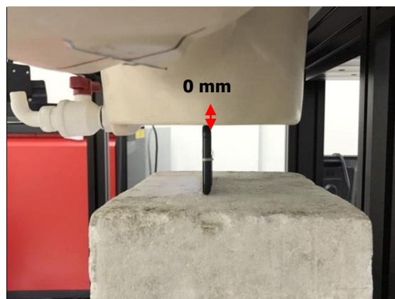
Fig.22 EUT Left side to flat phantom
