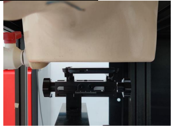
Fig.11 EUT Front side to flat phantom
