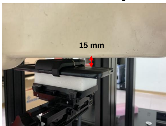
Fig.10 EUT Back side to flat phantom (with fan)
