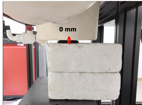
Fig.19 EUT Back side to flat phantom
