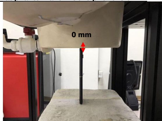
Fig.21 EUT Top side to flat phantom
