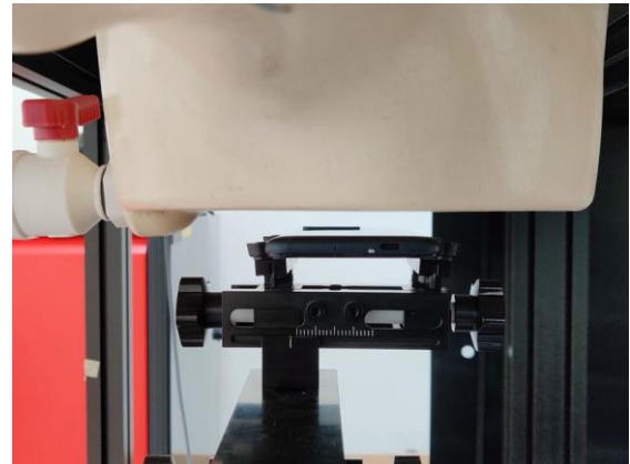
Fig.12 EUT Back side to flat phantom
