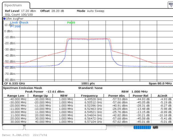
Plot on Channel 6535MHz
