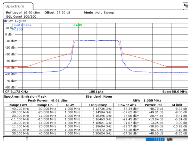
Plot on Channel 6175MHz
