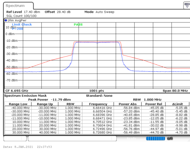
Plot on Channel 6695MHz
