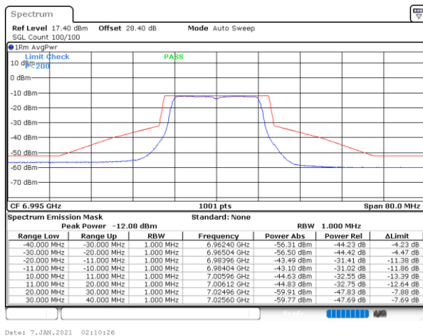
Plot on Channel 6995MHz
