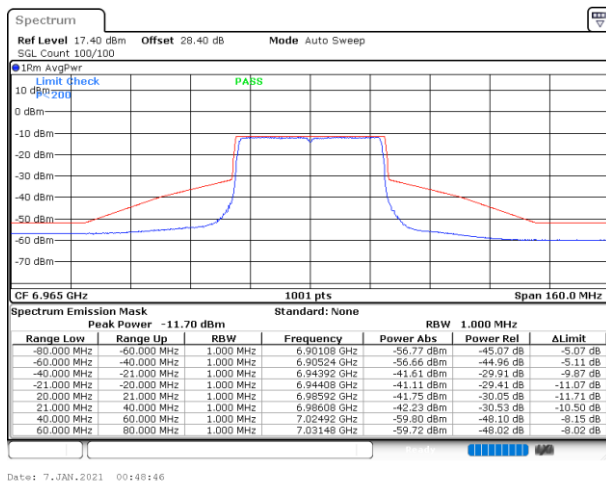
Plot on Channel 6965MHz
