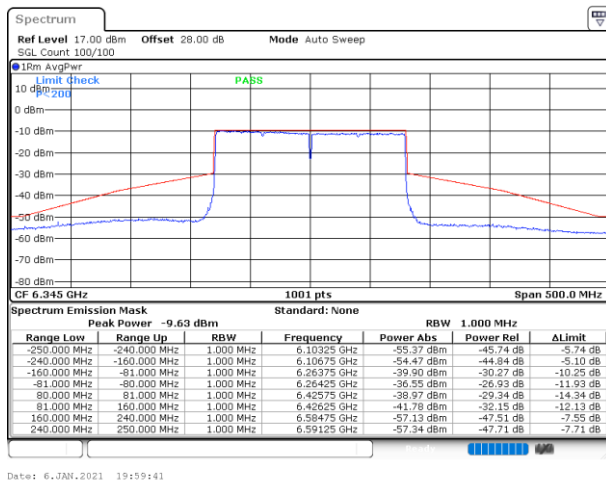
Plot on Channel 6345MHz
