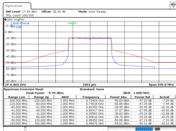
Plot on Channel 6865MHz
