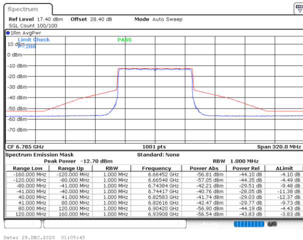
Plot on Channel 6785MHz
