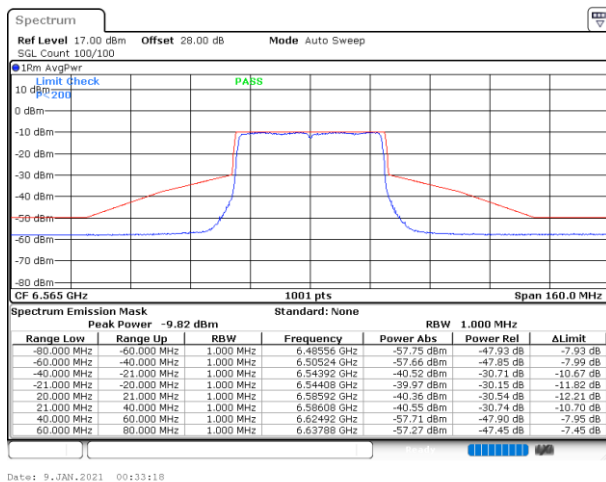
Plot on Channel 6565MHz
