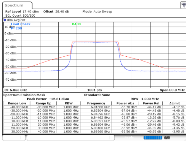
Plot on Channel 6855MHz
