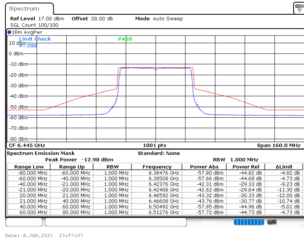
Plot on Channel 6445MHz
