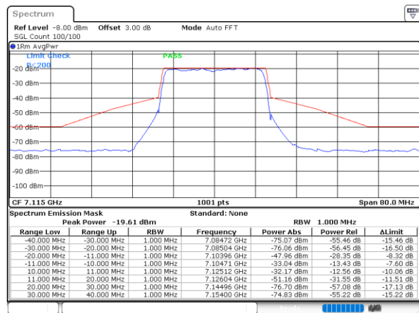
Plot on Channel 7115MHz
