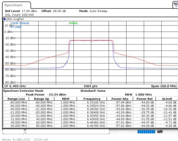
Plot on Channel 6405MHz
