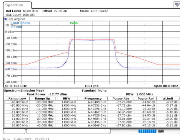
Plot on Channel 6435MHz
