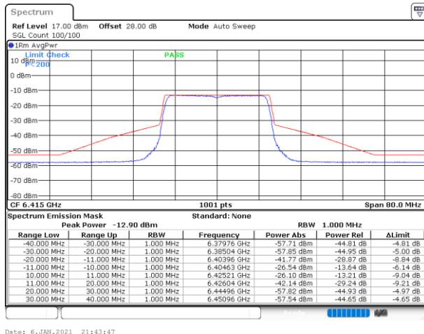
Plot on Channel 6415MHz
