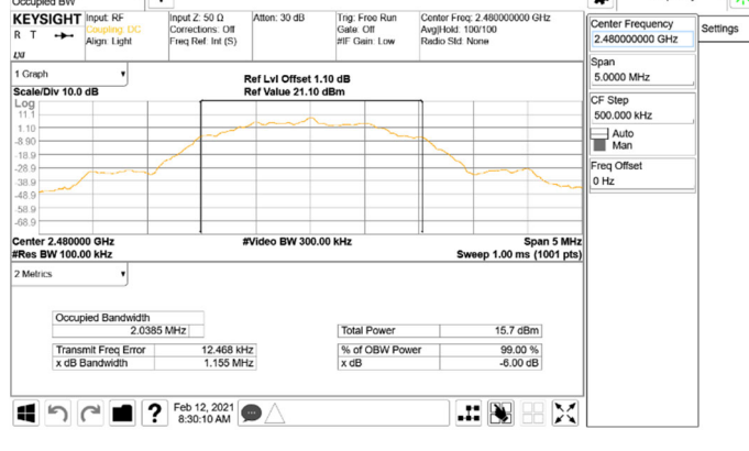
OBW 6dB_BLE_2M_HighCH39-2480
