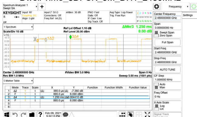
Dwell Time_8DPSK_3M_DH1_2480MHz
