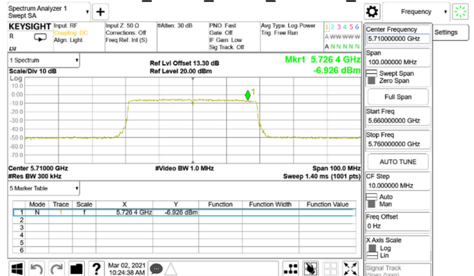
802.11ax_40MHz_Chain1_5710MHz_UNII 3
