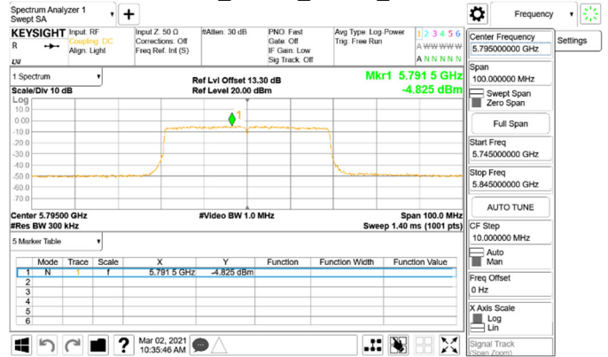
802.11ax_40MHz_Chain0_5795MHz_RU242_62
