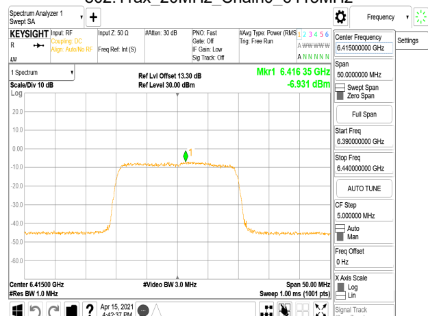
802.11ax_20MHz_Chain0_6415MHz
