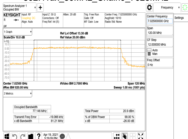
802.11ax_80MHz_Chain0_7025MHz
