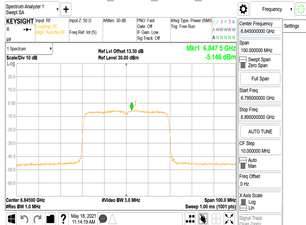
802.11ax_40MHz_Chain0_6845MHz_RU242_62
