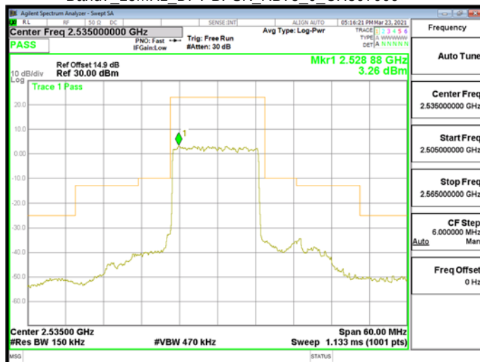
Band7_15MHz_DFT-BPSK_RB75_0_CH507000
