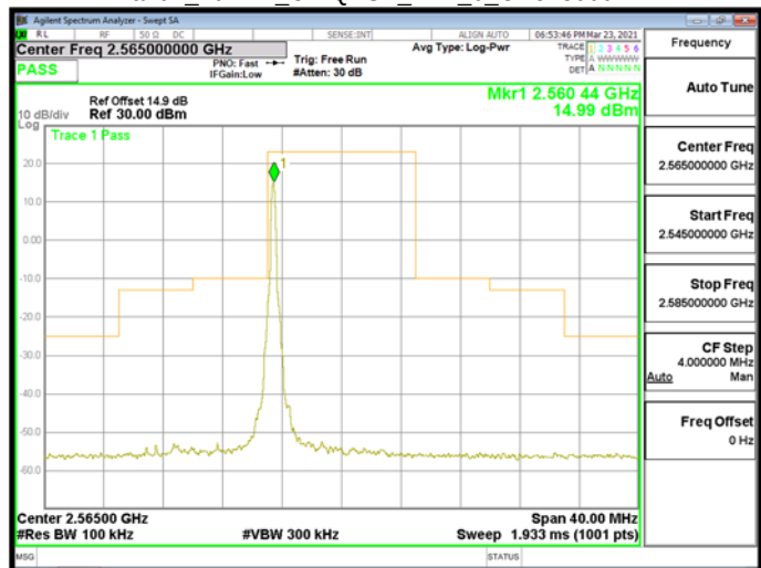
Band7 10MHz CP-QPSK RB1_0 CH513000
