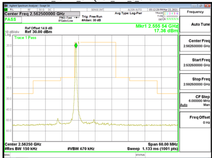
Band7_15MHz_CP-QPSK_RB1_0_CH512500
