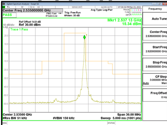
Band7 5MHz DFT BPSK RB1 24 CH507000
