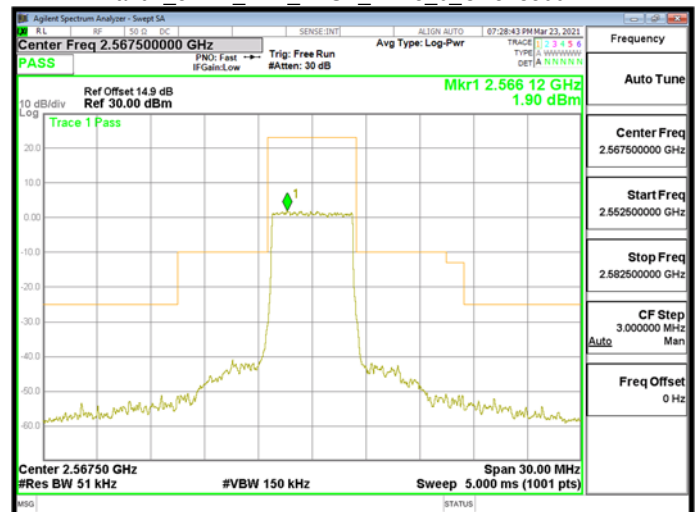
Band7 5MHz DFT BPSK RB25 0 CH513500
