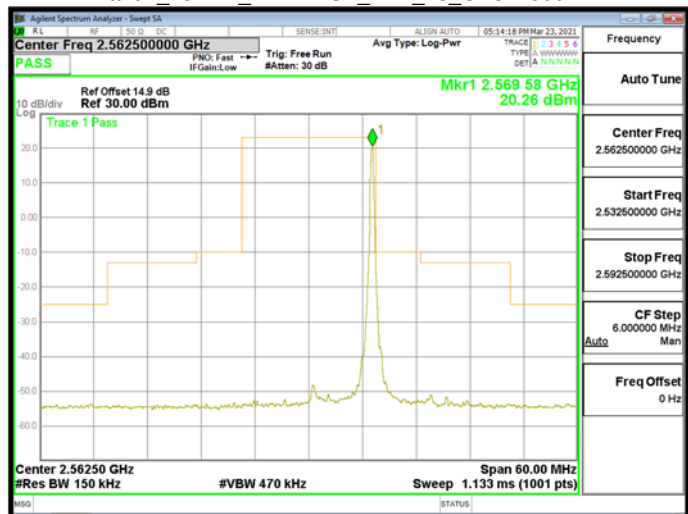
Band7_15MHz_DFT-BPSK_RB1_78_CH512500
