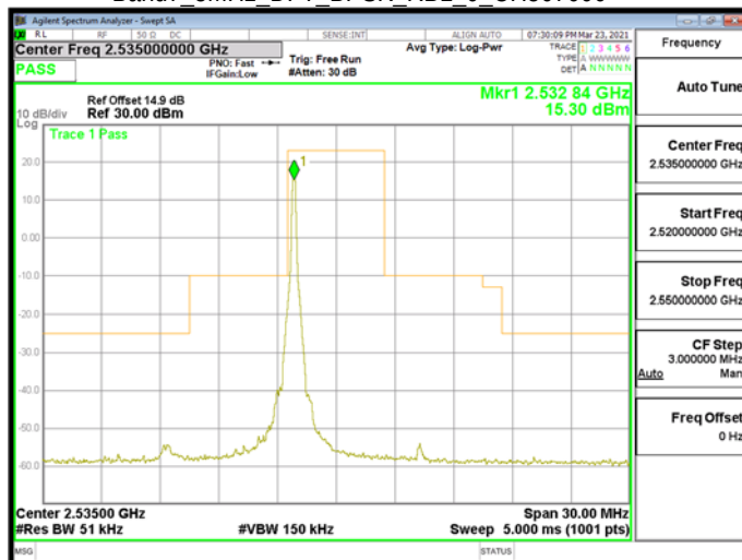
Band7_5MHz_DFT_BPSK_RB1_0_CH507000
