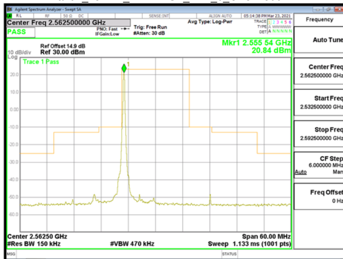
Band7_15MHz_DFT-BPSK_RB1_0_CH512500
