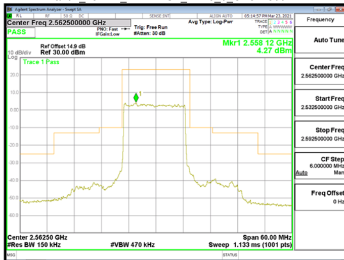
Band7_15MHz_DFT-BPSK_RB75_0_CH512500
