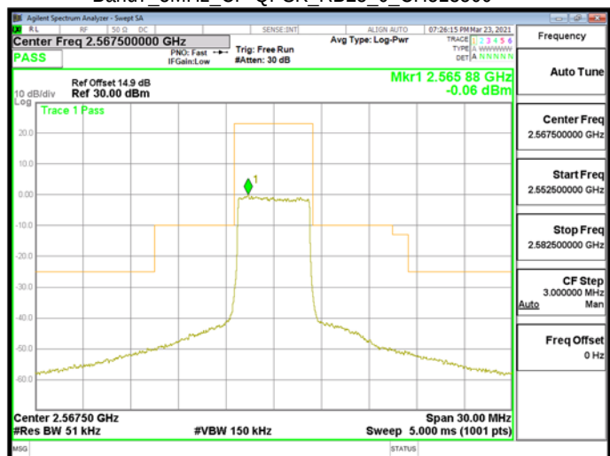
Band7_5MHz_CP-QPSK_RB25_0_CH513500
