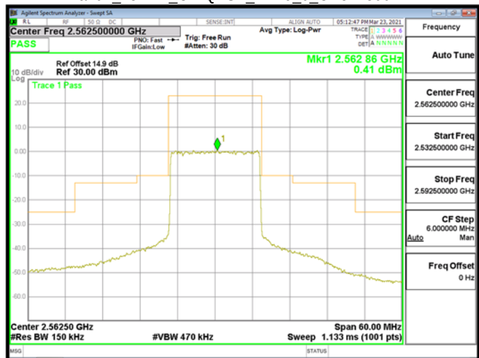
Band7_15MHz_CP-QPSK_RB79_0_CH512500
