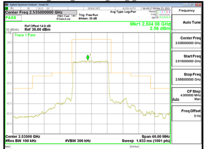
Band7_10MHz_DFT-BPSK_RB50_0_CH507000
