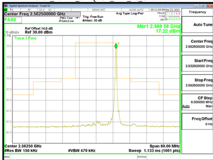
Band7_15MHz_CP-QPSK_RB1_78_CH512500
