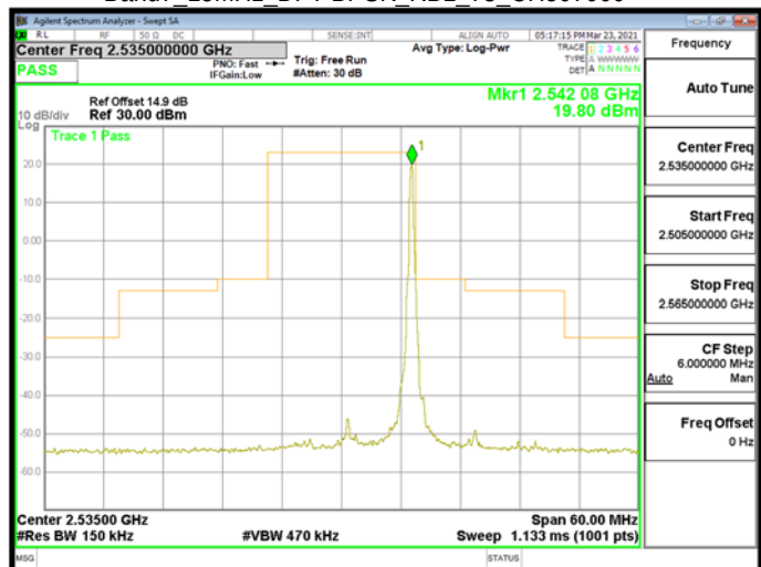
Band7_15MHz_DFT-BPSK_RB1_78_CH507000
