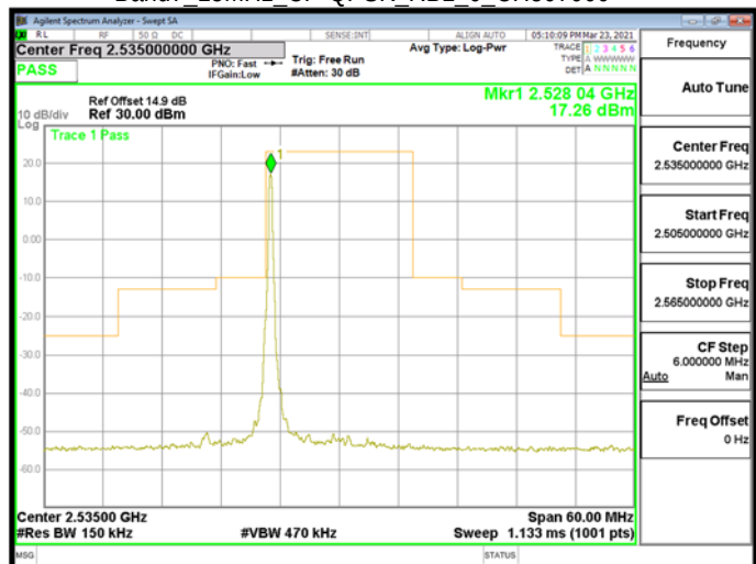
Band7_15MHz_CP-QPSK_RB1_0_CH507000
