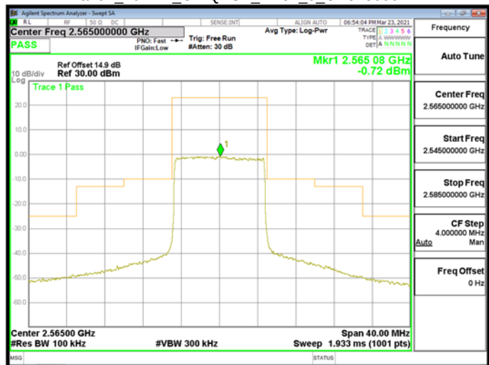
Band7_10MHz_CP-QPSK_RB52_0_CH513000
