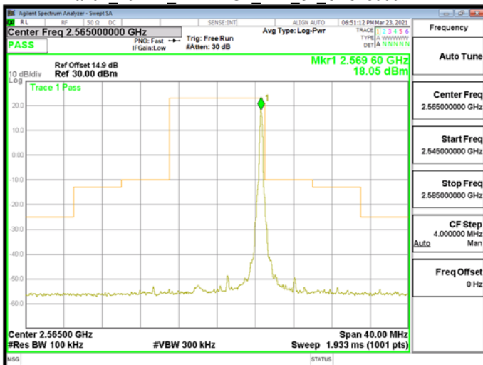
Band7_10MHz_DFT-BPSK_RB1_51_CH513000
