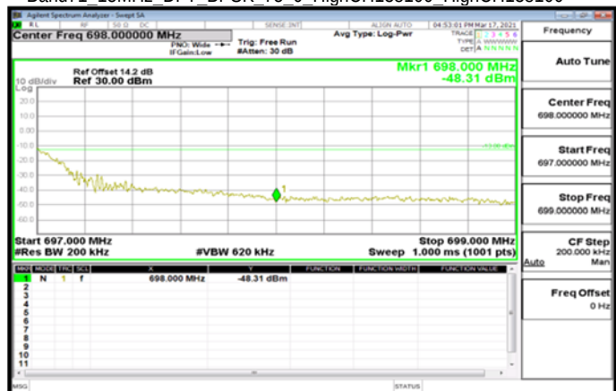
Band71_15MHz_DFT_BPSK_75_0_HighCH138100_HighCH138100
