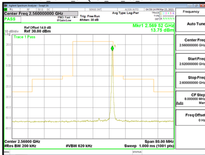
Band7 20MHz CP-QPSK RB1_105 CH512000
