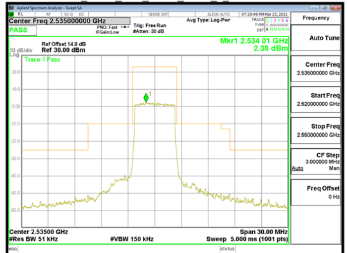
Band7 5MHz DFT BPSK RB25 0 CH507000
