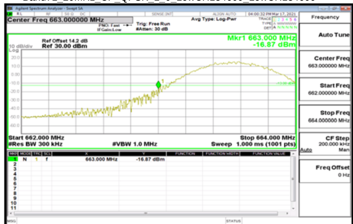
Band71_20MHz_CP_QPSK_1_0_LowCH134600_LowCH134600
