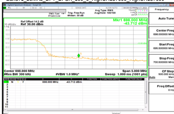
Band71_20MHz_DFT_BPSK_100_0_HighCH137600_HighCH137600
