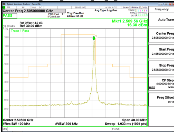
Band7_10MHz_DFT-BPSK_RB1_51_CH501000
