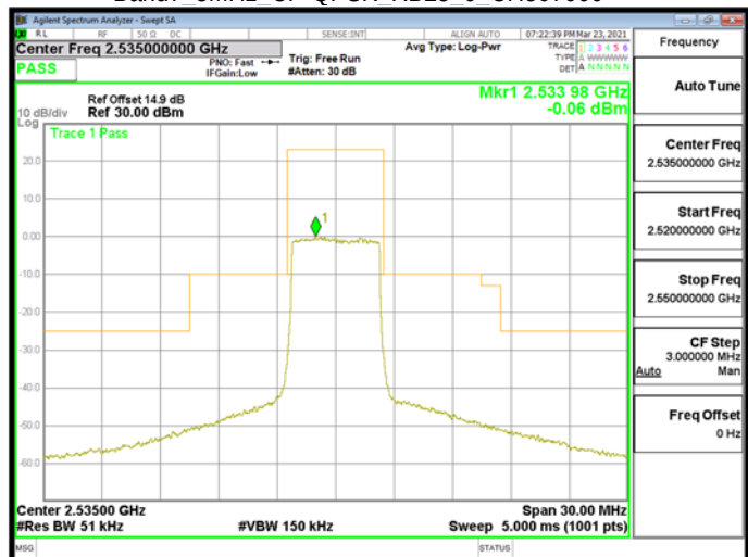
Band7_5MHz_CP-QPSK_RB25_0_CH507000
