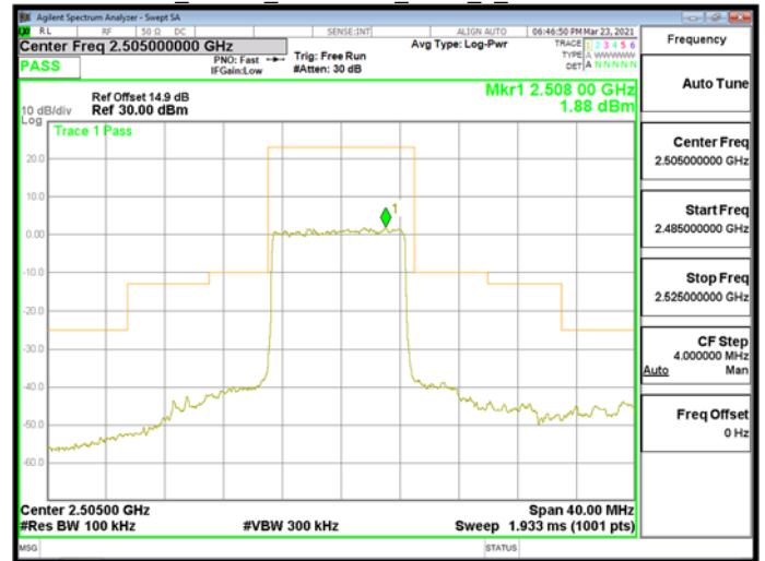
Band7_10MHz_DFT-BPSK_RB50_0_CH501000
