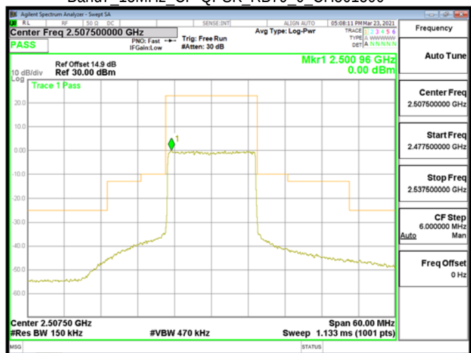
Band7_15MHz_CP-QPSK_RB79_0_CH507000
