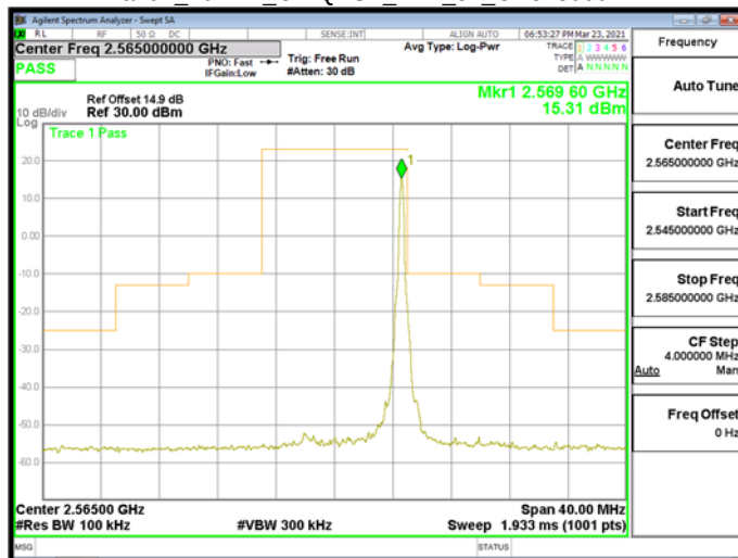
Band7 10MHz CP-QPSK RB1_51 CH513000
