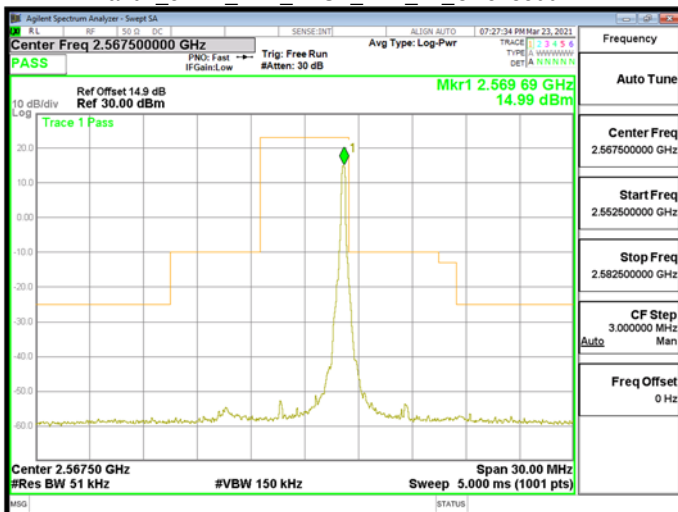
Band7 5MHz DFT BPSK RB1 24 CH513500
