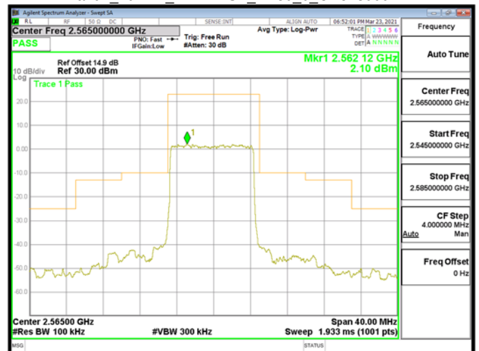
Band7_10MHz_DFT-BPSK_RB50_0_CH513000
