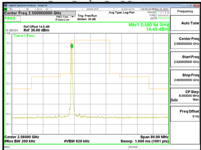
Band7 20MHz CP-QPSK RB1_0 CH512000
