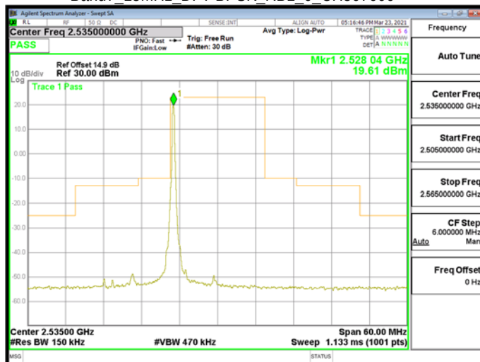
Band7_15MHz_DFT-BPSK_RB1_0_CH512500
