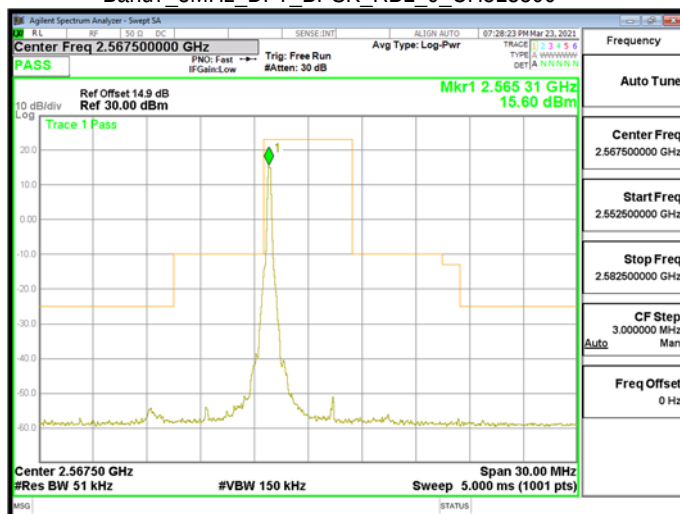
Band7_5MHz_DFT_BPSK_RB1_0_CH513500
