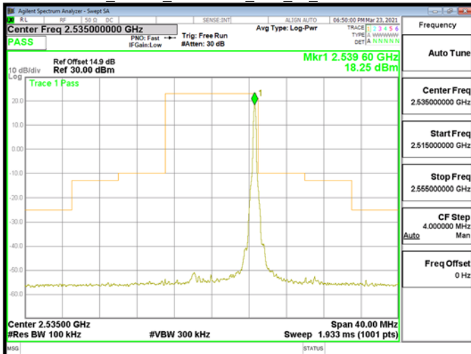
Band7_10MHz_DFT-BPSK_RB1_51_CH507000
