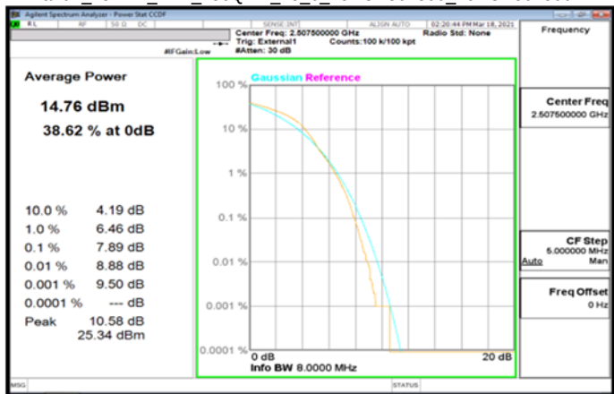
Band7_15MHz_DFT_256QAM_75_0_LowCH501500_LowCH501500
