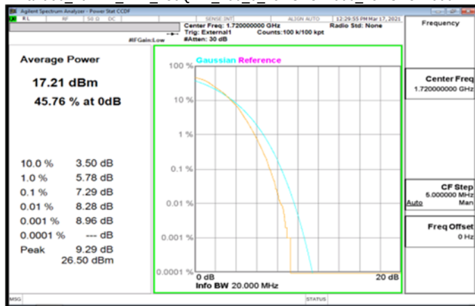
Band66_20MHz_DFT_256QAM_100_0_LowCH344000_LowCH344000
