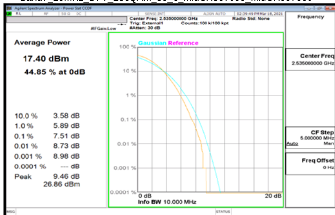
Band7_10MHz_DFT_256QAM_50_0_MidCH507000_MidCH507000
