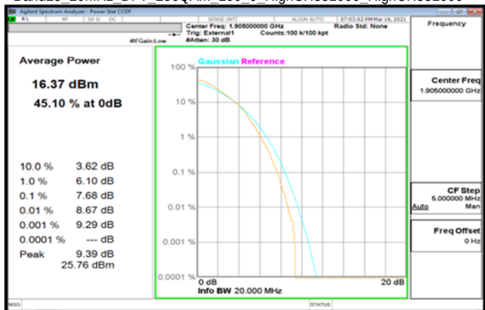
Band25_20MHz_DFT_256QAM_100_0_HighCH381000_HighCH381000
