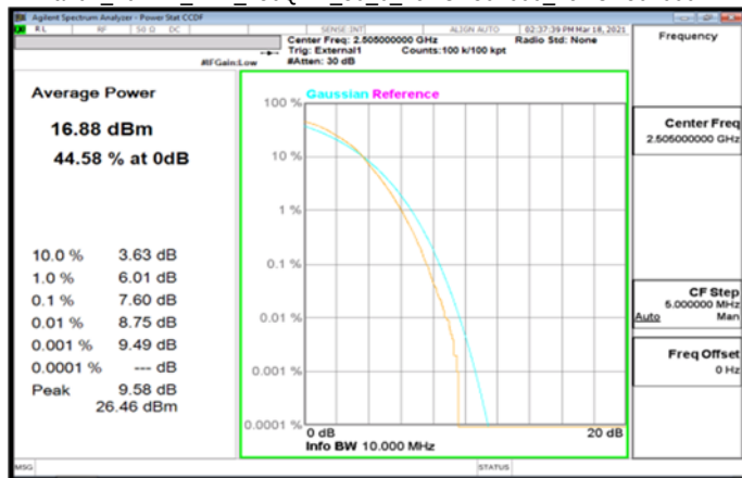
Band7_10MHz_DFT_256QAM_50_0_LowCH501000_LowCH501000
