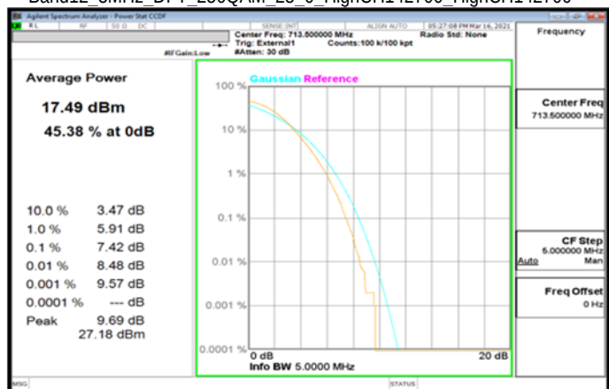
Band12_5MHz_DFT_256QAM_25_0_HighCH142700_HighCH142700
