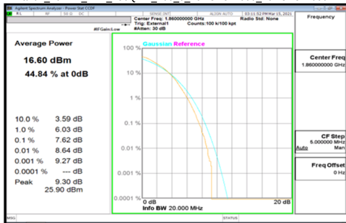
Band2_20MHz_DFT_256QAM_100_0_MidCH376000_MidCH376000
