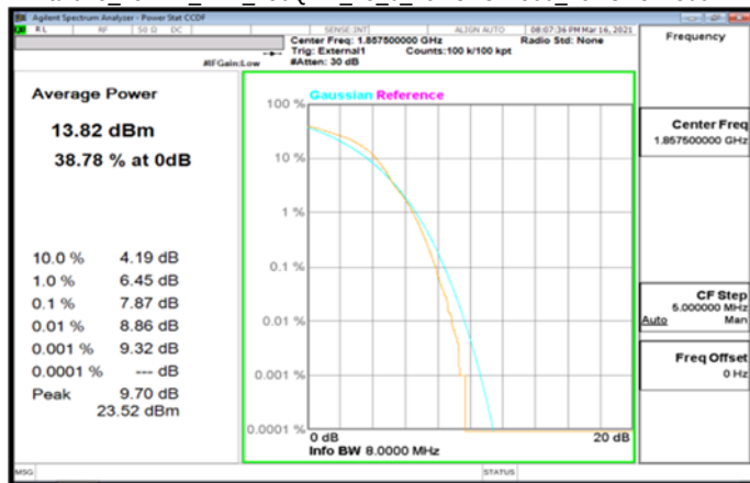
Band25_15MHz_DFT_256QAM_75_0_LowCH371500_LowCH371500
