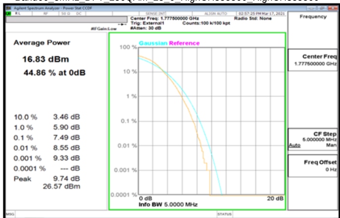
Band66_5MHz_DFT_256QAM_25_0_HighCH355500_HighCH355500
