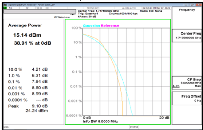
Band66_15MHz_DFT_256QAM_75_0_LowCH343500_LowCH343500
