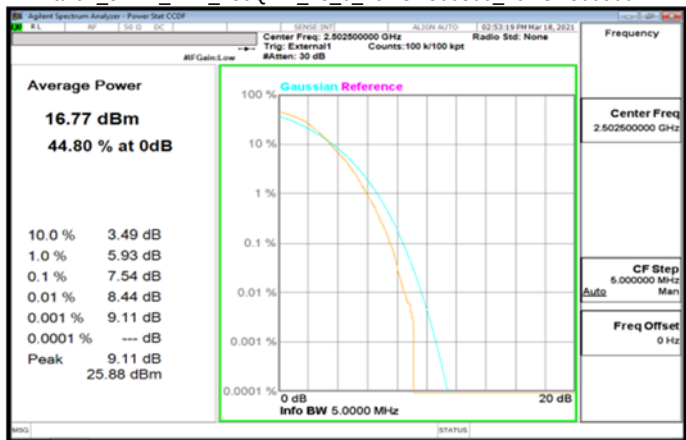
Band7_5MHz_DFT_256QAM_25_0_LowCH500500_LowCH500500
