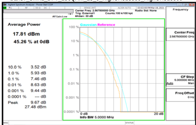
Band7_5MHz_DFT_256QAM_25_0_HighCH513500_HighCH513500
