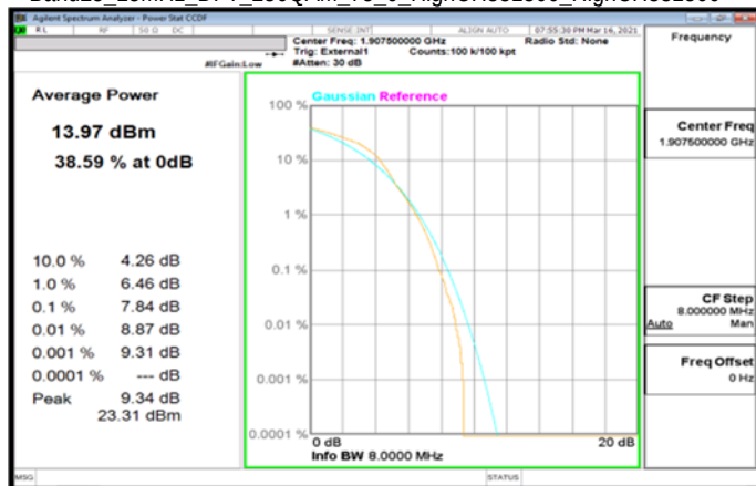
Band25_15MHz_DFT_256QAM_75_0_HighCH381500_HighCH381500
