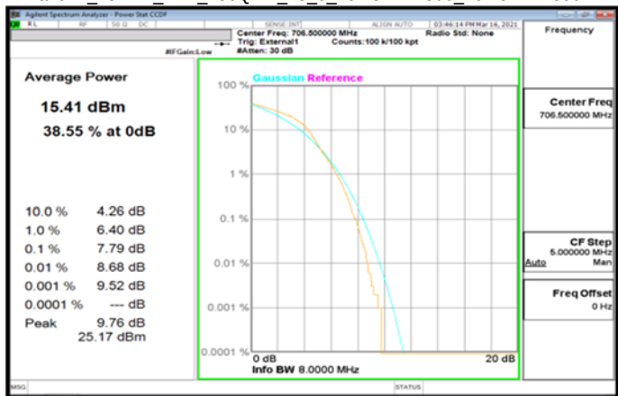
Band12_15MHz_DFT_256QAM_75_0_LowCH141300_LowCH141300
