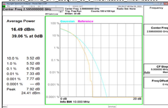
Band38_20MHz_DFT_256QAM_50_0_MidCH519000_MidCH519000
