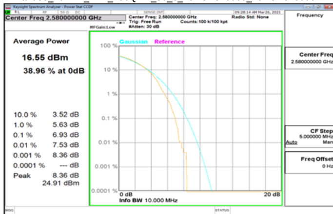
Band38_20MHz_DFT_256QAM_50_0_LowCH516000_LowCH516000
