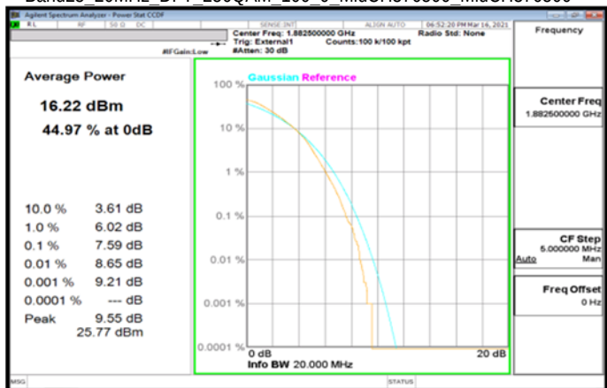
Band25_20MHz_DFT_256QAM_100_0_MidCH376500_MidCH376500
