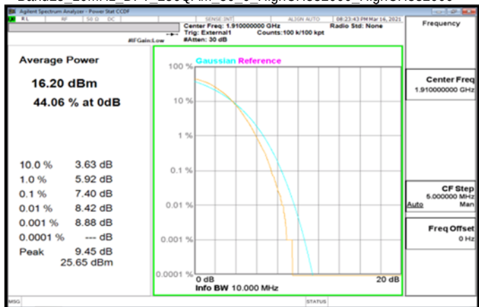
Band25_10MHz_DFT_256QAM_50_0_HighCH382000_HighCH382000
