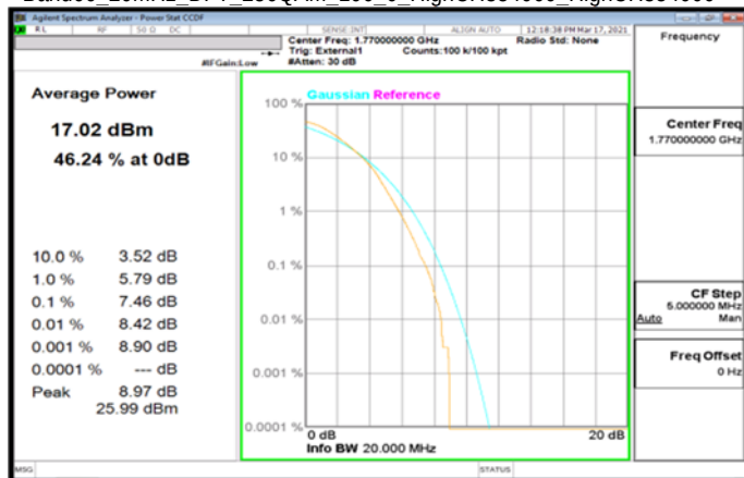
Band66_20MHz_DFT_256QAM_100_0_HighCH354000_HighCH354000
