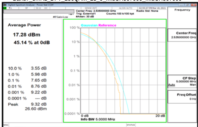
Band7_5MHz_DFT_256QAM_25_0_MidCH507000_MidCH507000
