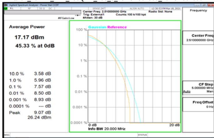
Band7_20MHz_DFT_256QAM_100_0_LowCH502000_LowCH502000
