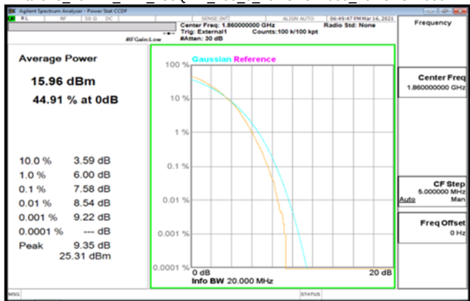
Band25_20MHz_DFT_256QAM_100_0_LowCH372000_LowCH372000
