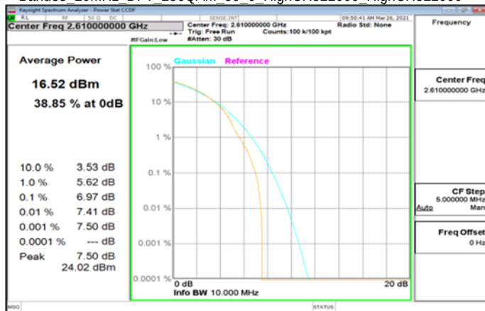
Band38_20MHz_DFT_256QAM_50_0_HighCH522000_HighCH522000
