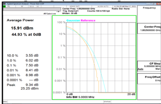
Band25_5MHz_DFT_256QAM_25_0_LowCH370500_LowCH370500
