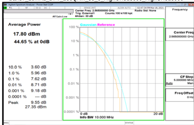
Band7_10MHz_DFT_256QAM_50_0_HighCH513000_HighCH513000
