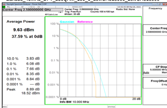
Band38_40MHz_DFT_256QAM_100_0_MidCH519000_MidCH519000
