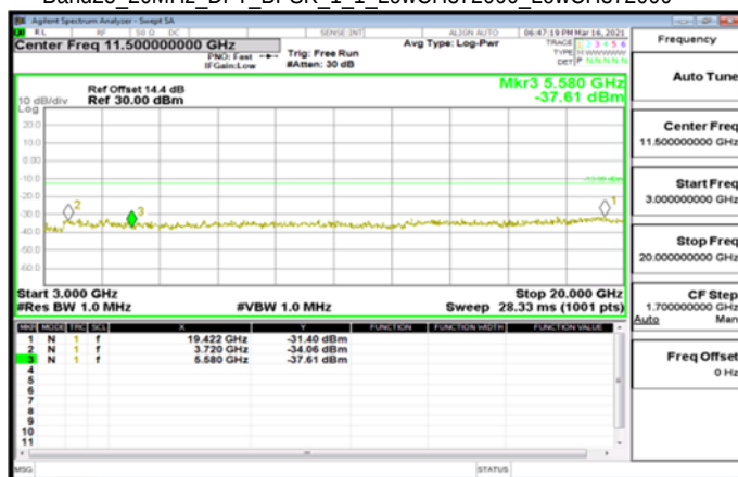
Band25_20MHz_DFT_BPSK_1_1_MidCH376500_MidCH376500
