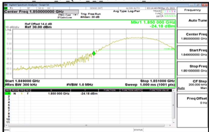
Band2_20MHz_CP_QPSK_1_0_LowCH372000_LowCH372000
