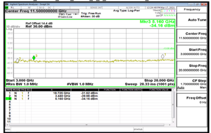
Band66_20MHz_DFT_BPSK_1_1_MidCH349000_MidCH349000
