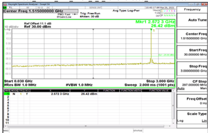
Band38_40MHz_DFT_BPSK_1_1_MidCH519000_MidCH519000
