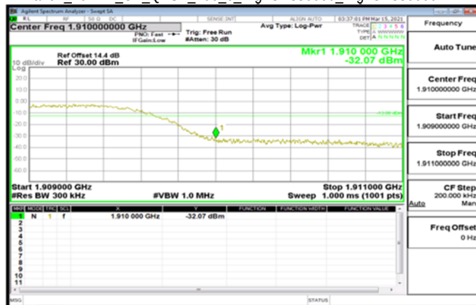
Band2_20MHz_CP_QPSK_106_0_HighCH380000_HighCH380000
