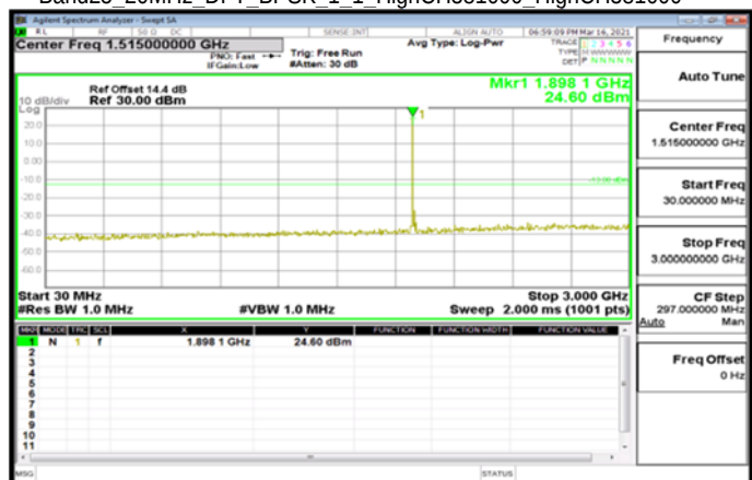
Band25_20MHz_DFT_BPSK_1_1_HighCH381000_HighCH381000
