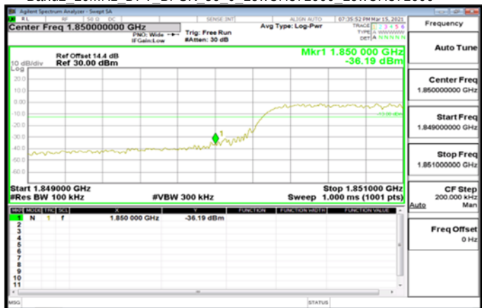
Band2_10MHz_DFT_BPSK_50_0_LowCH371000_LowCH371000
