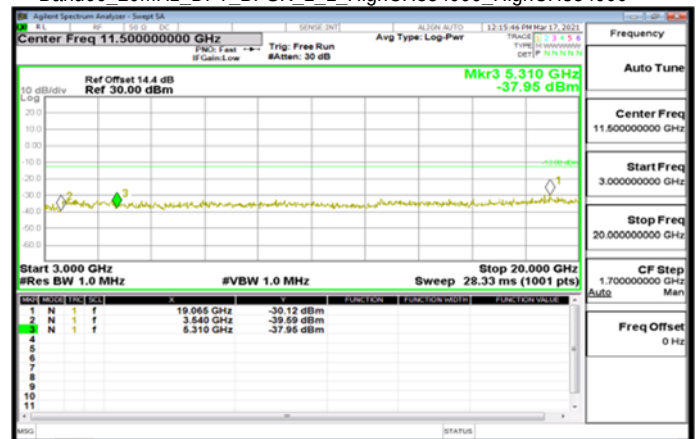
Band66_20MHz_DFT_BPSK_1_1_HighCH354000_HighCH354000
