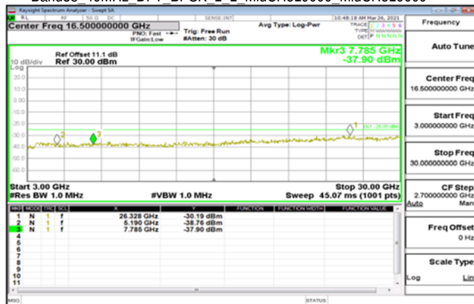
Band38_40MHz_DFT_BPSK_1_1_HighCH520000_HighCH520000
