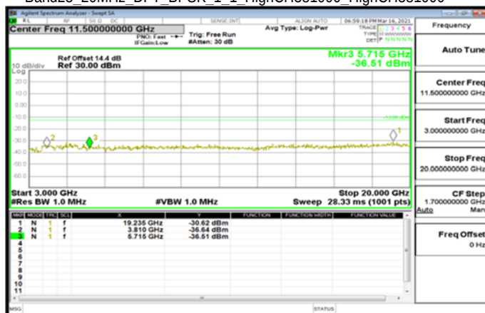
Band25_20MHz_DFT_BPSK_1_1_HighCH381000_HighCH381000
