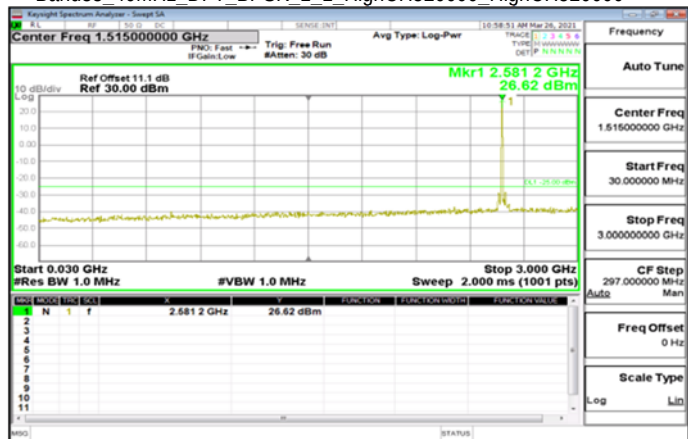
Band38_40MHz_DFT_BPSK_1_1_HighCH520000_HighCH520000
