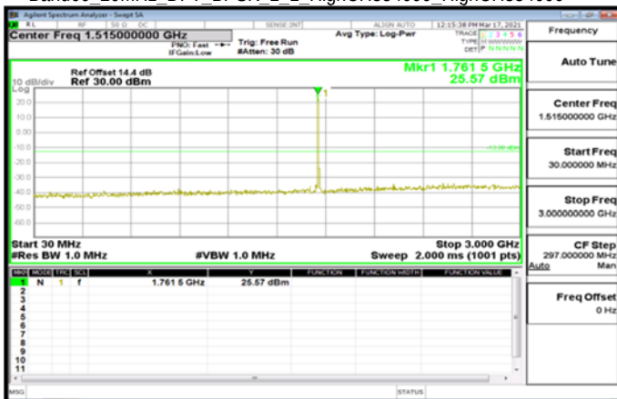
Band66_20MHz_DFT_BPSK_1_1_HighCH354000_HighCH354000
