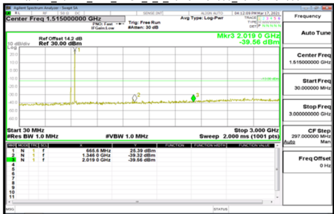
Band71_20MHz_DFT_BPSK_1_1_MidCH136100_MidCH136100
