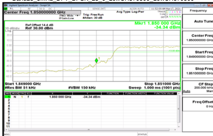
Band25_5MHz_DFT_BPSK_25_0_LowCH370500_LowCH370500
