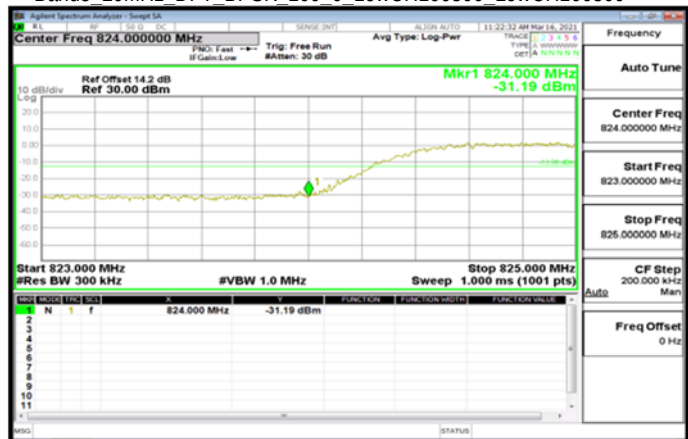
Band5 20MHz_DFT_BPSK_100_0_LowCH166800_LowCH166800
