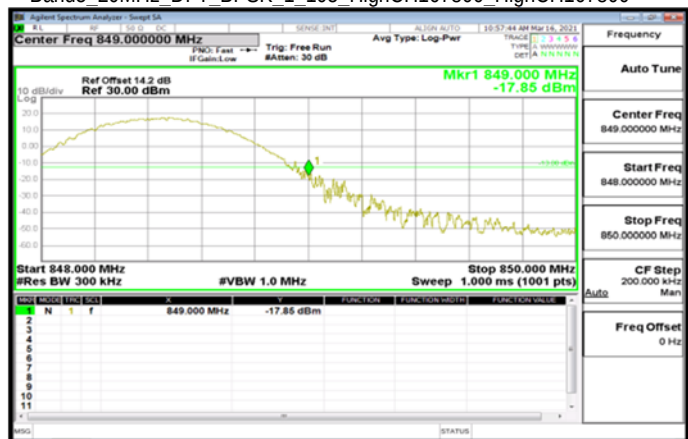
Band5 20MHz_DFT_BPSK_1_105_HighCH167800_HighCH167800
