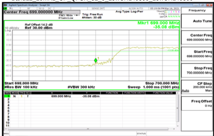
Band12_10MHz_CP_QPSK_52_0_LowCH140800_LowCH140800
