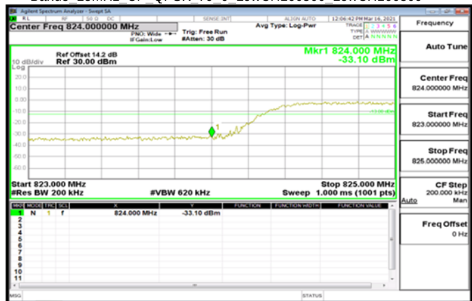
Band5_15MHz_CP_QPSK_79_0_LowCH166300_LowCH166300
