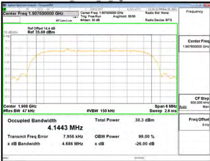
OBW 99%_HSUPA_B2_HighCH9538-1907.6
