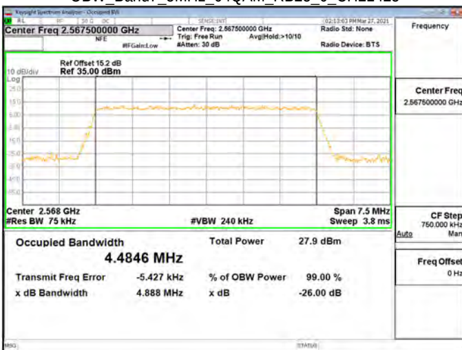
OBW Band7 5MHz 64QAM_RB25_0_CH21425
