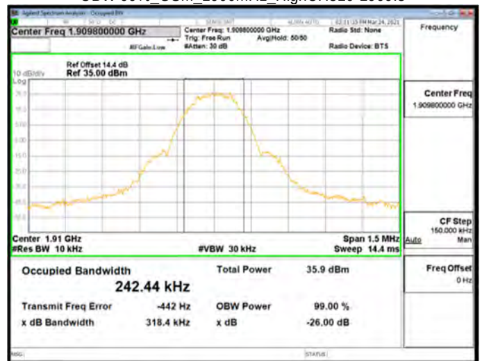
OBW 99%_GSM_1900MHz_HighCH810-1909.8
