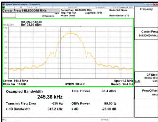
OBW 99%_EDGE_850MHz_HighCH251-848.8
