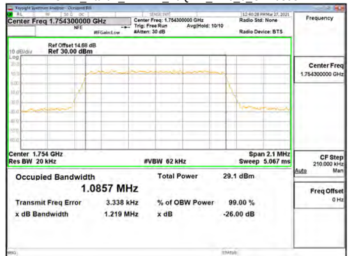
OBW_Band4_1.4MHz_16QAM_RB6_0_CH20393
