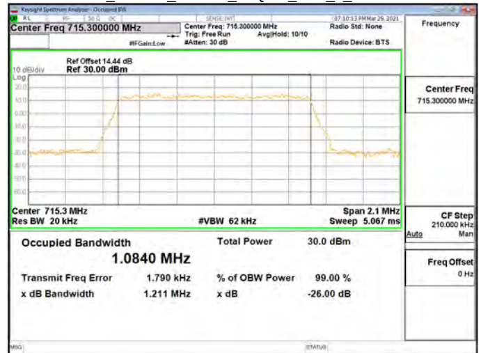
OBW_Band12_1.4MHz_16QAM_RB6_0_CH23173
