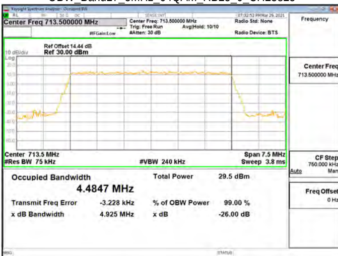
OBW_Band17_5MHz_64QAM_RB25_0_CH23825
