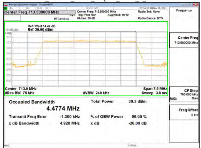
OBW_Band17_5MHz_16QAM_RB25_0_CH23825
