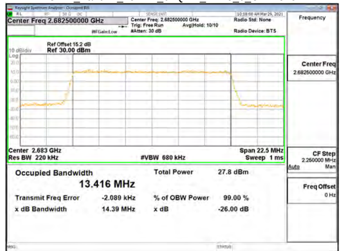
OBW_Band41_15MHz_64QAM_RB75_0_CH41515
