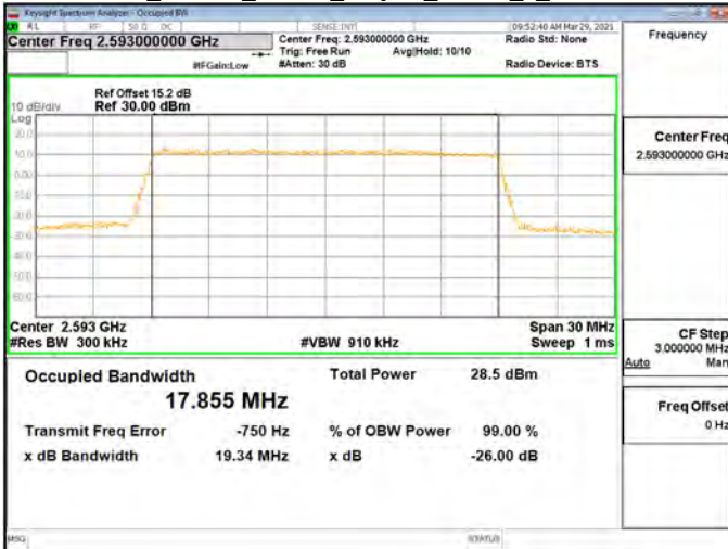
OBW_Band41_20MHz_64QAM_RB100_0_CH41490
