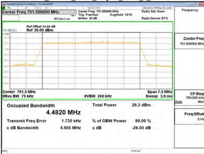
OBW_Band12_5MHz_64QAM_RB25_0_CH23095
