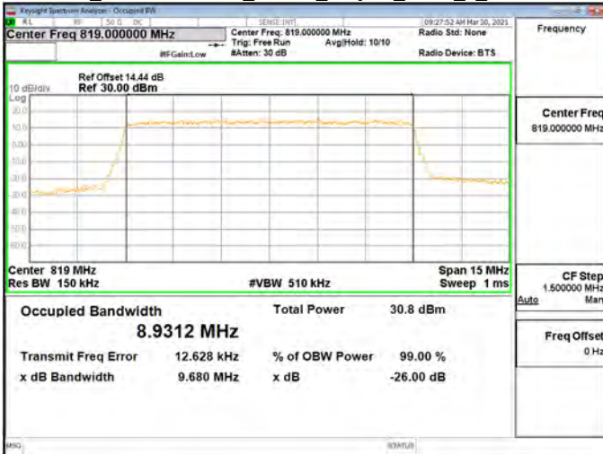
OBW_Band26-Part90s_10MHz_64QAM_RB50_0_CH26740
