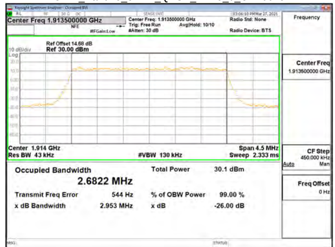
OBW_Band25_3MHz_QPSK_RB15_0_CH26675
