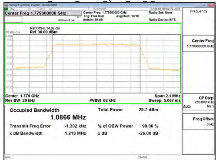
OBW_Band66_1.4MHz_QPSK_RB6_0_CH132665
