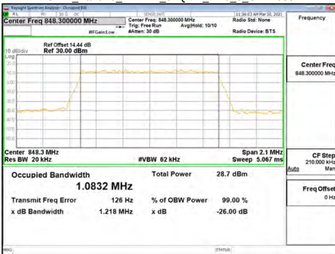
OBW_Band26_1.4MHz_64QAM_RB6_0_CH27033
