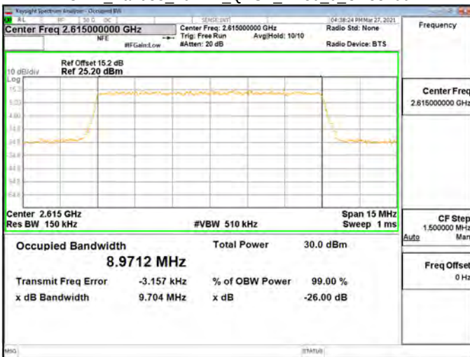
OBW_Band38_10MHz_QPSK_RB50_0_CH38200
