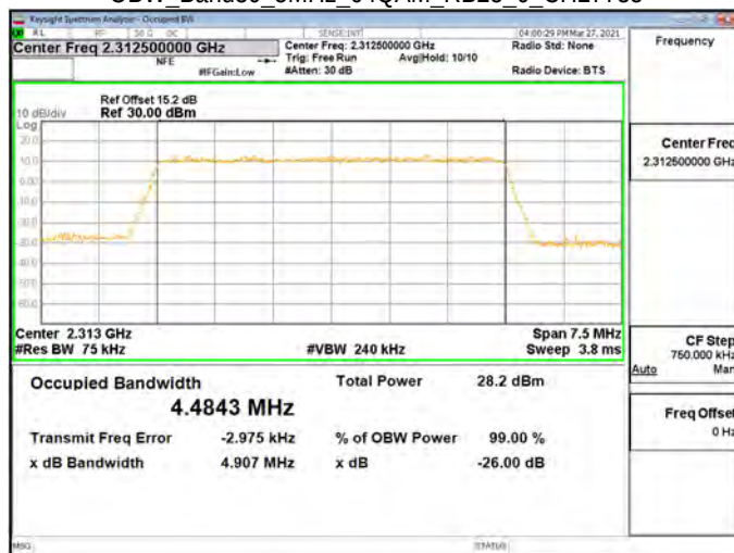
OBW Band30 5MHz 64OAM RB25 0 CH27735
