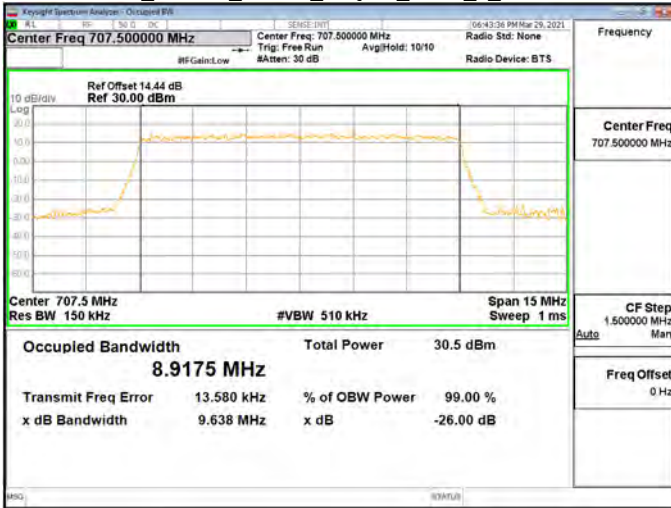
OBW_Band12_10MHz_16QAM_RB50_0_CH23130
