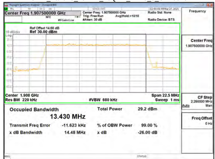
OBW_Band25_15MHz_16QAM_RB75_0_CH26615
