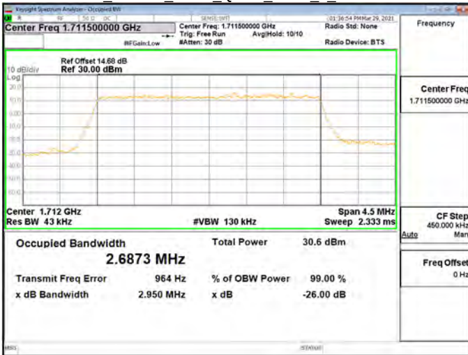
OBW_Band66_3MHz_QPSK_RB15_0_CH132322
