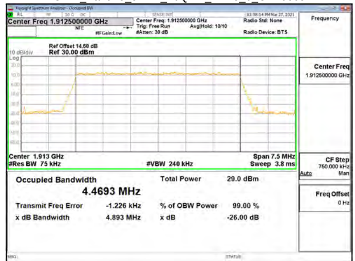
OBW_Band25_5MHz_16QAM_RB25_0_CH26665
