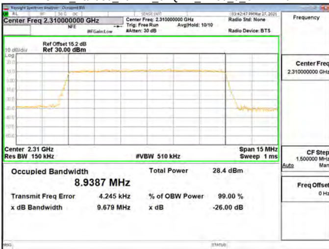
OBW_Band30_10MHz_64QAM_RB50_0_CH27710
