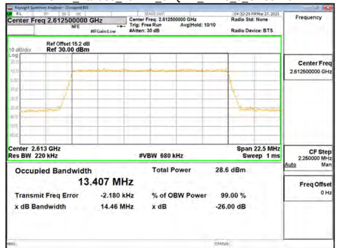
OBW_Band38_15MHz_64QAM_RB75_0_CH38175
