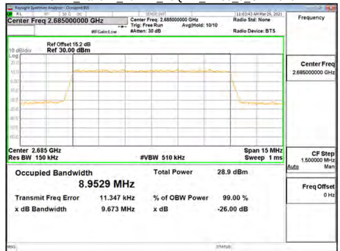
OBW_Band41_10MHz_16QAM_RB50_0_CH41540
