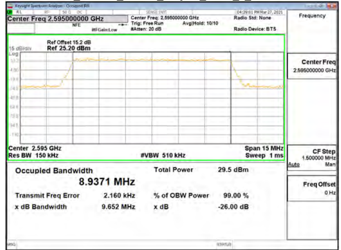
OBW_Band38_10MHz_16QAM_RB50_0_CH38200
