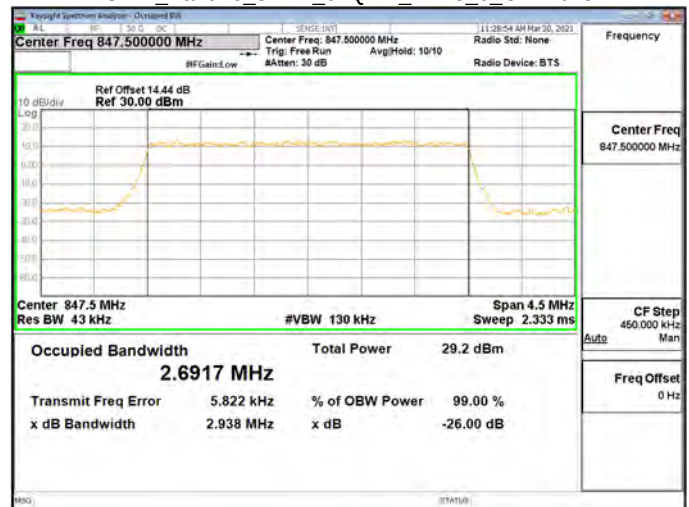
OBW_Band26_3MHz_64QAM_RB15_0_CH27025
