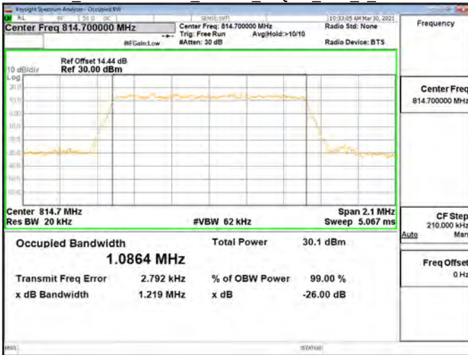
OBW Band26-Part90s_1.4MHz_16QAM_RB6_0_CH26740
