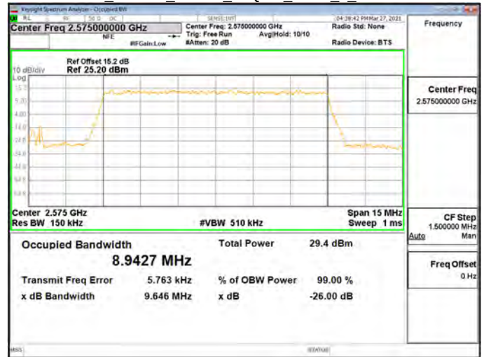
OBW_Band38_10MHz_16QAM_RB50_0_CH38000
