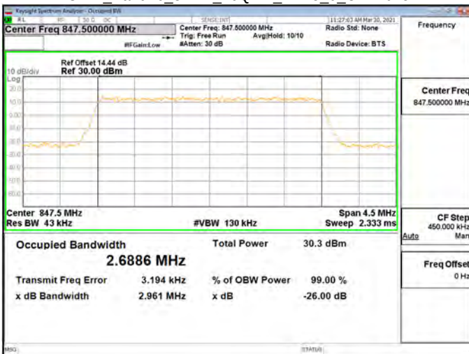
OBW_Band26_3MHz_16QAM_RB15_0_CH27025
