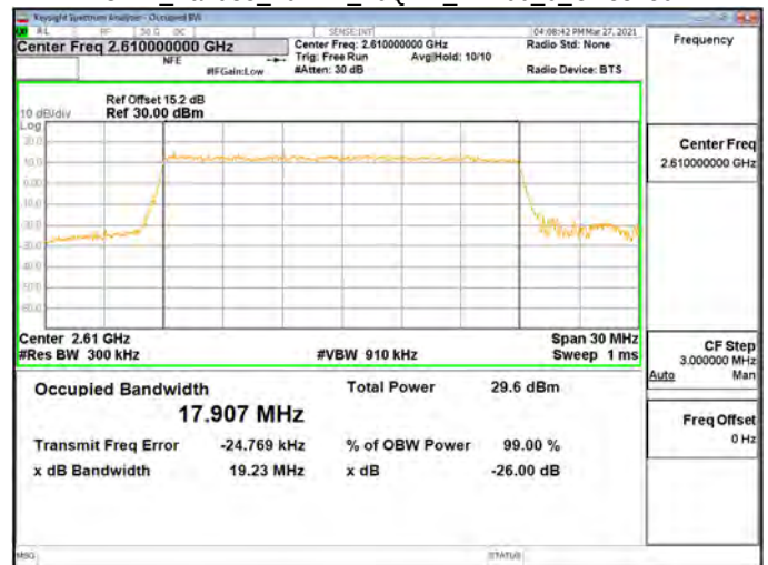
OBW_Band38_20MHz_16QAM_RB100_0_CH38150
