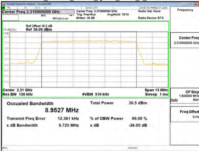
OBW_Band30_10MHz_16QAM_RB50_0_CH27710
