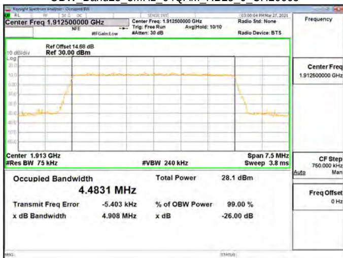
OBW Band25 5MHz 64OAM RB25 0 CH26665
