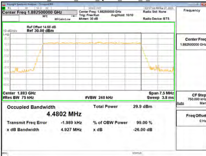
OBW_Band25_5MHz_QPSK_RB25_0_CH26665
