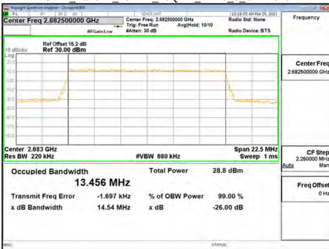
OBW_Band41_15MHz_16QAM_RB75_0_CH41515
