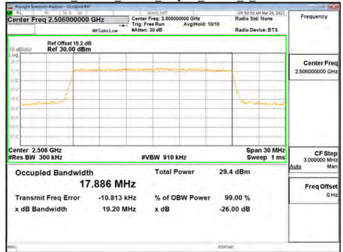
OBW_Band41_20MHz_16QAM_RB100_0_CH40620
