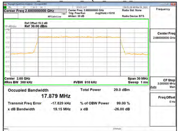
OBW_Band41_20MHz_16QAM_RB100_0_CH41490
