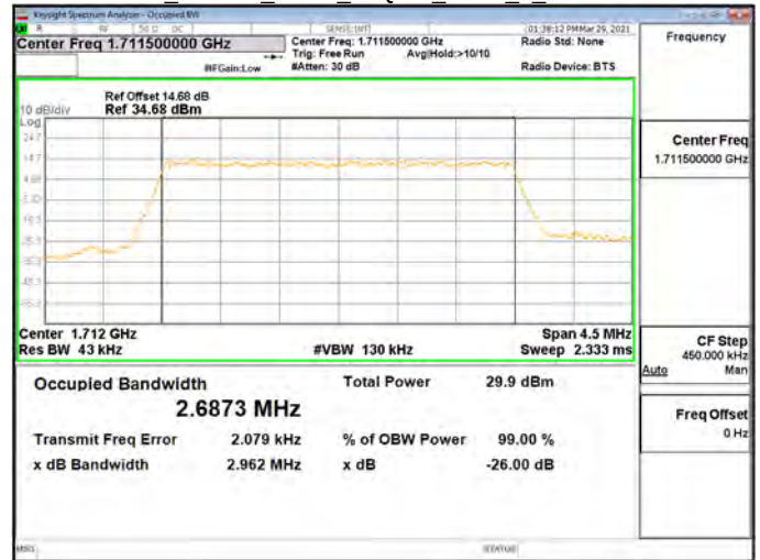
OBW_Band66_3MHz_16QAM_RB15_0_CH132322
