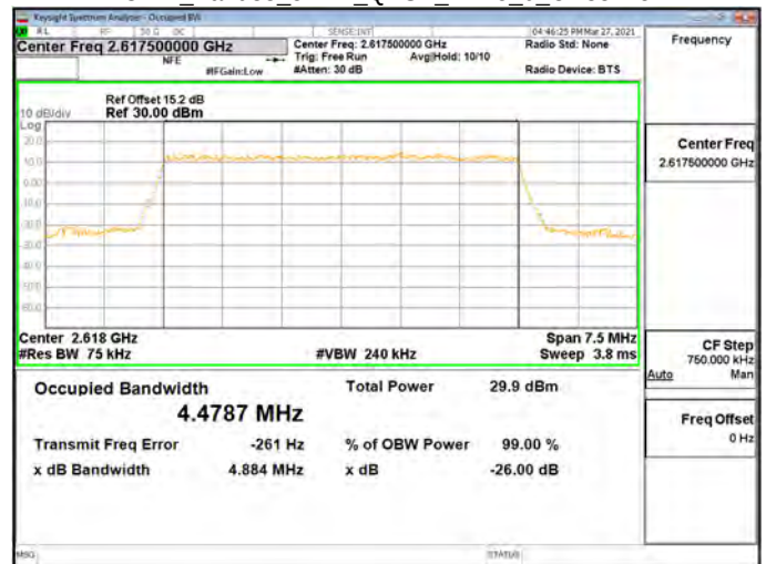
OBW_Band38_5MHz_QPSK_RB25_0_CH38225
