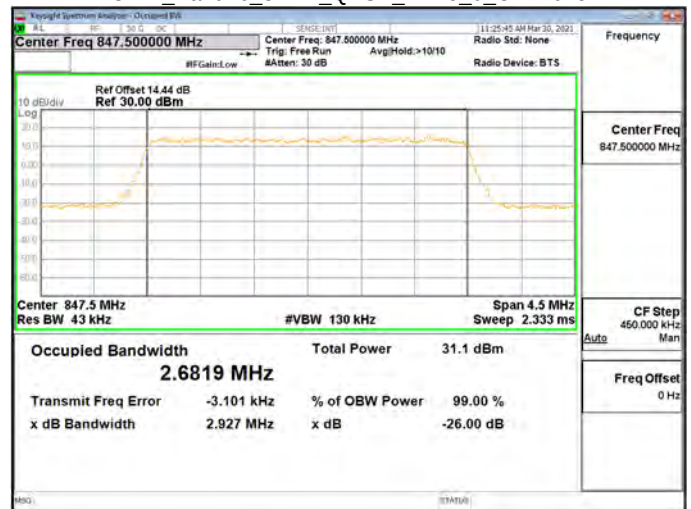
OBW_Band26_3MHz_QPSK_RB15_0_CH27025
