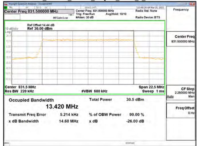
OBW_Band26_15MHz_16QAM_RB75_0_CH26915
