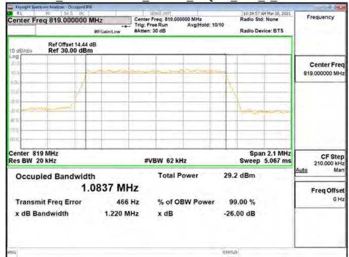
OBW Band26-Part90s_1.4MHz_64QAM_RB6_0_CH26783
