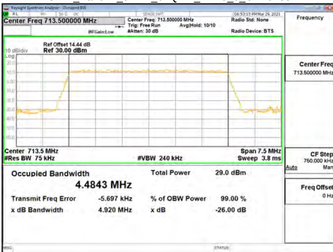
OBW_Band12_5MHz_64QAM_RB25_0_CH23155
