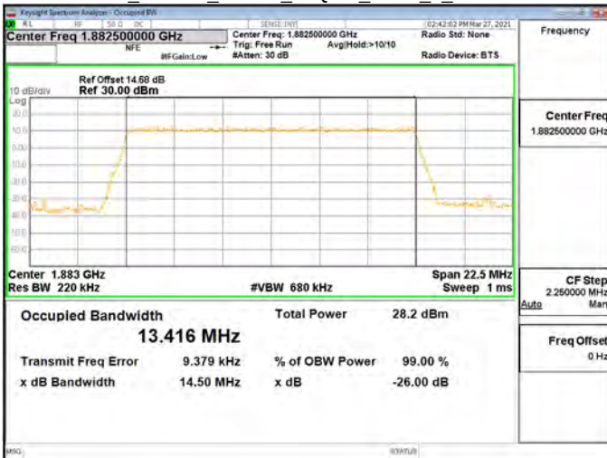
OBW_Band25_15MHz_64QAM_RB75_0_CH26615
