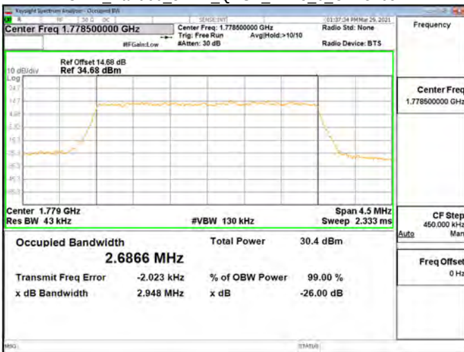
OBW_Band66_3MHz_QPSK_RB15_0_CH132657
