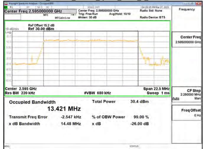
OBW_Band38_15MHz_QPSK_RB75_0_CH38175
