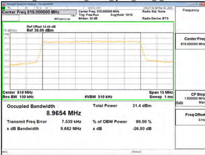
OBW_Band26-Part90s_10MHz_16QAM_RB50_0_CH26740
