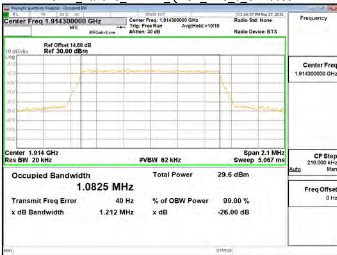
OBW_Band25_1.4MHz_QPSK_RB6_0_CH26683
