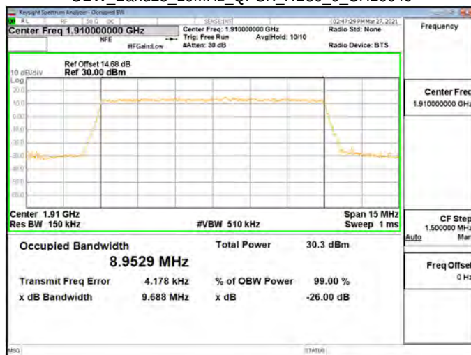
OBW Band25 10MHz QPSK RB50 0 CH26640
