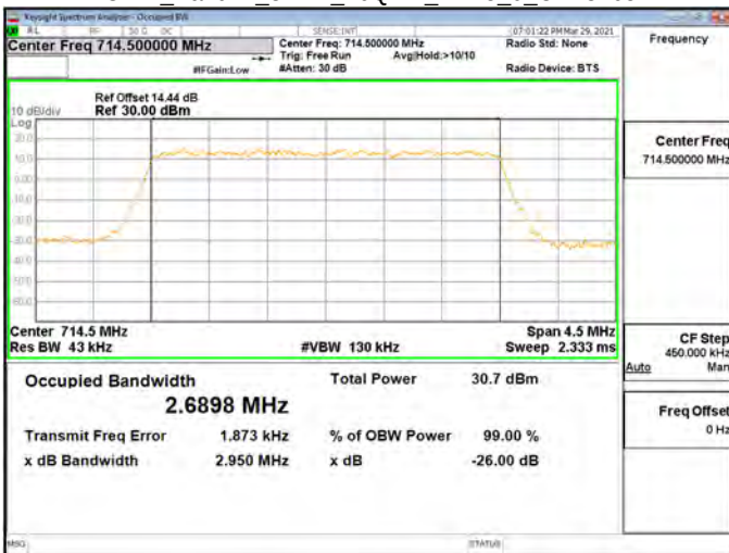
OBW_Band12_3MHz_16QAM_RB15_0_CH23165
