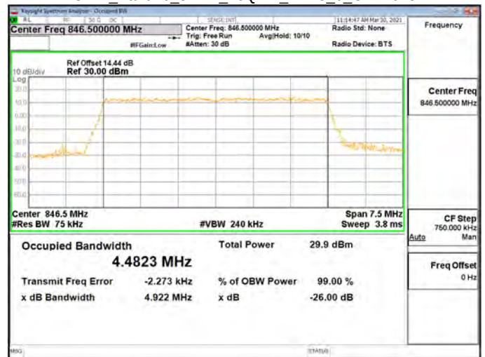
OBW_Band26_5MHz_16QAM_RB25_0_CH27015
