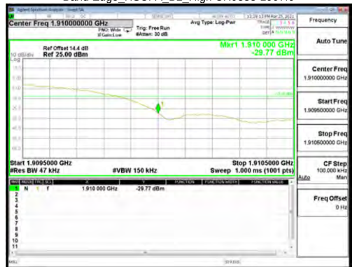
Band Edge_HSUPA_B2_High CH9538-1907.6
