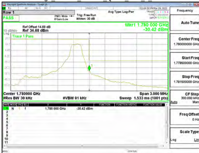
Band Edge_Band66_1.4MHz_QPSK_RB6_0_CH131979
