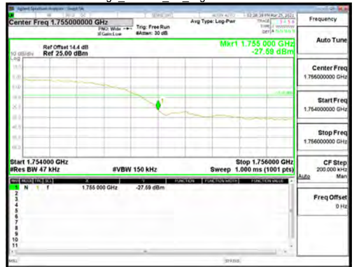
Band Edge_HSUPA_B4_High CH1513-1752.6
