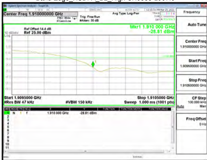
Band Edge_HSDPA_B2_High CH9538-1907.6
