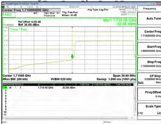
Band Edge_Band4_15MHz_QPSK_RB75_0_CH20325
