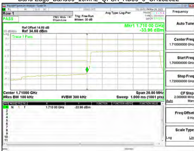
Band Edge_Band66_10MHz_QPSK_RB50_0_CH132022
