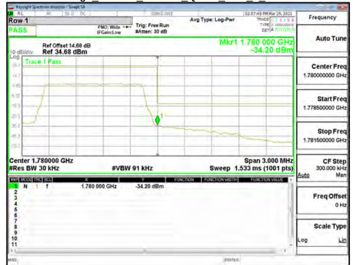
Band Edge_Band66_3MHz_QPSK_RB1_0_CH131987
