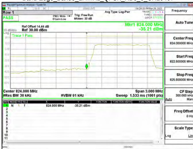
Band Edge_Band5_1.4MHz_QPSK_RB6_0_CH20407
