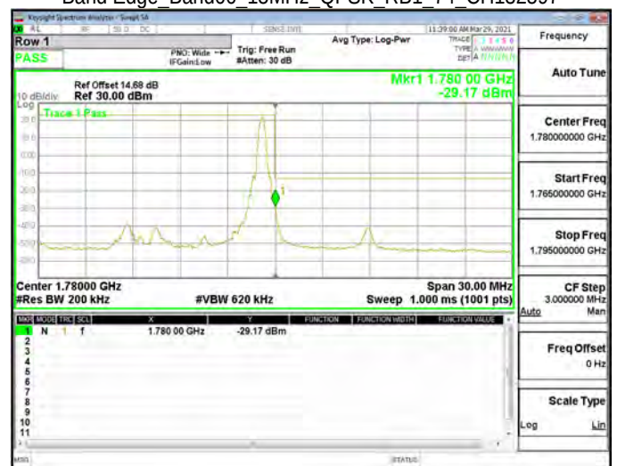
Band Edge_Band66_15MHz_QPSK_RB1_74_CH132597
