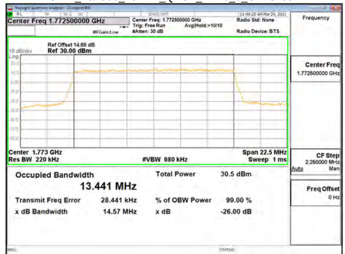
OBW Band66_15MHz_QPSK_RB75_0_CH132597
