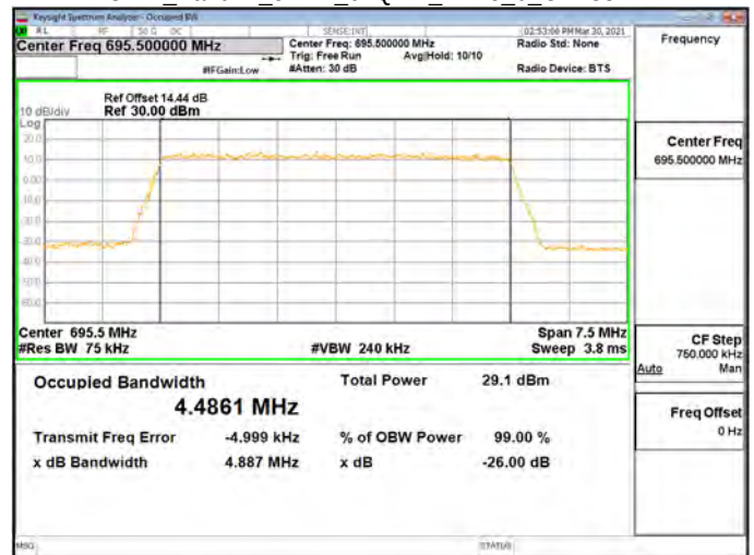
OBW_Band71_5MHz_64QAM_RB25_0_CH133447
