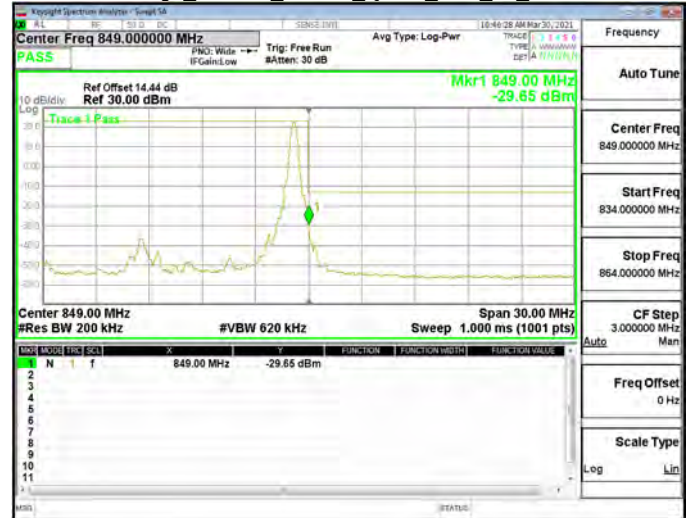
Band Edge Band26_15MHz_QPSK_RB75_0_CH26865
