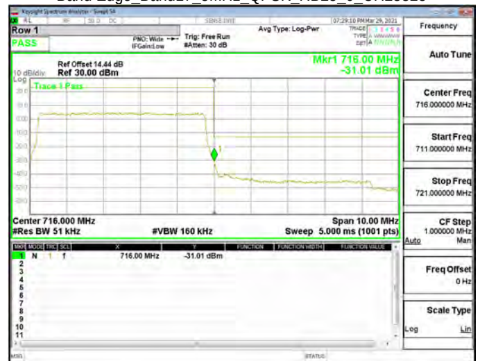
Band Edge_Band17_5MHz_QPSK_RB25_0_CH23825
