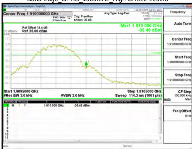
Band Edge_GPRS_1900MHz_High CH810-1909.8
