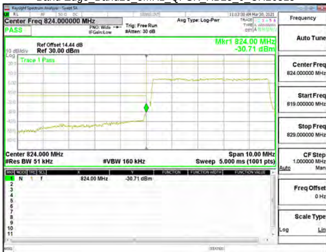
Band Edge_Band26_5MHz_QPSK_RB25_0_CH26815
