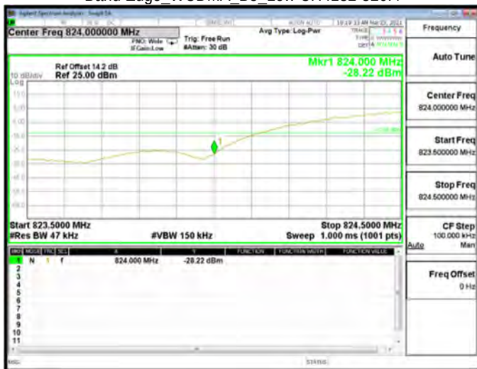
Band Edge_WCDMA_B5_Low CH4132-826.4
