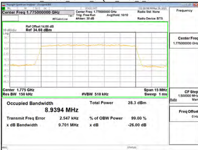
OBW Band66_10MHz_64QAM_RB50_0_CH132622
