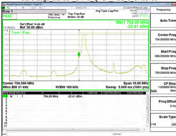
Band Edge_Band17_5MHz_QPSK_RB1_0_CH23755
