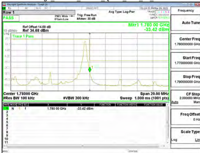
Band Edge_Band66_10MHz_QPSK_RB50_0_CH132022
