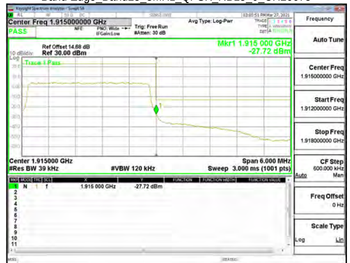
Band Edge_Band25_3MHz_QPSK_RB15_0_CH26675
