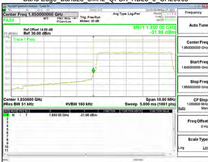
Band Edge_Band25_5MHz_QPSK_RB25_0_CH26065
