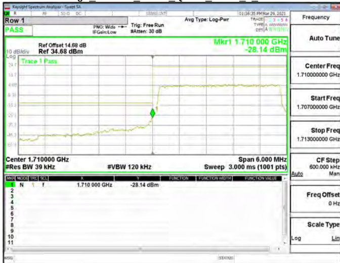
Band Edge_Band66_3MHz_QPSK_RB15_0_CH132657
