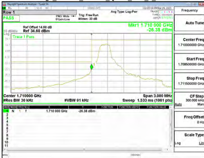
Band Edge_Band66_1.4MHz_QPSK_RB1_5_CH132665
