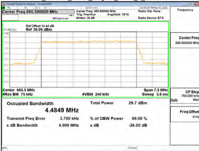
OBW_Band71_5MHz_16QAM_RB25_0_CH133297
