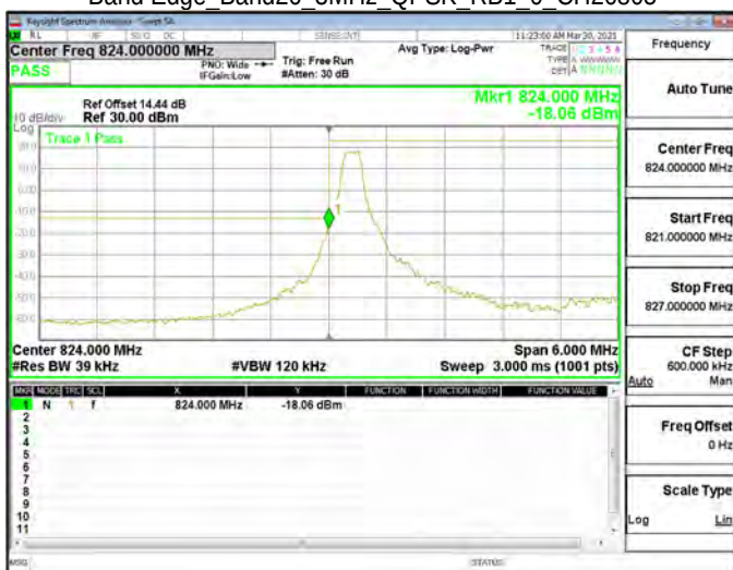
Band Edge_Band26_3MHz_QPSK_RB1_0_CH26805
