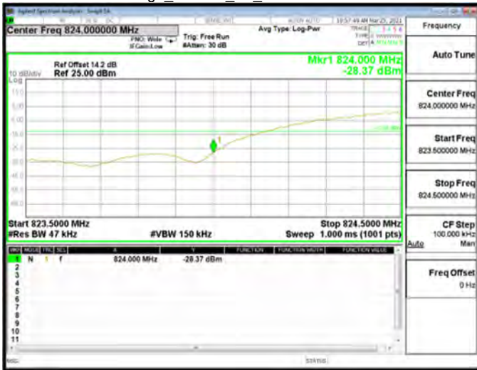
Band Edge_HSUPA_B5_Low CH4132-826.4
