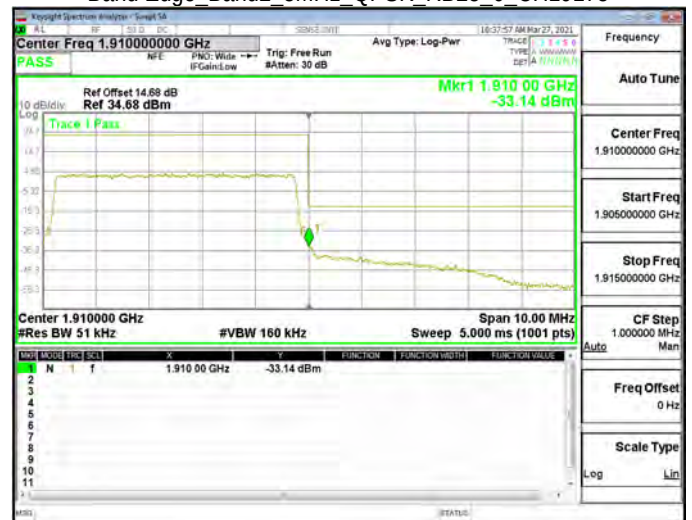
Band Edge_Band2_5MHz_QPSK_RB25_0_CH19175
