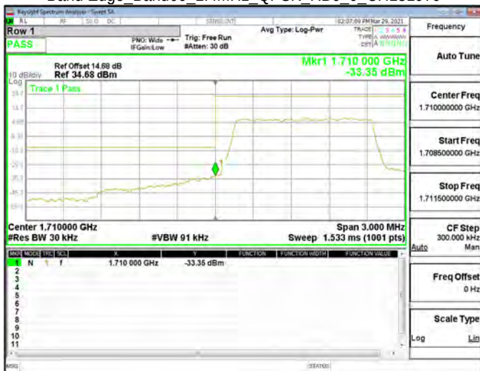
Band Edge_Band66_1.4MHz_QPSK_RB6_0_CH131979
