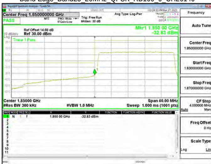
Band Edge_Band25_20MHz_QPSK_RB100_0_CH26140
