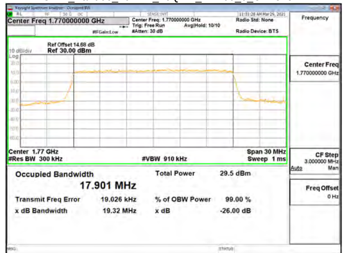
OBW_Band66_20MHz_16QAM_RB100_0_CH132572
