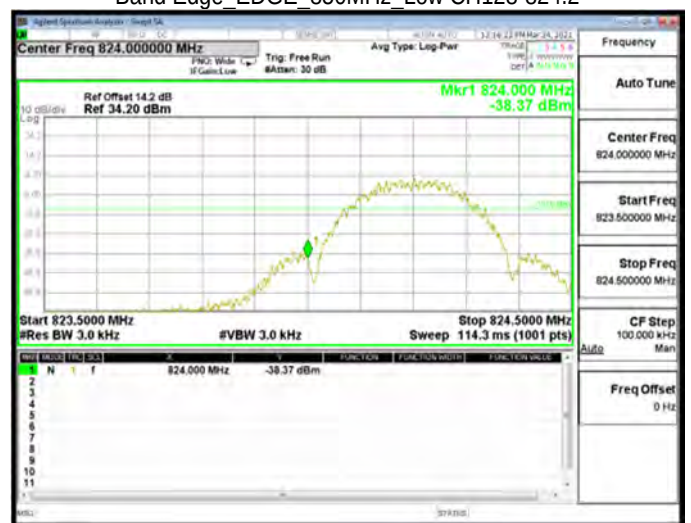
Band Edge_EDGE_850MHz_Low CH128-824.2
