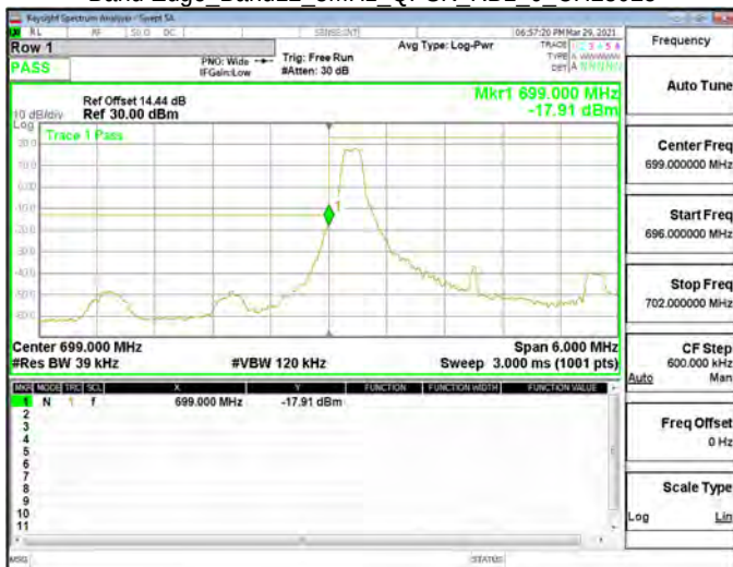
Band Edge_Band12_3MHz_QPSK_RB1_0_CH23025
