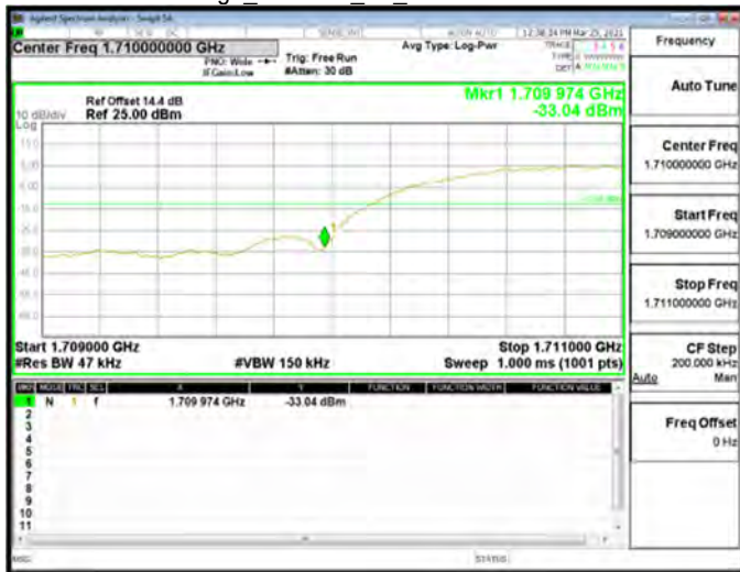
Band Edge_WCDMA_B4_Low CH1312-1712.4
