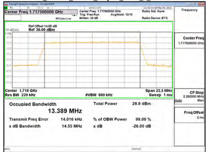
OBW Band66_15MHz_64QAM_RB75_0_CH132322
