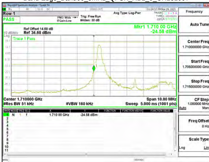
Band Edge_Band66_5MHz_QPSK_RB1_0_CH131997
