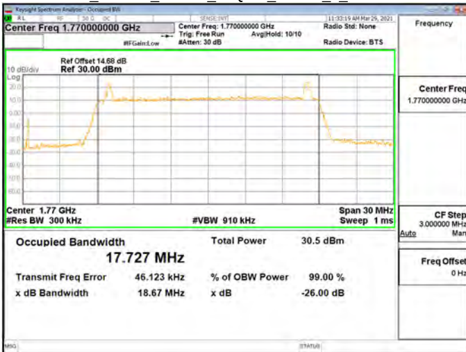
OBW_Band66_20MHz_64QAM_RB100_0_CH132572
