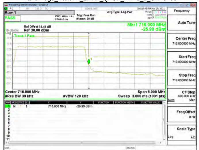
Band Edge_Band12_3MHz_QPSK_RB15_0_CH23165
