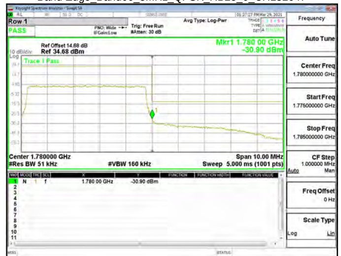
Band Edge_Band66_5MHz_QPSK_RB25_0_CH132647
