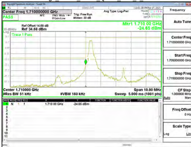
Band Edge_Band4_5MHz_QPSK_RB1_0_CH19975
