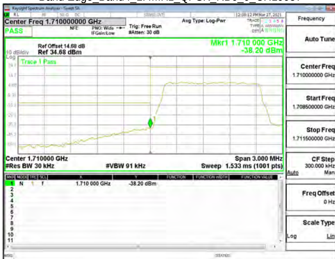
Band Edge_Band4_1.4MHz_QPSK_RB6_0_CH19957
