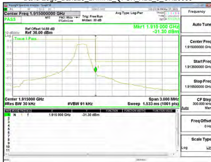
Band Edge Band25 1.4MHz QPSK RB1 5 CH26683
