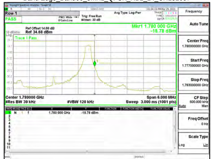
Band Edge_Band66_3MHz_QPSK_RB1_14_CH132657
