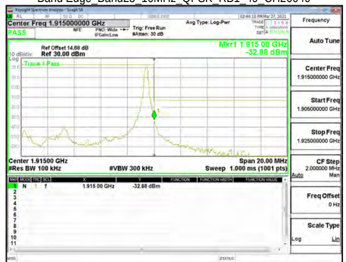
Band Edge_Band25_10MHz_QPSK_RB1_49_CH26640
