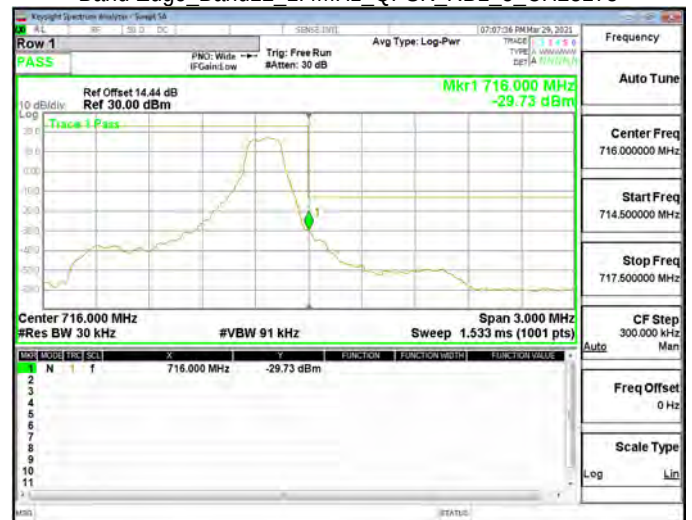
Band Edge_Band12_1.4MHz_QPSK_RB1_5_CH23173
