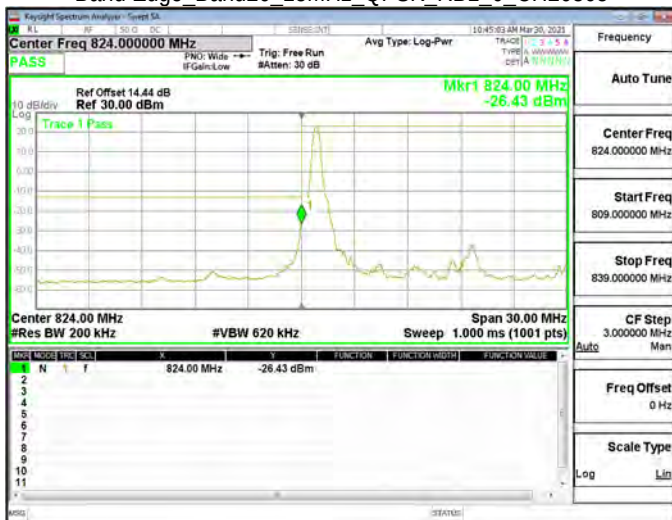
Band Edge Band26_15MHz_QPSK_RB1_0_CH26865
