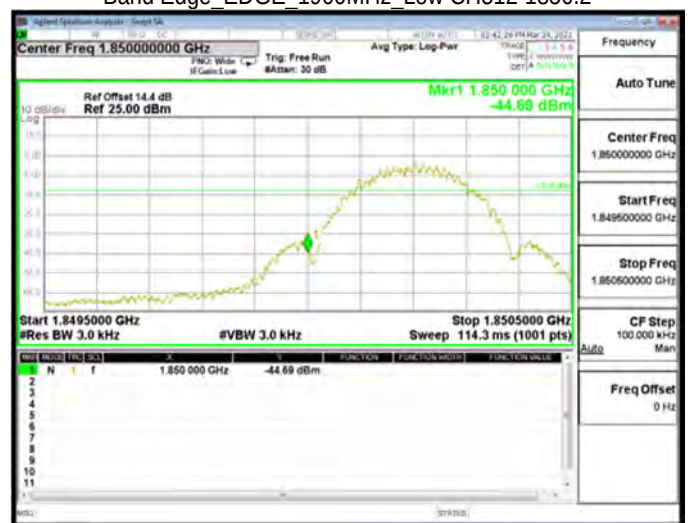
Band Edge_EDGE_1900MHz_Low CH512-1850.2
