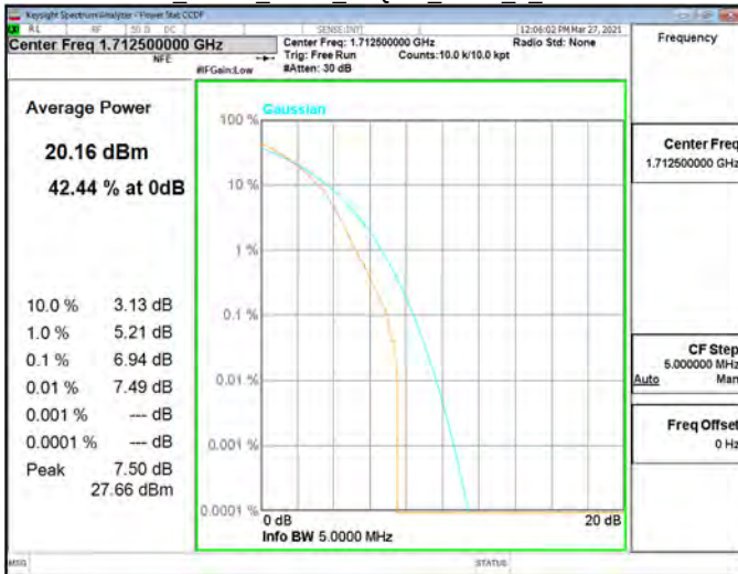
CCDF Band4 5MHz 64QAM RB25 0 CH20175
