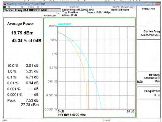
CCDF Band5 10MHz 64QAM RB50 0 CH20600
