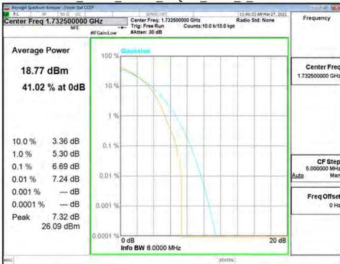
CCDF_Band4_15MHz_64QAM_RB75_0_CH20325
