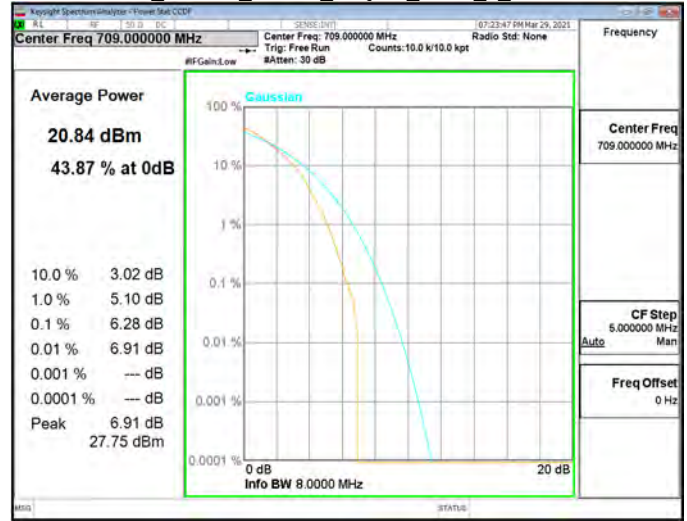
CCDF Band17 10MHz 64QAM_RB50_0_CH23790
