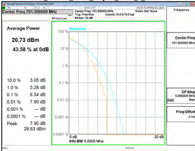
CCDF Band12_5MHz_64QAM_RB25_0_CH23095
