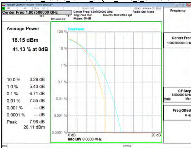
CCDF_Band25_15MHz_64QAM_RB75_0_CH26615
