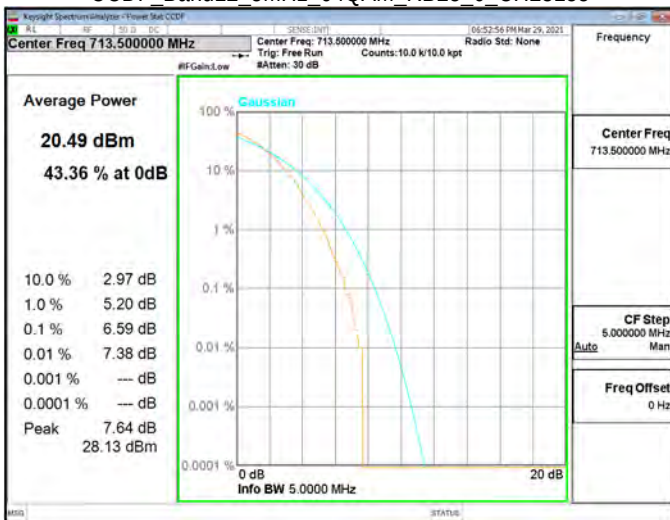
CCDF Band12_5MHz_64QAM_RB25_0_CH23155
