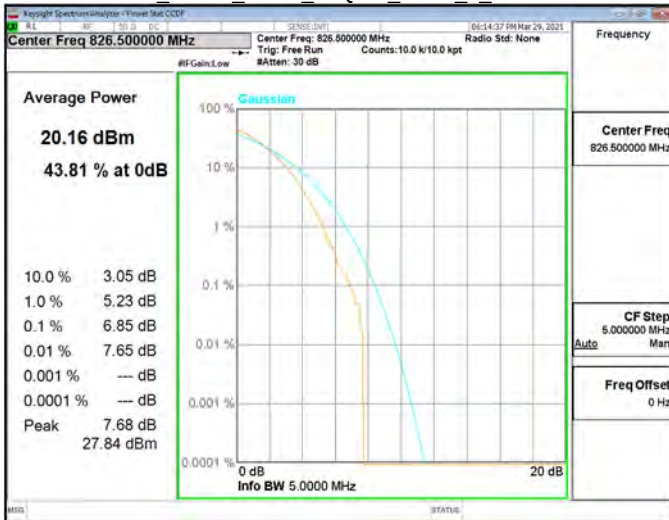
CCDF Band5 5MHz 64QAM RB25 0 CH20525
