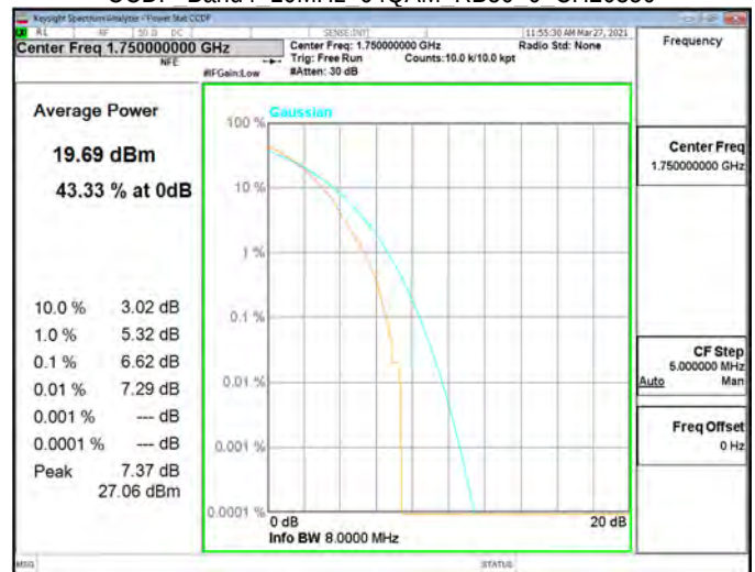
CCDF Band4 10MHz 64QAM RB50 0 CH20350
