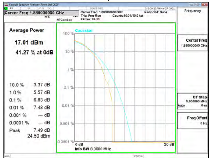
CCDF_Band2_20MHz_64QAM_RB100_0_CH19100
