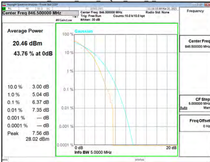
CCDF_Band26_5MHz_64QAM_RB25_0_CH27015
