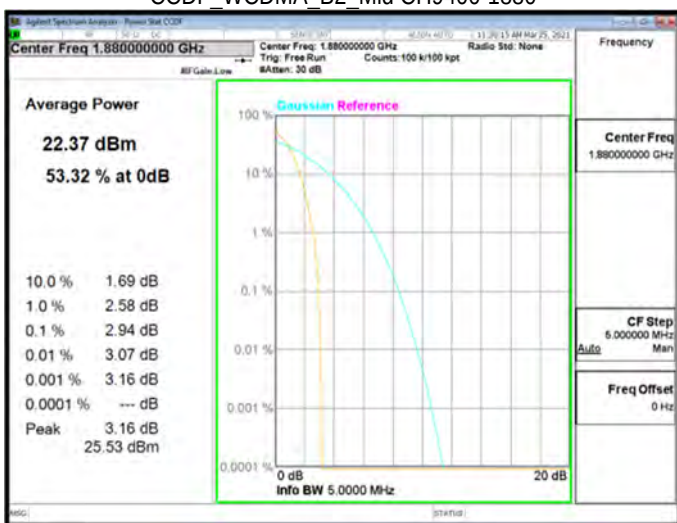
CCDF_WCDMA_B2_Mid CH9400-1880
