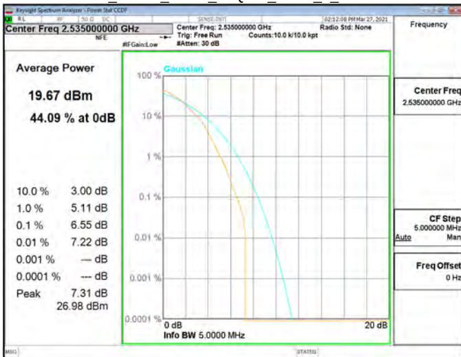
CCDF Band7 5MHz 64QAM RB25 0 CH21425
