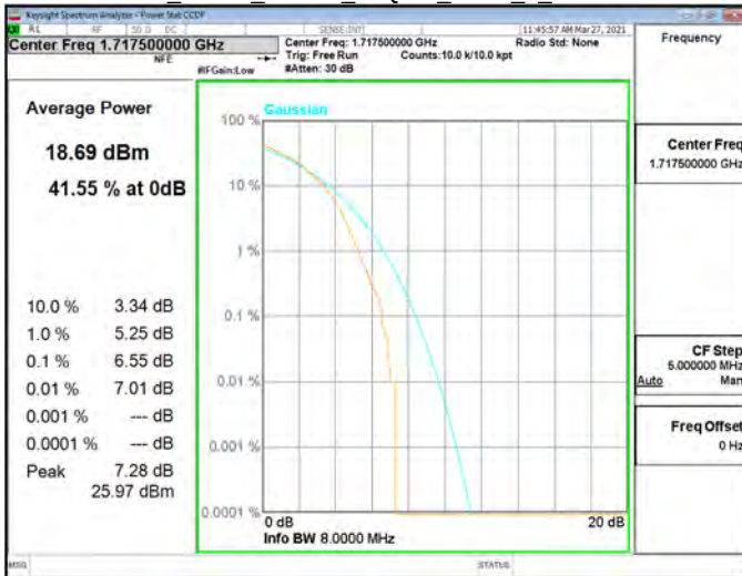
CCDF_Band4_15MHz_64QAM_RB75_0_CH20175
