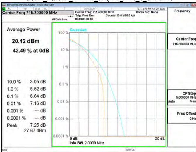
CCDF Band12 1.4MHz 64QAM_RB6_0_CH23173
