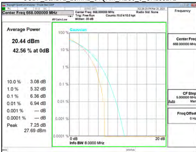
CCDF_Band71_10MHz_64QAM_RB50_0_CH133172
