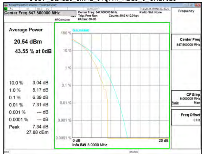
CCDF Band26 3MHz 64QAM_RB15_0_CH27025
