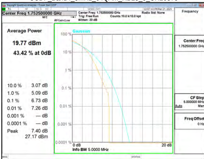
CCDF Band4 5MHz 64QAM RB25 0 CH20375
