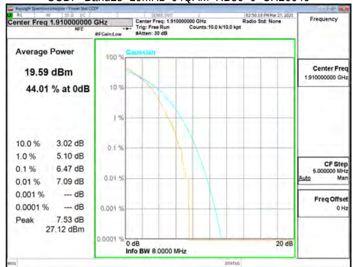
CCDF Band25 10MHz 64QAM_RB50_0_CH26640
