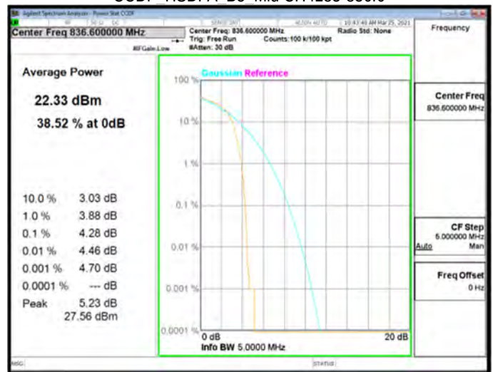
CCDF_HSDPA_B5_Mid CH4183-836.6
