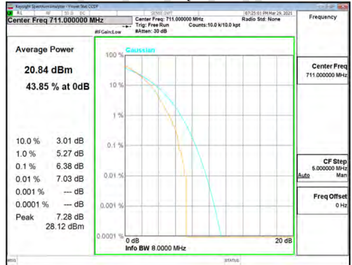
CCDF Band17 10MHz 64QAM_RB50_0_CH23800
