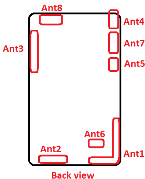
Fig.23 Antenna position of EUT
