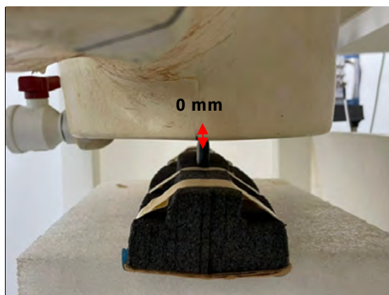
Fig.19 EUT Right side to flat phantom
