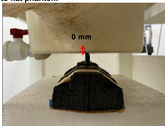
Fig.20 EUT Left side to flat phantom
