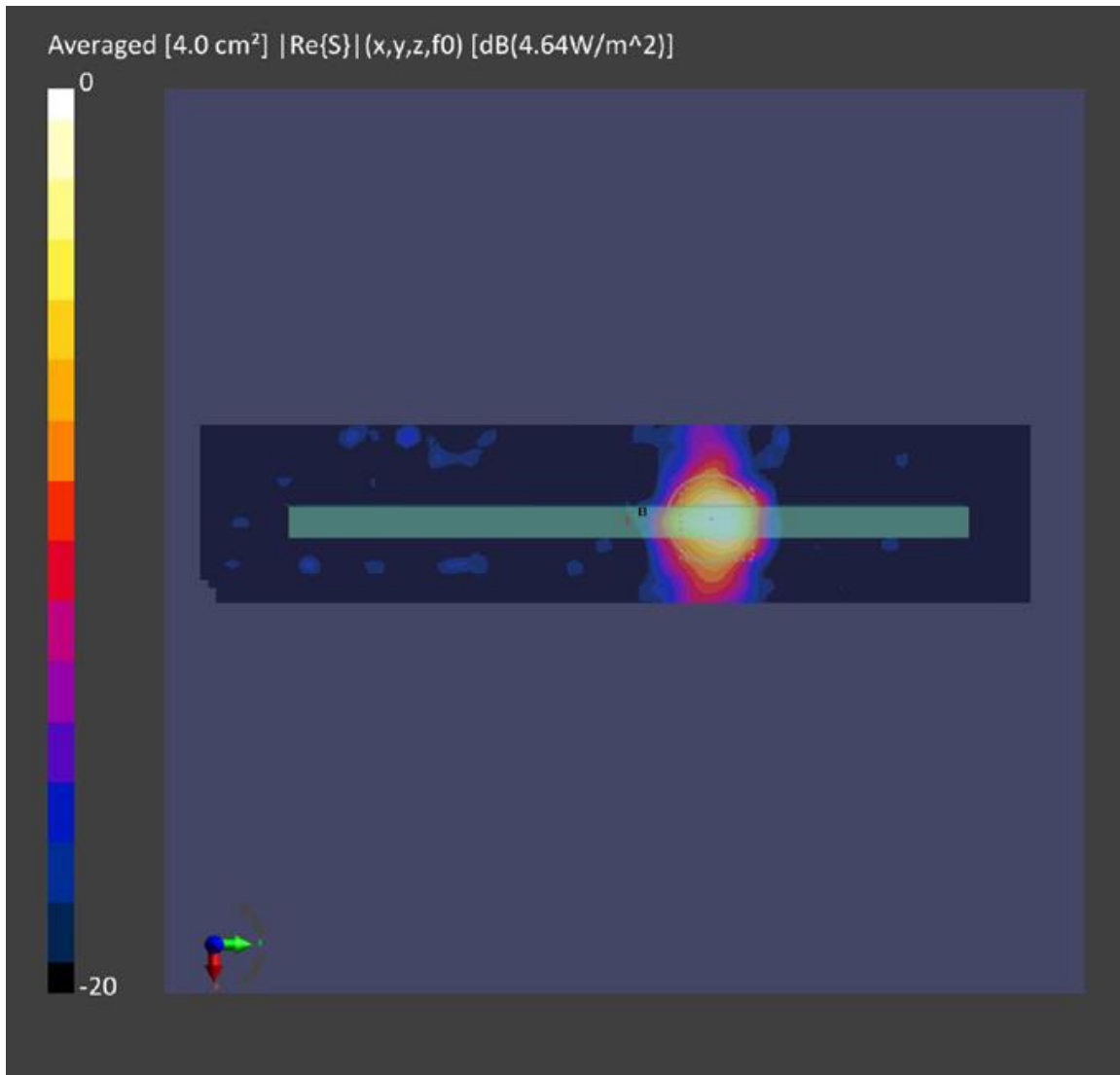
Figure 8-3: 4cm2-averaged power density distribution measured at input.power.limit of 3.087 dBm on the Right Side surface for n258 beam 37
