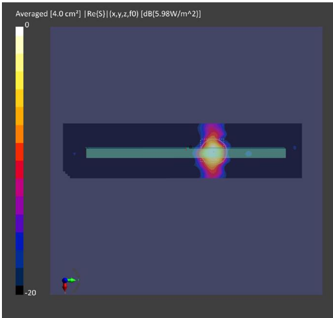
Figure 8-2: 4cm2-averaged power density distribution measured at input.power.limit of 3.064 dBm on the Right Side surface for n257 beam 35
