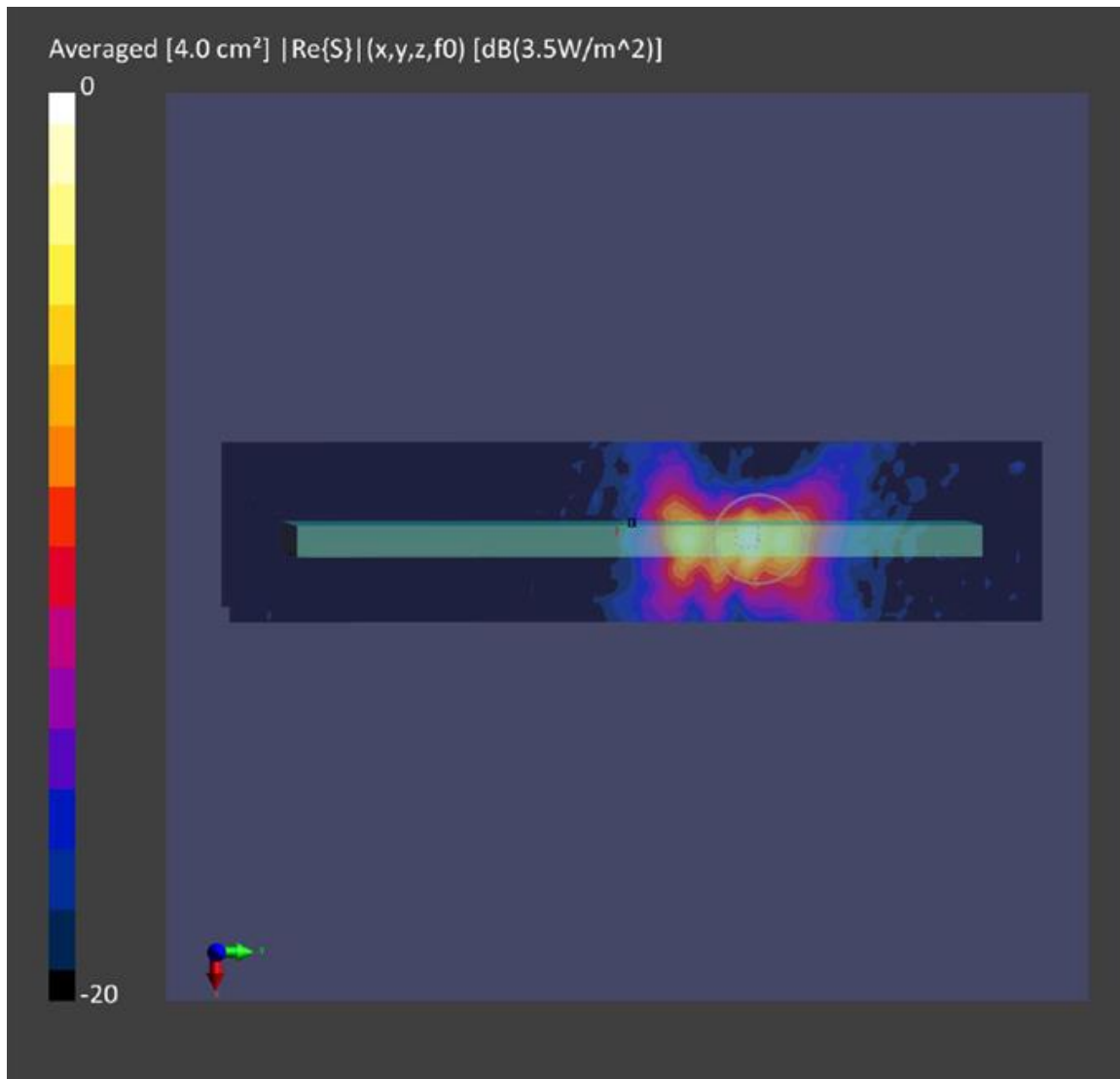
Figure 8-4: 4cm2-averaged power density distribution measured at input.power.limit of 2.841 dBm on the Back for n260 beam 40
