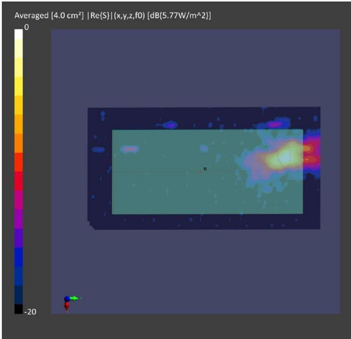
Figure 8-5: 4cm2-averaged power density distribution measured at input.power.limit of 4.871dBm on the back surface for n261 beam 42
