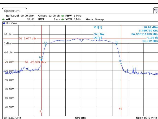
26dB Bandwidth
