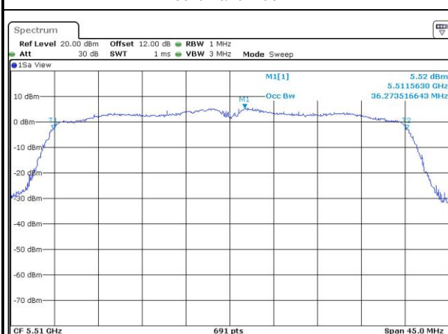
99% Bandwidth
