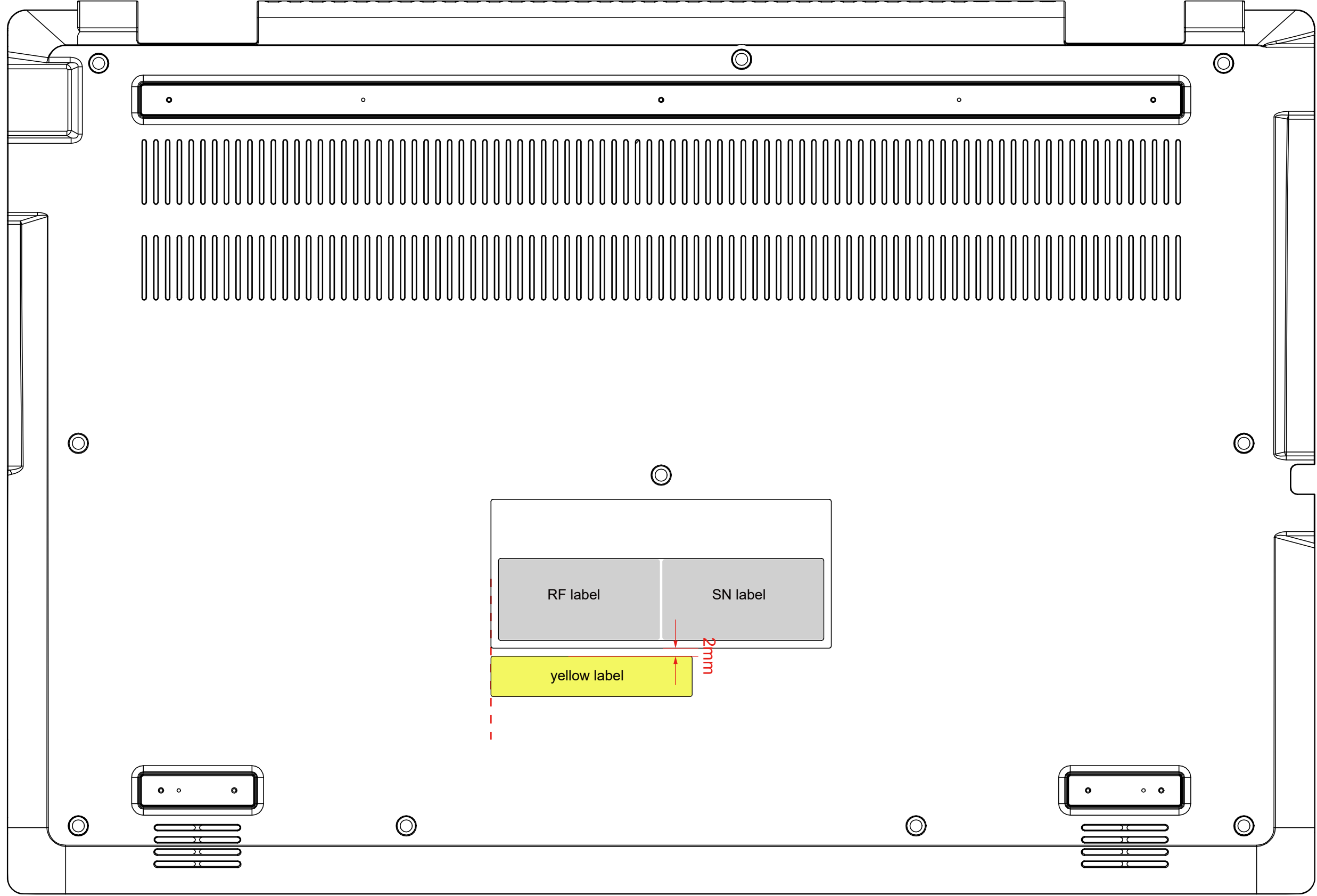
D壳 label location
