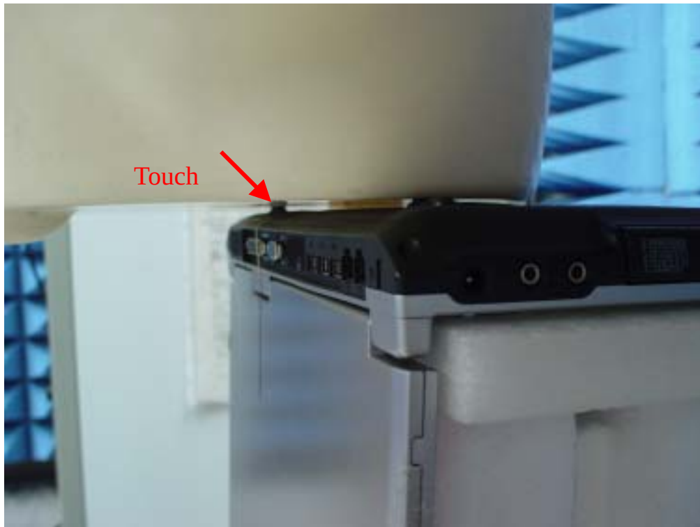
Fig.5 Photograph of the Bottom face of the EUT is paralleled with flat phantom. Spacing between EUT and phantom - In contact (0 cm)
