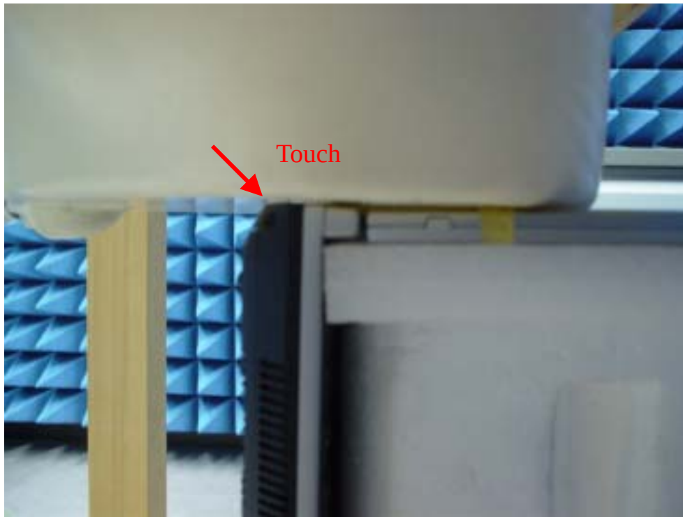
Fig.3 Photograph of the Rear side of the EUT is paralleled with flat phantom; Spacing between EUT and phantom - In contact (0 cm).
