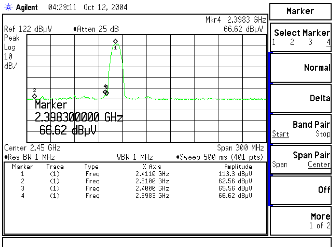
Figure Channel 1: (Vertical)
