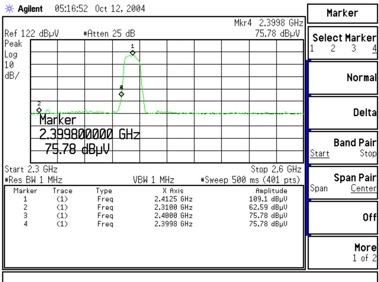
Figure Channel 1: (Vertical)
