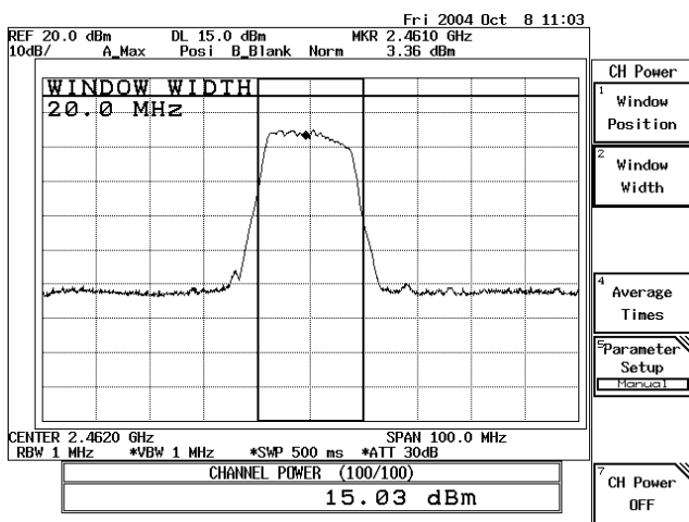
54Mbps-CH11
