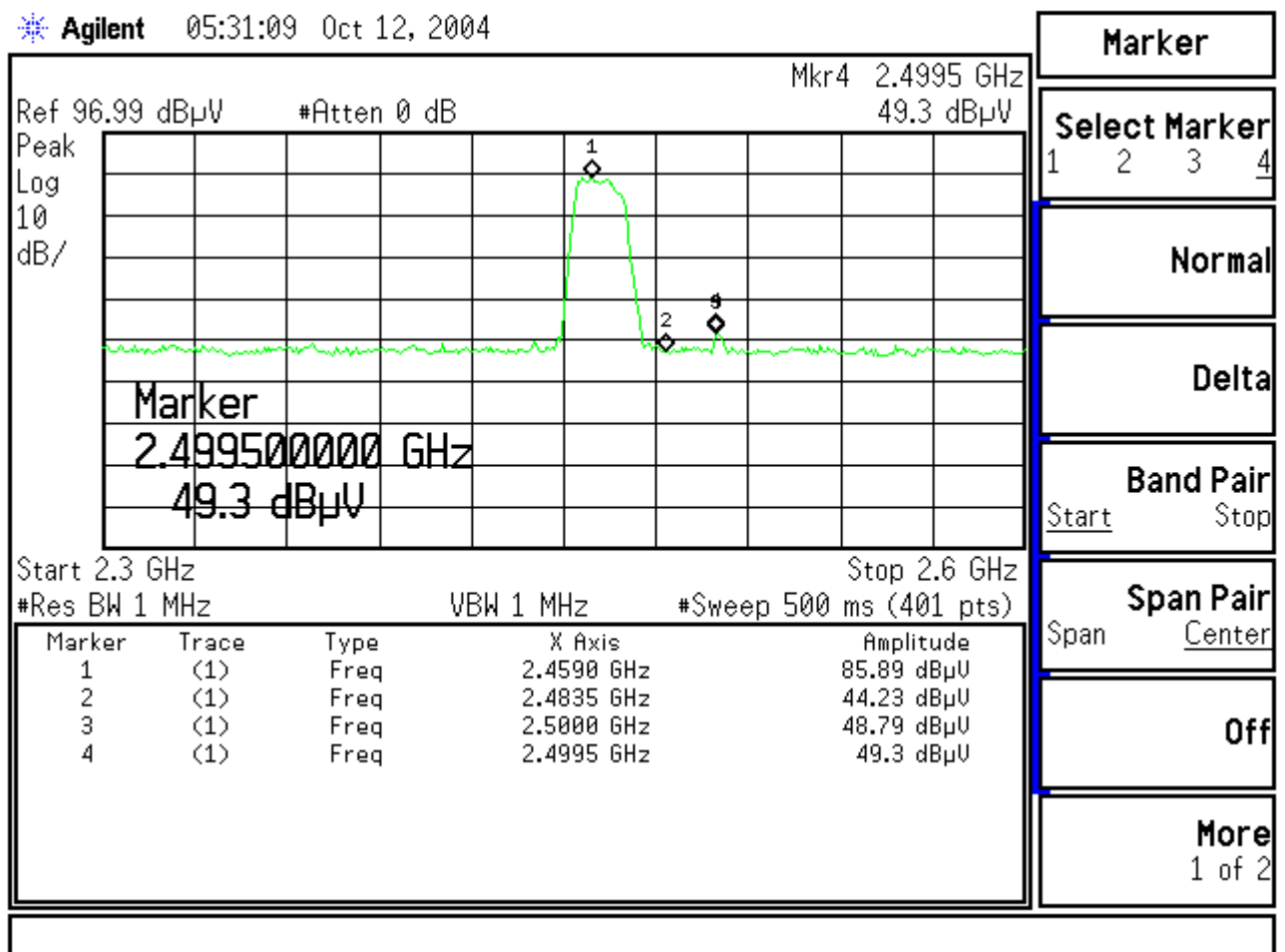
Figure Channel 11: (Horizontal)
