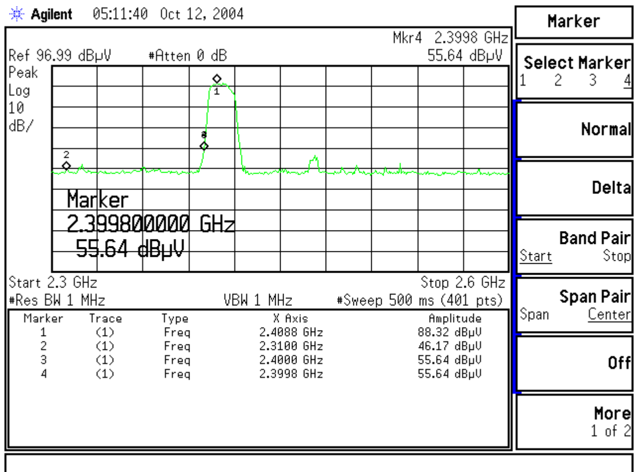
Figure Channel 1: (Horizontal)
