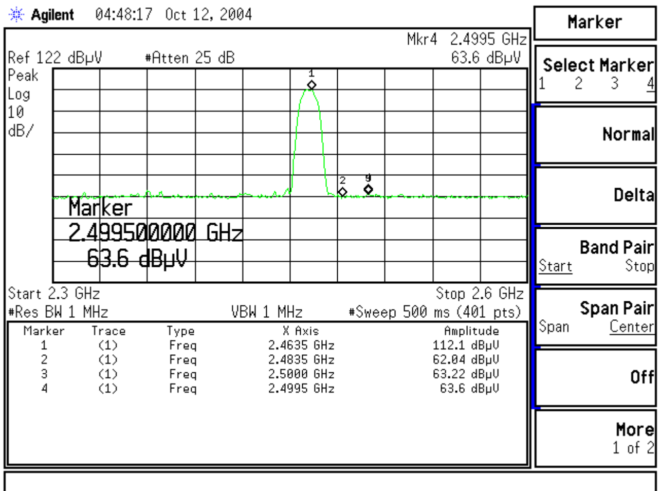
Figure Channel 11: (Vertical)
