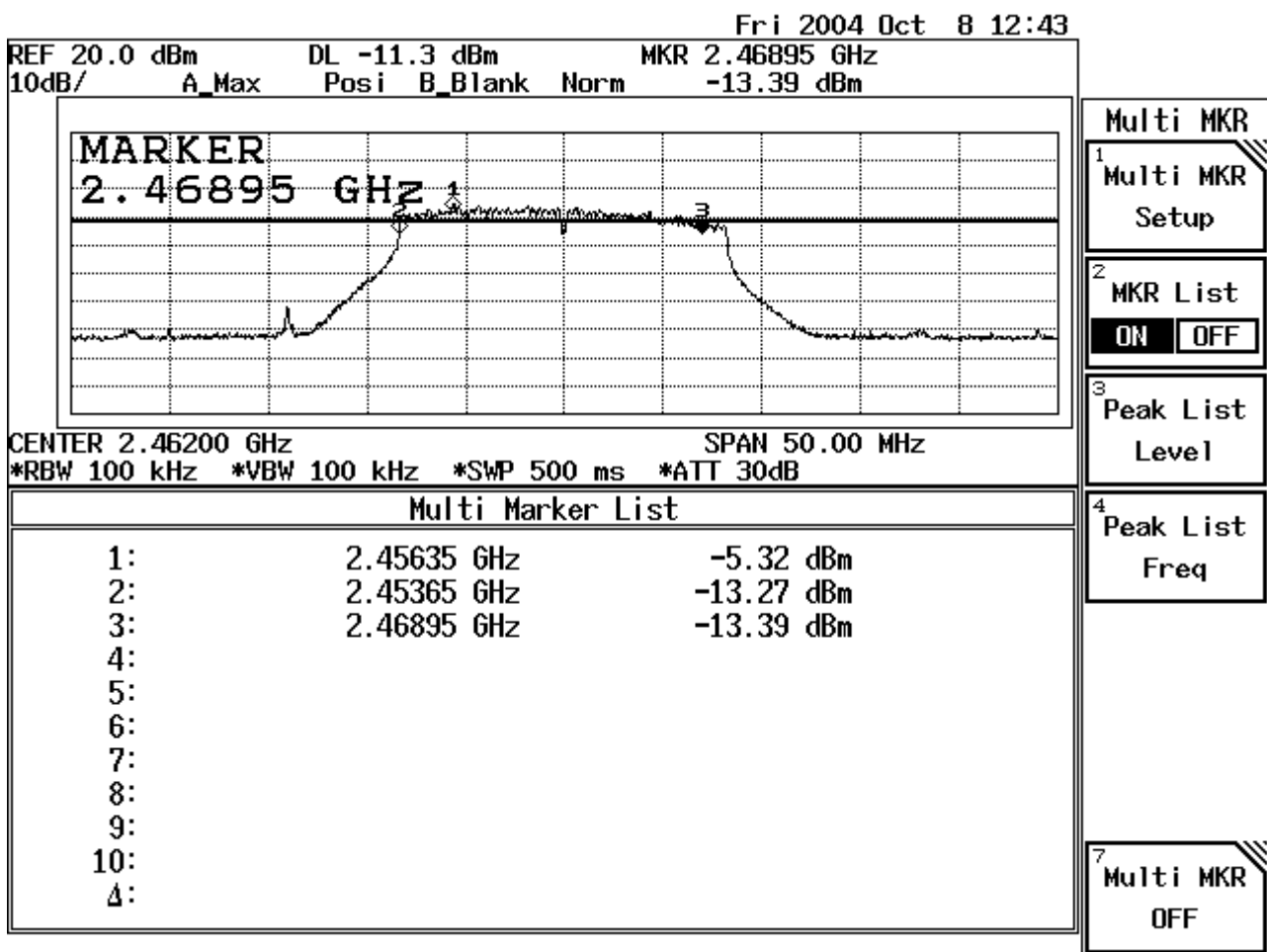
Figure Channel 11: 54Mbps
