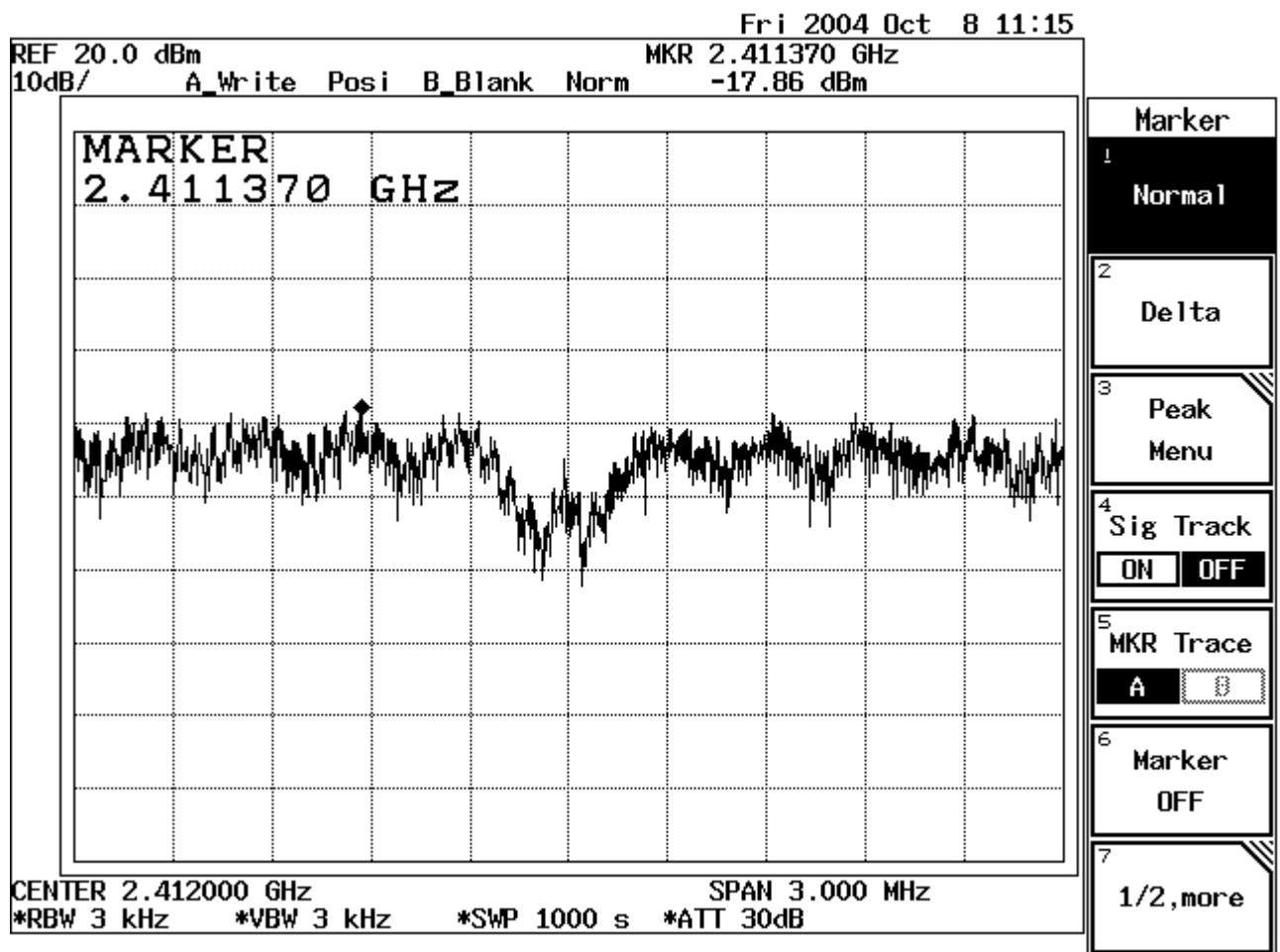
Figure Channel 1:
