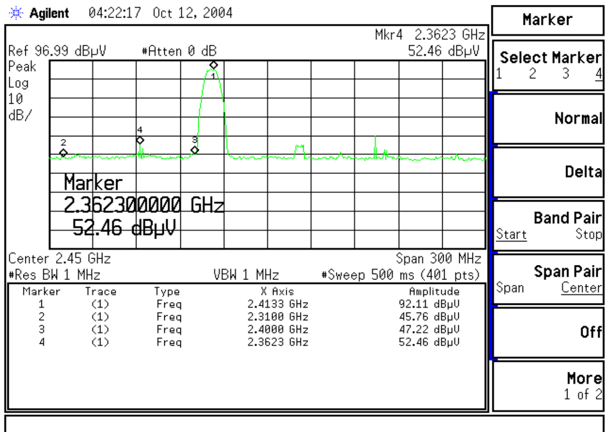
Figure Channel 1: (Horizontal)
