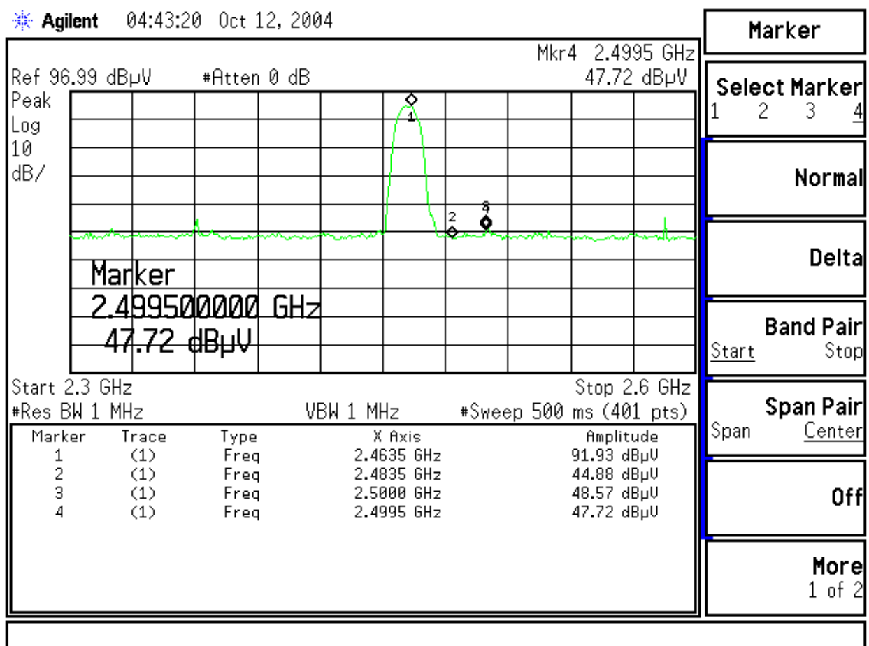
Figure Channel 11: (Horizontal)
