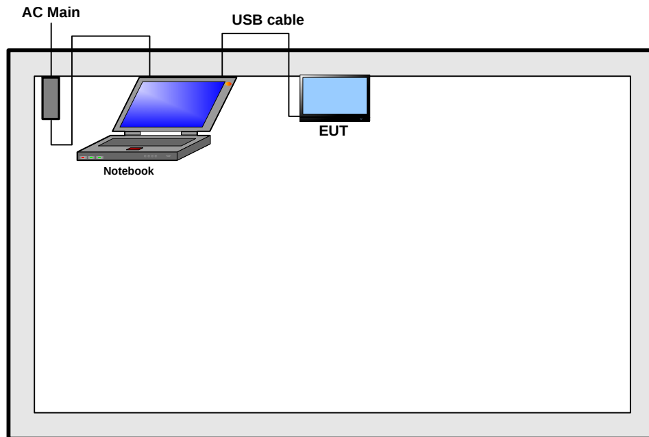
Test Setup Diagram - Radiated Test Above 1GHz (Mode 1)
