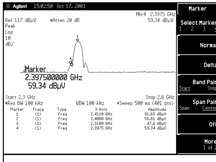
Figure Channel 01: (Vertical)
