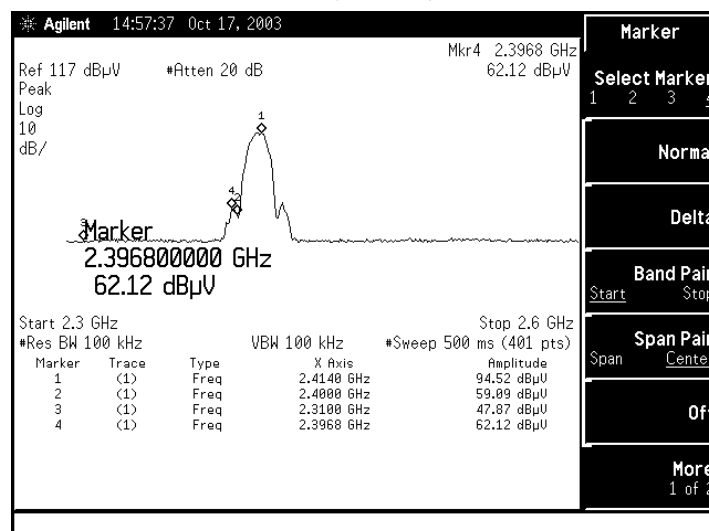
Figure Channel 01: (Vertical)
