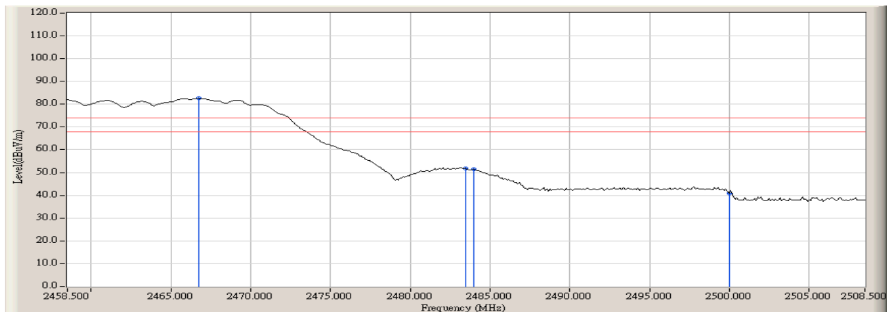
Figure Channel 11: (Vertical)
