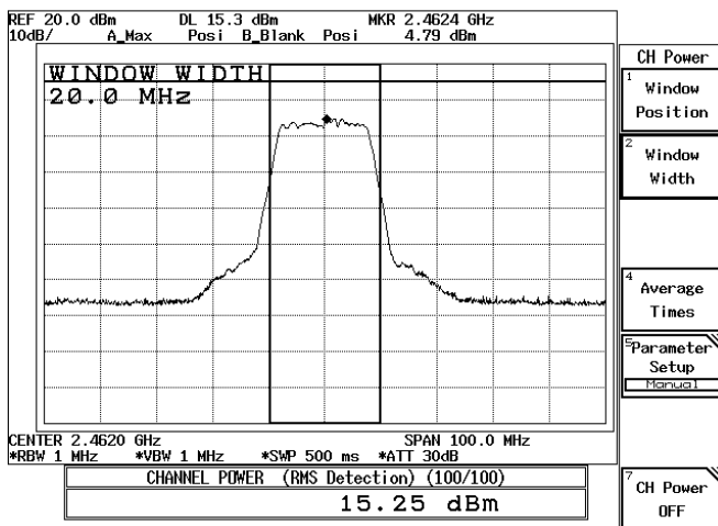
54Mbps-CH11
