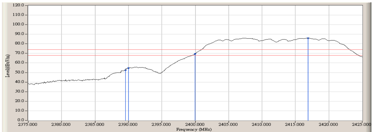
Figure Channel 1: (Horizontal)
