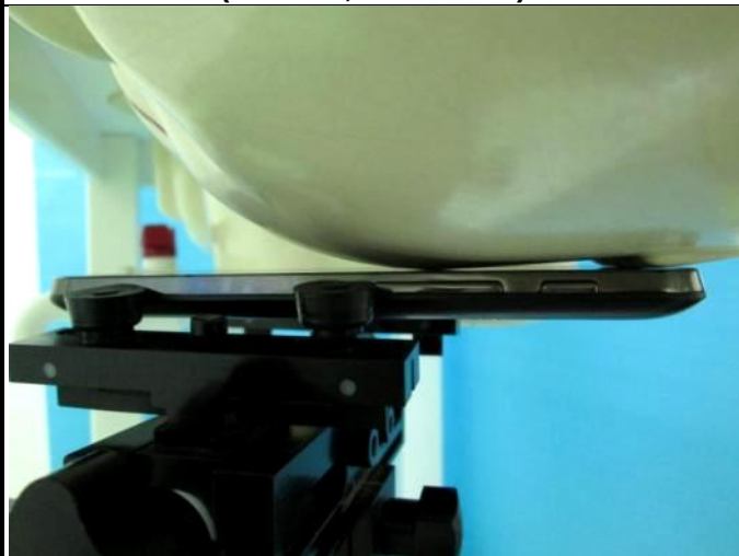
Left Cheek (Handset, Head Mode)
