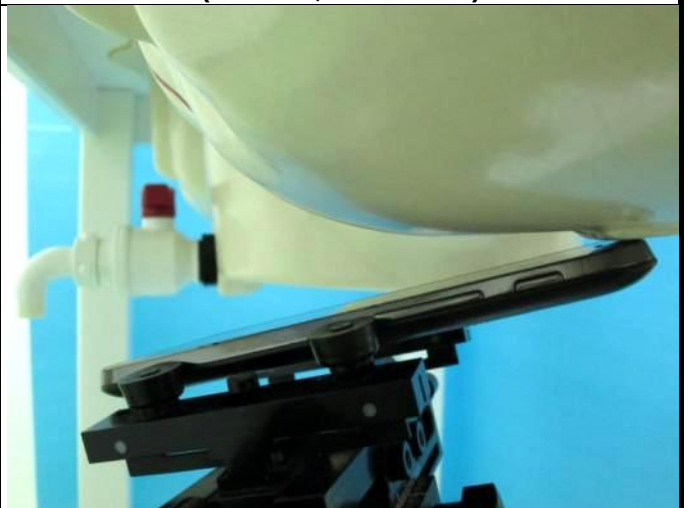
Left Tilted (Handset, Head Mode)
