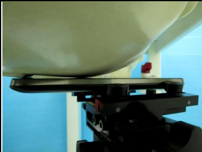
Right Cheek (Handset, Head Mode)
