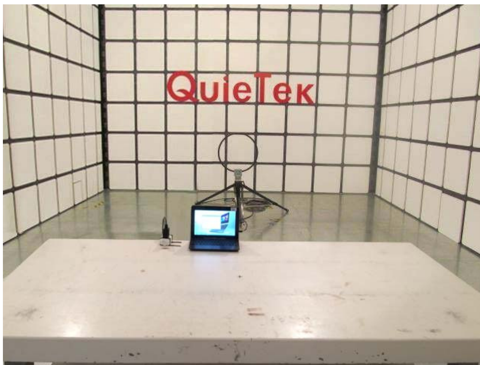
Description: Radiated Emission Test Setup for Below 30MHz
