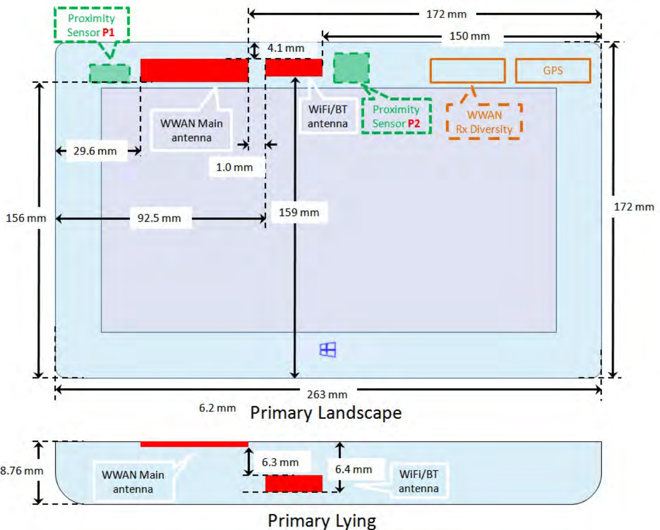
Fig.12 Antenna position of EUT
