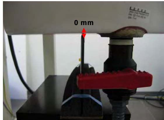
Fig.7 EUT Primary Landscape mode to flat phantom (Test distance is 0 mm)
