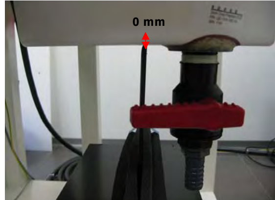
Fig.6 EUT Secondary Portrait mode to flat phantom (Test distance is 0 mm)
