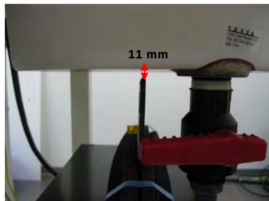
Fig.9 EUT Secondary Landscape mode to flat phantom (Test distance is 11 mm)
