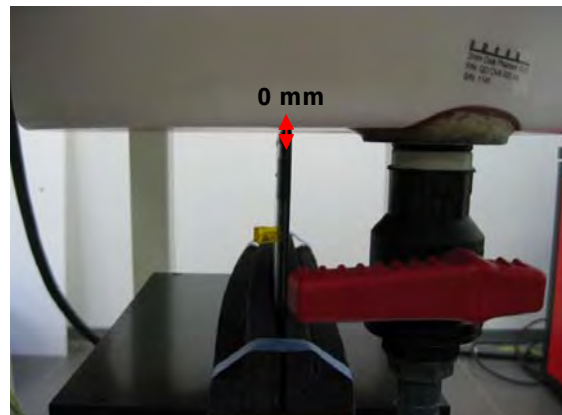
Fig.8 EUT Secondary Landscape mode to flat phantom (Test distance is 0 mm)
