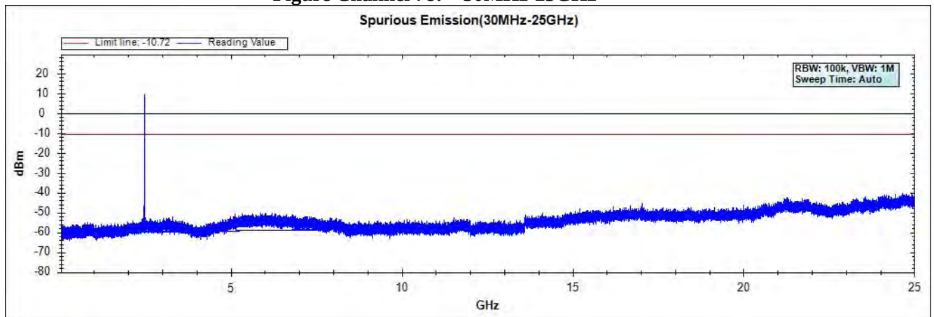
Figure Channel 78: 30MHz-25GHz
