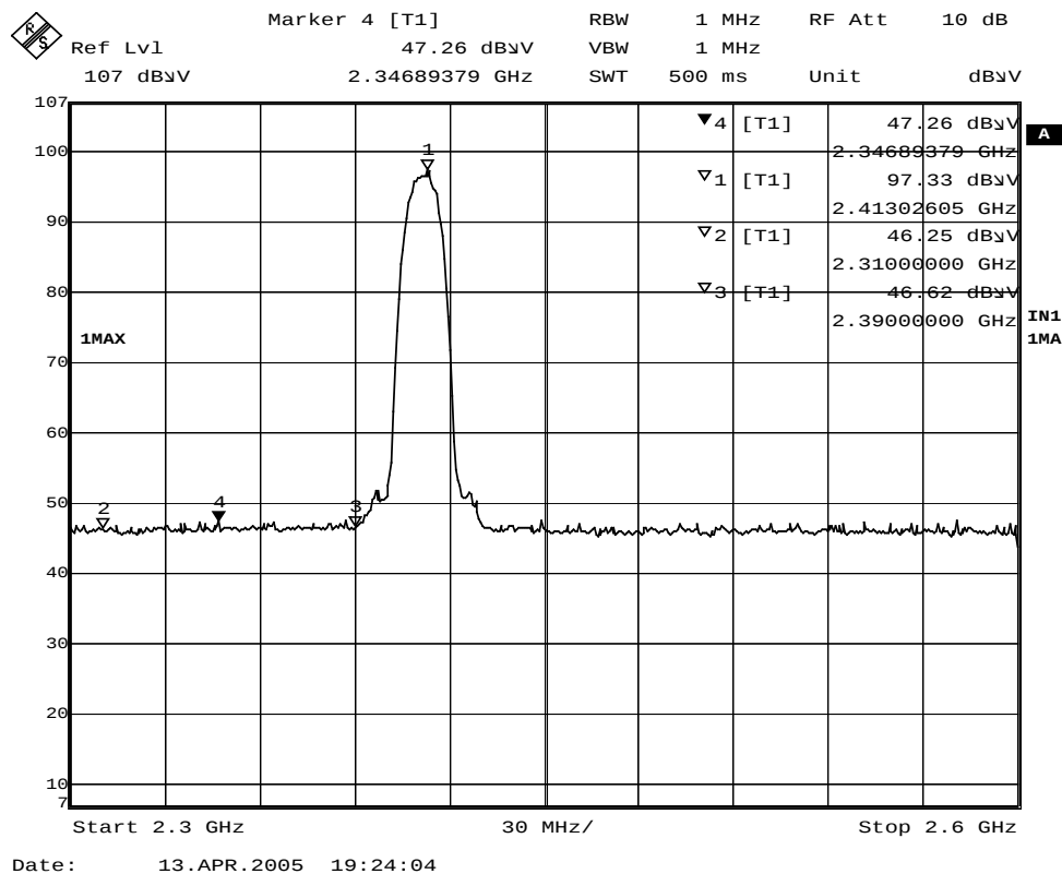
Figure Channel 1: (Horizontal)
