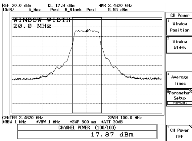
54Mbps-CH11
