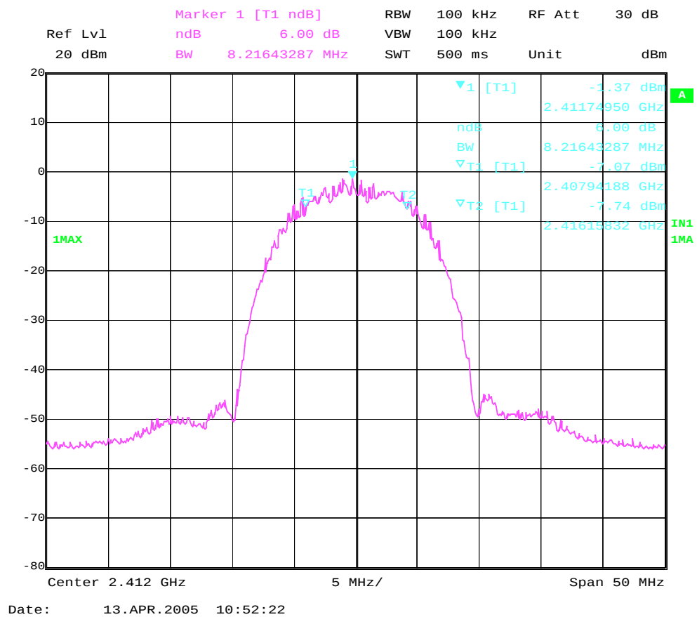
Figure Channel 1: 11Mbps
