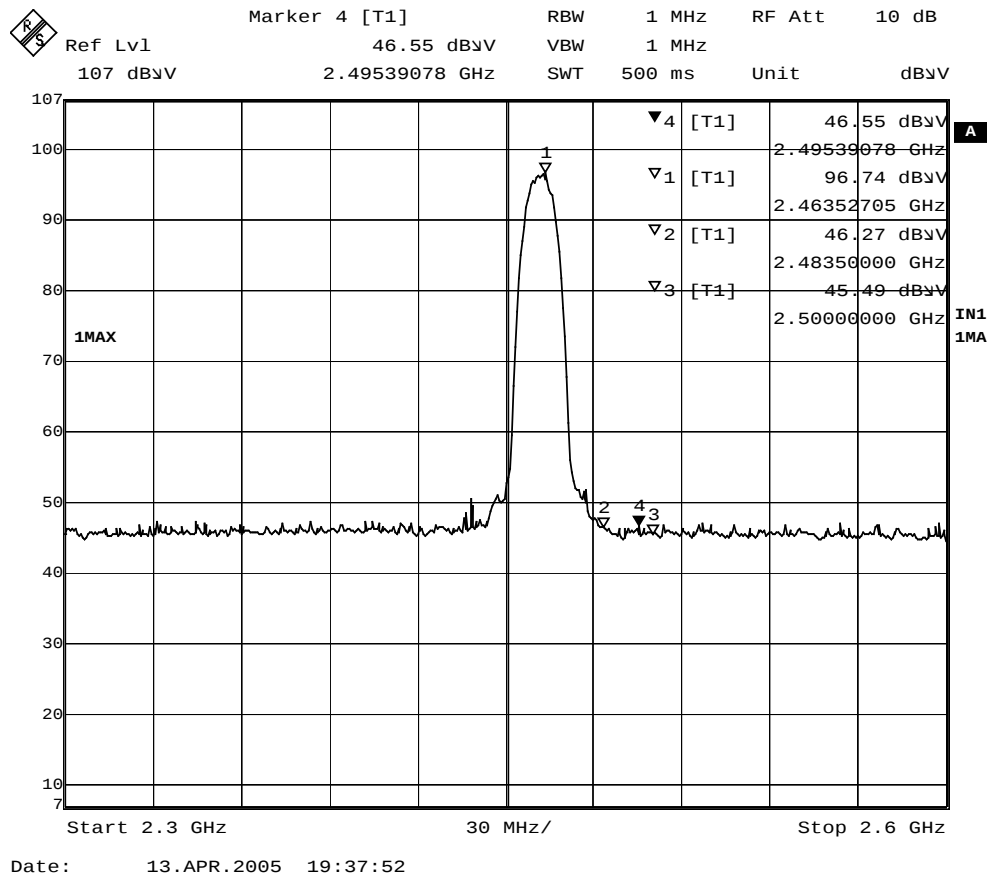
Figure Channel 11: (Horizontal)
