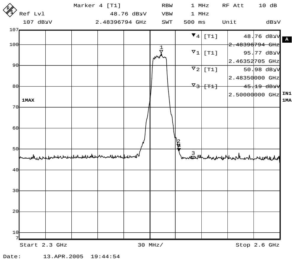
Figure Channel 11: (Horizontal)
