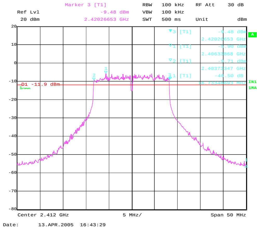
Figure Channel 1: 54Mbps
