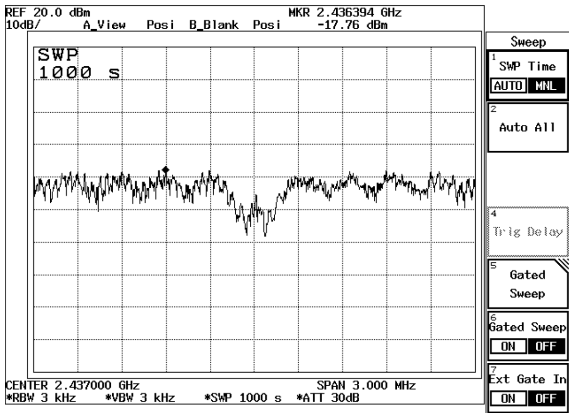
Figure Channel 6:
