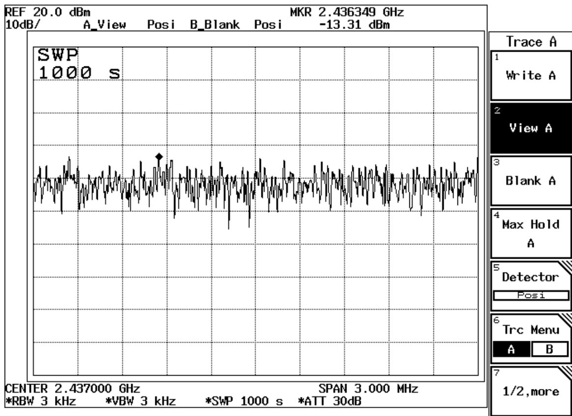
Figure Channel 6: 11Mbps
