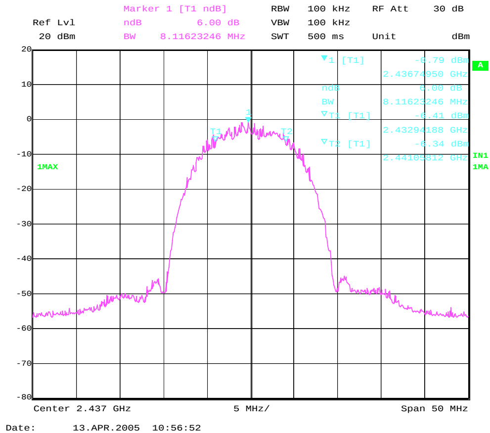
Figure Channel 6: 11Mbps
