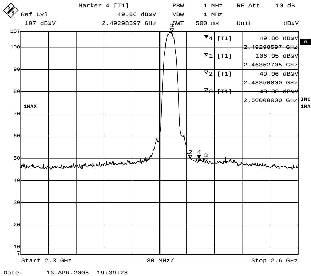
Figure Channel 11: (Vertical)
