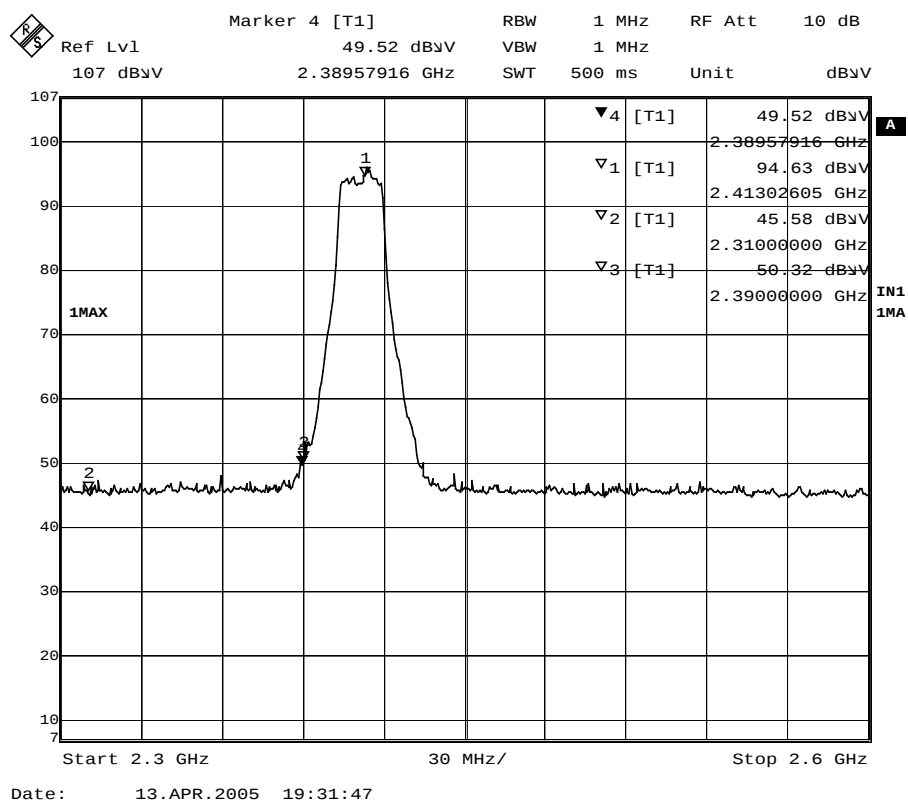
Figure Channel 1: (Horizontal)
