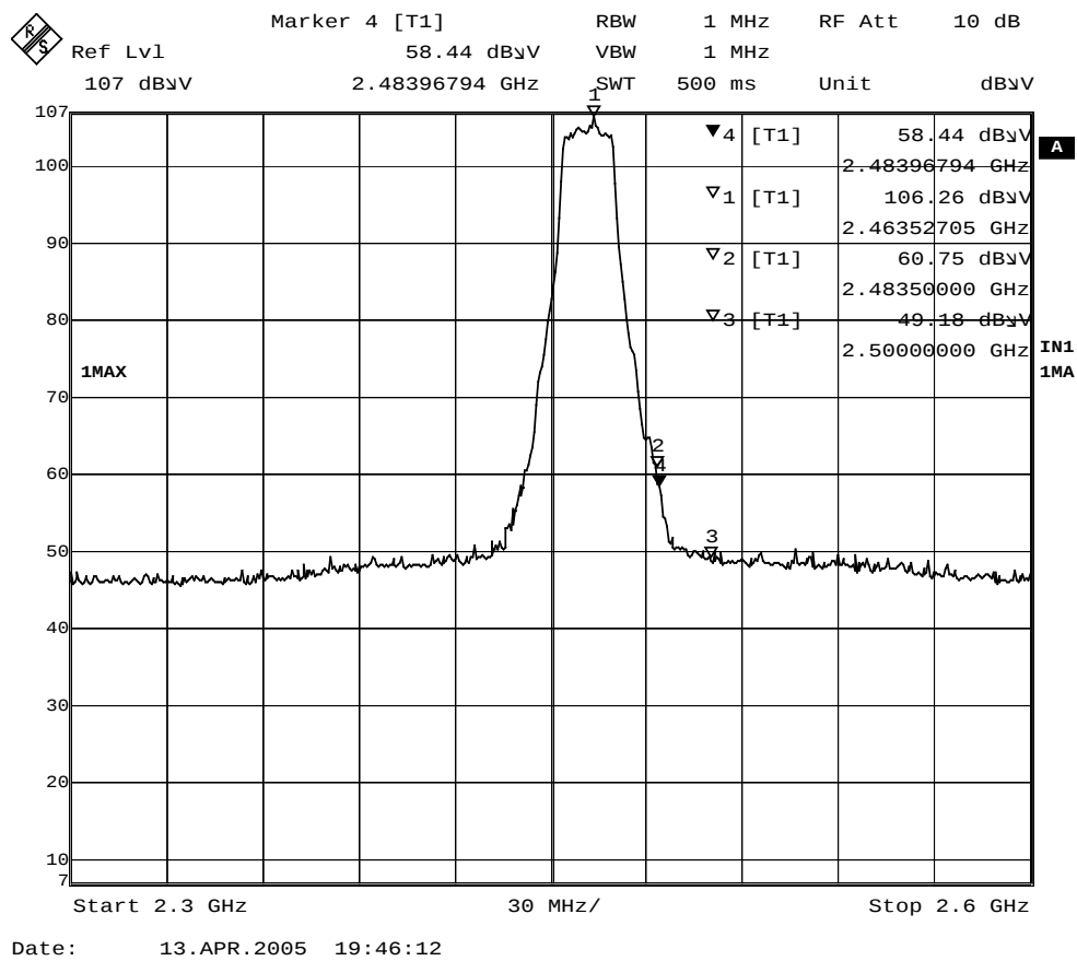
Figure Channel 11: (Vertical)
