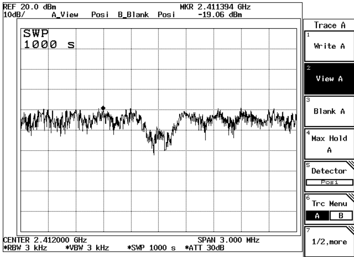
Figure Channel 1:
