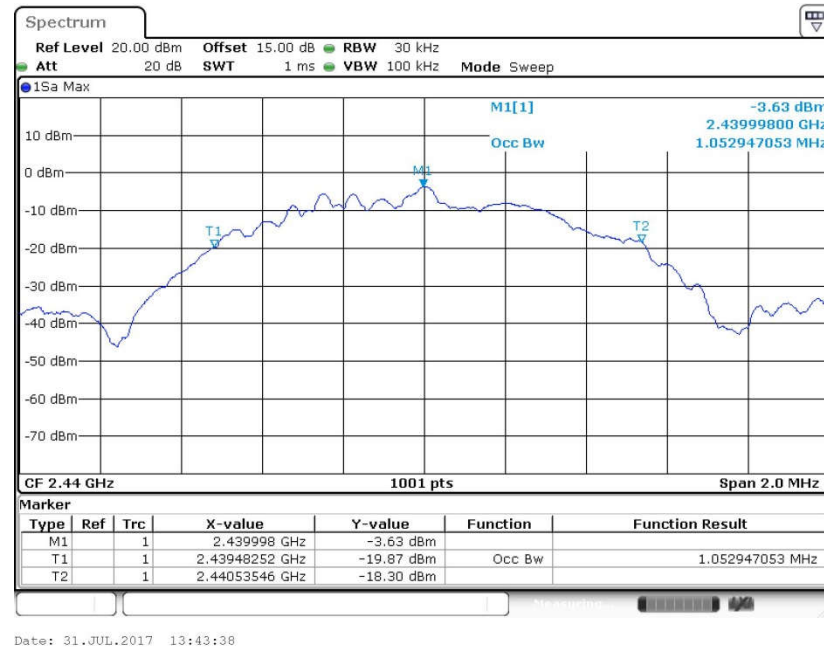
99% Occupied Bandwidth Plot on Channel 19
