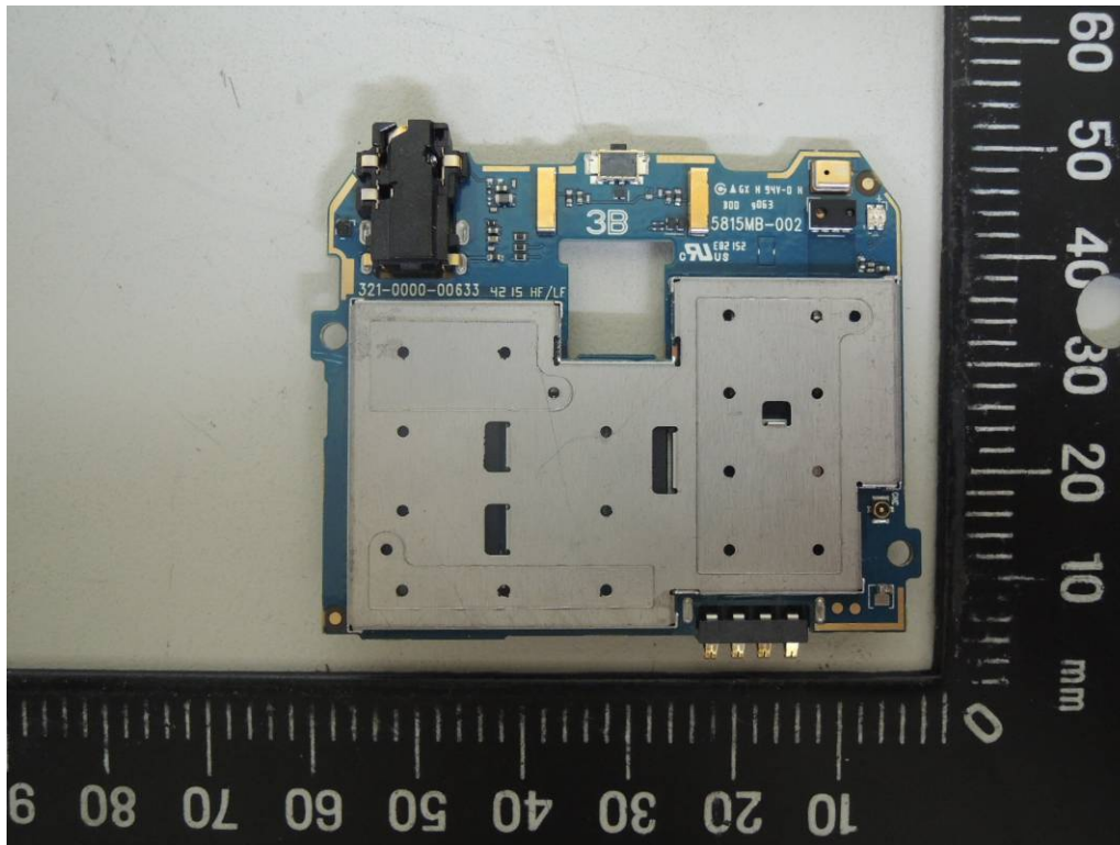
Internal View of EUT – 4 (16G)
