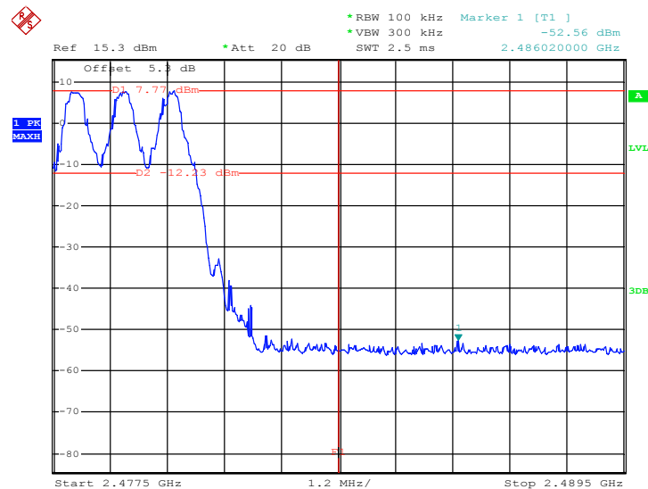
Hopping Mode High Band Edge Plot
