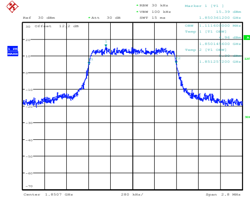
Lowest Channel / 1.4MHz / 16QAM
