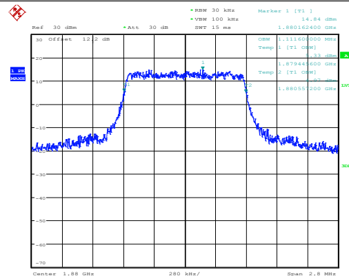
Middle Channel / 1.4MHz / 16QAM
