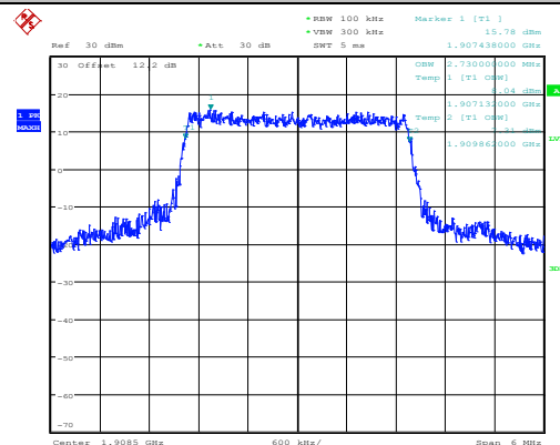
Highest Channel / 3MHz / 16QAM
