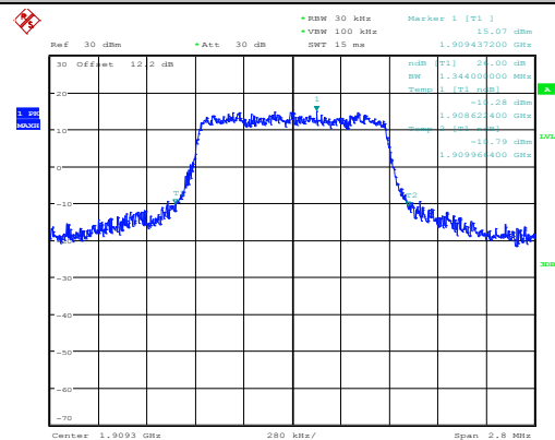
Highest Channel / 1.4MHz / 16QAM
