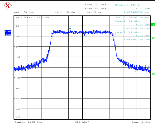
Middle Channel / 3MHz / 16QAM
