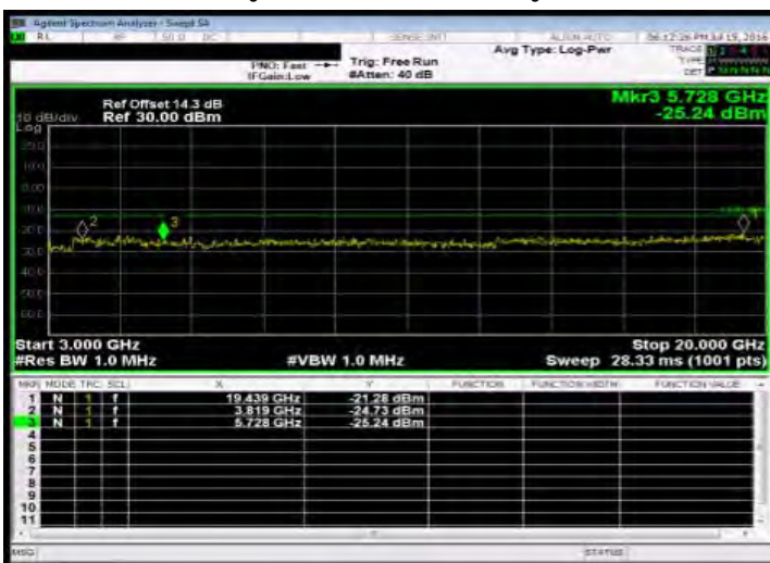
Out of Band Emission High_Band2 1.4MHz_QPSK 1 0_HighCH19193-1909.3
