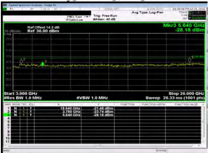
Out of Band Emission High_Band2 20MHz_QPSK 1 0_HighCH19100-1900
