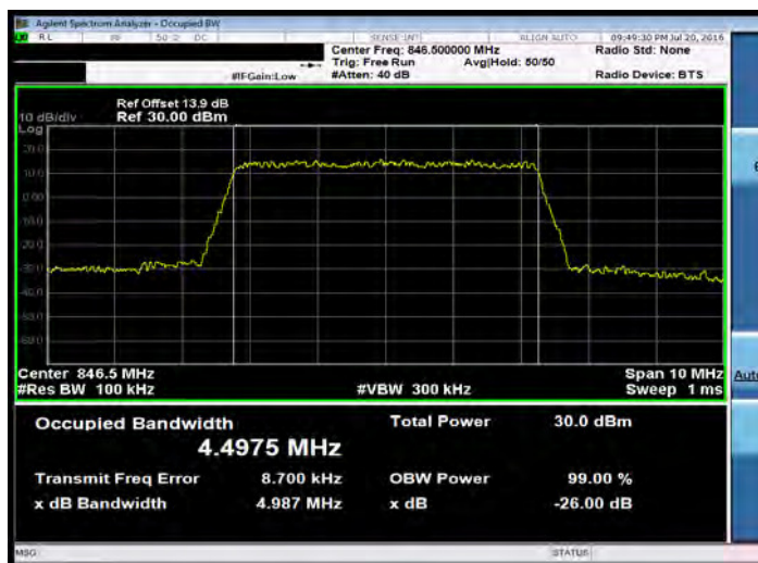
LTE Band 26 for Part 90S_5M_QPSK_HIGH
