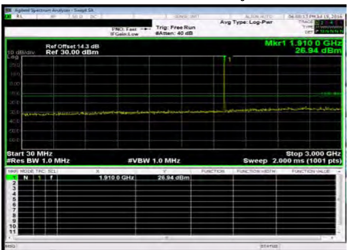
Out of Band Emission Low_Band2 3MHz_QPSK 1 0_HighCH19185-1908.5
