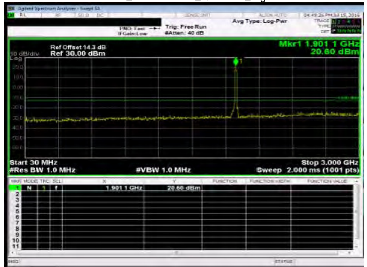
Out of Band Emission Low_Band2 20MHz_QPSK 1 0_HighCH19100-1900
