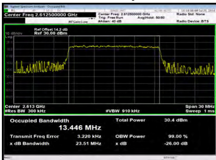
Band38 15MHz_QPSK 75 0_HighCH38175-2612.5
