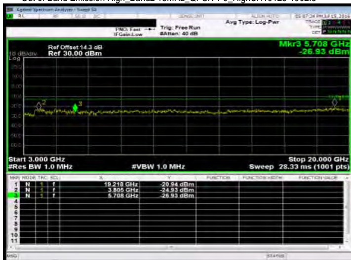
Out of Band Emission High_Band2 15MHz_QPSK 1 0_HighCH19125-1902.5
