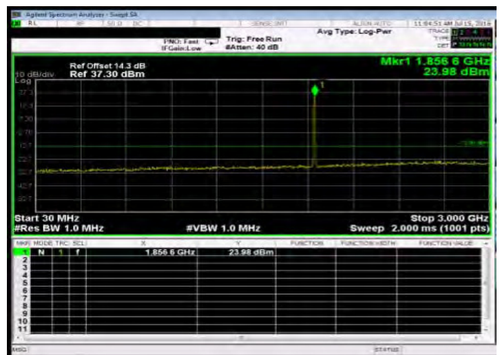
Out of Band Emission Low_WCDMA_B2_LowCH9262-1852.4
