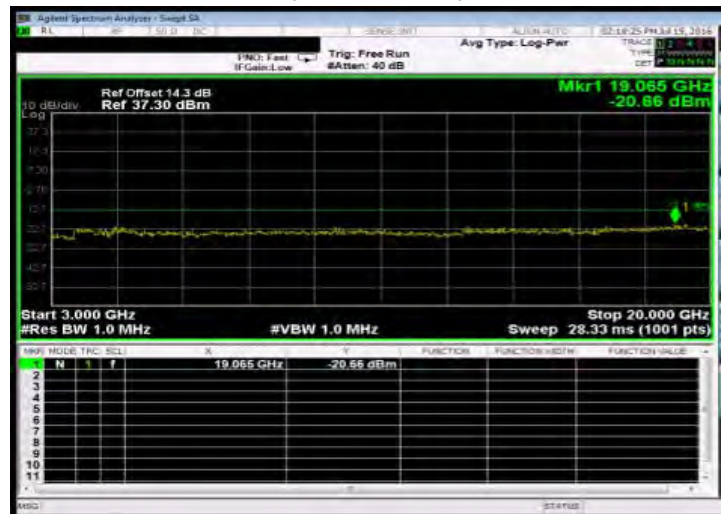
Out of Band Emission High_HSUPA_B2_HighCH9538-1907.6
