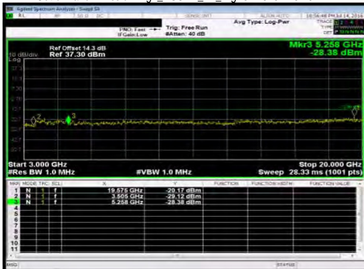
Out of Band Emission Low_WCDMA_B5_LowCH4132-826.4
