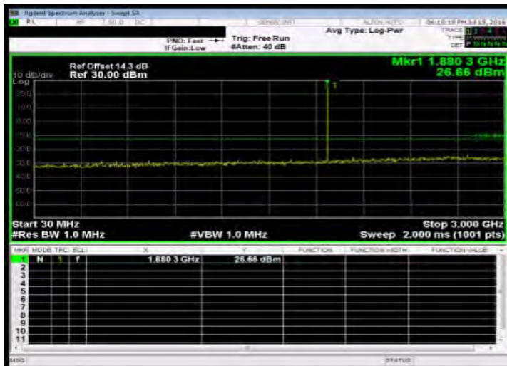
Out of Band Emission Low_Band2 1.4MHz_QPSK 1 0_MidCH18900-1880
