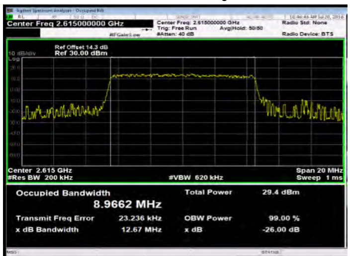
Band38 10MHz_16-QAM 50 0_HighCH38200-2615
