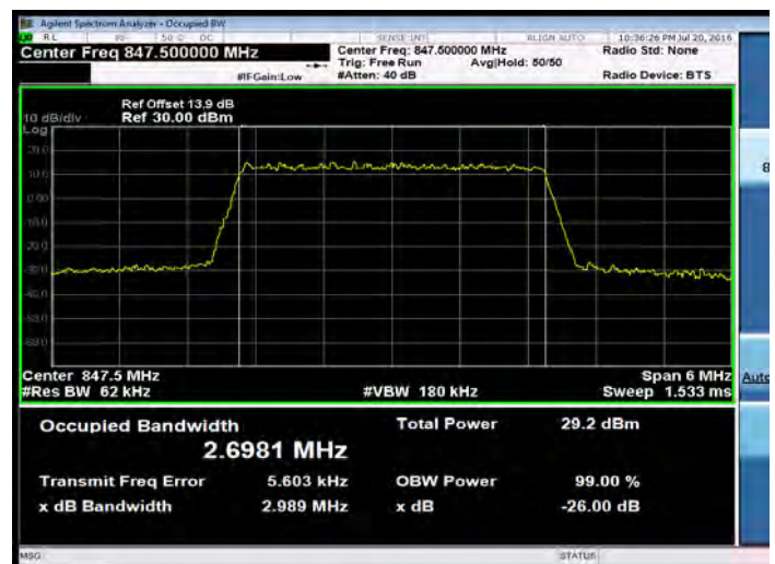
LTE Band 26 for Part 90S_3M_16QAM_HIGH
