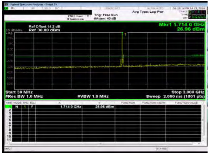
Out of Band Emission Low_Band4 20MHz_QPSK 1 0_MidCH20175-1732.5
