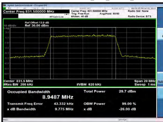
LTE Band 26 for Part 90S_10M_16QAM_MID
