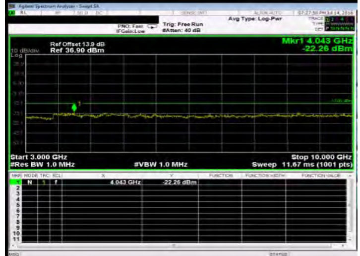
Out of Band Emission High_GSM_850MHz_LowCH128-824.2
