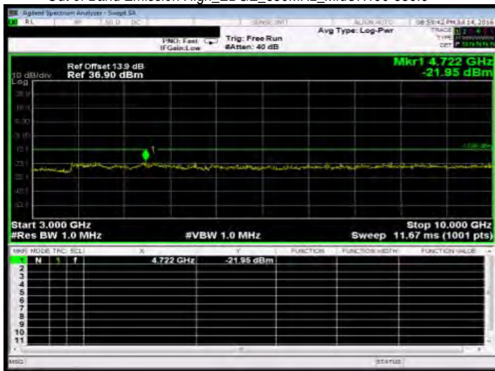
Out of Band Emission High_EDGE_850MHz_HighCH251-848.8
