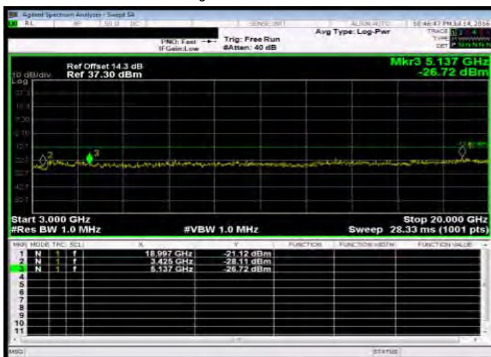
Out of Band Emission High_HSDPA_B4_LowCH1312-1712.4
