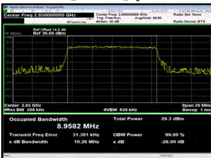
Band41 10MHz_16-QAM 50 0_HighCH41190-2650
