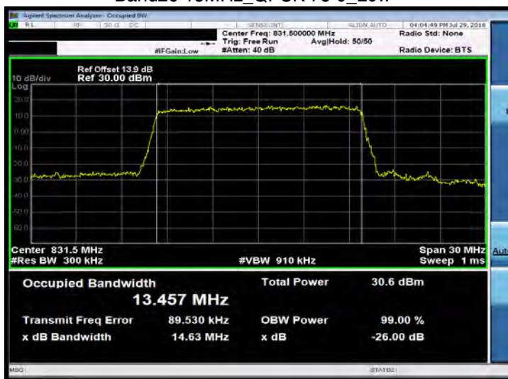
Band26 15MHz_QPSK 75 0_Mid
