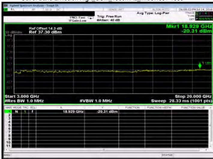
Out of Band Emission High_GSM_1900MHz_HighCH810-1909.8
