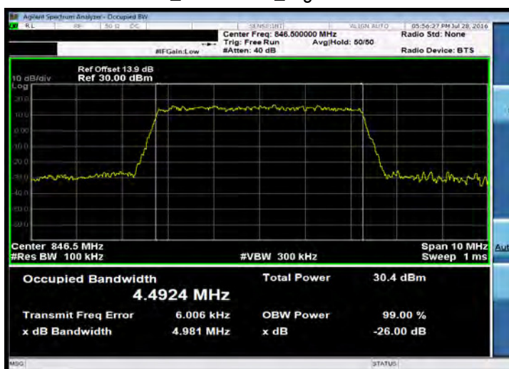
Band26 5MHz_QPSK 25 0_HighCH27015-846.5
