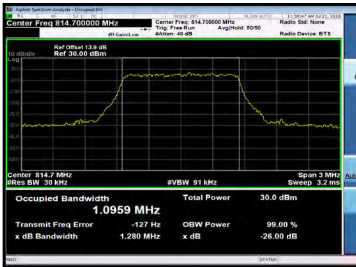
LTE Band 26 for Part 90S_1.4M_QPSK_MID
