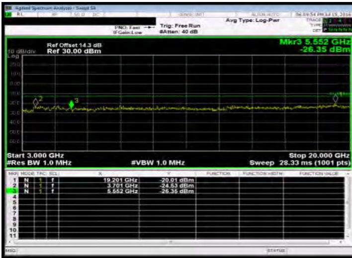
Out of Band Emission High_Band2 1.4MHz_QPSK 1 0_MidCH18900-1880
