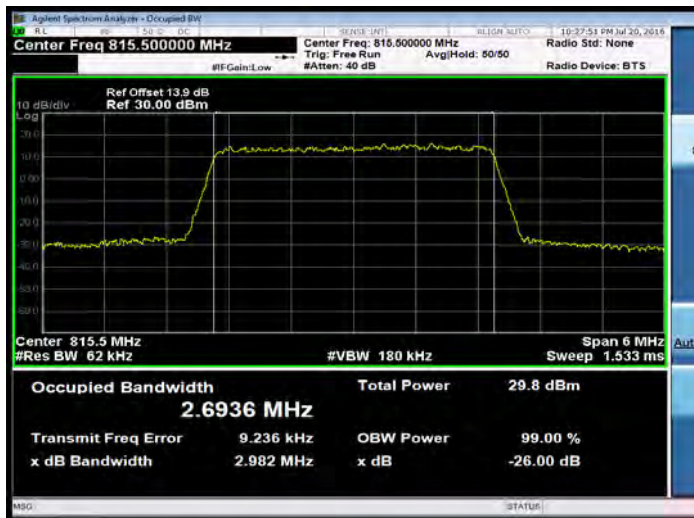
LTE Band 26 for Part 90S_3M_QPSK_MID
