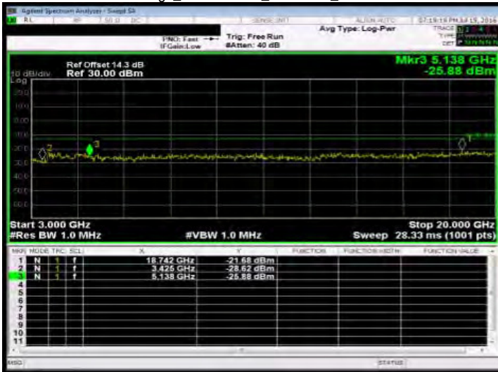
Out of Band Emission High_Band4 5MHz_QPSK 1 0_MidCH20175-1732.5
