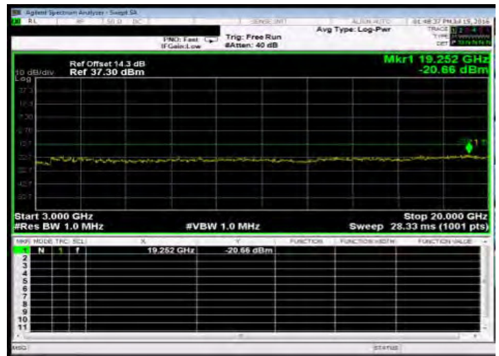
Out of Band Emission High_WCDMA_B2_HighCH9538-1907.6
