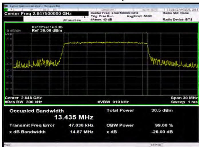
Band41 15MHz_QPSK 75 0_HighCH41165-2647.5
