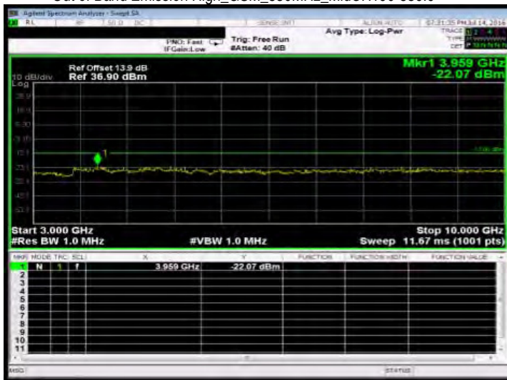
Out of Band Emission High_GSM_850MHz_HighCH251-848.8
