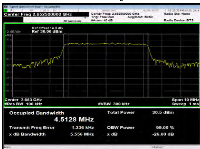
Band41 5MHz_QPSK 25 0_HighCH41215-2652.5
