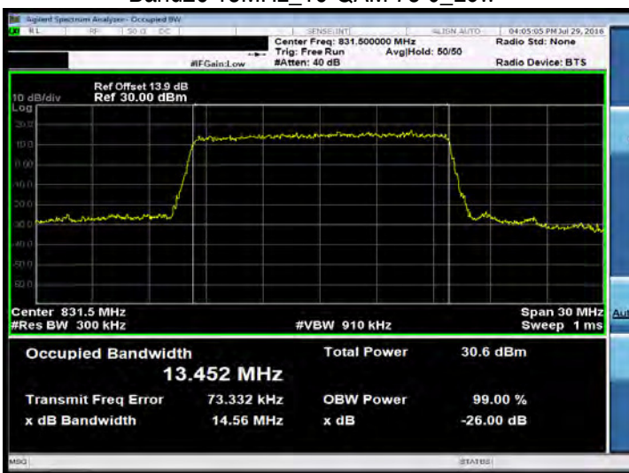
Band26 15MHz_16-QAM 75 0_Mid
