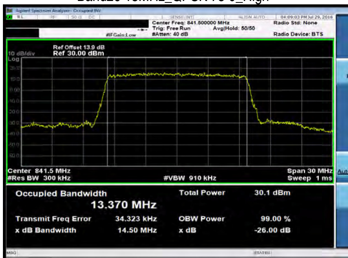
Band26 15MHz_QPSK 75 0_High
