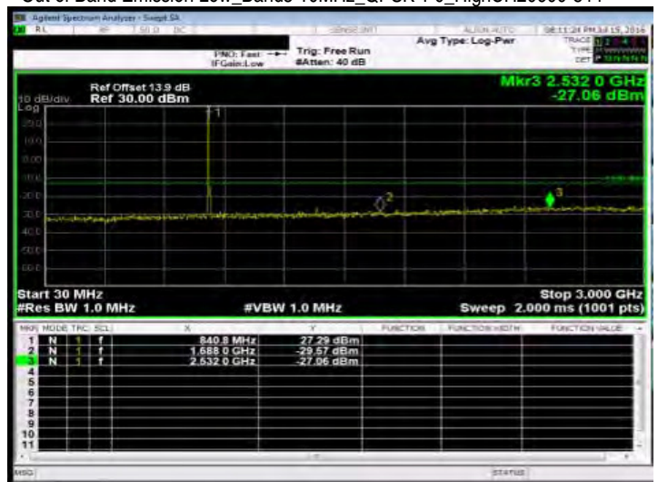
Out of Band Emission Low_Band5 10MHz_QPSK 1 0_HighCH20600-844
