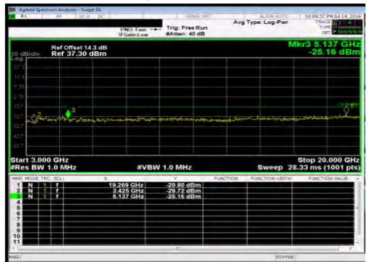
Out of Band Emission High_WCDMA_B4_LowCH1312-1712.4
