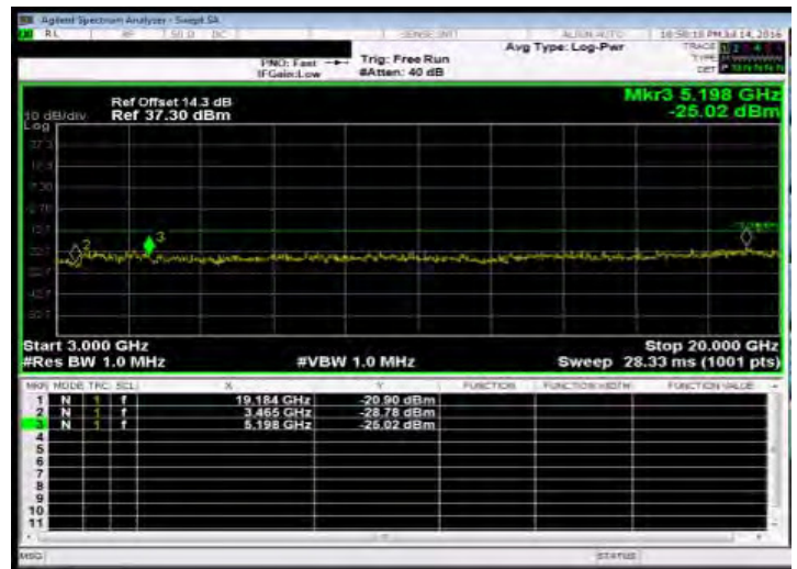
Out of Band Emission High_HSDPA_B4_HighCH1513-1752.6
