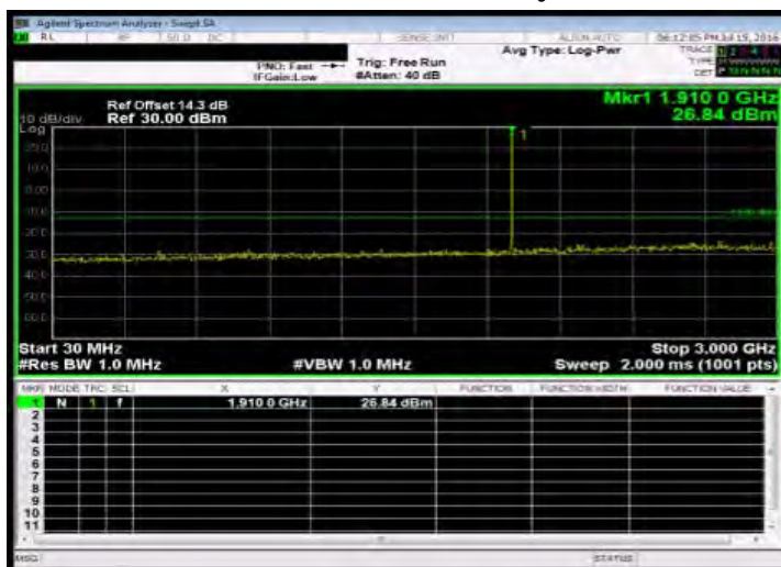
Out of Band Emission Low_Band2 1.4MHz_QPSK 1 0_HighCH19193-1909.3
