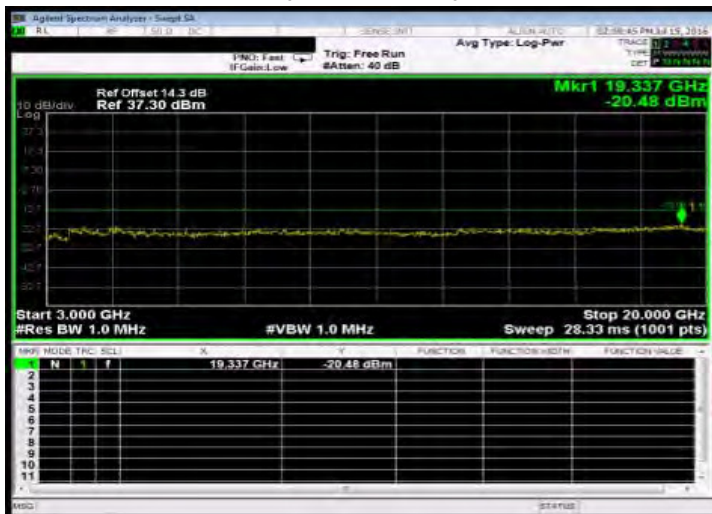
Out of Band Emission High_HSDPA_B2_HighCH9538-1907.6
