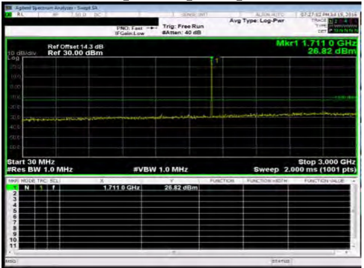
Out of Band Emission Low_Band4 3MHz_QPSK 1 0_MidCH20175-1732.5
