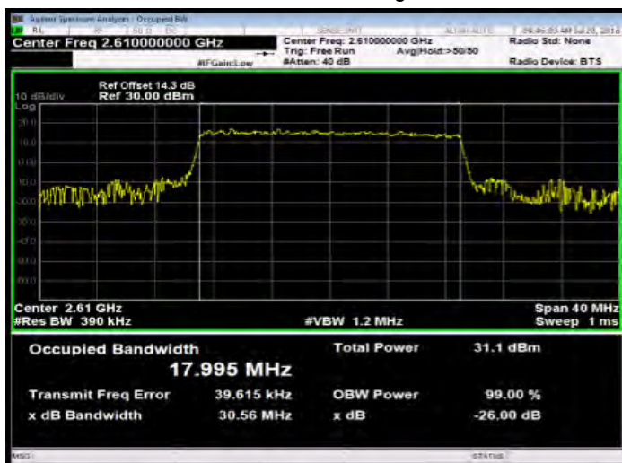
Band38 20MHz_QPSK 100 0_HighCH38150-2610
