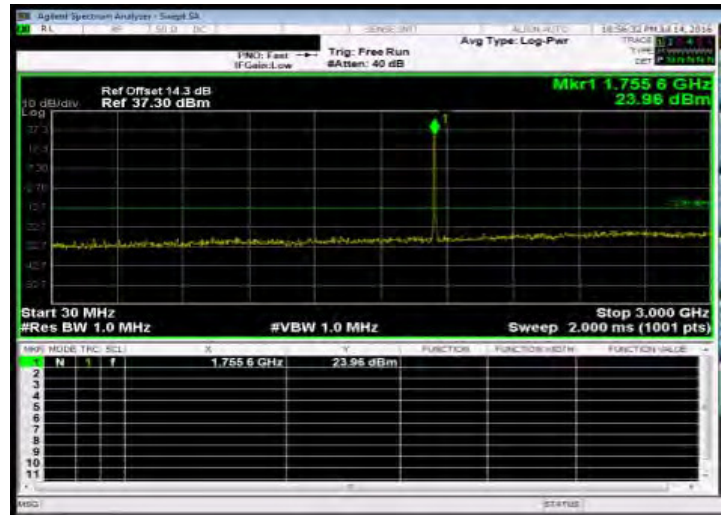
Out of Band Emission Low_HSUPA_B4_HighCH1513-1752.6
