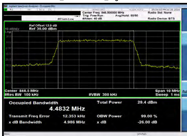
Band26 5MHz_16-QAM 25 0_HighCH27015-846.5
