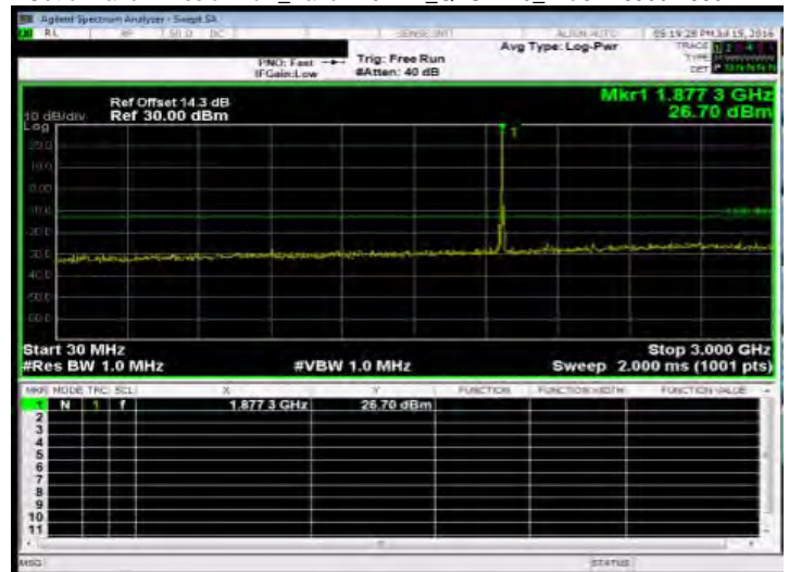
Out of Band Emission Low_Band2 10MHz_QPSK 1 0_HighCH19150-1905
