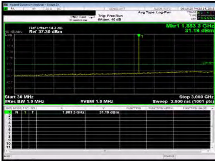
Out of Band Emission Low_GPRS_1900MHz_HighCH810-1909.8
