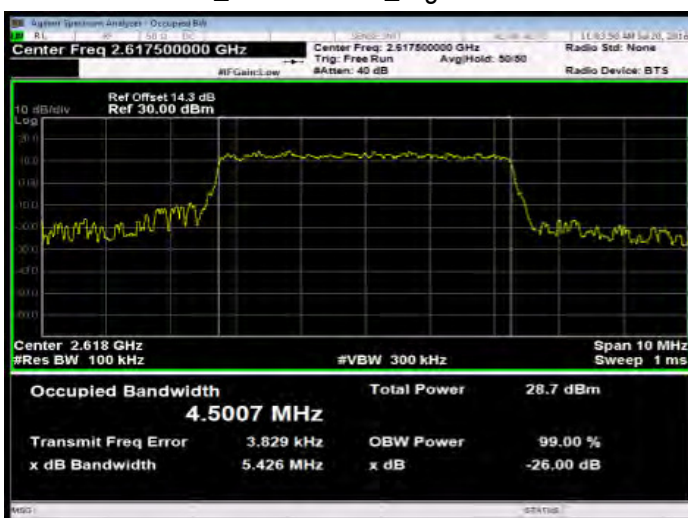
Band38 5MHz_16-QAM 25 0_HighCH38225-2617.5
