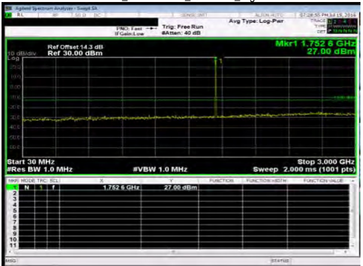
Out of Band Emission Low_Band4 3MHz_QPSK 1 0_HighCH20385-1753.5
