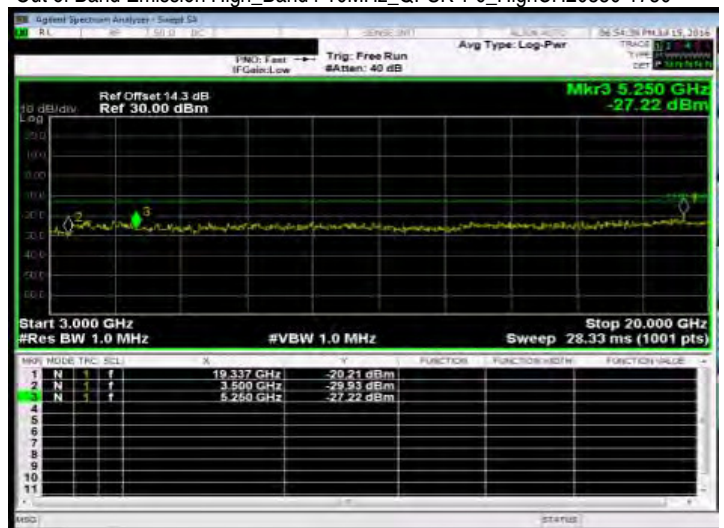
Out of Band Emission High_Band4 10MHz_QPSK 1 0_HighCH20350-1750
