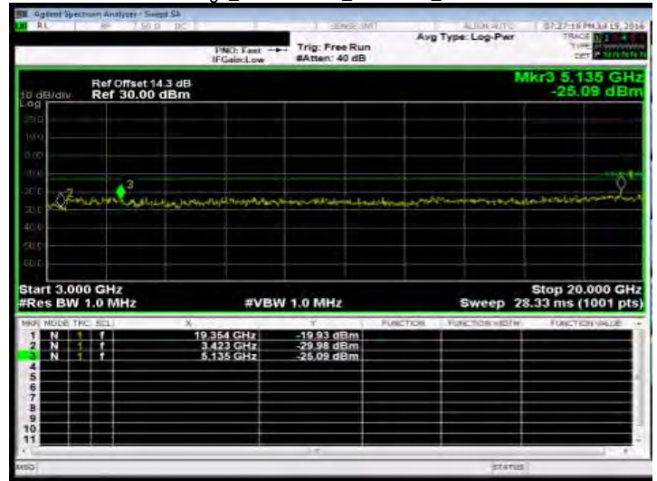
Out of Band Emission High_Band4 3MHz_QPSK 1 0_MidCH20175-1732.5
