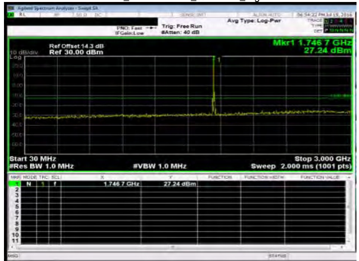
Out of Band Emission Low_Band4 10MHz_QPSK 1 0_HighCH20350-1750
