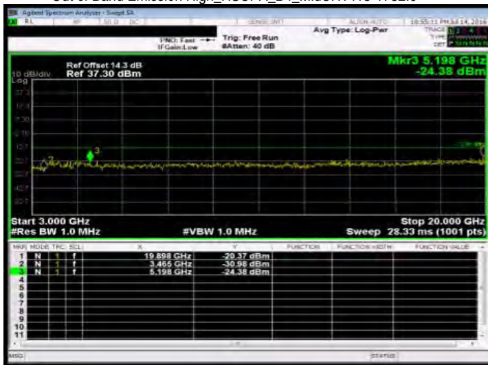
Out of Band Emission High_HSUPA_B4_HighCH1513-1752.6
