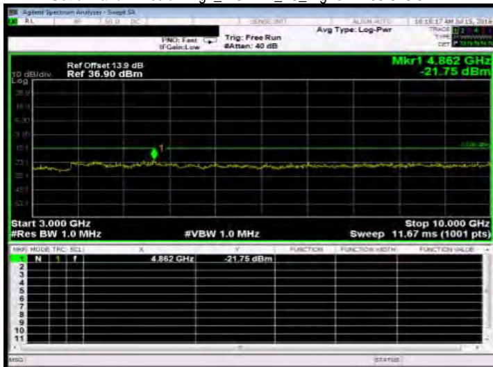
Out of Band Emission High_HSDPA_B5_LowCH4132-826.4
