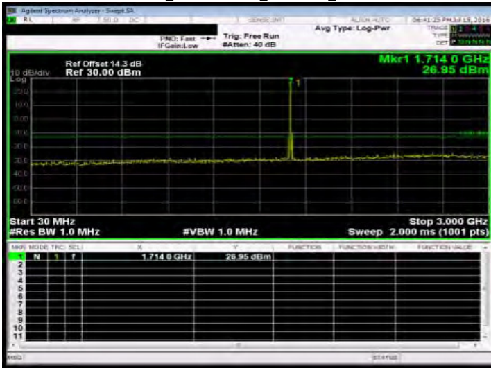
Out of Band Emission Low_Band4 15MHz_QPSK 1 0_MidCH20175-1732.5
