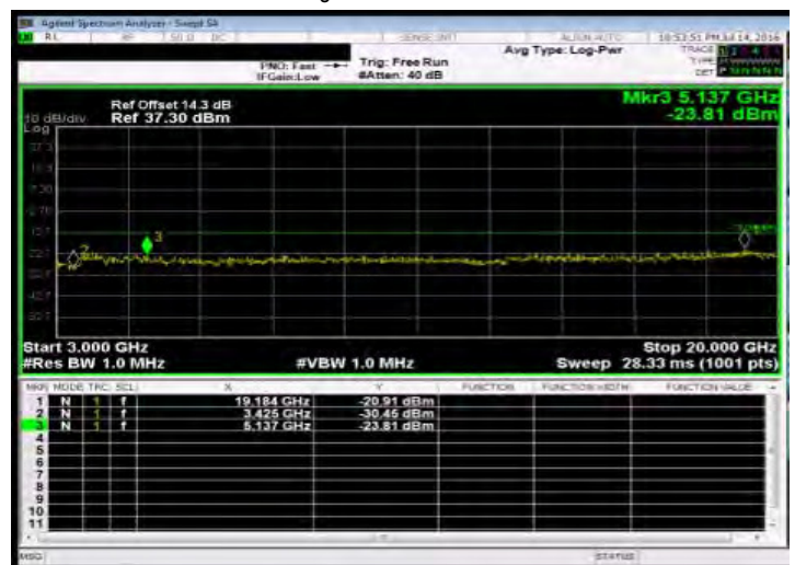
Out of Band Emission High_HSUPA_B4_LowCH1312-1712.4
