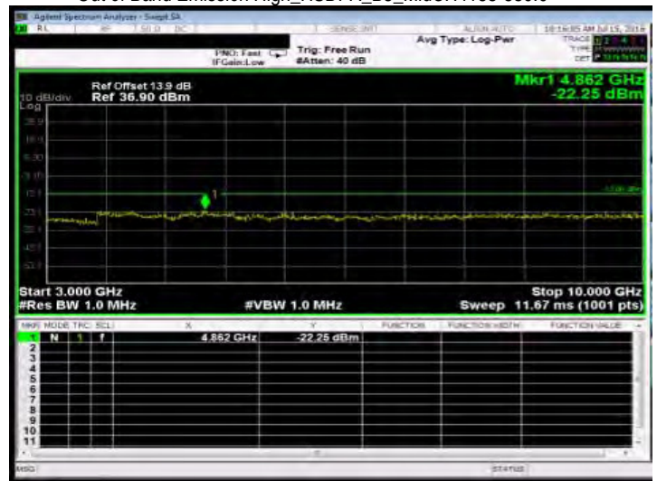
Out of Band Emission High_HSDPA_B5_HighCH4233-846.6
