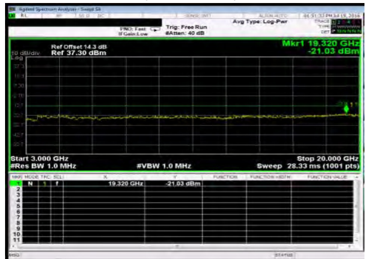
Out of Band Emission High_WCDMA_B2_HighCH9538-1907.6
