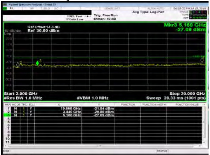
Out of Band Emission High_Band4 20MHz_QPSK 1 0_MidCH20175-1732.5
