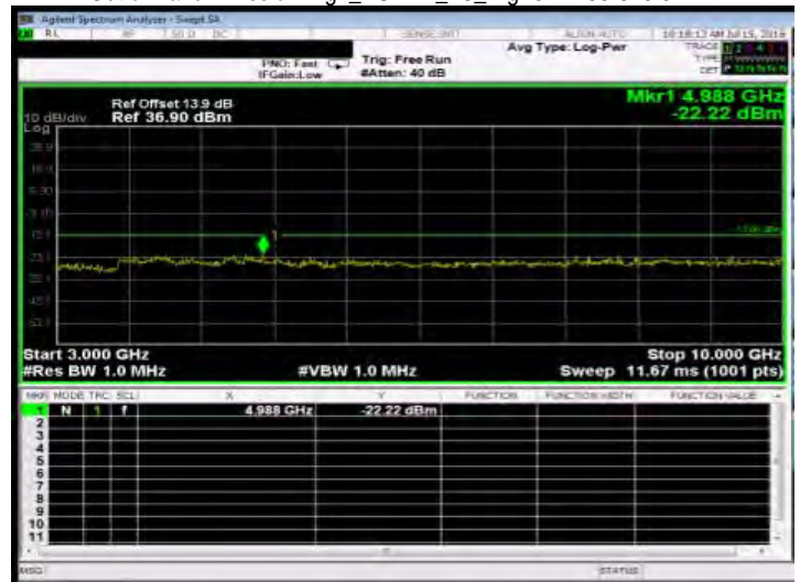
Out of Band Emission High_HSUPA_B5_LowCH4132-826.4
