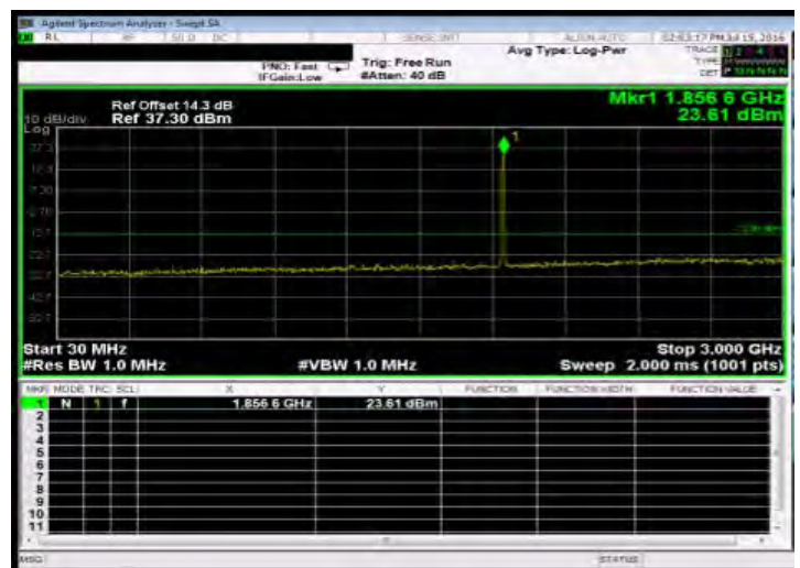
Out of Band Emission Low_HSUPA_B2_LowCH9262-1852.4
