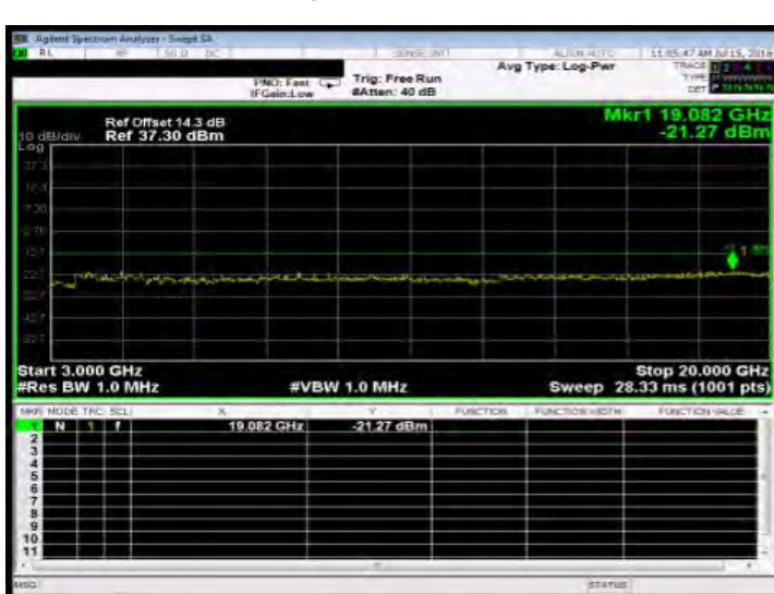
Out of Band Emission High_WCDMA_B2_LowCH9262-1852.4
