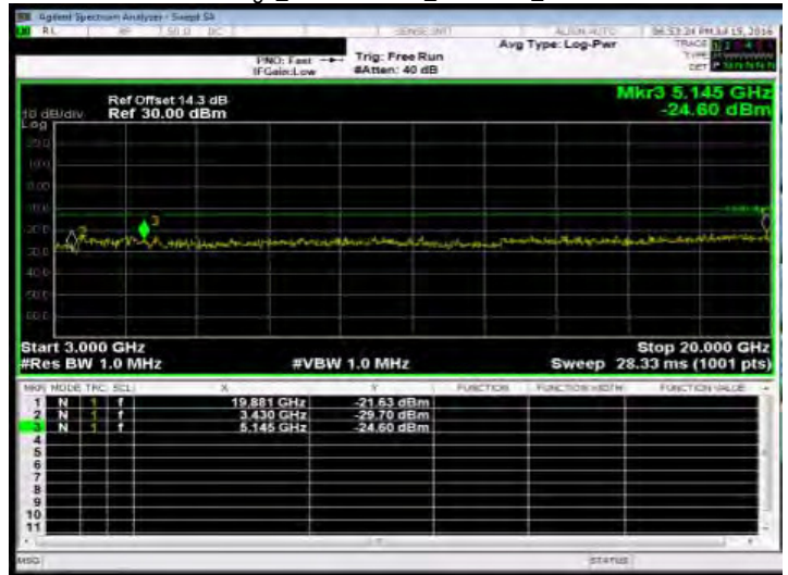
Out of Band Emission High_Band4 10MHz_QPSK 1 0_MidCH20175-1732.5
