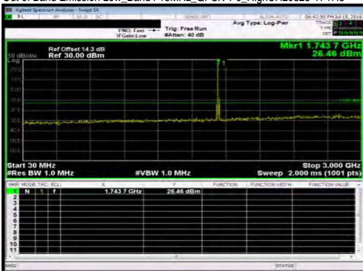
Out of Band Emission Low_Band4 15MHz_QPSK 1 0_HighCH20325-1747.5
