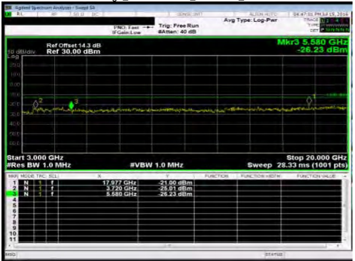
Out of Band Emission High_Band2 20MHz_QPSK 1 0_MidCH18900-1880
