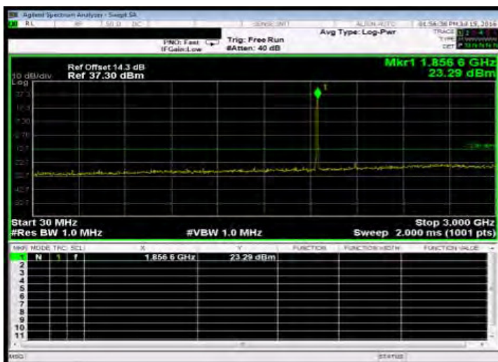
Out of Band Emission Low_HSDPA_B2_LowCH9262-1852.4
