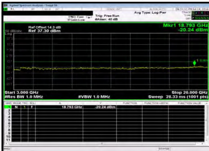
Out of Band Emission High_EDGE_1900MHz_HighCH810-1909.8
