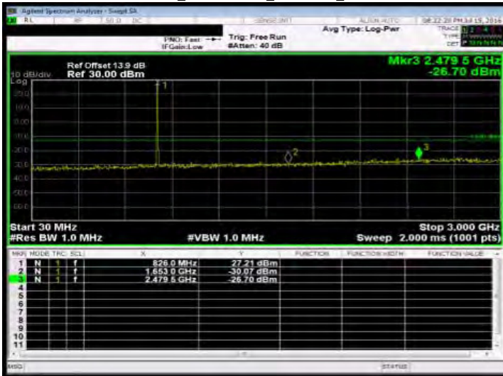
Out of Band Emission Low_Band5 5MHz_QPSK 1 0_MidCH20525-836.5
