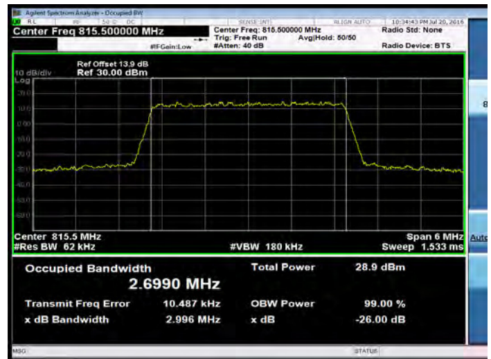
LTE Band 26 for Part 90S_3M_16QAM_MID
