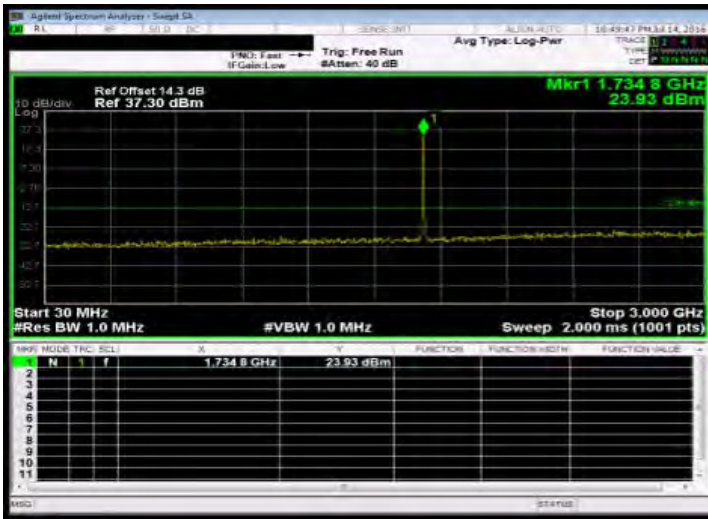
Out of Band Emission Low_HSDPA_B4_HighCH1513-1752.6
