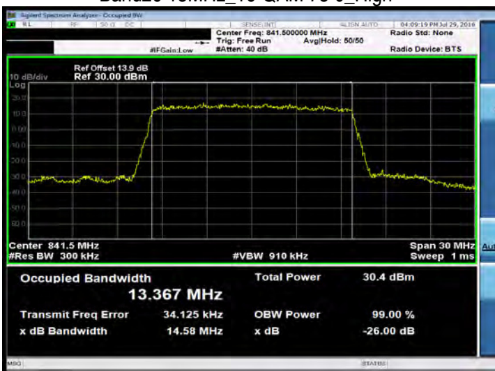
Band26 15MHz_16-QAM 75 0_High
