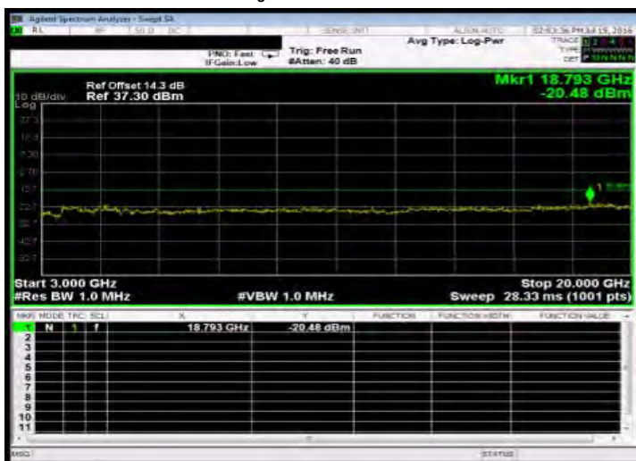
Out of Band Emission High_HSUPA_B2_LowCH9262-1852.4
