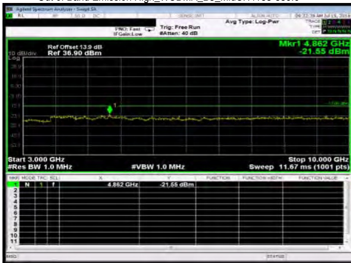
Out of Band Emission High_WCDMA_B5_HighCH4233-846.6
