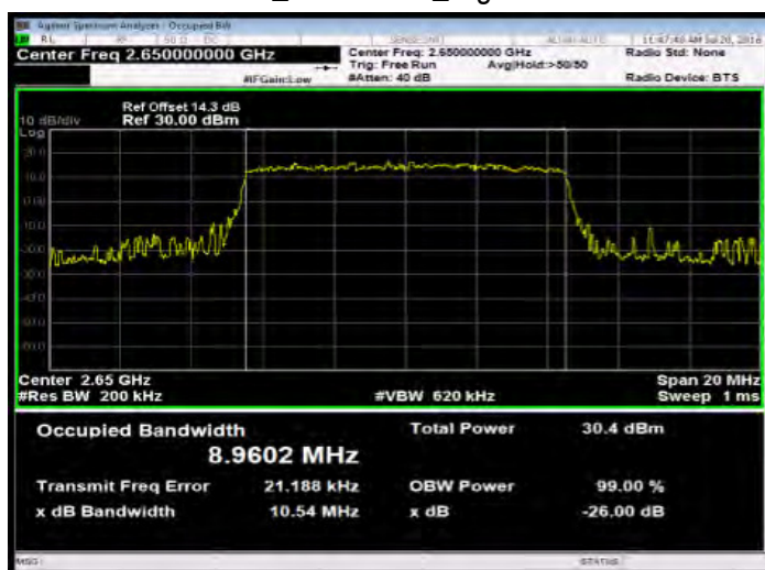
Band41 10MHz_QPSK 50 0_HighCH41190-2650
