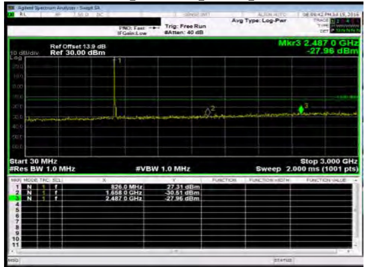
Out of Band Emission Low_Band5 10MHz_QPSK 1 0_MidCH20525-836.5
