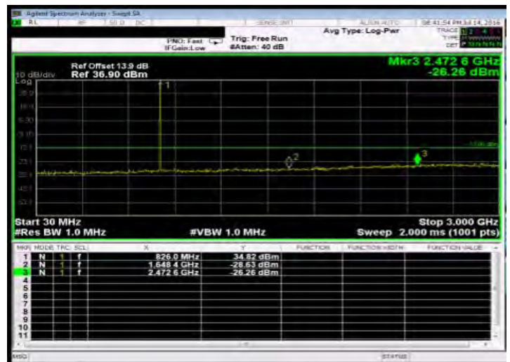
Out of Band Emission Low_GPRS_850MHz_LowCH128-824.2
