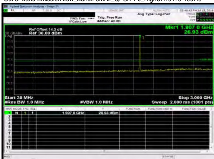
Out of Band Emission Low_Band2 5MHz_QPSK 1 0_HighCH19175-1907.5
