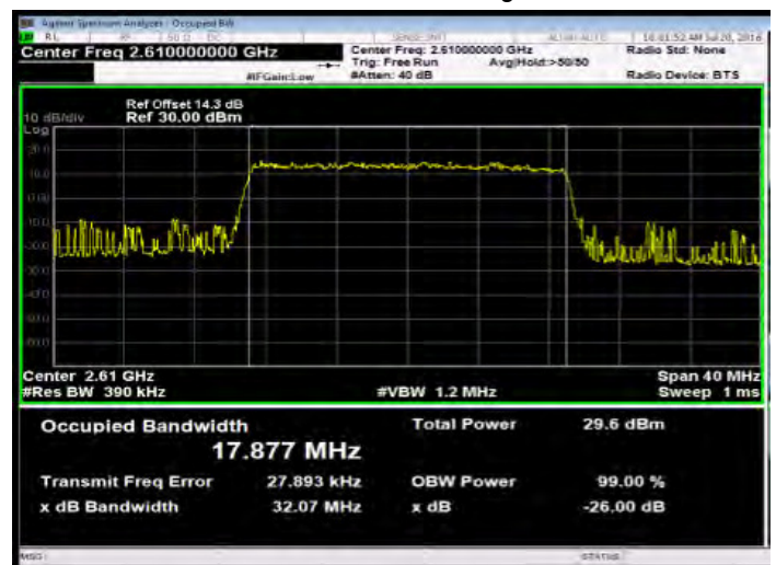
Band38 20MHz_16-QAM 100 0_HighCH38150-2610
