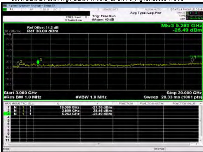
Out of Band Emission High_Band4 1.4MHz_QPSK 1 0_HighCH20393-1754.3
