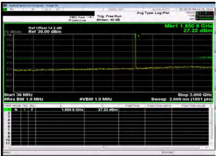
Out of Band Emission Low_Band2 3MHz_QPSK 1 0_LowCH18615-1851.5
