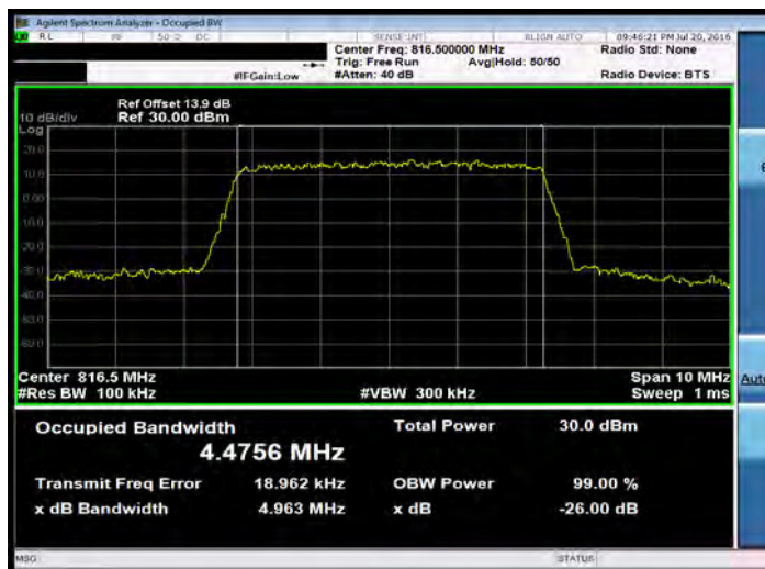
LTE Band 26 for Part 90S_5M_QPSK_MID
