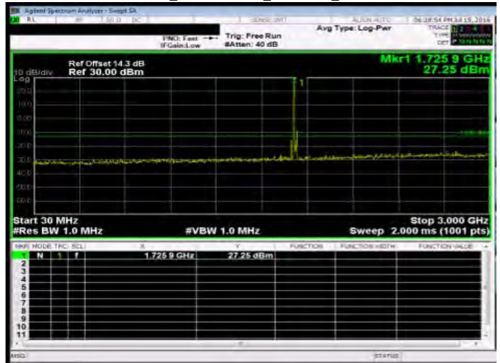
Out of Band Emission Low_Band4 20MHz_QPSK 1 0_HighCH20300-1745
