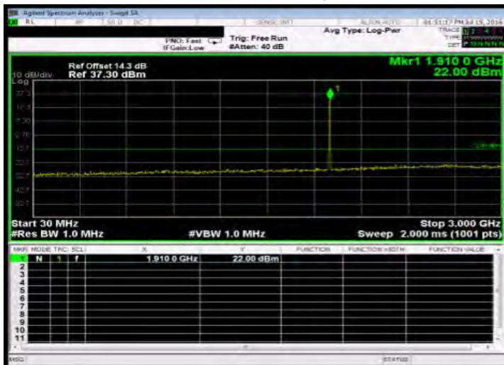
Out of Band Emission Low_WCDMA_B2_HighCH9538-1907.6
