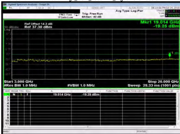
Out of Band Emission High_GPRS_1900MHz_LowCH512-1850.2
