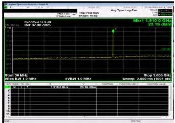
Out of Band Emission Low_HSDPA_B2_HighCH9538-1907.6
