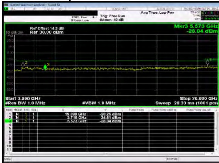
Out of Band Emission High_Band2 15MHz_QPSK 1 0_MidCH18900-1880
