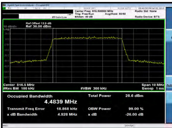
LTE Band 26 for Part 90S_5M_16QAM_MID
