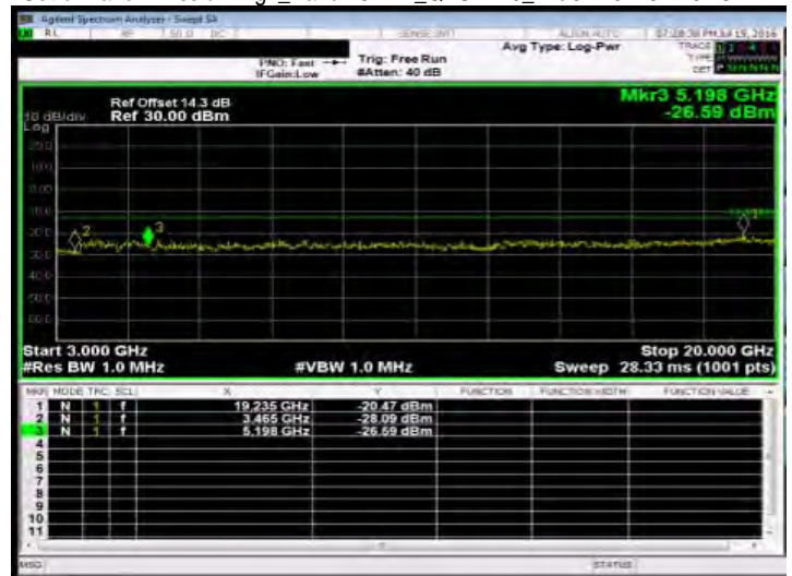
Out of Band Emission High_Band4 3MHz_QPSK 1 0_HighCH20385-1753.5
