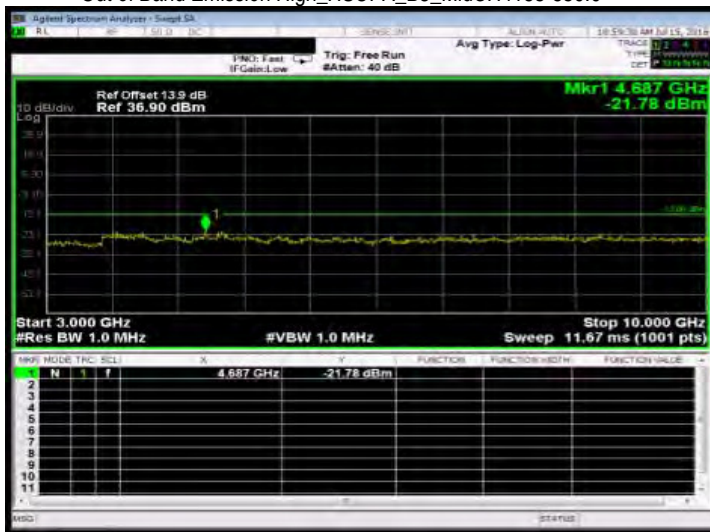
Out of Band Emission High_HSUPA_B5_HighCH4233-846.6
