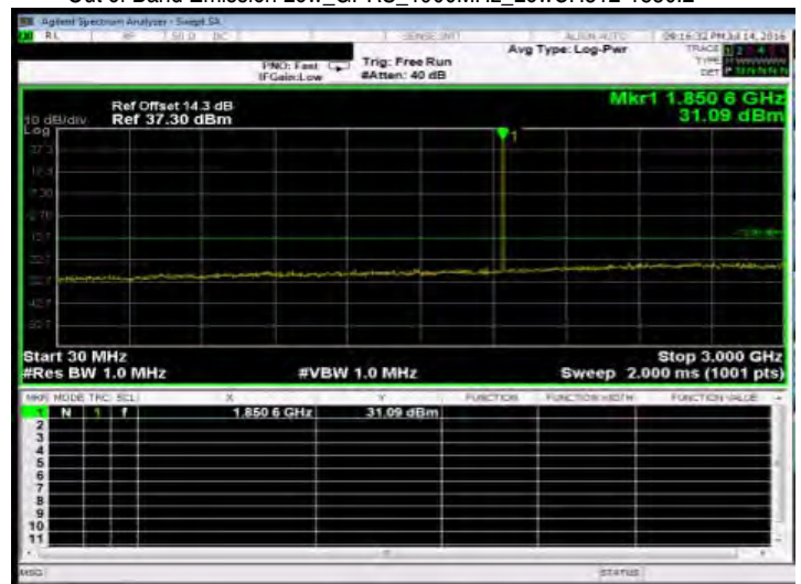
Out of Band Emission Low_GPRS_1900MHz_LowCH512-1850.2
