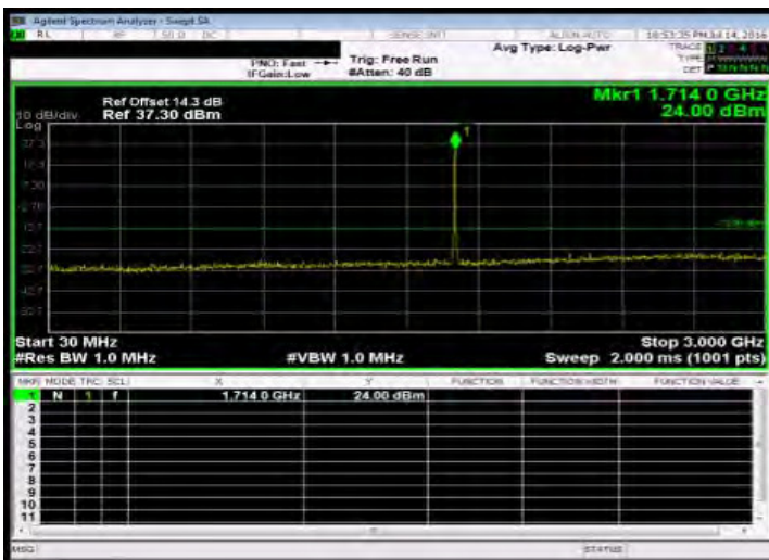
Out of Band Emission Low_HSUPA_B4_LowCH1312-1712.4
