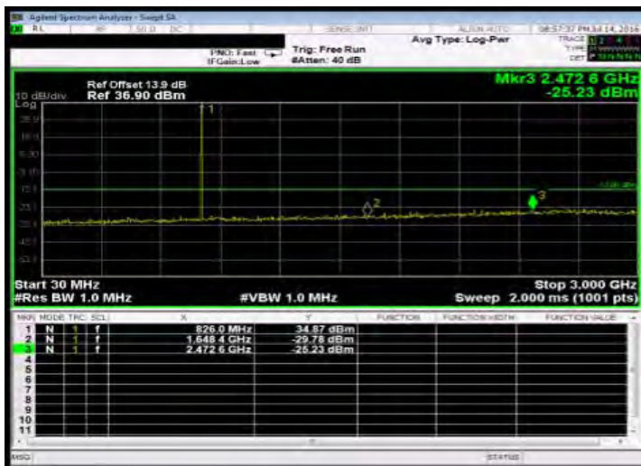
Out of Band Emission Low_EDGE_850MHz_LowCH128-824.2
