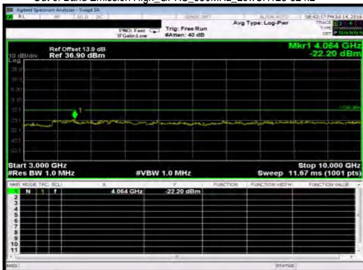
Out of Band Emission High_GPRS_850MHz_LowCH128-824.2
