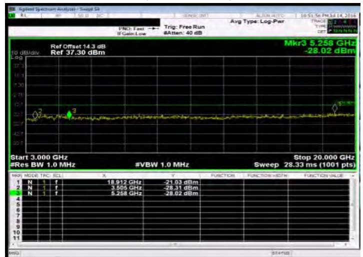
Out of Band Emission High_HSDPA_B4_HighCH1513-1752.6
