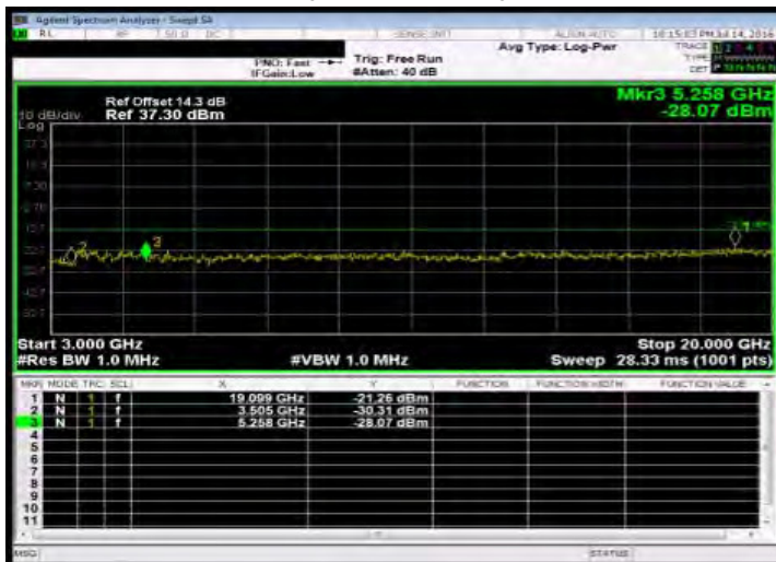
Out of Band Emission High_WCDMA_B4_HighCH1513-1752.6
