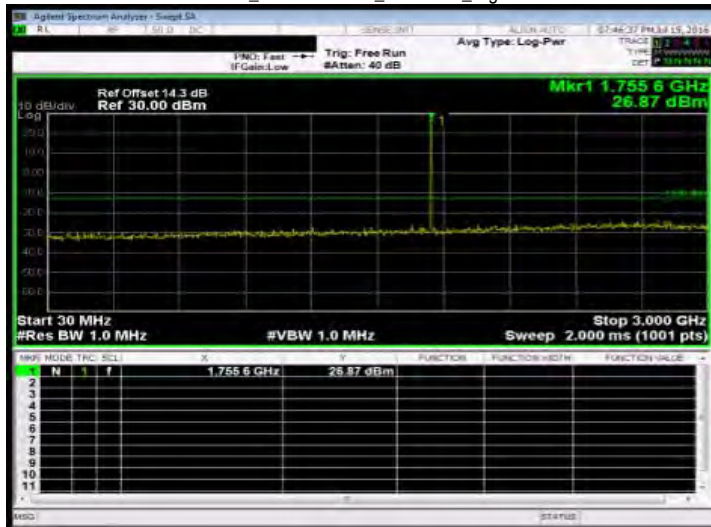
Out of Band Emission Low_Band4 1.4MHz_QPSK 1 0_HighCH20393-1754.3
