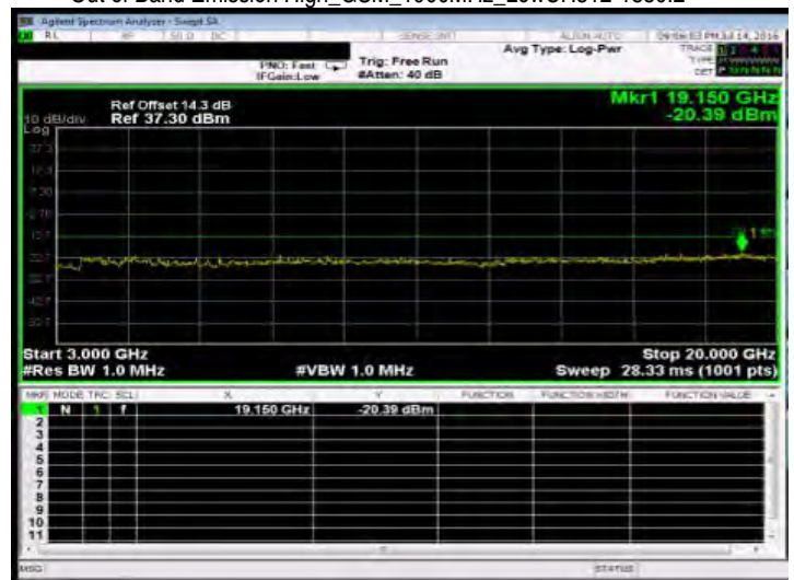
Out of Band Emission High_GSM_1900MHz_LowCH512-1850.2
