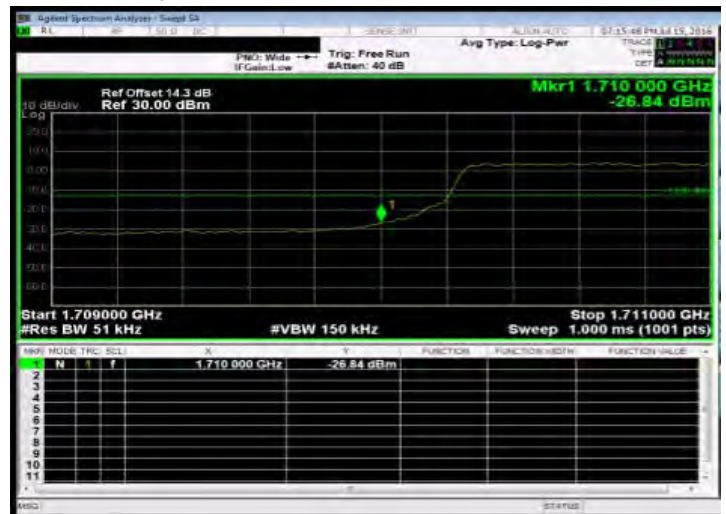
Band Edge_Band4 5MHz_QPSK 25 0_LowCH19975-1712.5
