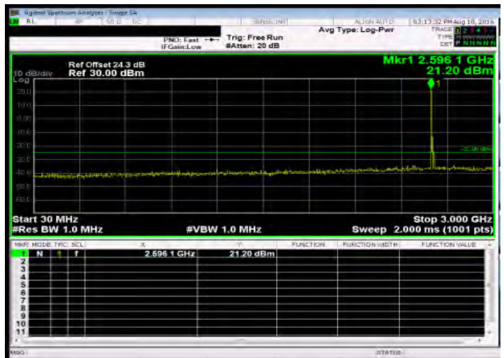
Out of Band Emission Low_Band41 10MHz_QPSK 1 0_MidCH40690-2600
