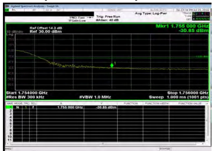
Band Edge_Band4 20MHz_QPSK 100 0_HighCH20300-1745
