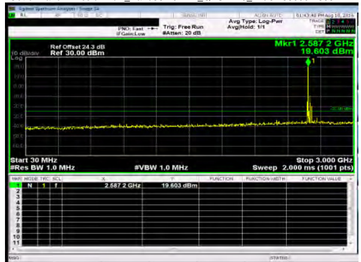
Out of Band Emission Low_Band38 20MHz_QPSK 1 0_HighCH38150-2610
