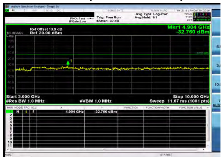
Out of Band Emission High_Band26 15MHz_QPSK 1 0_High
