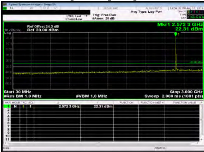
Out of Band Emission Low_Band38 15MHz_QPSK 1 0_MidCH38000-2595
