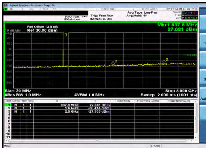
Out of Band Emission Low_Band26 1.4MHz_QPSK 1 0_MidCH26915-836.5
