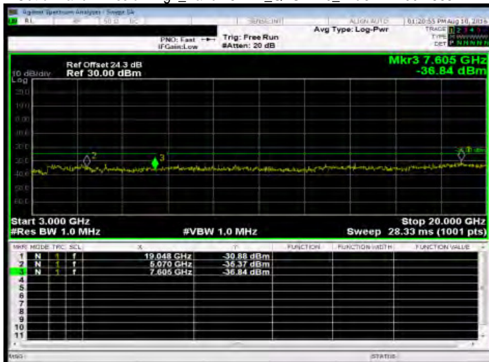
Out of Band Emission High_Band7 5MHz_QPSK 1 0_HighCH21425-2567.5
