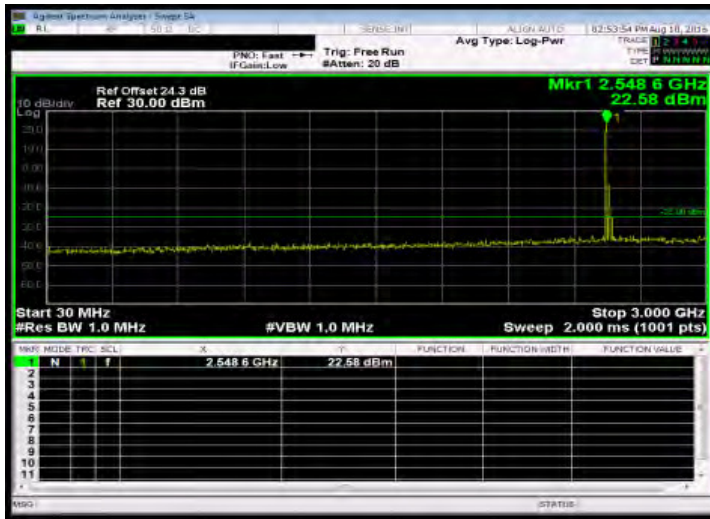
Out of Band Emission Low_Band41 15MHz_QPSK 1 0_MidCH40690-2600
