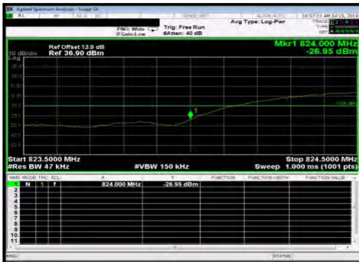
Band Edge_HSUPA_B5_LowCH4132-826.4
