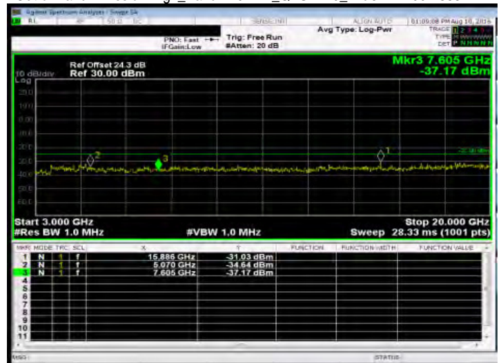
Out of Band Emission High_Band7 10MHz_QPSK 1 0_HighCH21400-2565
