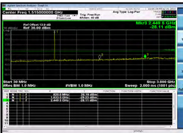
Out of Band Emission_Band26 for Part 90S_5M-QPSK-1 24-LOW-30M-3G
