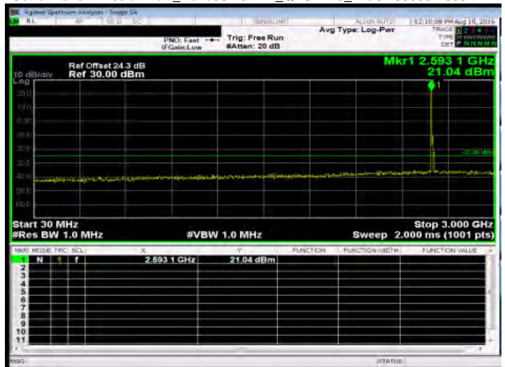
Out of Band Emission Low_Band38 10MHz_QPSK 1 0_HighCH38200-2615
