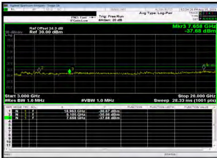
Out of Band Emission High_Band41 15MHz_QPSK 1 0_LowCH40215-2552.5
