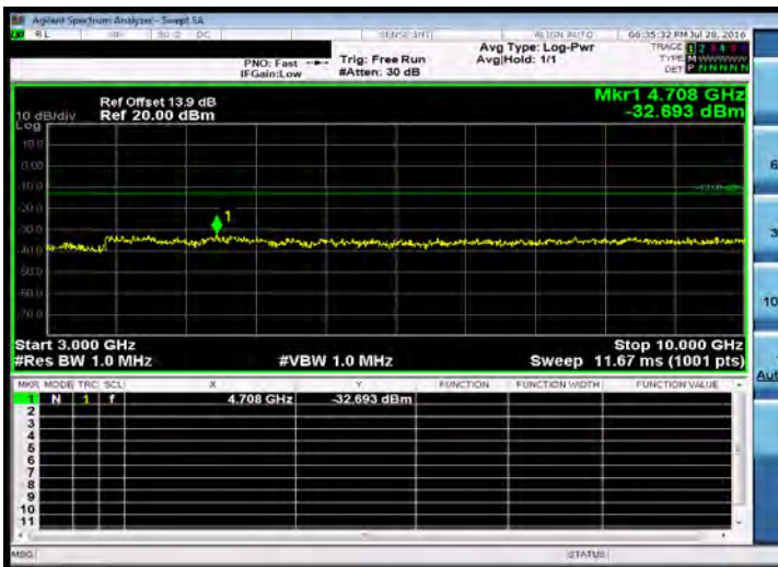
Out of Band Emission High_Band26 3MHz_QPSK 1 0_MidCH26915-836.5
