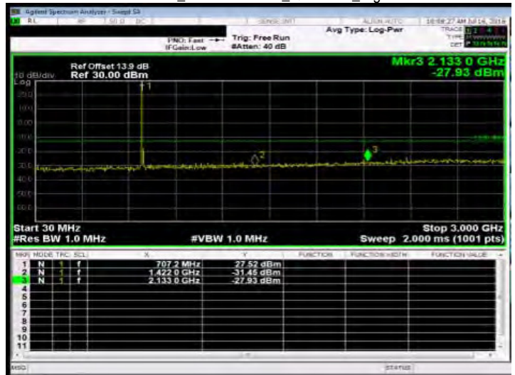
Out of Band Emission Low_Band17 10MHz_QPSK 1 0_HighCH23800-711
