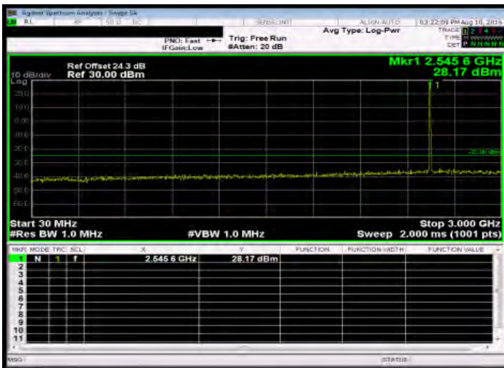
Out of Band Emission Low_Band41 5MHz_QPSK 1 0_LowCH40165-2547.5
