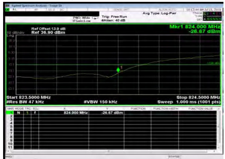
Band Edge_HSDPA_B5_LowCH4132-826.4
