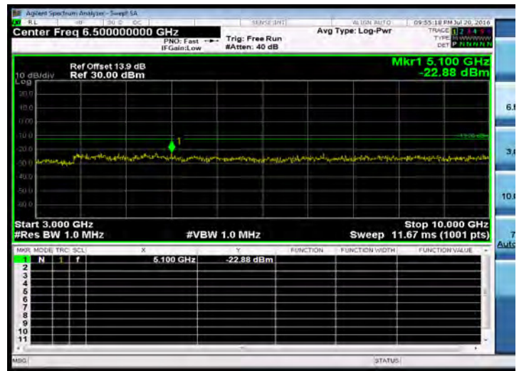
Out of Band Emission_Band26 for Part 90S_5M-QPSK-1 0-MID-30M-3G
