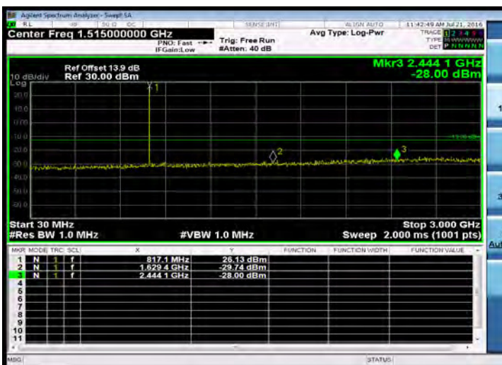
Out of Band Emission_Band26 for Part 90S_1.4M-QPSK-1 0-LOW-30M-3G
