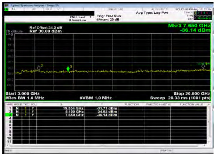
Out of Band Emission High_Band41 10MHz_QPSK 1 0_MidCH40690-2600
