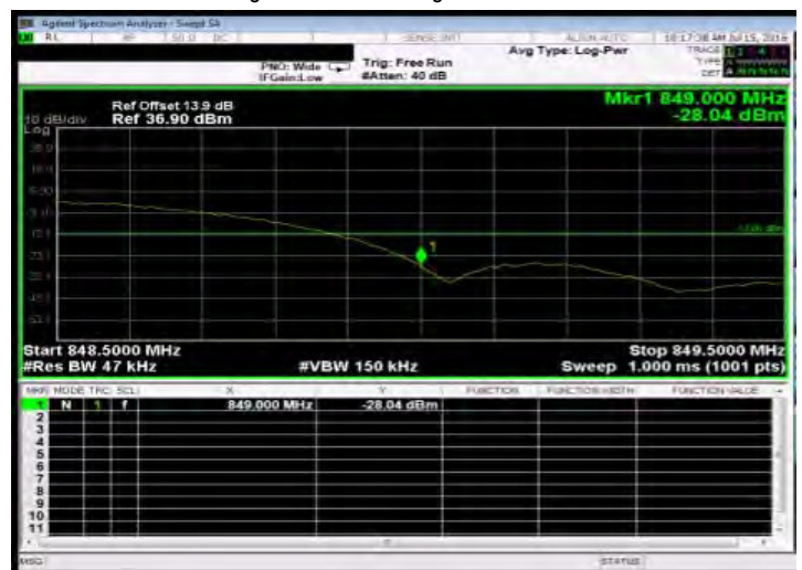
Band Edge_HSDPA_B5_HighCH4233-846.6
