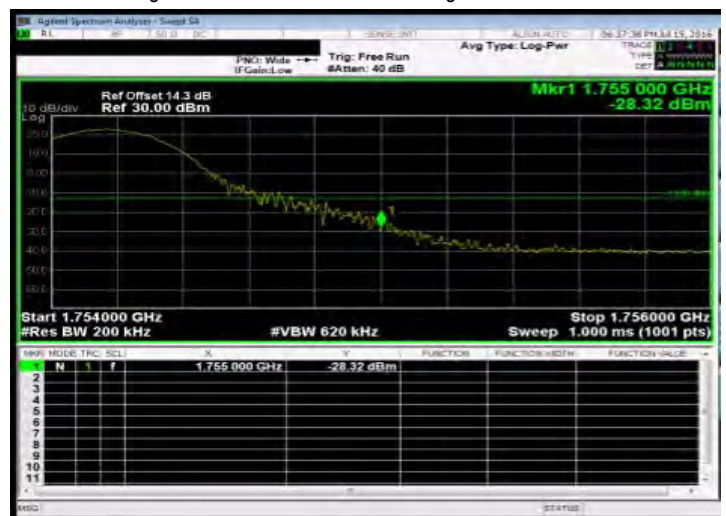
Band Edge_Band4 15MHz_QPSK 1 74_HighCH20325-1747.5
