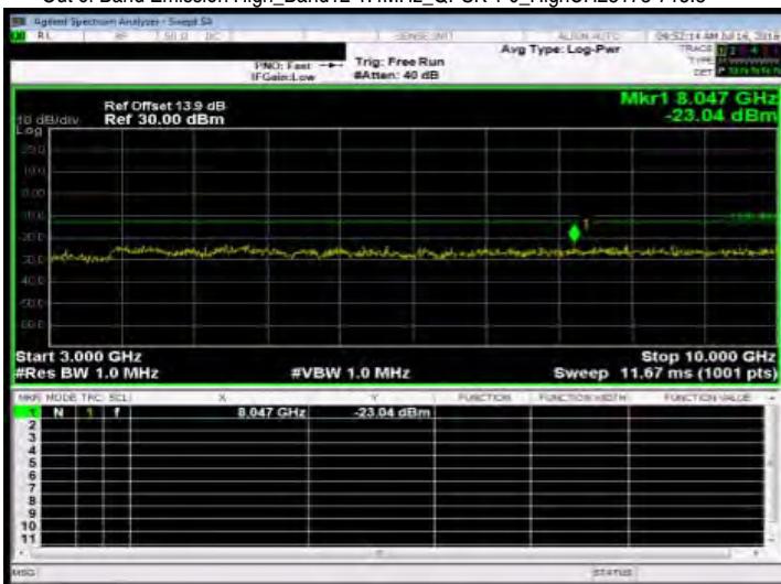
Out of Band Emission High_Band12 1.4MHz_QPSK 1 0_HighCH23173-715.3
