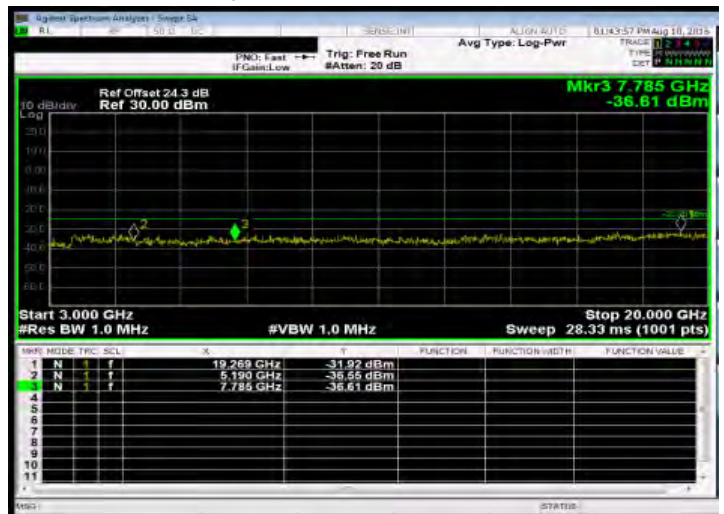
Out of Band Emission High_Band38 20MHz_QPSK 1 0_MidCH38000-2595
