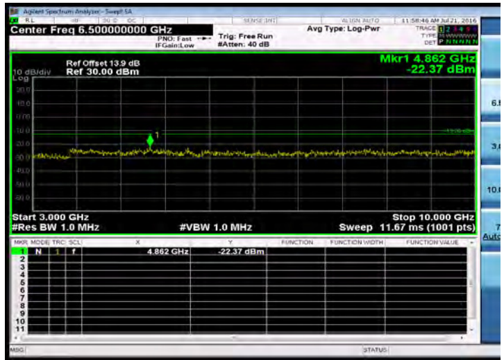
Out of Band Emission_Band26 for Part 90S_1.4M-QPSK-1 5-MID-30M-3G
