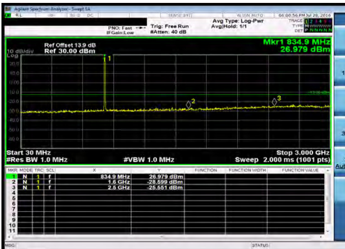
Out of Band Emission Low_Band26 5MHz_QPSK 1 0_MidCH26915-836.5
