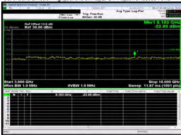
Out of Band Emission High_Band12 5MHz_QPSK 1 0_MidCH23095-707.5
