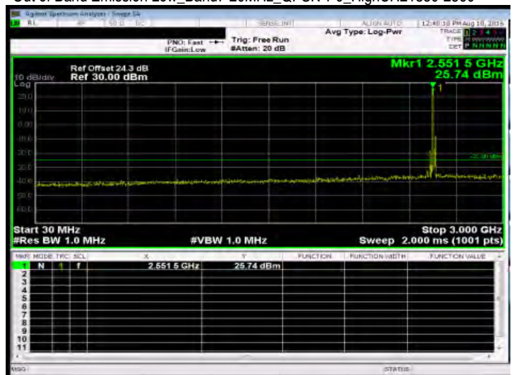
Out of Band Emission Low_Band7 20MHz_QPSK 1 0_HighCH21350-2560
