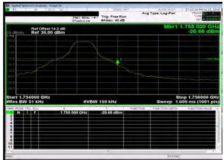
Band Edge_Band4 5MHz_QPSK 1 24_HighCH20375-1752.5
