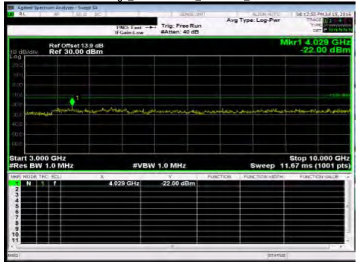
Out of Band Emission High_Band5 10MHz_QPSK 1 0_MidCH20525-836.5
