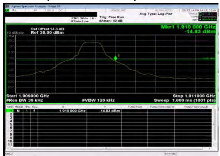
Band Edge_Band2 3MHz_QPSK 1 14_HighCH19185-1908.5
