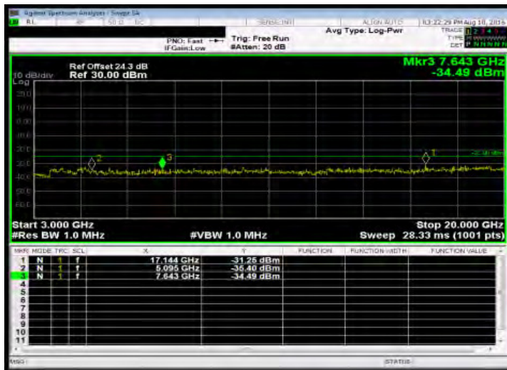
Out of Band Emission High_Band41 5MHz_QPSK 1 0_MidCH40690-2600
