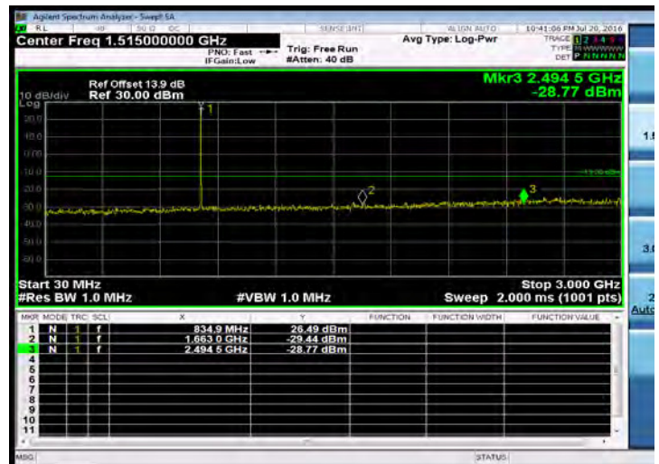
Out of Band Emission_Band26 for Part 90S_3M-QPSK-1 14-MID-30M-3G
