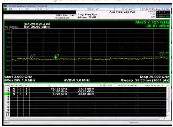
Out of Band Emission High_Band38 10MHz_QPSK 1 0_MidCH38000-2595
