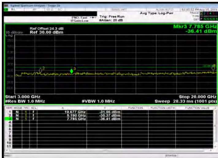
Out of Band Emission High_Band38 15MHz_QPSK 1 0_MidCH38000-2595
