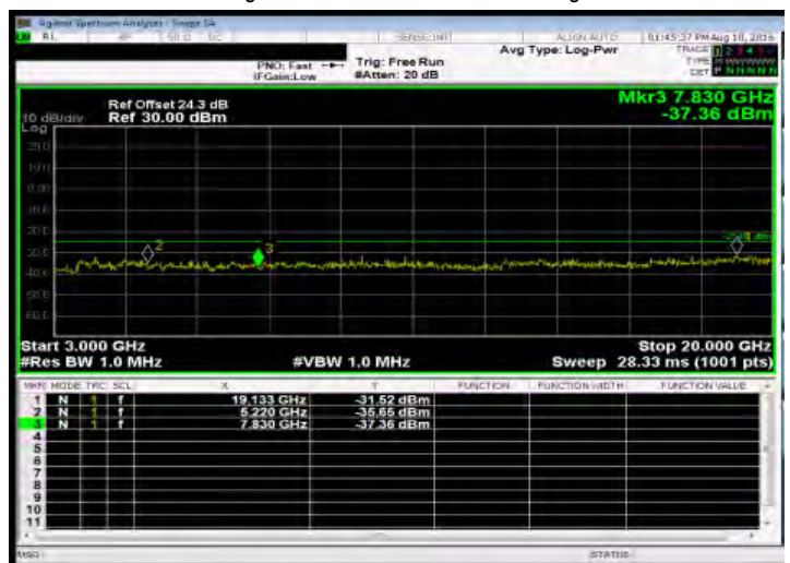
Out of Band Emission High_Band38 20MHz_QPSK 1 0_HighCH38150-2610
