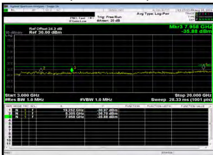
Out of Band Emission High_Band41 5MHz_QPSK 1 0_HighCH41215-2652.5
