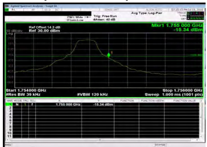
Band Edge_Band4 3MHz_QPSK 1 14_HighCH20385-1753.5
