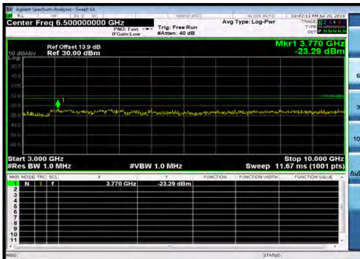
Out of Band Emission_Band26 for Part 90S_3M-QPSK-1 14-HIGH-3G-10G
