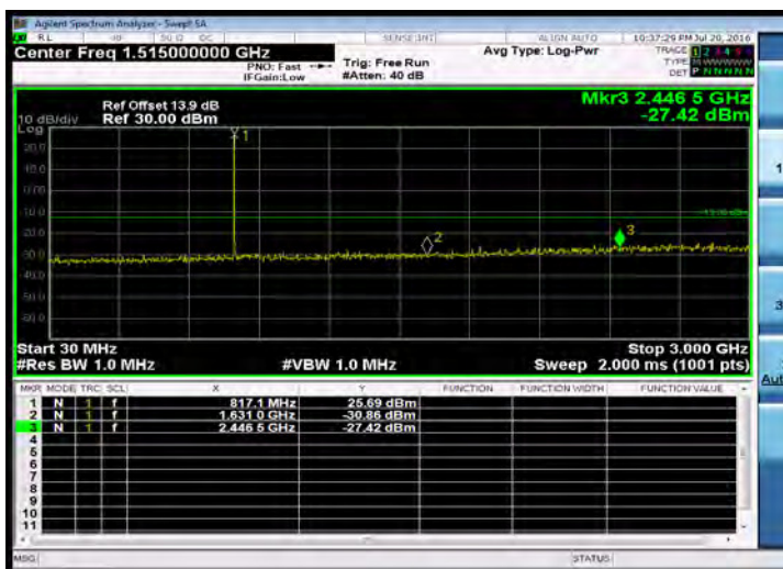
Out of Band Emission_Band26 for Part 90S_3M-QPSK-1 0-LOW-30M-3G
