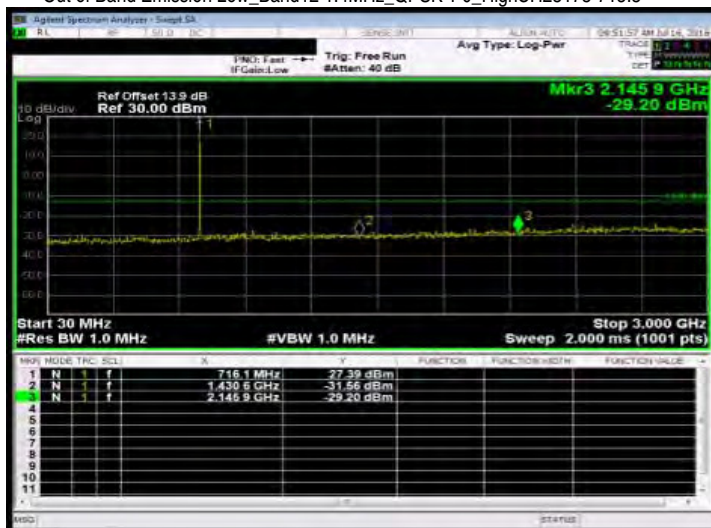
Out of Band Emission Low_Band12 1.4MHz_QPSK 1 0_HighCH23173-715.3
