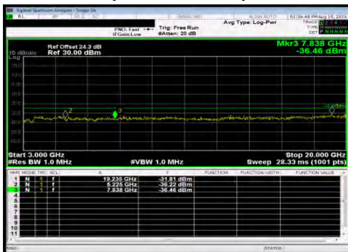
Out of Band Emission High_Band38 15MHz_QPSK 1 0_HighCH38175-2612.5
