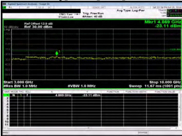
Out of Band Emission High_Band5 5MHz_QPSK 1 0_MidCH20525-836.5
