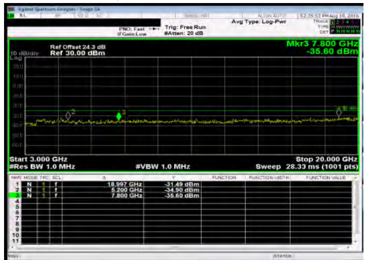
Out of Band Emission High_Band41 20MHz_QPSK 1 0_MidCH40690-2600
