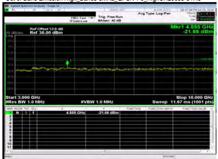
Out of Band Emission High_Band5 3MHz_QPSK 1 0_HighCH20635-847.5
