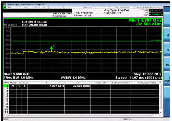
Out of Band Emission High_Band26 5MHz_QPSK 1 0_MidCH26915-836.5
