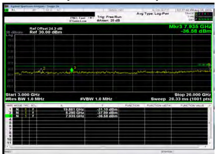
Out of Band Emission High_Band41 20MHz_QPSK 1 0_HighCH41140-2645
