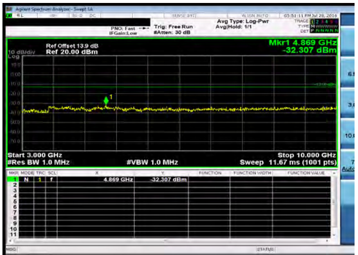
Out of Band Emission High_Band26 5MHz_QPSK 1 0_MidCH26915-836.5
