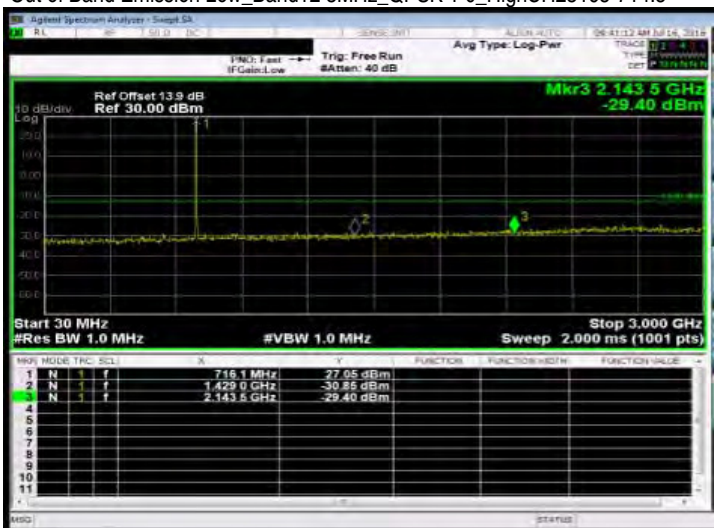
Out of Band Emission Low_Band12 3MHz_QPSK 1 0_HighCH23165-714.5
