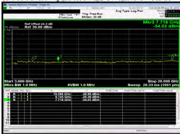
Out of Band Emission High_Band38 5MHz_QPSK 1 0_MidCH38000-2595
