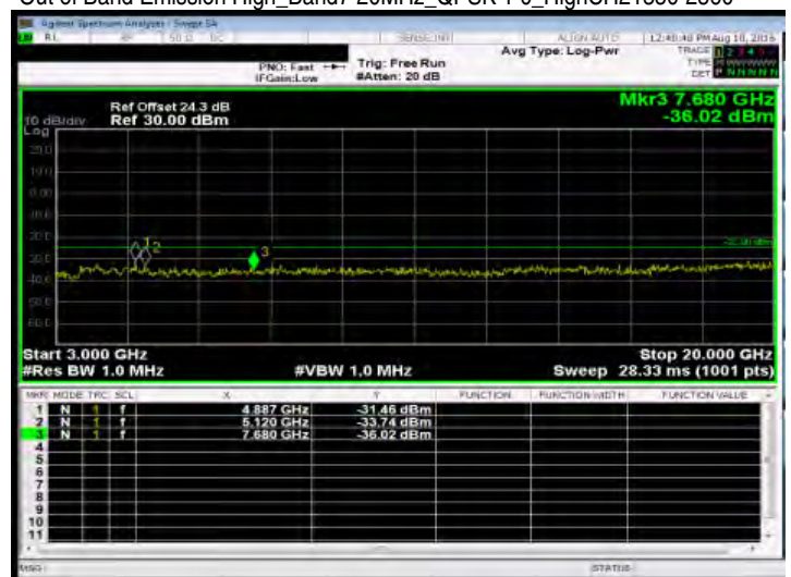
Out of Band Emission High_Band7 20MHz_QPSK 1 0_HighCH21350-2560
