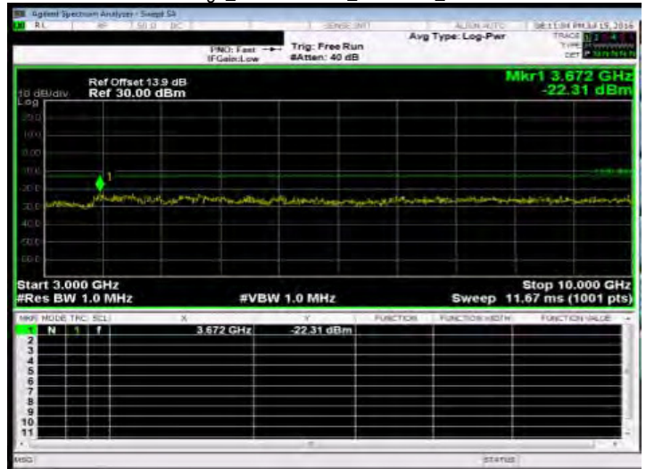
Out of Band Emission High_Band5 10MHz_QPSK 1 0_HighCH20600-844
