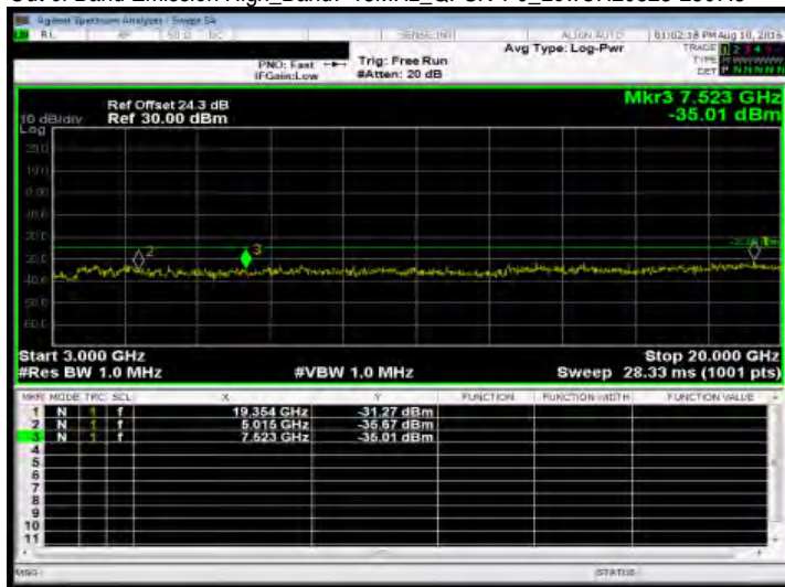
Out of Band Emission High_Band7 15MHz_QPSK 1 0_MidCH20175-1732.5
