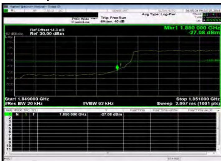
Band Edge_Band2 1.4MHz_QPSK 6 0_LowCH18607-1850.7
