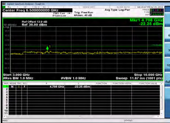
Out of Band Emission_Band26 for Part 90S_10M-QPSK-1 0-MID-3G-10G
