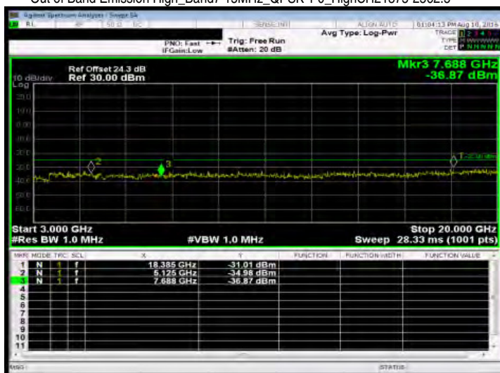
Out of Band Emission High_Band7 15MHz_QPSK 1 0_HighCH21375-2562.5
