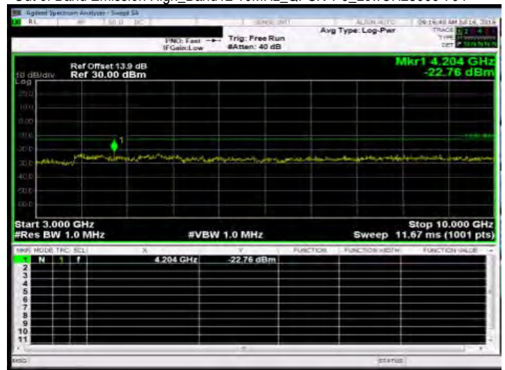
Out of Band Emission High_Band12 10MHz_QPSK 1 0_MidCH23095-707.5
