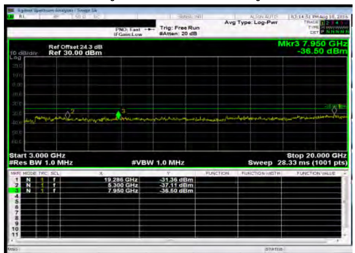
Out of Band Emission High_Band41 10MHz_QPSK 1 0_HighCH41190-2650
