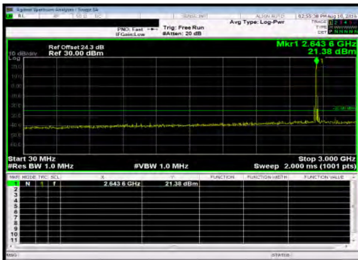
Out of Band Emission Low_Band41 15MHz_QPSK 1 0_HighCH41165-2647.5
