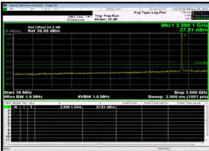
Out of Band Emission Low_Band41 5MHz_QPSK 1 0_MidCH40690-2600
