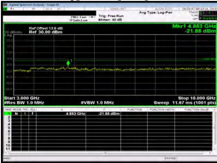
Out of Band Emission High_Band12 1.4MHz_QPSK 1 0_MidCH23095-707.5
