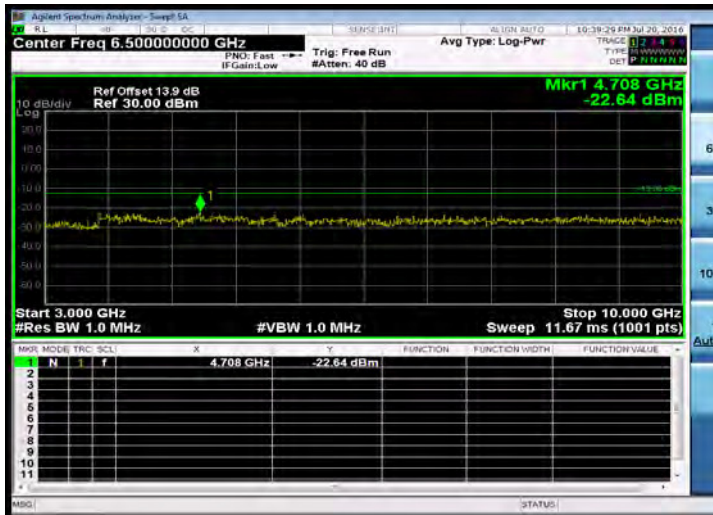
Out of Band Emission_Band26 for Part 90S_3M-QPSK-1 0-LOW-30M-3G
