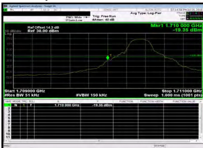
Band Edge_Band4 5MHz_QPSK 1 0_LowCH19975-1712.5
