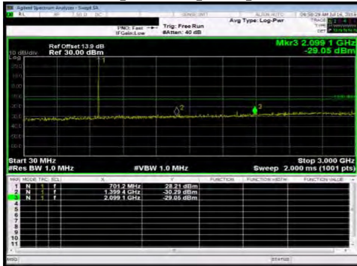
Out of Band Emission Low_Band12 1.4MHz_QPSK 1 0_MidCH23095-707.5
