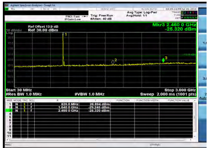
Out of Band Emission Low_Band26 10MHz_QPSK 1 0_LowCH26840-829
