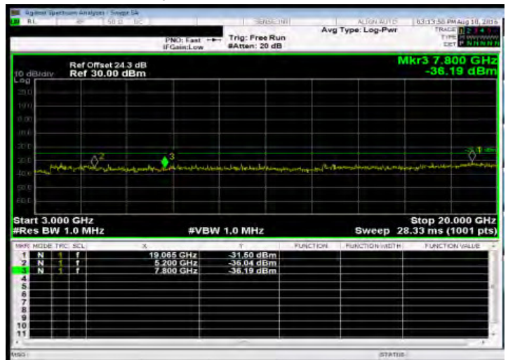
Out of Band Emission High_Band41 10MHz_QPSK 1 0_MidCH40690-2600
