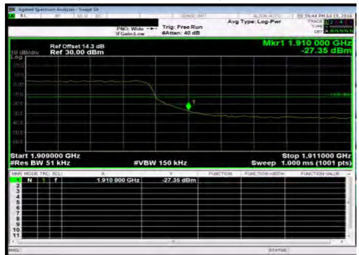
Band Edge_Band2 5MHz_QPSK 25 0_HighCH19175-1907.5
