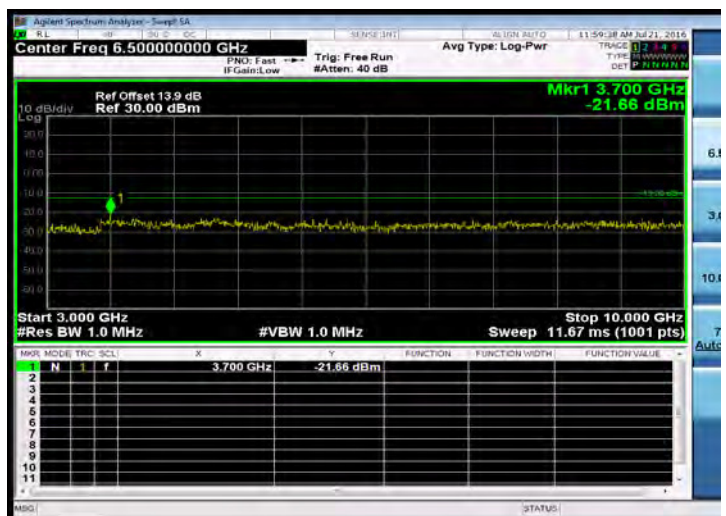
Out of Band Emission_Band26 for Part 90S_1.4M-QPSK-1 5-MID-3G-10G
