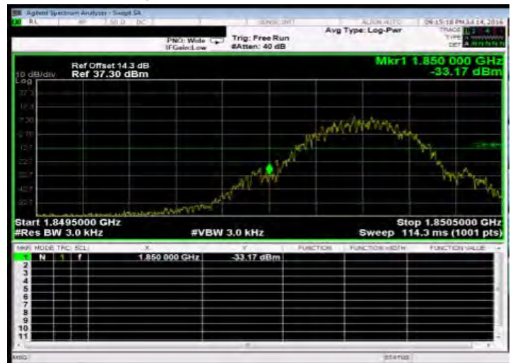
Band Edge_GPRS_1900MHz_LowCH512-1850.2
