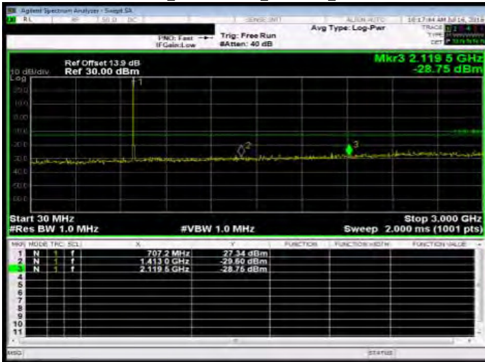
Out of Band Emission Low_Band17 5MHz_QPSK 1 0_MidCH23790-710
