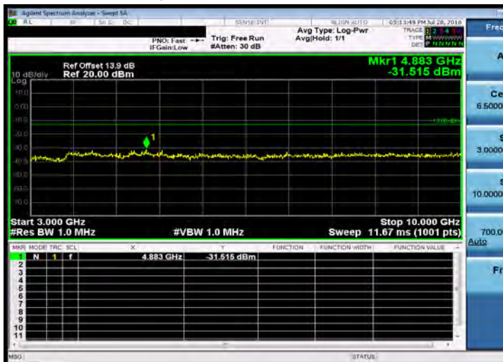
Out of Band Emission High_Band26 10MHz_QPSK 1 0_MidCH26915-836.5
