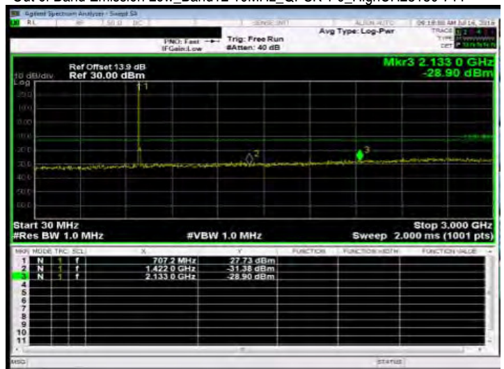
Out of Band Emission Low_Band12 10MHz_QPSK 1 0_HighCH23130-711
