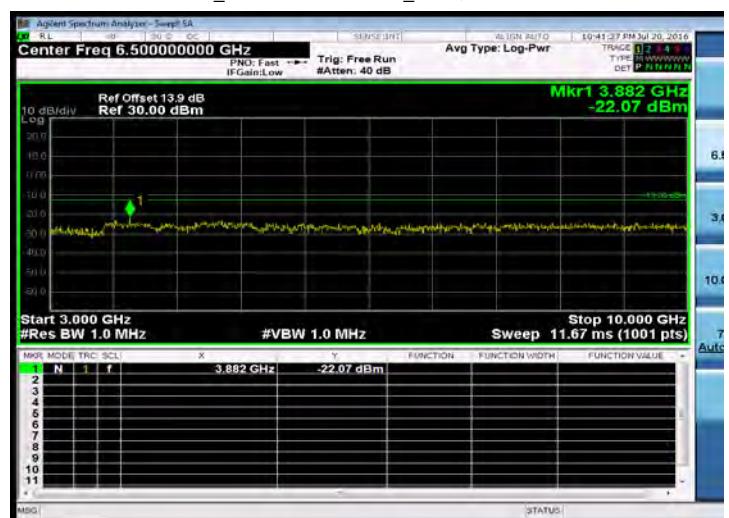
Out of Band Emission_Band26 for Part 90S_3M-QPSK-1 14-MID-3G-10G
