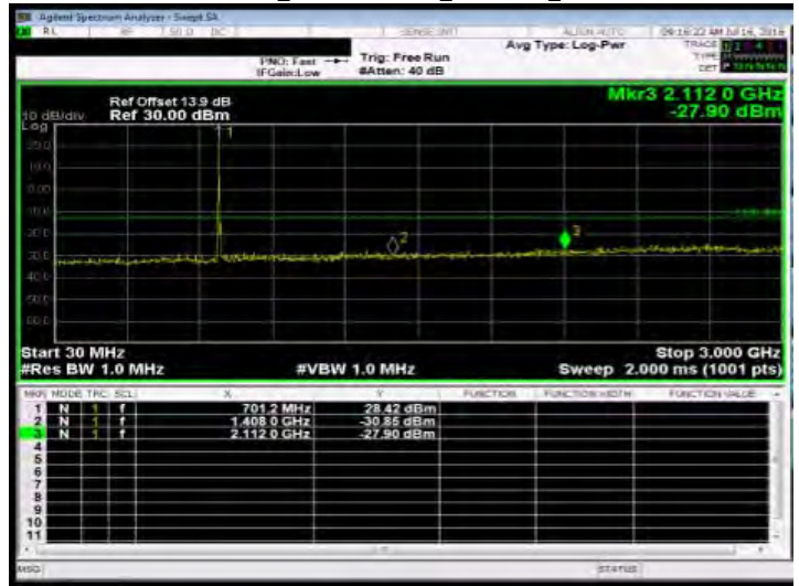
Out of Band Emission Low_Band12 10MHz_QPSK 1 0_MidCH23095-707.5
