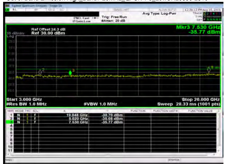
Out of Band Emission High_Band7 20MHz_QPSK 1 0_MidCH21100-2535
