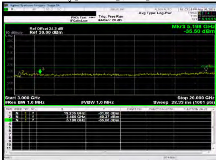
Out of Band Emission High_Band7 15MHz_QPSK 1 0_HighCH21375-2562.5
