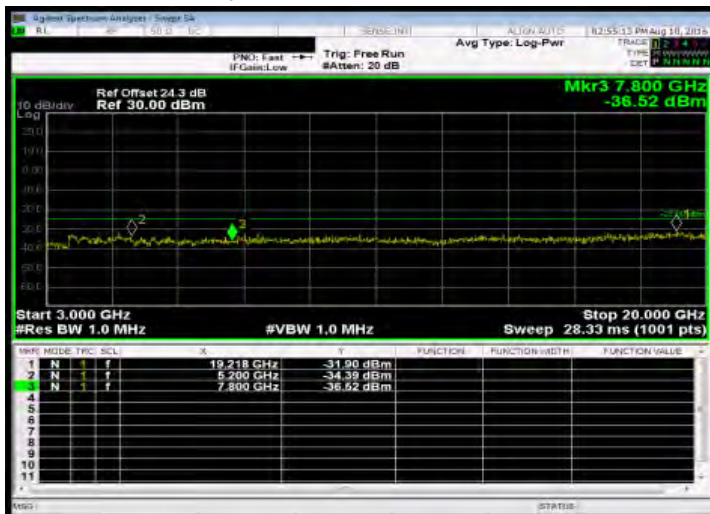
Out of Band Emission High_Band41 15MHz_QPSK 1 0_MidCH40690-2600
