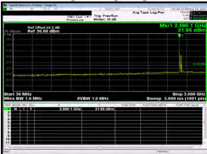
Out of Band Emission Low_Band38 15MHz_QPSK 1 0_HighCH38175-2612.5
