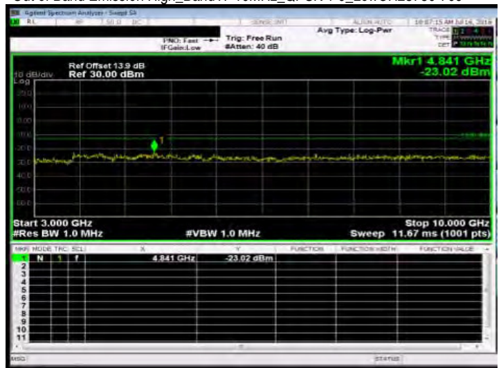
Out of Band Emission High_Band17 10MHz_QPSK 1 0_MidCH23790-710
