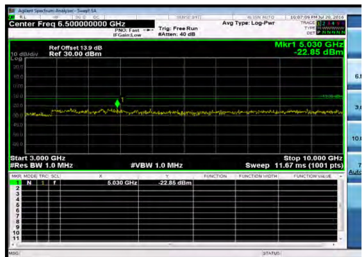
Out of Band Emission_Band26 for Part 90S_5M-QPSK-1 24-MID-3G-10G
