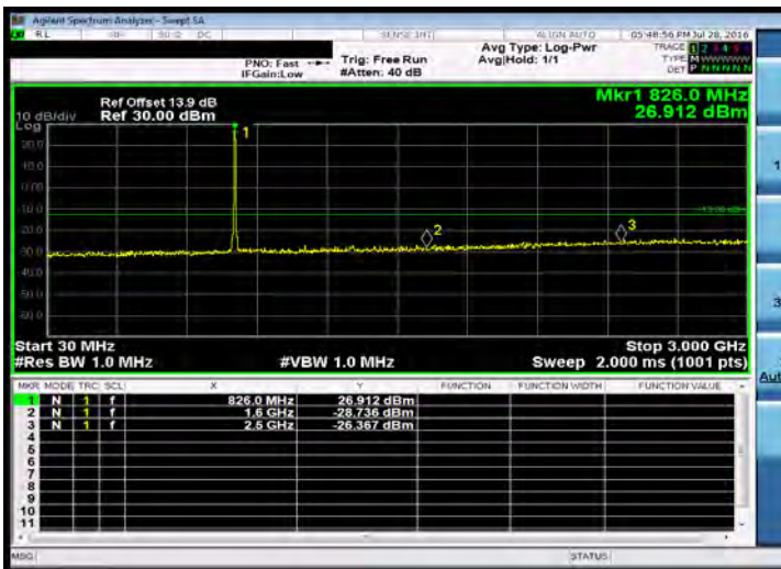
Out of Band Emission Low_Band26 5MHz_QPSK 1 0_LowCH26815-826.5
