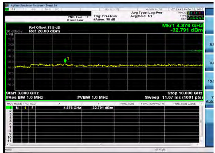
Out of Band Emission High_Band26 1.4MHz_QPSK 1 0_MidCH26915-836.5
