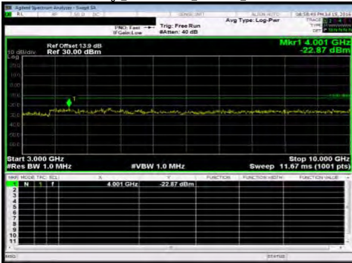
Out of Band Emission High_Band5 1.4MHz_QPSK 1 0_MidCH20525-836.5
