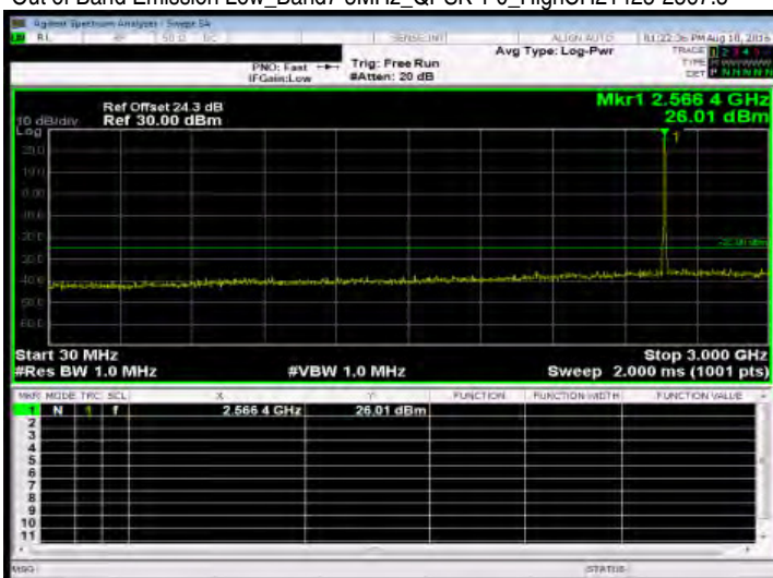
Out of Band Emission Low_Band7 5MHz_QPSK 1 0_HighCH21425-2567.5
