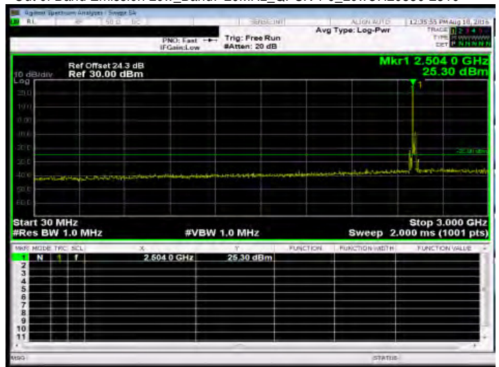
Out of Band Emission Low_Band7 20MHz_QPSK 1 0_MidCH21100-2535
