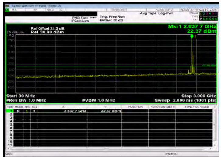
Out of Band Emission Low_Band41 20MHz_QPSK 1 0_HighCH41140-2645
