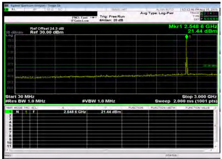
Out of Band Emission Low_Band41 10MHz_QPSK 1 0_LowCH40190-2550
