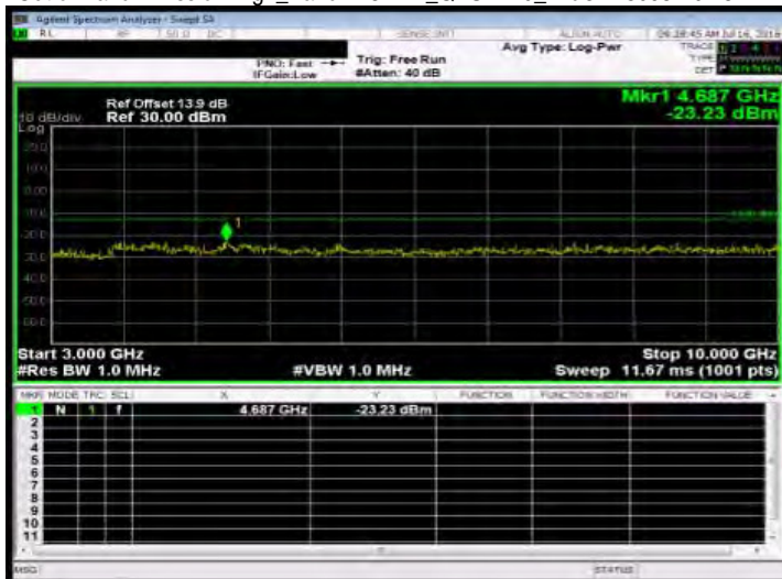
Out of Band Emission High_Band12 5MHz_QPSK 1 0_HighCH23155-713.5
