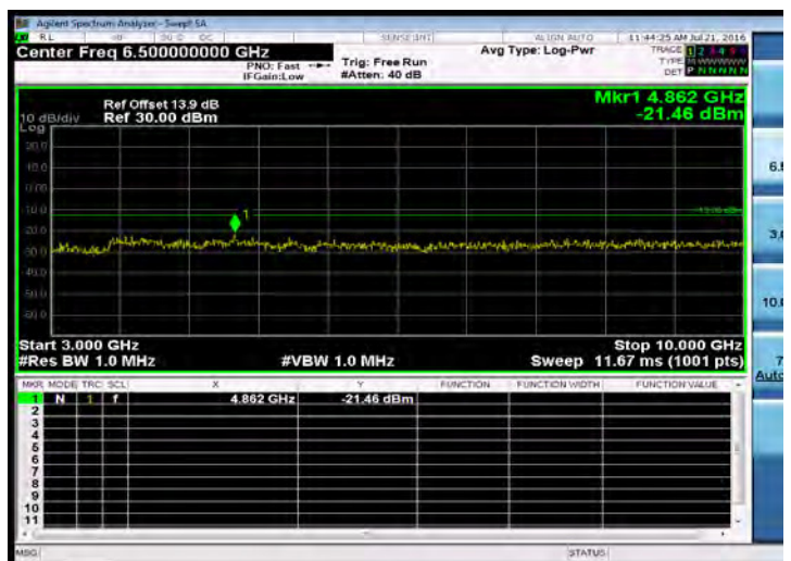
Out of Band Emission_Band26 for Part 90S_1.4M-QPSK-1 0-MID-3G-10G
