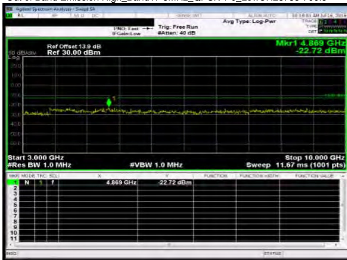
Out of Band Emission High_Band17 5MHz_QPSK 1 0_MidCH23790-710
