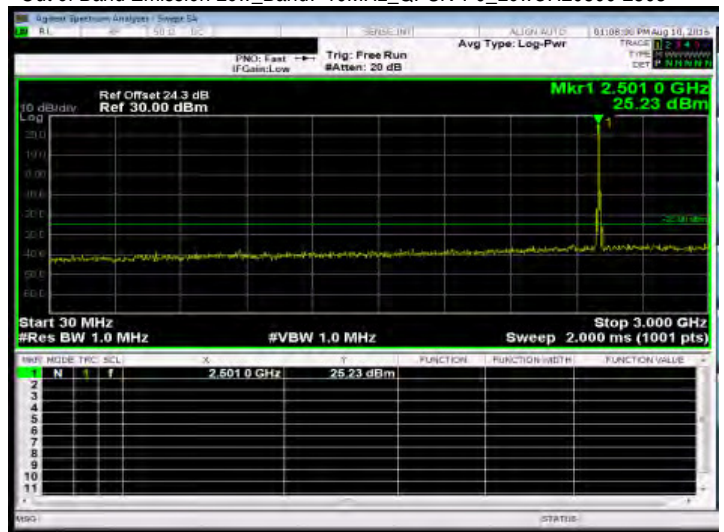
Out of Band Emission Low_Band7 10MHz_QPSK 1 0_MidCH21100-2535
