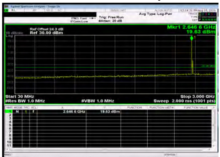
Out of Band Emission Low_Band41 10MHz_QPSK 1 0_HighCH41190-2650
