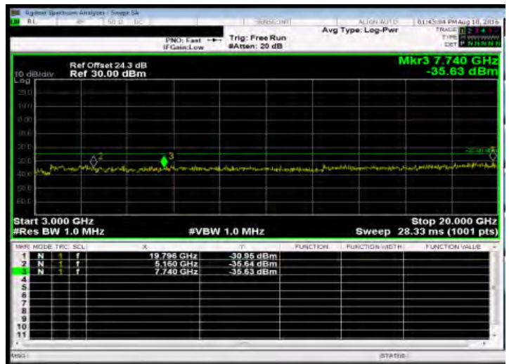
Out of Band Emission High_Band38 20MHz_QPSK 1 0_LowCH37850-2580
