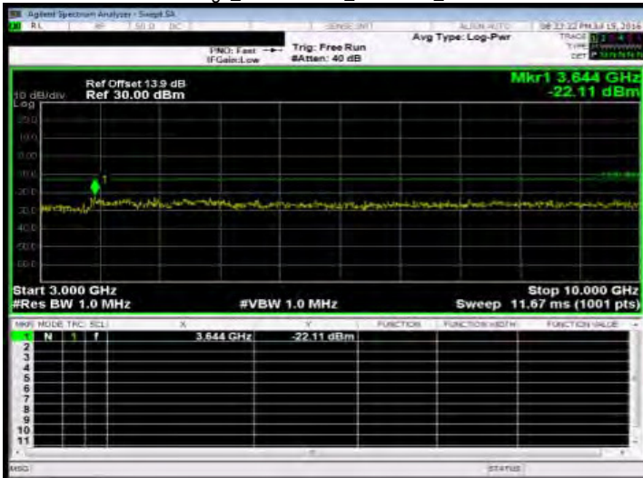
Out of Band Emission High_Band5 5MHz_QPSK 1 0_HighCH20625-846.5
