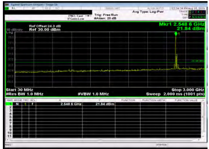
Out of Band Emission Low_Band41 20MHz_QPSK 1 0_MidCH40690-2600
