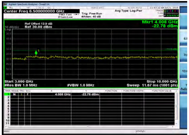
Out of Band Emission_Band26 for Part 90S_1.4M-QPSK-1 0-MID-30M-3G
