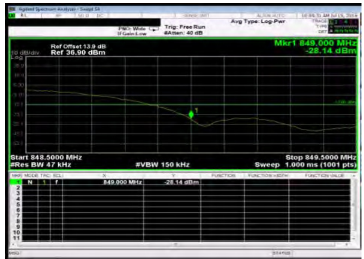
Band Edge_WCDMA_B5_HighCH4233-846.6
