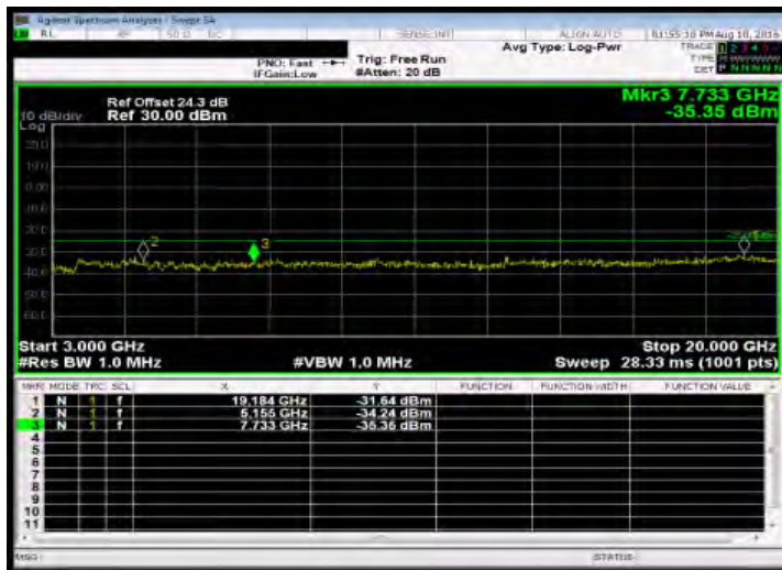
Out of Band Emission High_Band38 15MHz_QPSK 1 0_LowCH37825-2577.5
