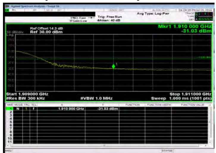
Band Edge_Band2 20MHz_QPSK 100 0_HighCH19100-1900
