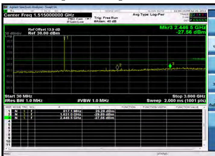
Out of Band Emission_Band26 for Part 90S_3M-QPSK-1 14-LOW-30M-3G
