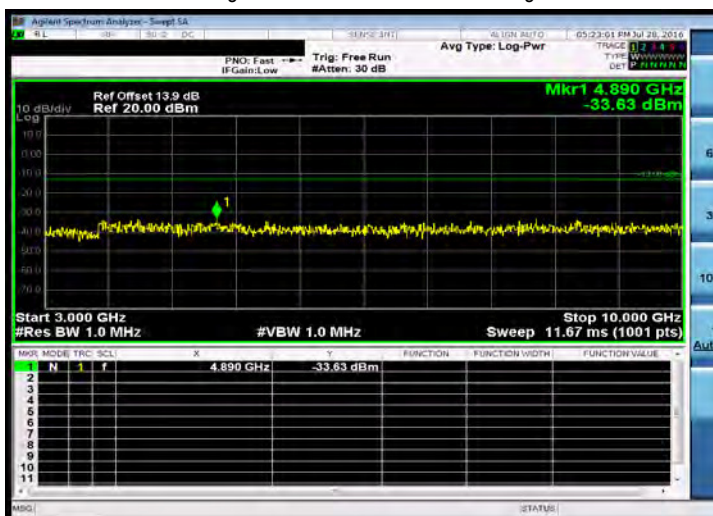
Out of Band Emission High_Band26 10MHz_QPSK 1 0_HighCH26990-844
