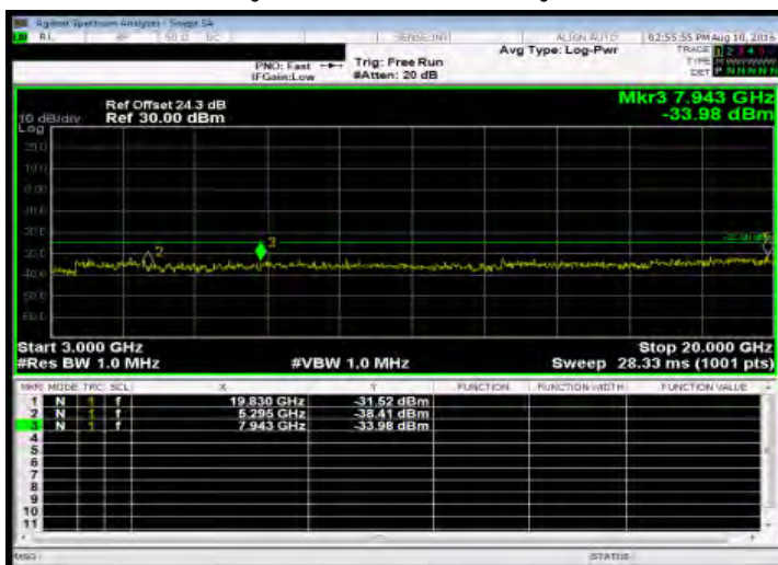
Out of Band Emission High_Band41 15MHz_QPSK 1 0_HighCH41165-2647.5
