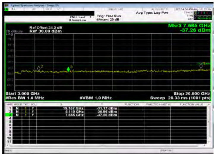
Out of Band Emission High_Band41 20MHz_QPSK 1 0_LowCH40240-2555
