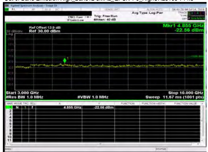
Out of Band Emission High_Band12 3MHz_QPSK 1 0_HighCH23165-714.5
