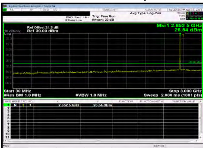
Out of Band Emission Low_Band41 5MHz_QPSK 1 0_HighCH41215-2652.5
