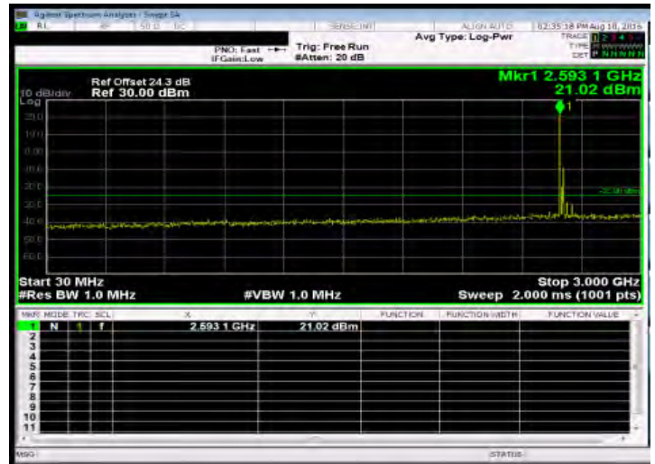
Out of Band Emission Low_Band41 20MHz_QPSK 1 0_MidCH40690-2600
