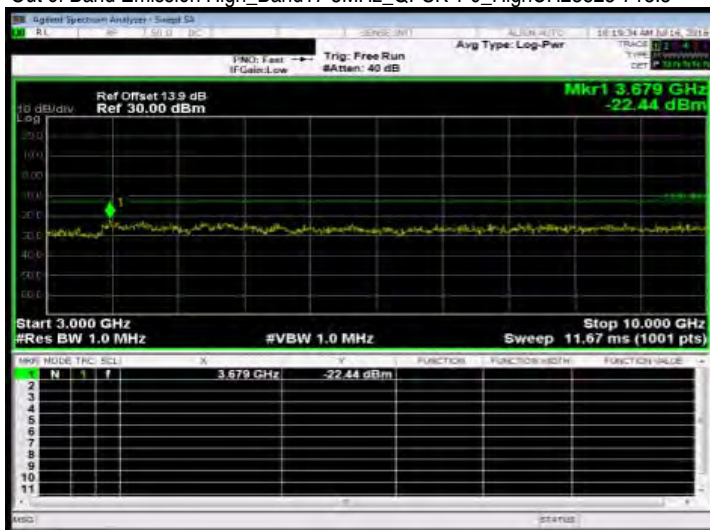
Out of Band Emission High_Band17 5MHz_QPSK 1 0_HighCH23825-713.5
