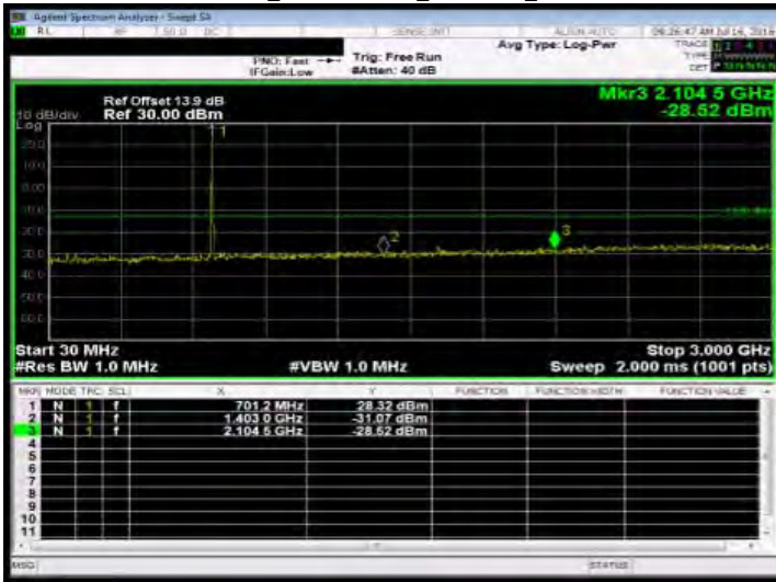
Out of Band Emission Low_Band12 5MHz_QPSK 1 0_MidCH23095-707.5
