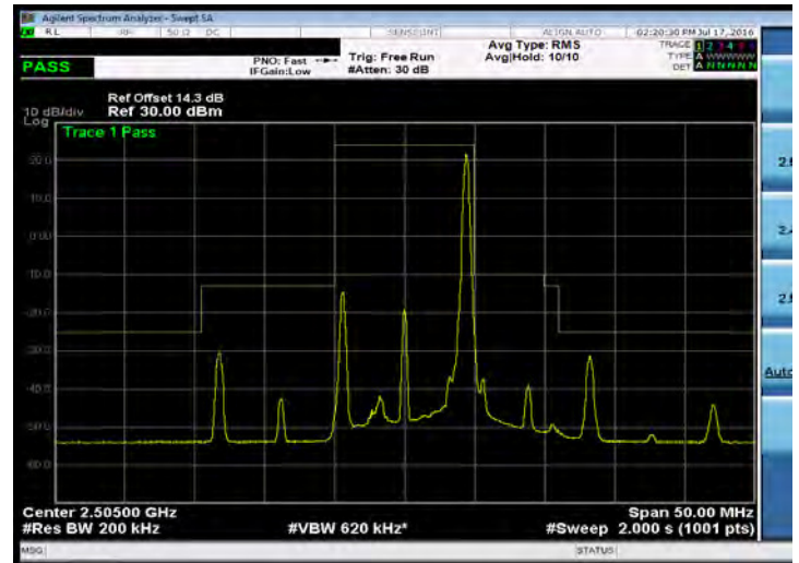
Emission Mask_Band 7_10M_QPSK_LOW_RB1,49
