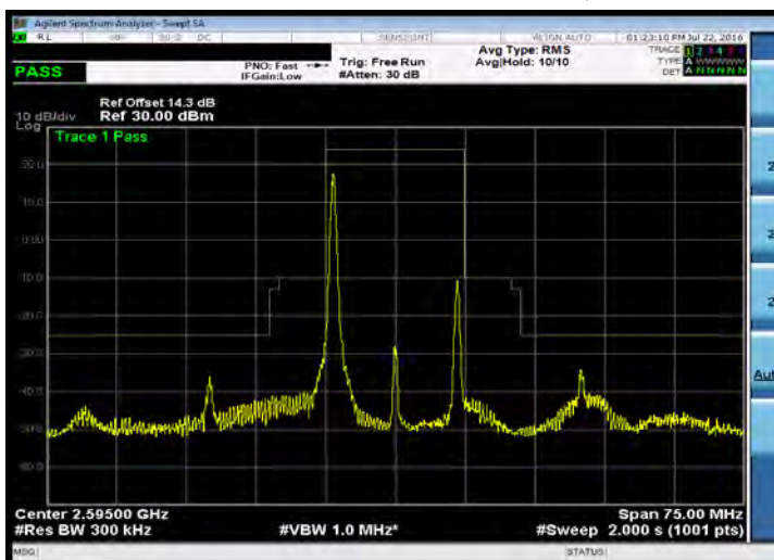
Emission Mask_Band 38_15M_16QAM_MID_RB1,0
