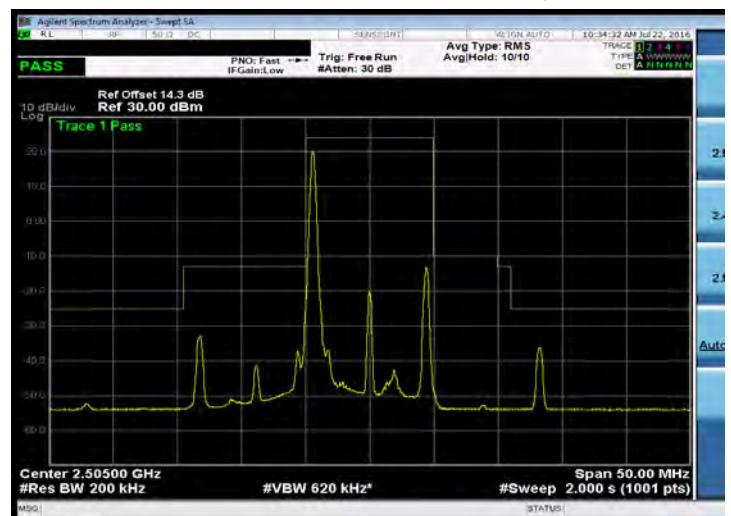
Emission Mask_Band 7_10M_16QAM_LOW_RB1,0
