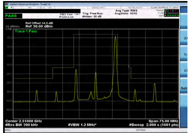
Emission Mask_Band 7_20M_QPSK_LOW_RB1,99
