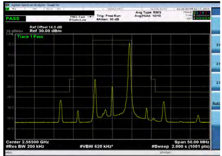
Emission Mask_Band 7_10M_QPSK_HIGH_RB50,0
