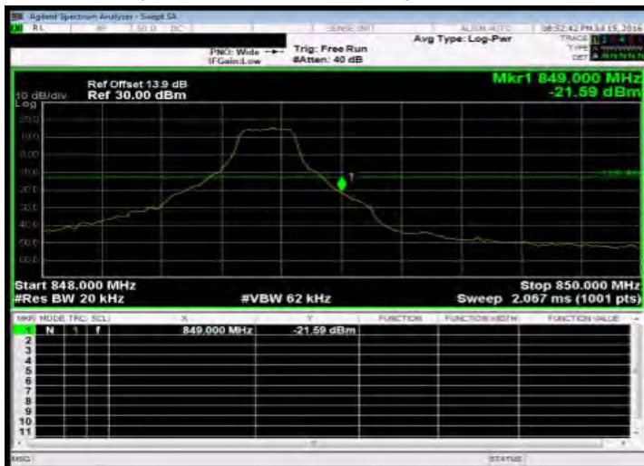
Band Edge_Band5 1.4MHz_QPSK 1 5_HighCH20643-848.3
