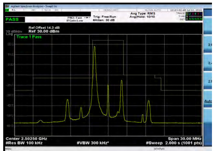
Emission Mask_Band 7_5M_16QAM_LOW_RB1,0
