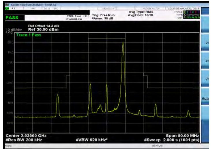
Emission Mask_Band 7_10M_16QAM_MID_RB1,49
