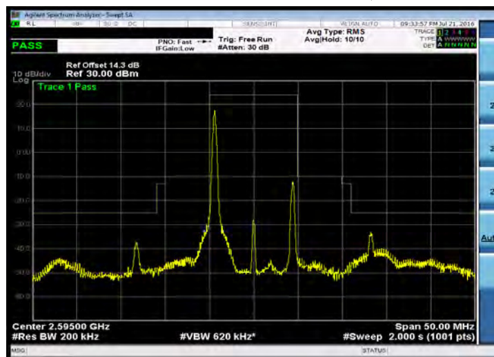
Emission Mask_Band 38_10M_QPSK_MID_RB1,0
