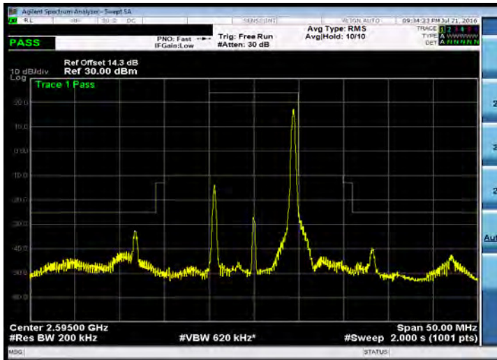
Emission Mask_Band 38_10M_QPSK_MID_RB1,49
