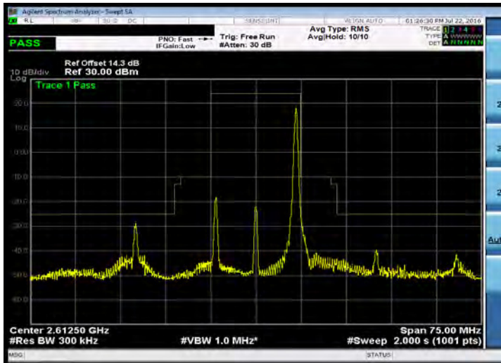
Emission Mask_Band 38_15M_16QAM_HIGH_RB1,74
