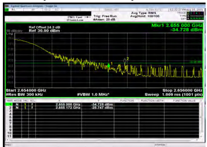
Band Edge_Band41 20MHz_QPSK 1 99_HighCH41140-2645
