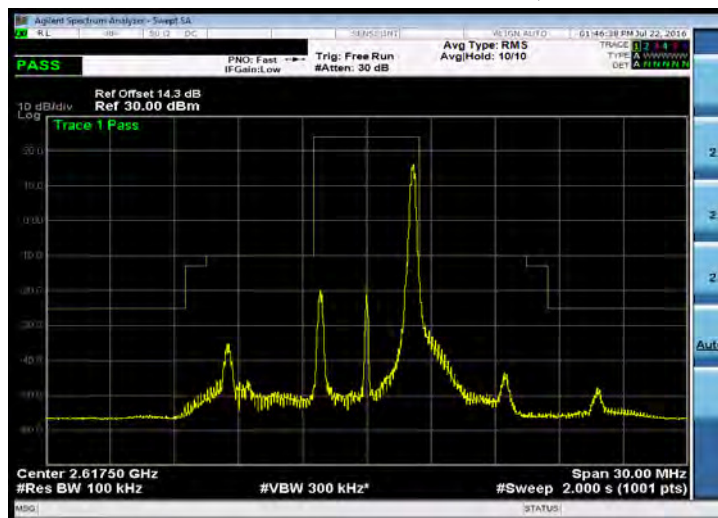
Emission Mask_Band 38_5M_16QAM_HIGH_RB25,0
