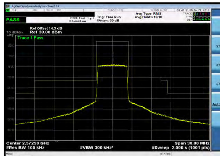
Emission Mask_Band 38_5M_QPSK_LOW_RB25,0
