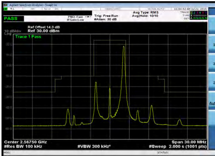
Emission Mask_Band 7_5M_16QAM_HIGH_RB1,24
