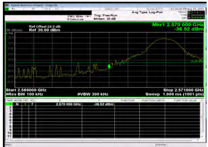
Band Edge_Band38 10MHz_QPSK 1 0_LowCH37800-2575
