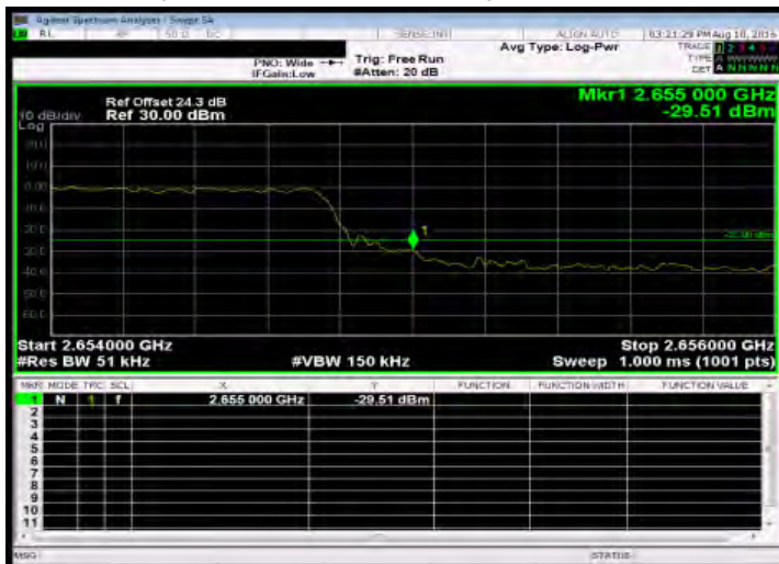
Band Edge_Band41 5MHz_QPSK 25 0_HighCH41215-2652.5
