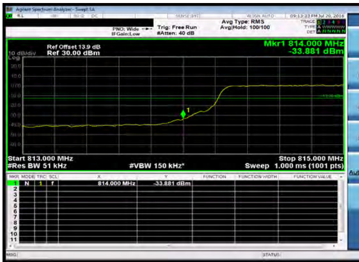
Band Edge_Band 26 for Part 90S_5M-16QAM-25 0-HIGH
