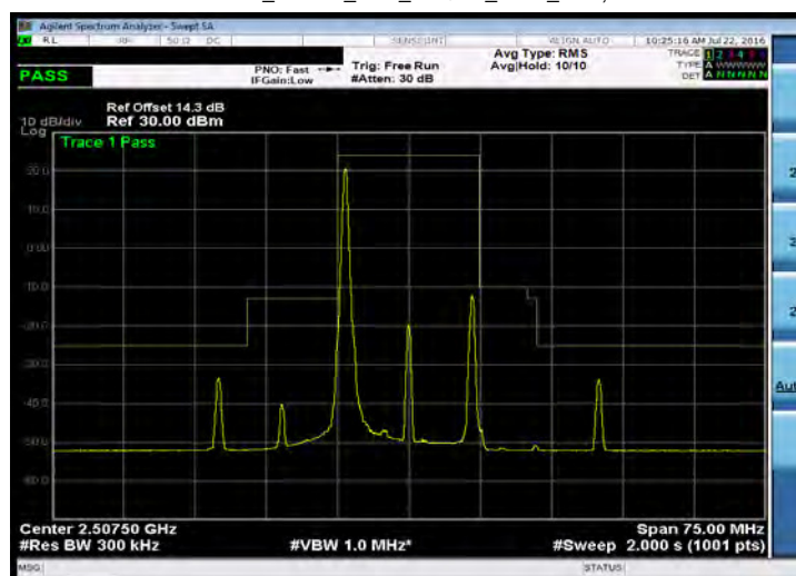
Emission Mask_Band 7_15M_16QAM_LOW_RB1,0
