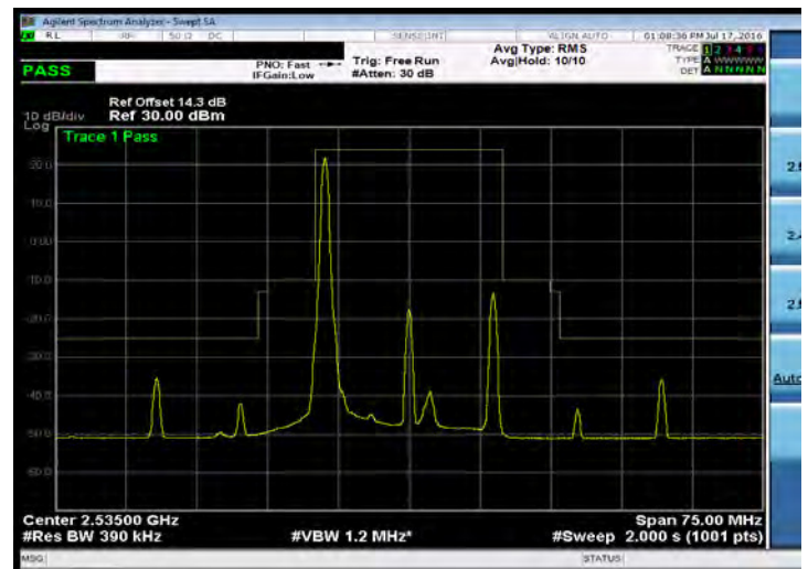
Emission Mask_Band 7_20M_QPSK_MID_RB1,0
