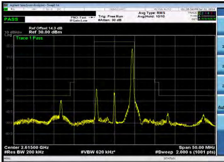
Emission Mask_Band 38_10M_16QAM_HIGH_RB1,49
