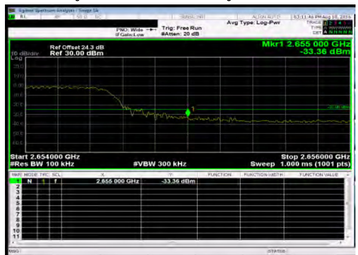
Band Edge_Band41 10MHz_QPSK 50 0_HighCH41190-2650
