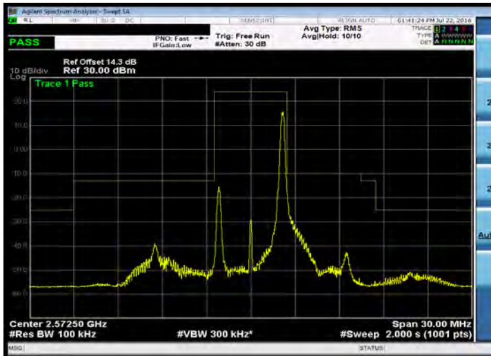
Emission Mask_Band 38_5M_16QAM_LOW_RB1,24
