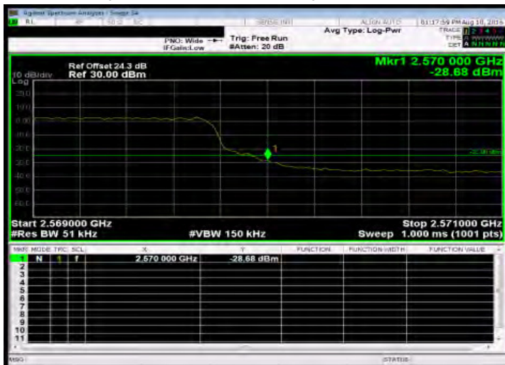
Band Edge_Band7 5MHz_QPSK 25 0_HighCH21425-2567.5
