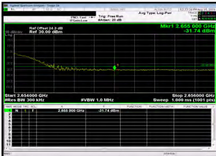
Band Edge_Band41 20MHz_QPSK 100 0_HighCH41140-2645
