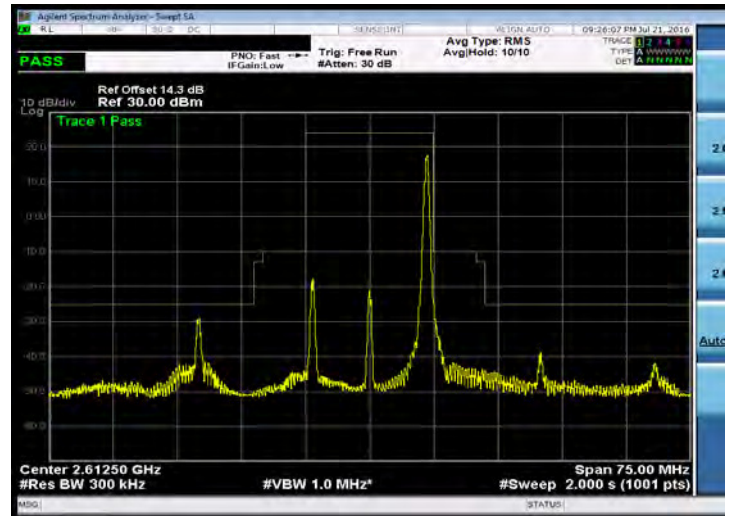
Emission Mask_Band 38_15M_QPSK_HIGH_RB1,74
