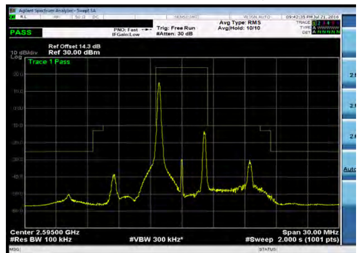
Emission Mask_Band 38_5M_QPSK_MID_RB1,0
