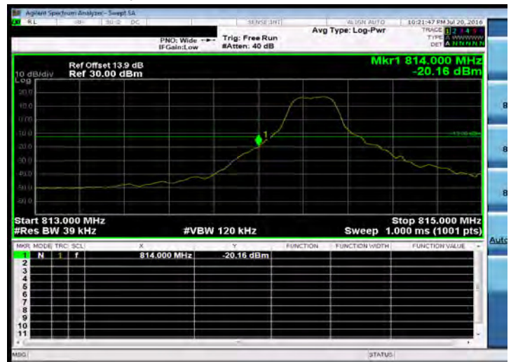
Band Edge_Band 26 for Part 90S_3M-QPSK-1 14-HIGH
