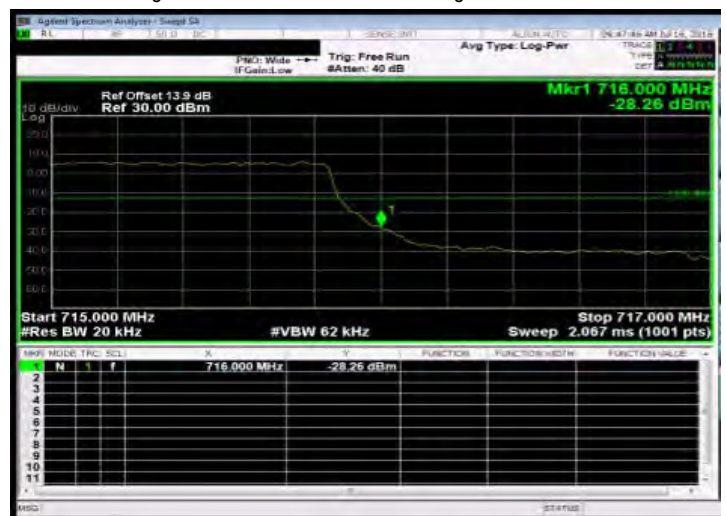
Band Edge_Band12 1.4MHz_QPSK 6 0_HighCH23173-715.3
