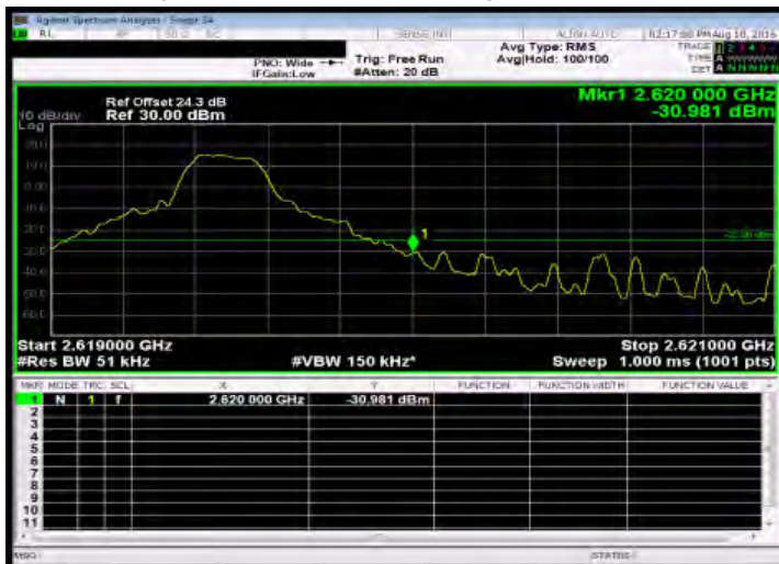
Band Edge_Band38 5MHz_QPSK 1 24_HighCH38225-2617.5
