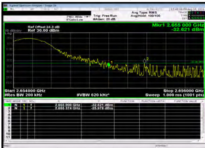
Band Edge_Band41 15MHz_QPSK 1 74_HighCH41165-2647.5
