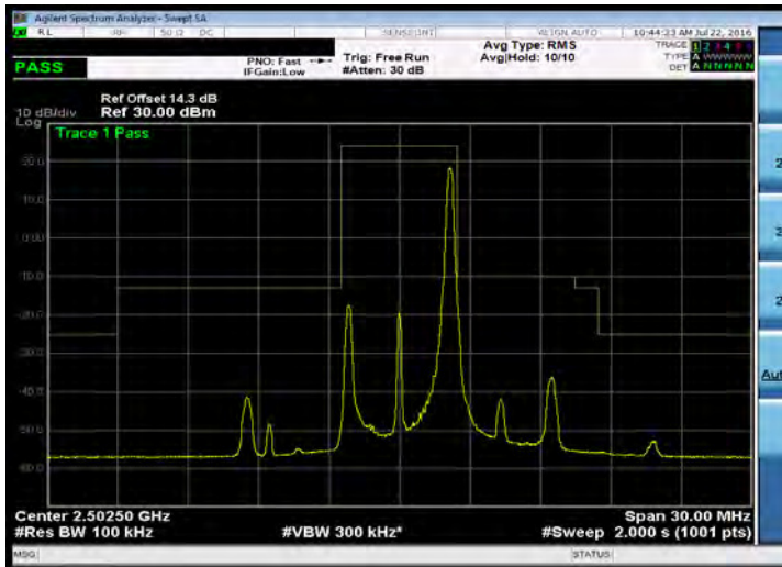
Emission Mask_Band 7_5M_16QAM_LOW_RB1,24
