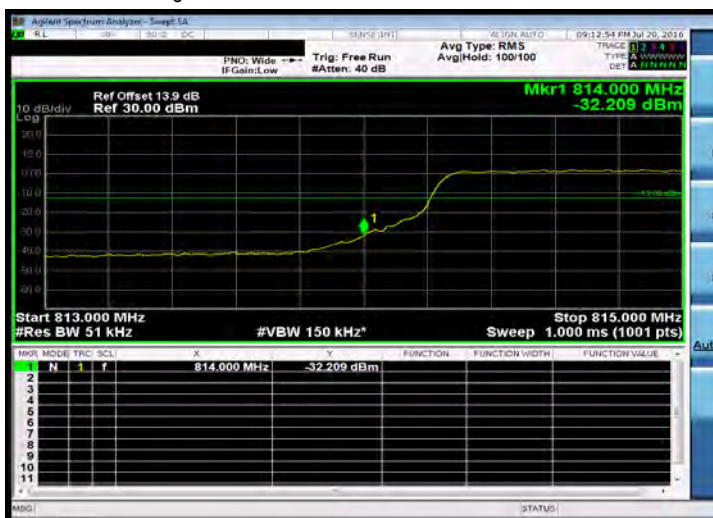
Band Edge_Band 26 for Part 90S_5M-QPSK-25 0-LOW
