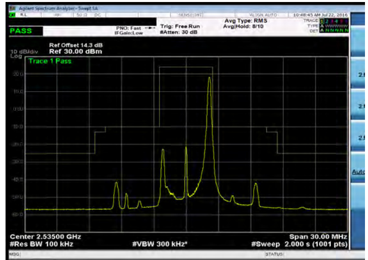
Emission Mask_Band 7_5M_16QAM_MID_RB1,24
