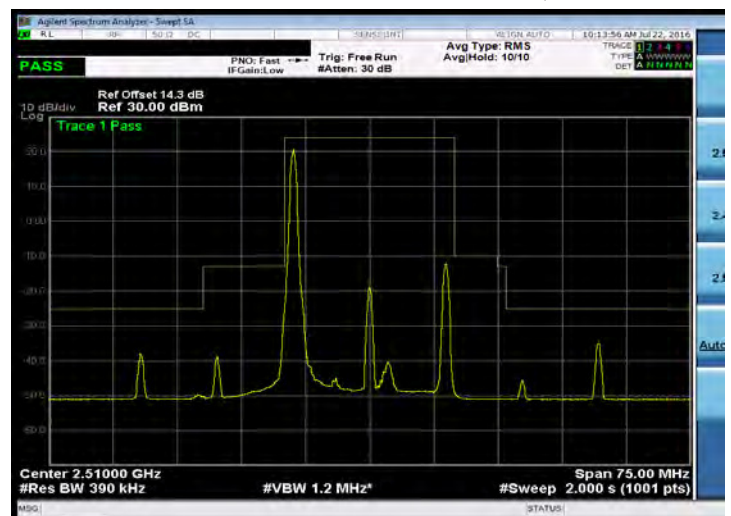
Emission Mask_Band 7_20M_16QAM_LOW_RB1,0
