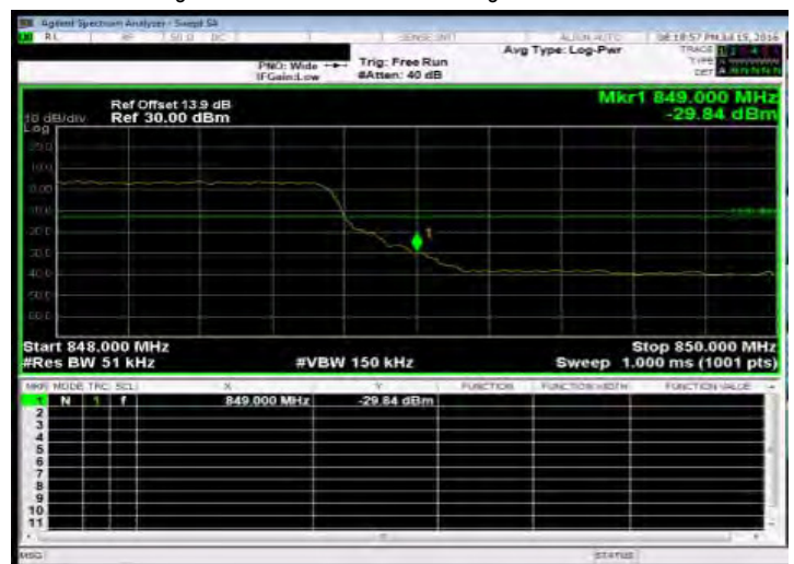
Band Edge_Band5 5MHz_QPSK 25 0_HighCH20625-846.5
