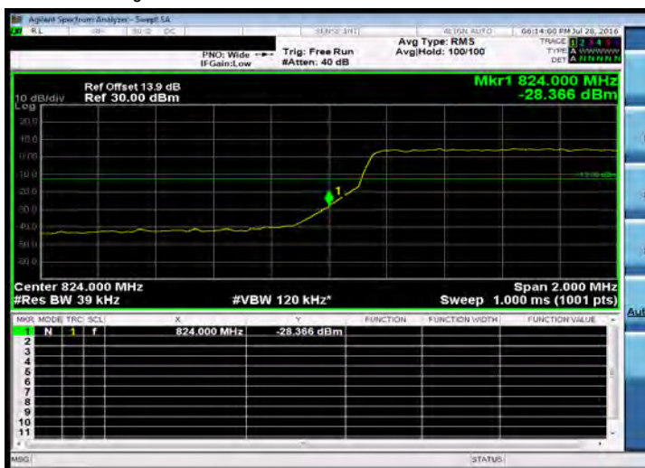
Band Edge_Band26 3MHz_QPSK 15 0_Low CH26805-825.5
