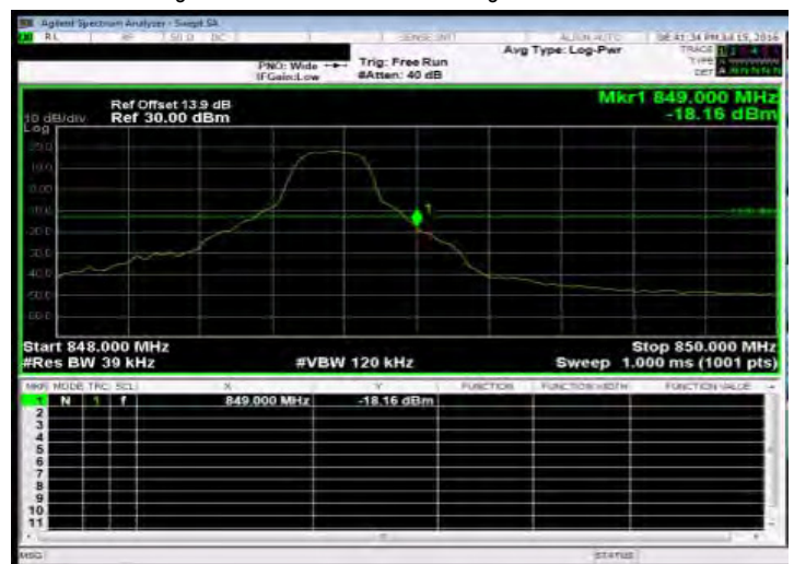
Band Edge_Band5 3MHz_QPSK 1 14_HighCH20635-847.5
