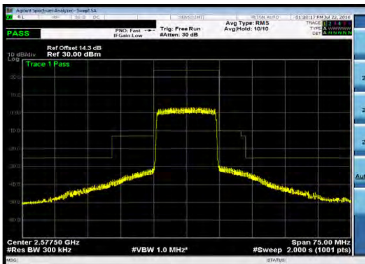
Emission Mask_Band 38_15M_16QAM_LOW_RB75,0
