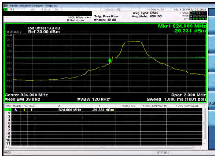
Band Edge_Band26 3MHz_QPSK 1 0_Low CH26805-825.5
