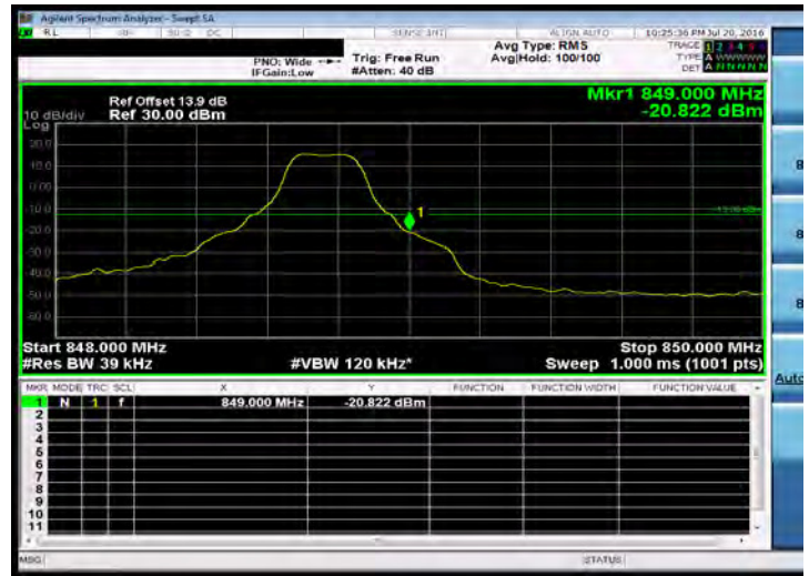
Band Edge_Band 26 for Part 90S_3M-16QAM-15 0-LOW
