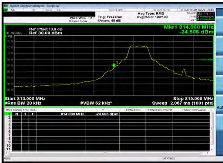
Band Edge_Band 26 for Part 90S_1.4M-16QAM-1 5-HIGH
