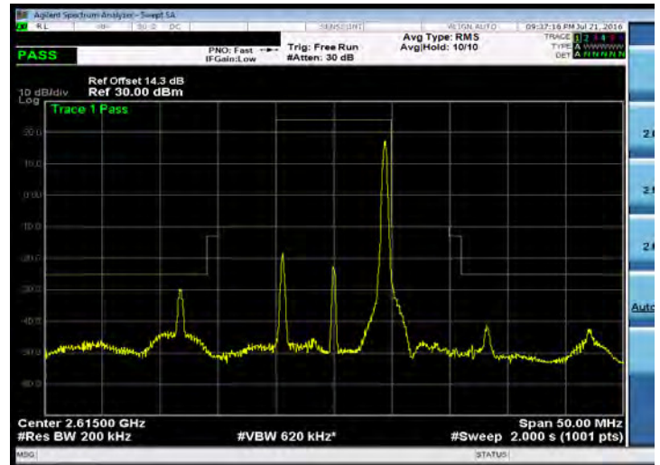
Emission Mask_Band 38_10M_QPSK_HIGH_RB1,49
