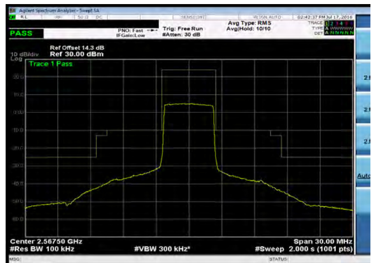
Emission Mask_Band 7_5M_QPSK_HIGH_RB25,0
