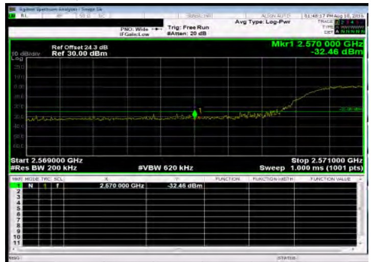
Band Edge_Band38 15MHz_QPSK 75 0_LowCH37825-2577.5
