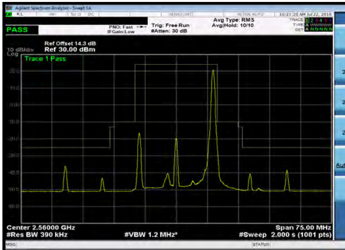
Emission Mask_Band 7_20M_16QAM_HIGH_RB100,0
