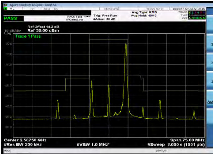
Emission Mask_Band 7_15M_16QAM_LOW_RB1,74
