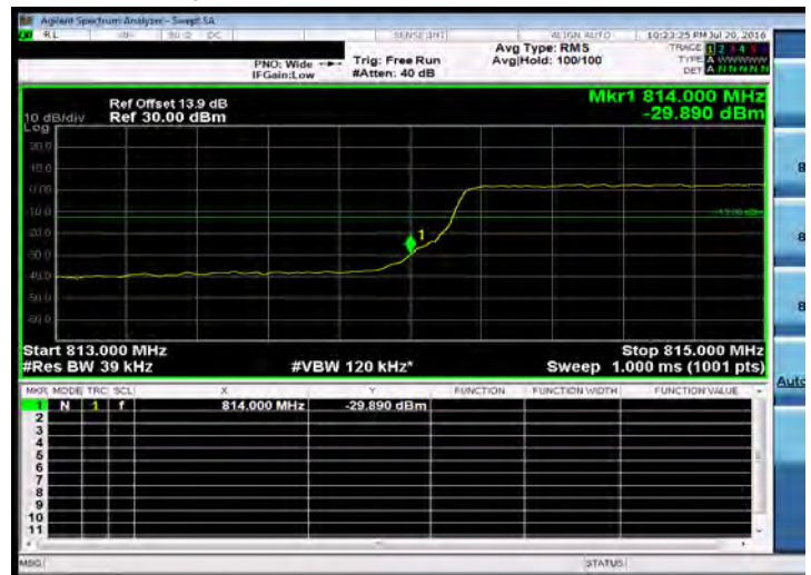
Band Edge_Band 26 for Part 90S_3M-16QAM-15 0-HIGH
