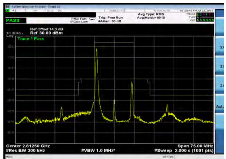
Emission Mask_Band 38_15M_16QAM_HIGH_RB1,0
