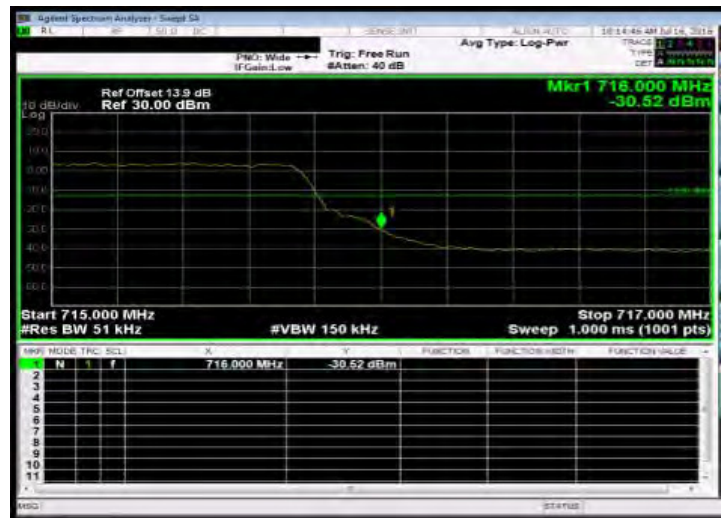
Band Edge_Band17 5MHz_QPSK 25 0_HighCH23825-713.5
