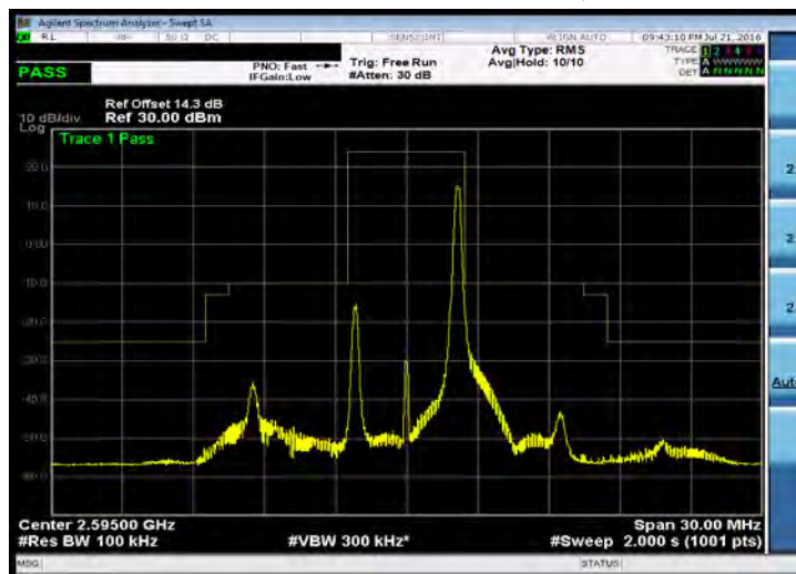
Emission Mask_Band 38_5M_QPSK_MID_RB25,0
