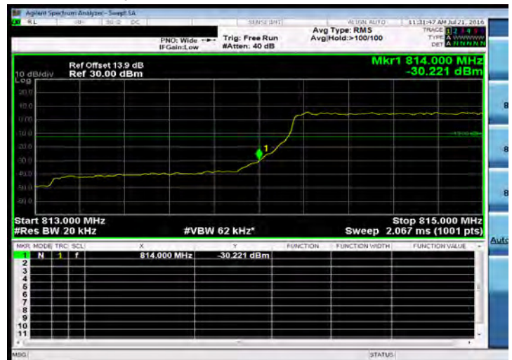
Band Edge_Band 26 for Part 90S_1.4M-QPSK-6 0-LOW
