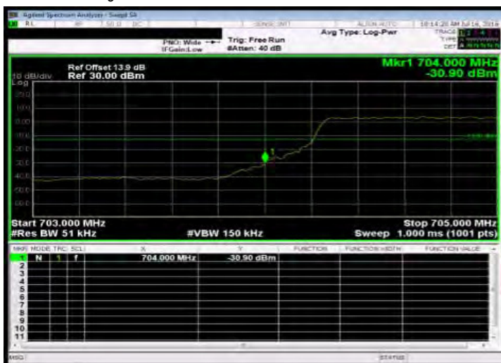
Band Edge_Band17 5MHz_QPSK 25 0_LowCH23755-706.5
