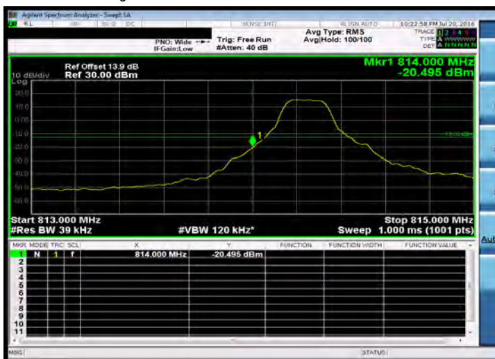
Band Edge_Band 26 for Part 90S_3M-16QAM-1 0-LOW
