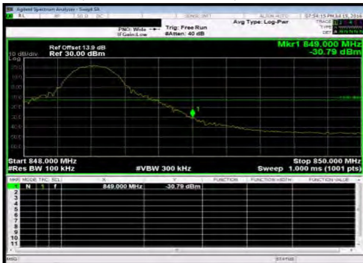
Band Edge_Band5 10MHz_QPSK 1 49_HighCH20600-844
