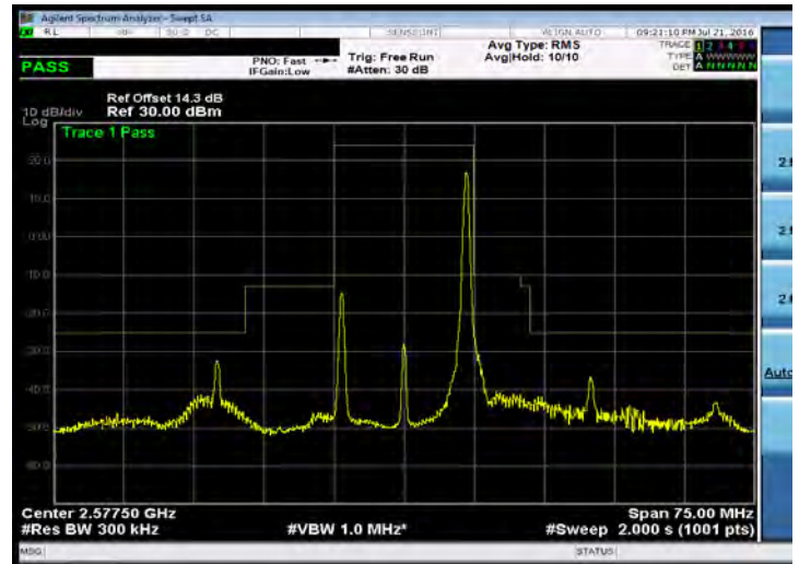
Emission Mask_Band 38_15M_QPSK_LOW_RB1,74
