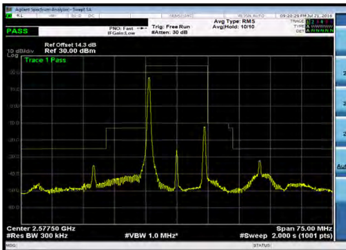
Emission Mask_Band 38_15M_QPSK_LOW_RB1,0
