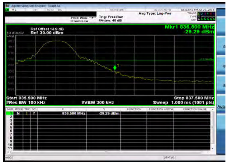
Band Edge_Band 26 for Part 90S_10M-QPSK-50 0-MID/L
