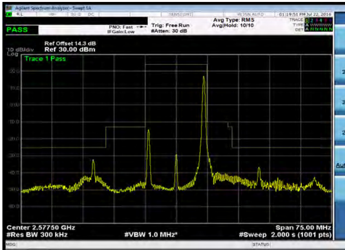
Emission Mask_Band 38_15M_16QAM_LOW_RB1,74
