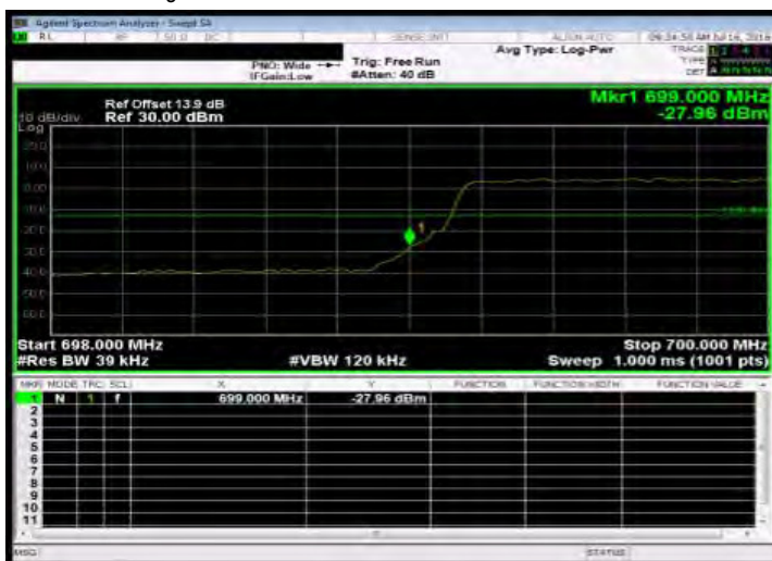
Band Edge_Band12 3MHz_QPSK 15 0_LowCH23025-700.5
