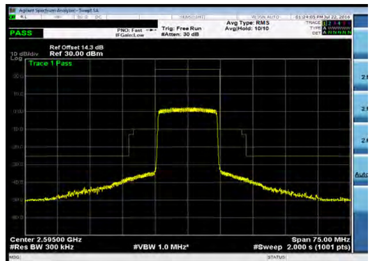
Emission Mask_Band 38_15M_16QAM_MID_RB75,0
