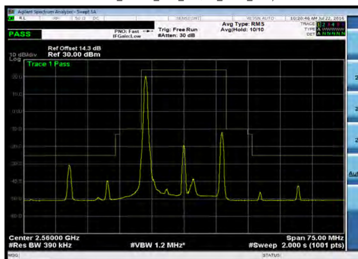
Emission Mask_Band 7_20M_16QAM_HIGH_RB1,0
