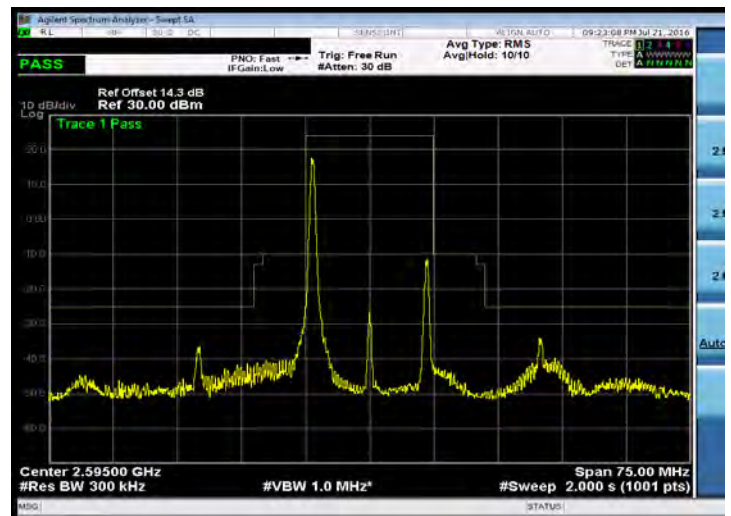
Emission Mask_Band 38_15M_QPSK_MID_RB1,0
