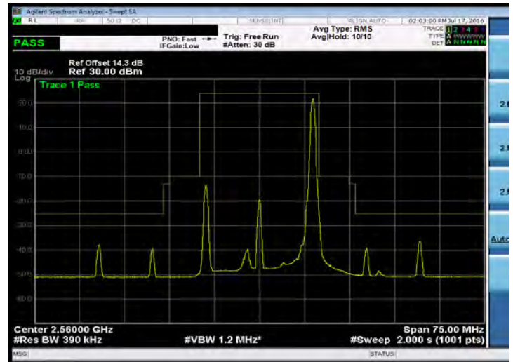
Emission Mask_Band 7_20M_QPSK_HIGH_RB100,0
