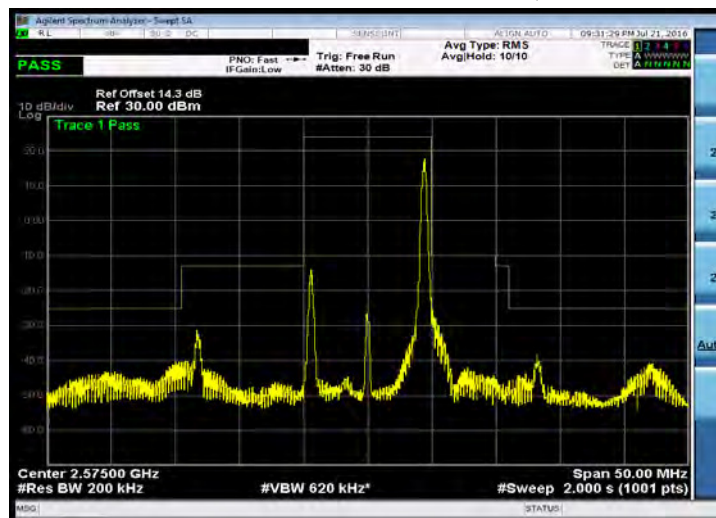
Emission Mask_Band 38_10M_QPSK_LOW_RB50,0
