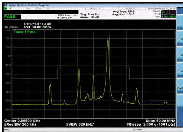
Emission Mask_Band 7_10M_16QAM_HIGH_RB50,0
