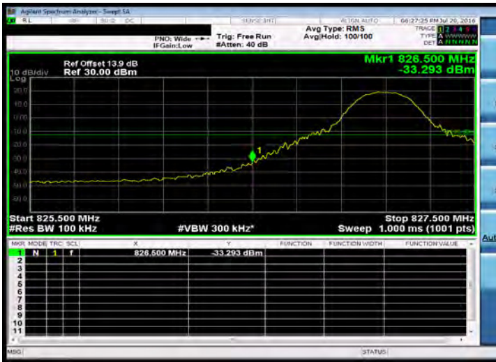
Band Edge_Band 26 for Part 90S_10M-16QAM-1 49-MID
