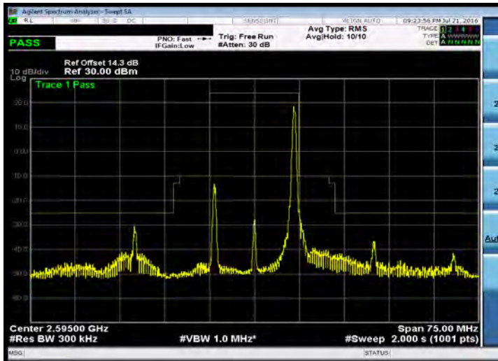
Emission Mask_Band 38_15M_QPSK_MID_RB1,74
