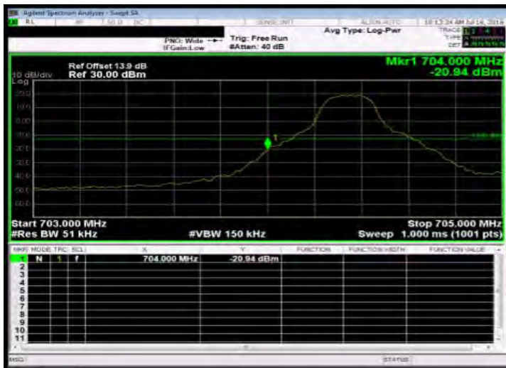
Band Edge_Band17 5MHz_QPSK 1 0_LowCH23755-706.5
