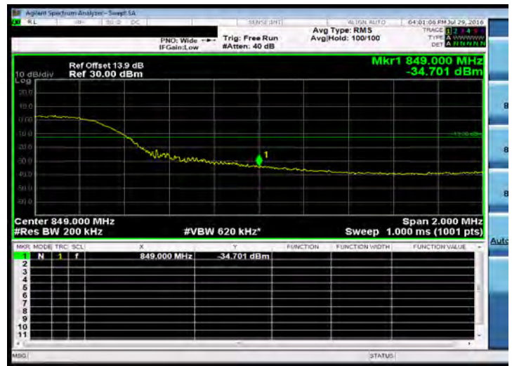
Band Edge_Band26 10MHz_QPSK 75 0_High
