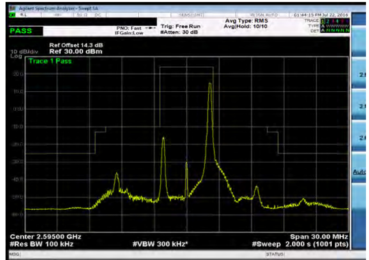
Emission Mask_Band 38_5M_16QAM_MID_RB1,24
