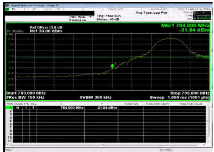
Band Edge_Band17 10MHz_QPSK 1 0_LowCH23780-709
