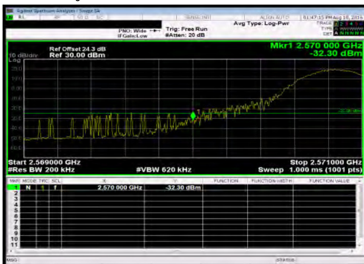
Band Edge_Band38 15MHz_QPSK 1 0_LowCH37825-2577.5
