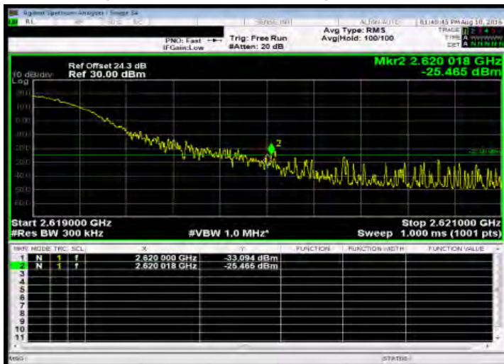
Band Edge_Band38 20MHz_QPSK 1 99_HighCH38150-2610
