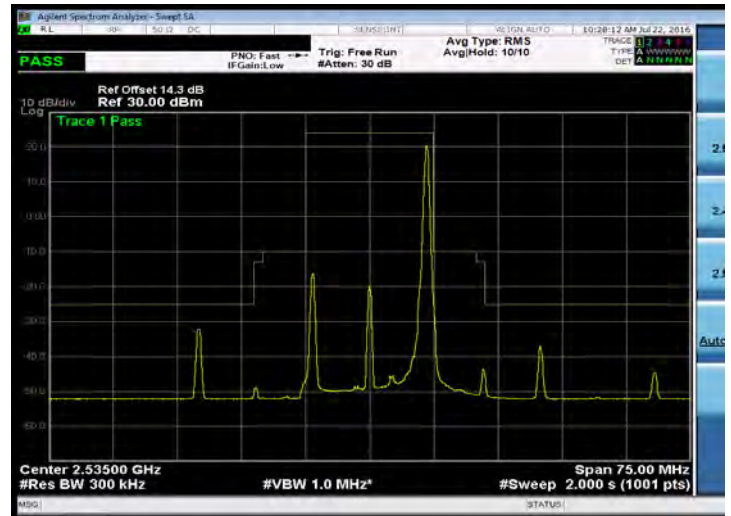
Emission Mask_Band 7_15M_16QAM_MID_RB1,74
