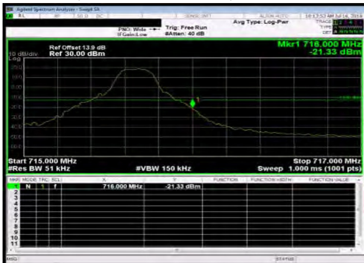
Band Edge_Band17 5MHz_QPSK 1 24_HighCH23825-713.5
