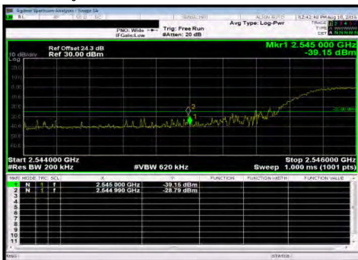
Band Edge_Band41 15MHz_QPSK 75 0_LowCH40215-2552.5
