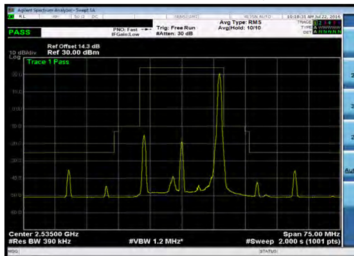
Emission Mask_Band 7_20M_16QAM_MID_RB100,0
