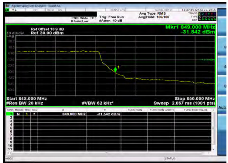
Band Edge_Band 26 for Part 90S_3M-QPSK-1 0-LOW
