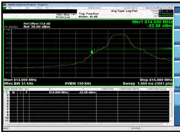
Band Edge_Band 26 for Part 90S_5M-QPSK-1 24-HIGH
