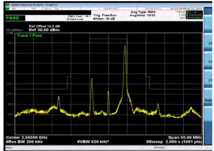
Emission Mask_Band 38_10M_16QAM_MID_RB50,0
