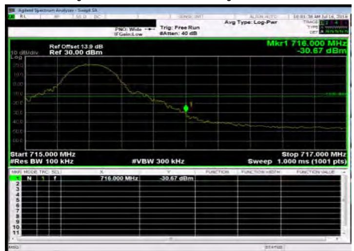
Band Edge_Band17 10MHz_QPSK 1 49_HighCH23800-711
