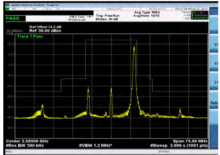
Emission Mask_Band 38_20M_QPSK_LOW_RB1,99
