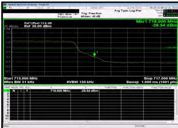
Band Edge_Band12 5MHz_QPSK 25 0_HighCH23155-713.5
