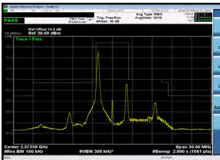
Emission Mask_Band 38_5M_QPSK_LOW_RB1,0
