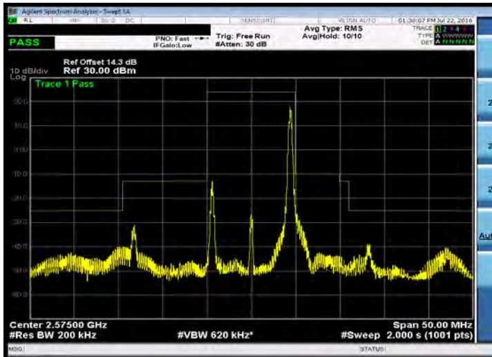
Emission Mask_Band 38_10M_16QAM_LOW_RB50,0
