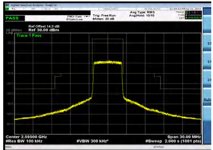
Emission Mask_Band 38_5M_16QAM_HIGH_RB1,0
