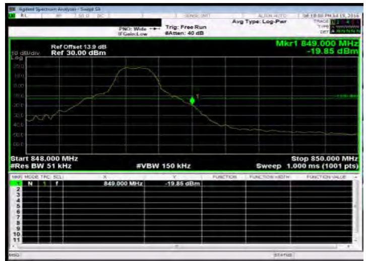
Band Edge_Band5 5MHz_QPSK 1 24_HighCH20625-846.5
