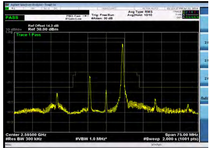
Emission Mask_Band 38_15M_16QAM_MID_RB1,74
