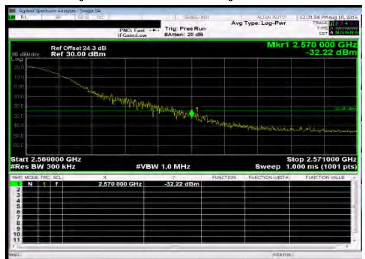
Band Edge_Band7 20MHz_QPSK 1 99_HighCH21350-2560
