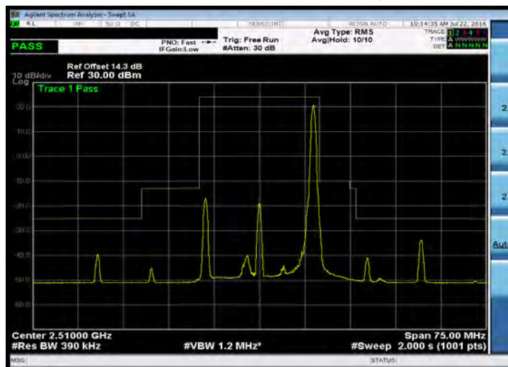
Emission Mask_Band 7_20M_16QAM_LOW_RB100,0
