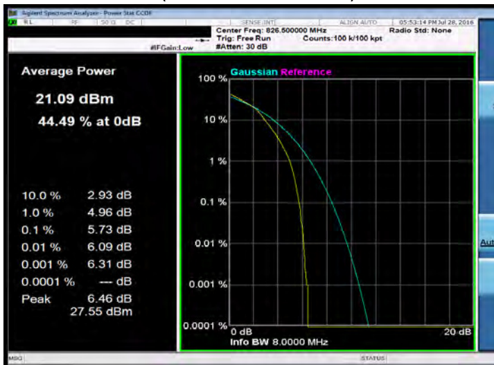
5MHz BW LTE-Band 26(16QAM Number: 25 Offset: 0) Channel Mid
