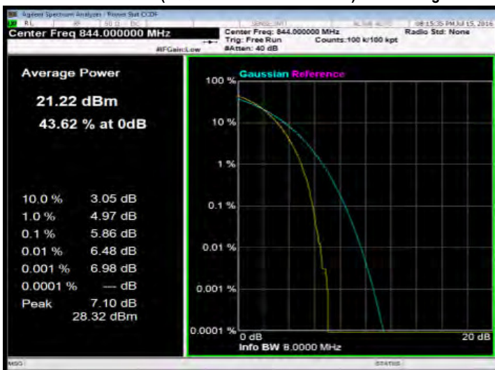
10MHz BW LTE-Band 5(16QAM Number: 50 Offset: 0) Channel High
