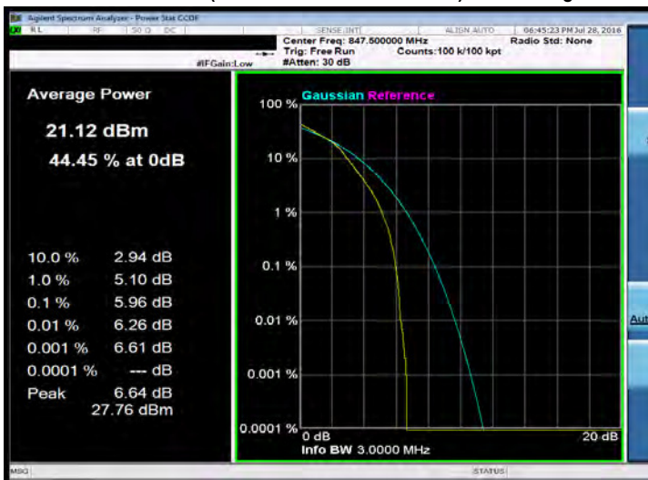
3MHz BW LTE-Band 26(16QAM Number: 15 Offset: 0) Channel High
