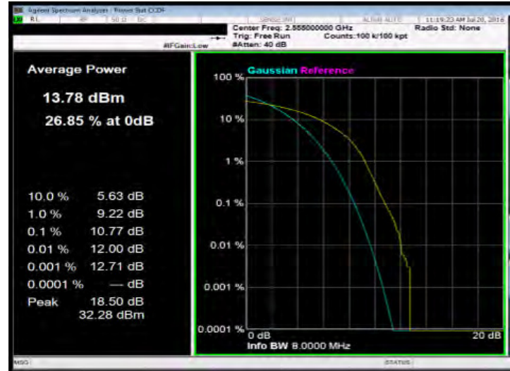
20MHz BW LTE-Band 41(16QAM Number: 100 Offset: 0) Channel Mid
