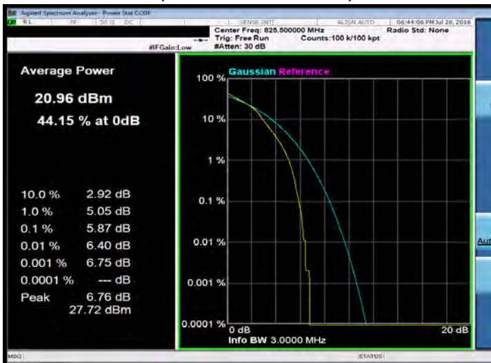
3MHz BW LTE-Band 26(16QAM Number: 15 Offset: 0) Channel Mid
