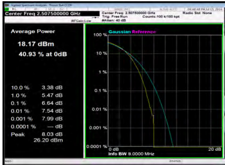
15MHz BW LTE-Band 7(16QAM Number: 75 Offset: 0) Channel Mid
