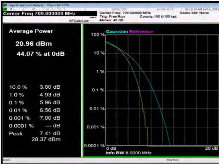
10MHz BW LTE-Band 17(16QAM Number: 50 Offset: 0) Channel Mid
