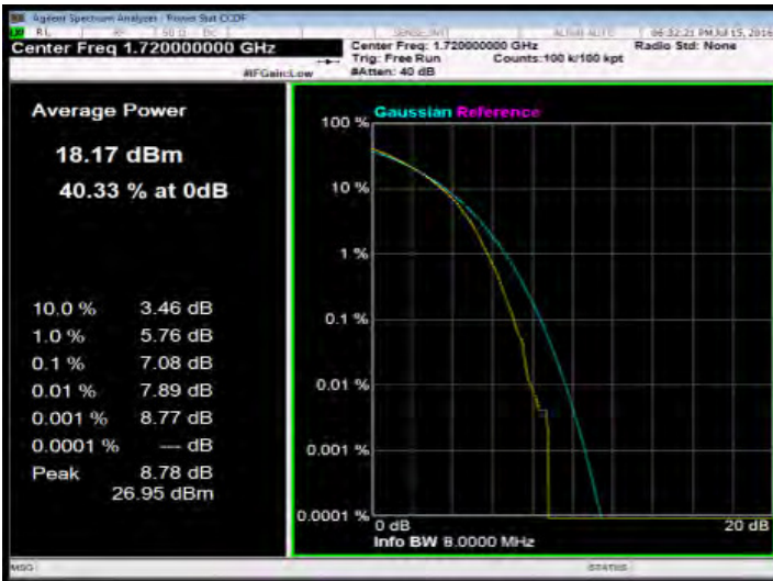
20MHz BW LTE-Band 4(16QAM Number: 100 Offset: 0) Channel Mid
