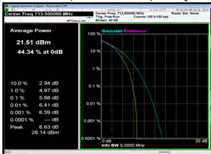
5MHz BW LTE-Band 12(16QAM Number: 25 Offset: 0) Channel High
