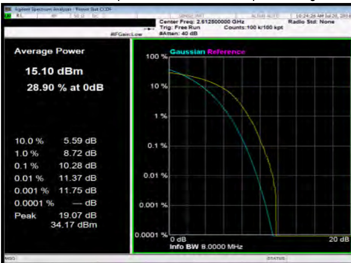
15MHz BW LTE-Band 38(16QAM Number: 75 Offset: 0) Channel High
