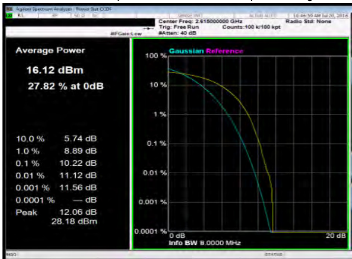
10MHz BW LTE-Band 38(16QAM Number: 50 Offset: 0) Channel High
