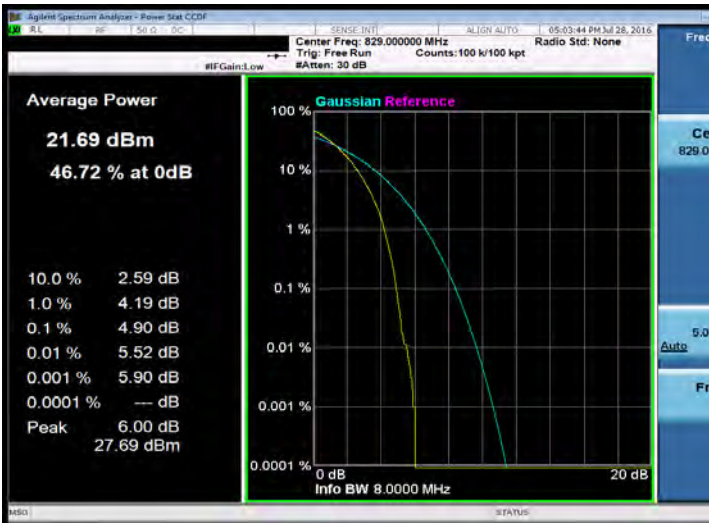
10MHz BW LTE-Band 26(16QAM Number: 50 Offset: 0) Channel Mid
