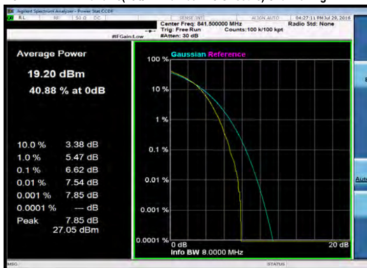
15MHz BW LTE-Band 26(16QAM Number: 75 Offset: 0) Channel High
