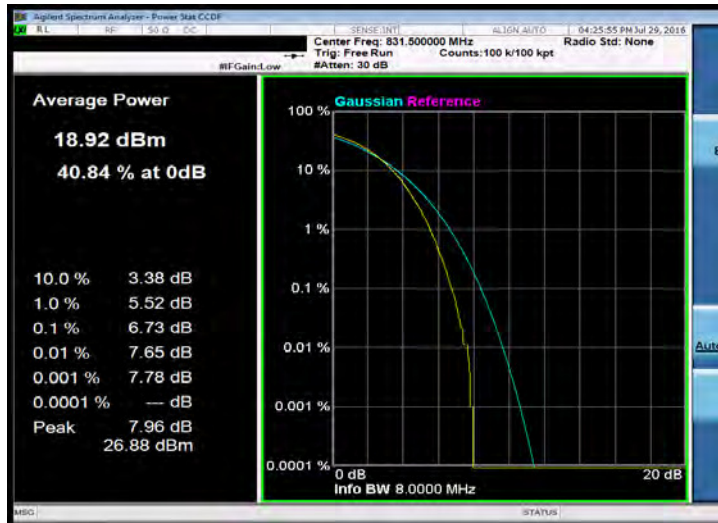
15MHz BW LTE-Band 26(16QAM Number: 75 Offset: 0) Channel Mid
