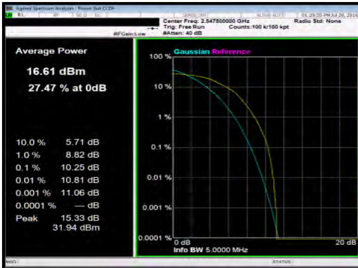
5MHz BW LTE-Band 41(16QAM Number: 25 Offset: 0) Channel Mid
