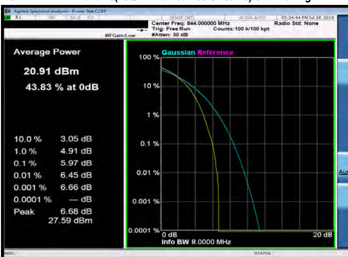
10MHz BW LTE-Band 26(16QAM Number: 50 Offset: 0) Channel High
