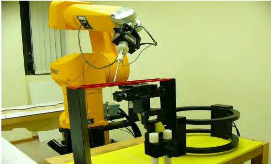
Fig. 1 Photograph of the DASY 5 measurement system
