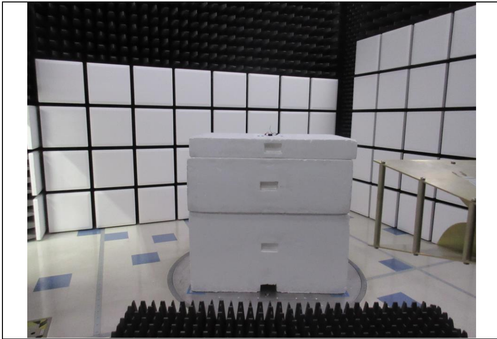
RF Radiated #4 (Radiated Testing for Restricted Band Edge)
