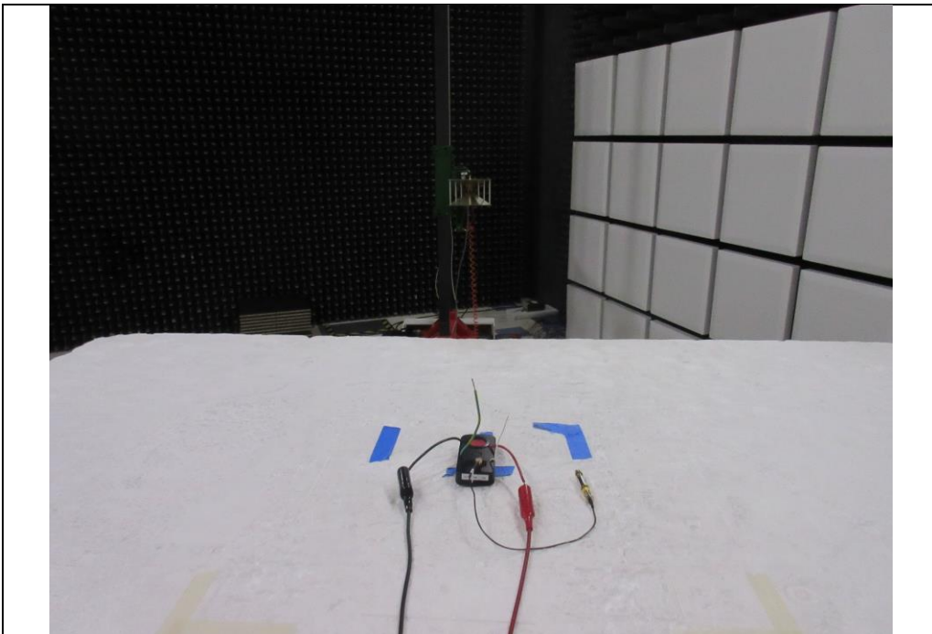
RF Radiated #6
