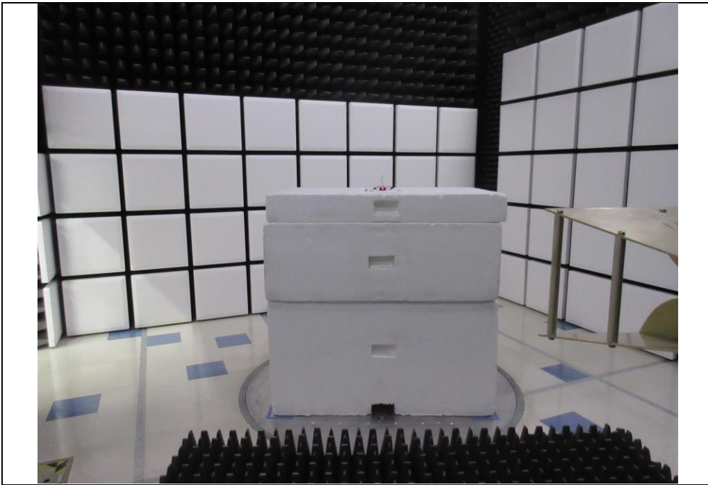
RF Radiated #6
