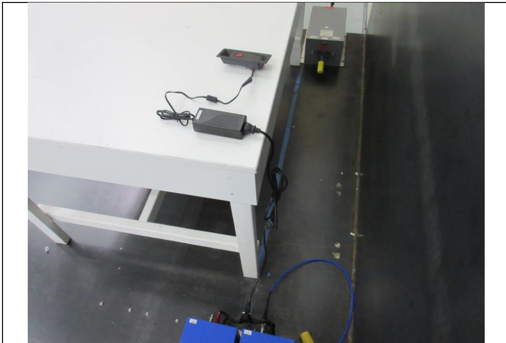
AC Conducted #2
