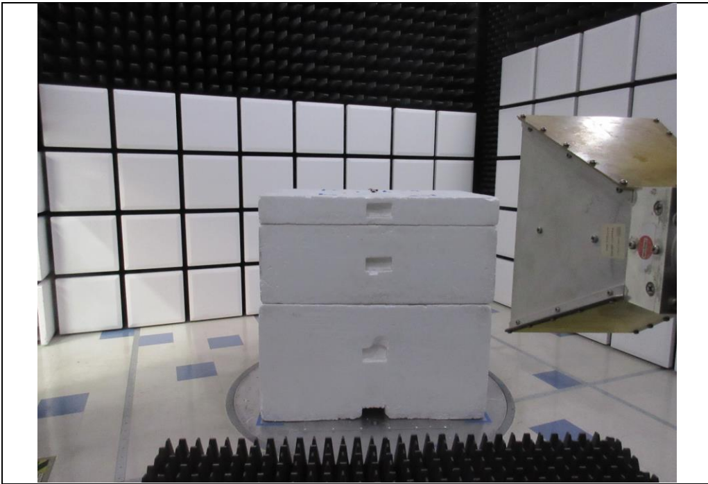
RF Radiated #4
