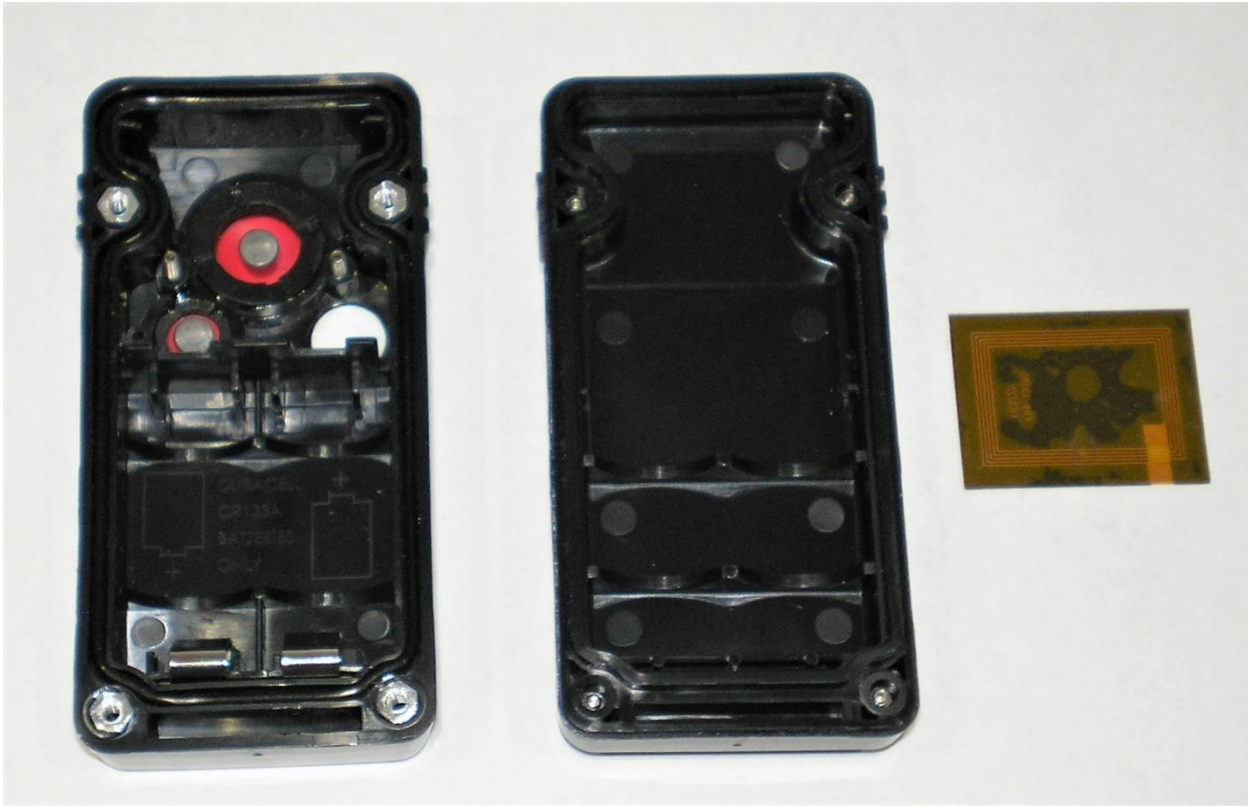
Case interior and NFC antenna. Antenna shown with adhesive side up.
