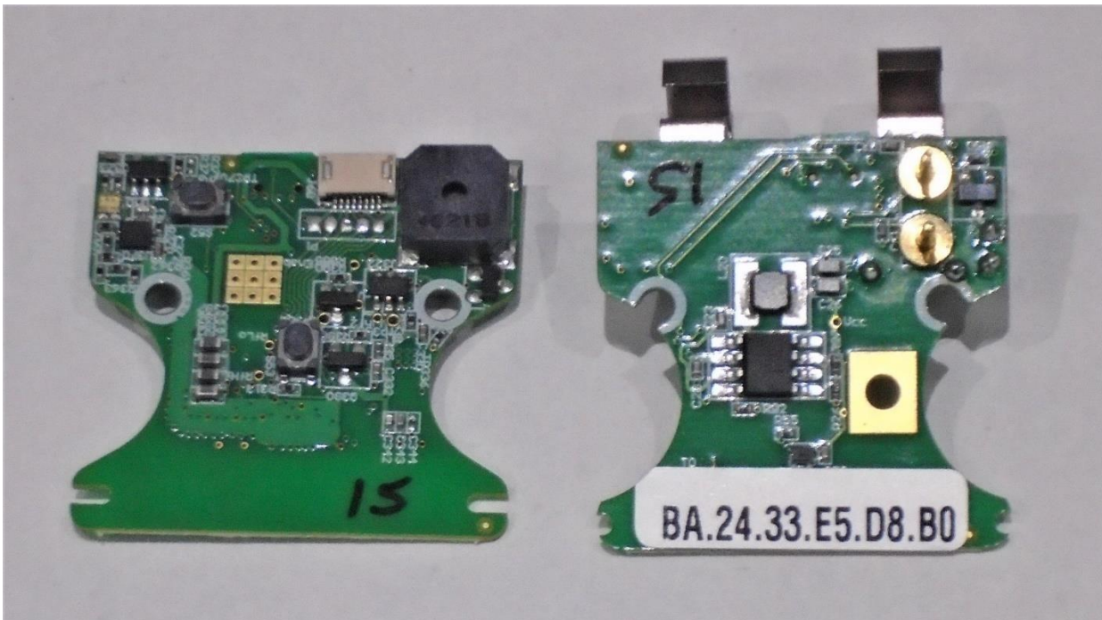
PCB Outer Surfaces (These surfaces face away from one another in the assembled unit)
