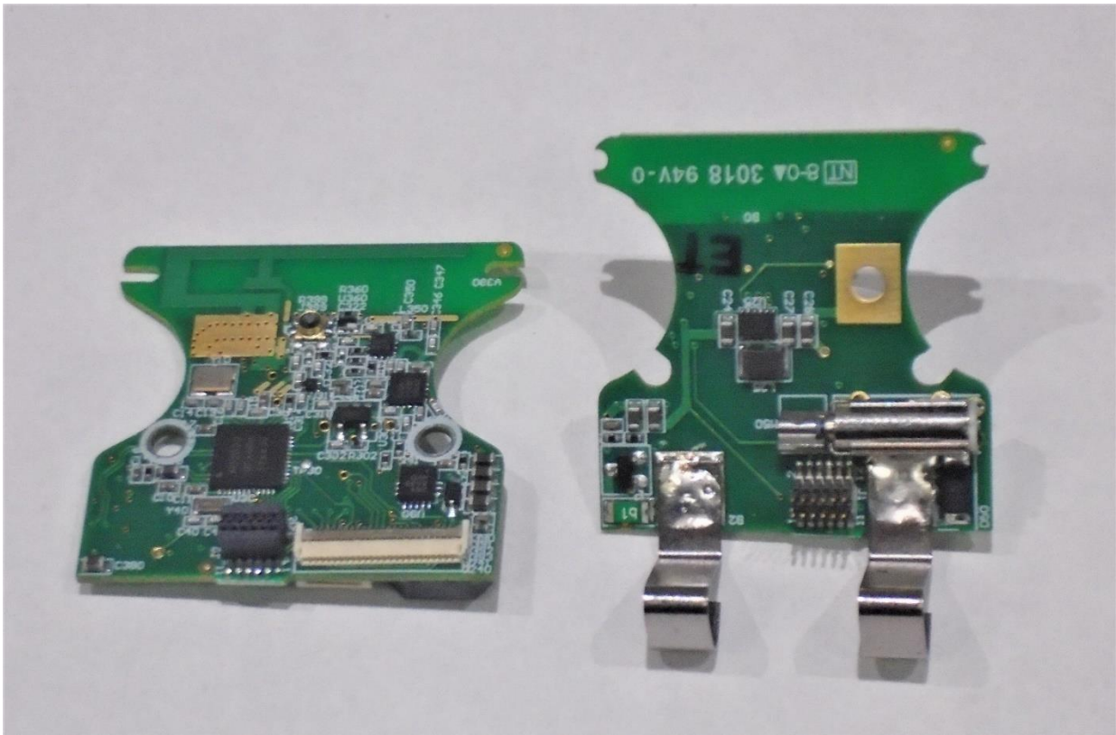
PCB Inner Surfaces (These surfaces face one another in the assembled unit)
