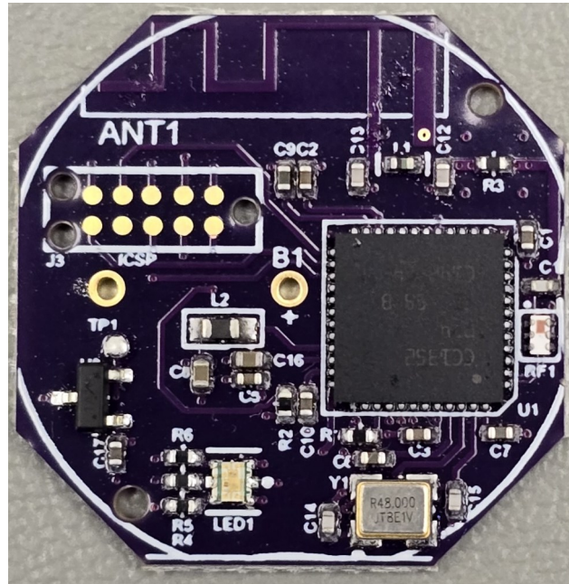
Top of PCB
