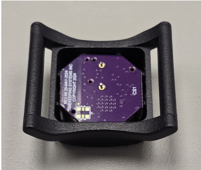
Printed Circuit Board in Housing without Potting
