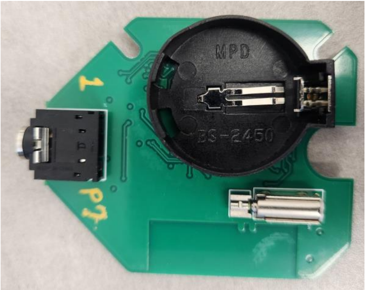
Back of Board
