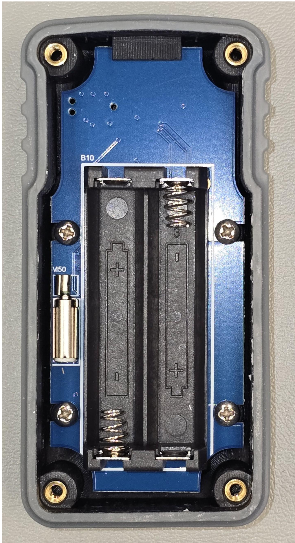
Rear View: Cover removed
