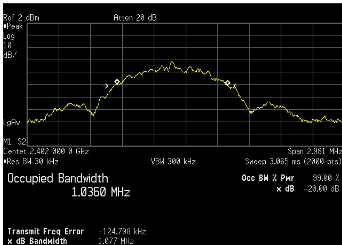
Figure 2. Occupied Bandwidth Plot
