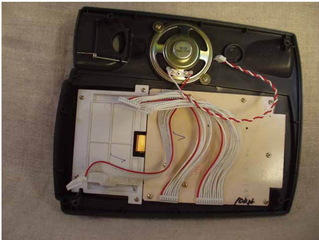
Figure 4: Internal top cover with circuit boards
